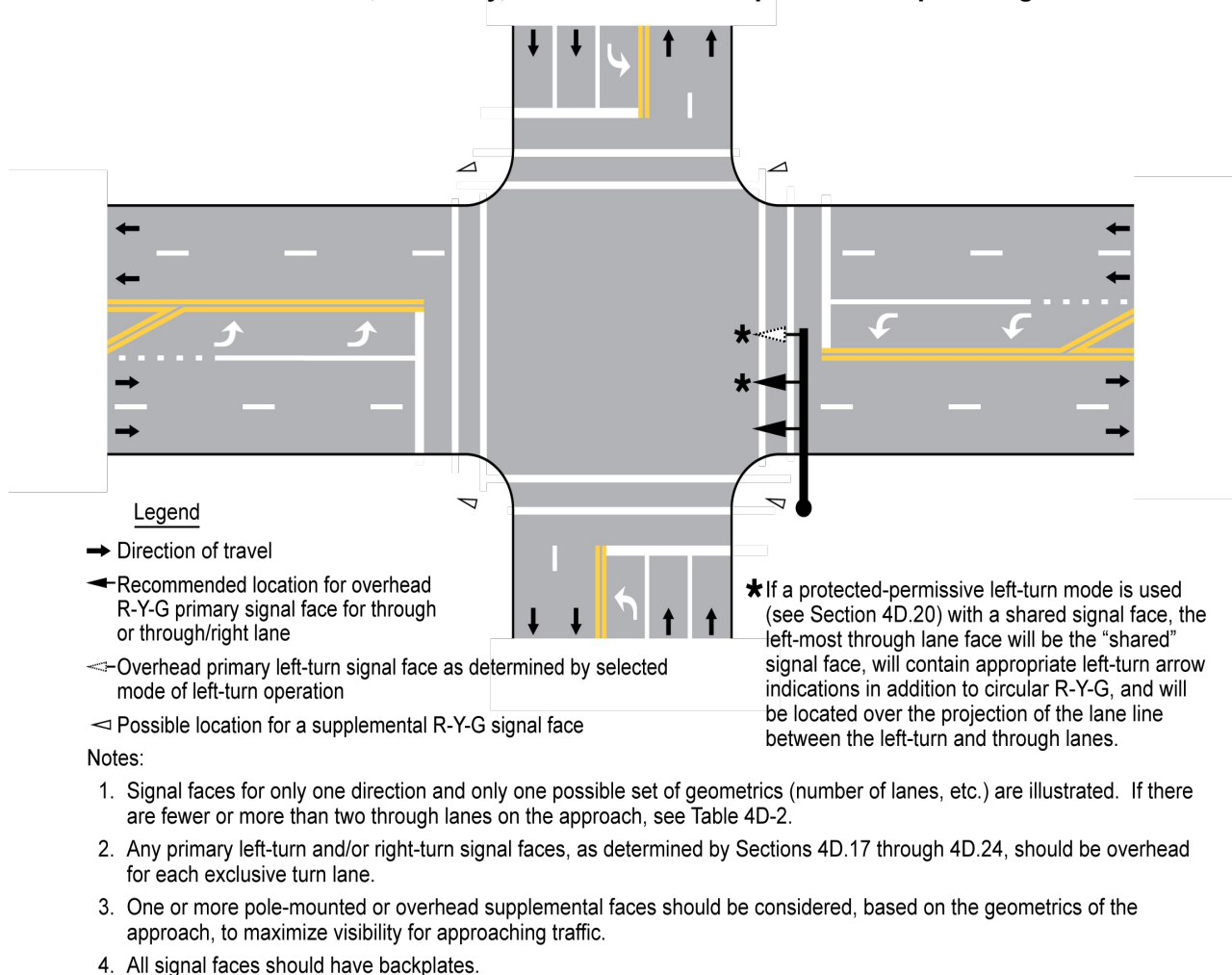
Figure 4D-3. Recommended Vehicular Signal Faces for Approaches with Posted, Statutory, or 85 th -Percentile Speed of 45 mph or Higher
