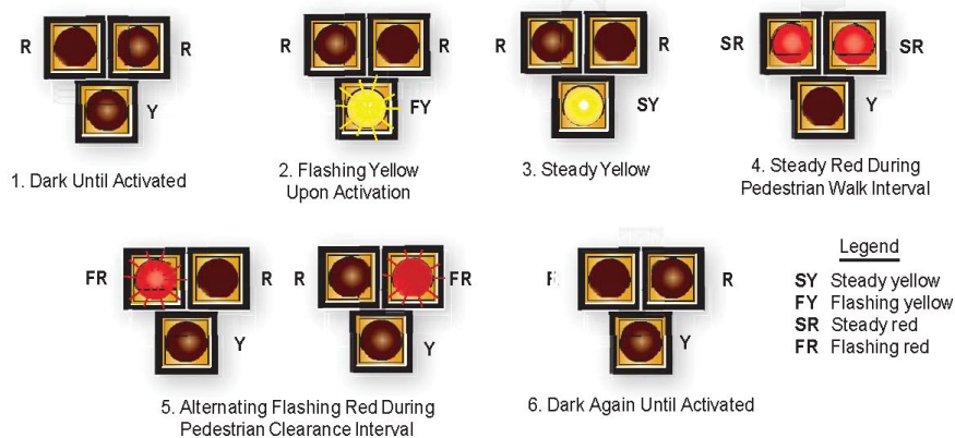
Figure 5-4. Sequence for a Pedestrian Hybrid Beacon
