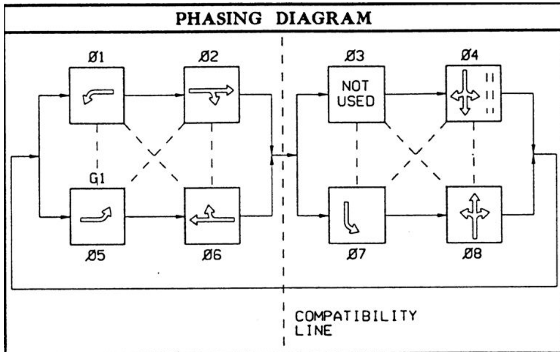
Figure 5-1. Typical phasing diagram.
