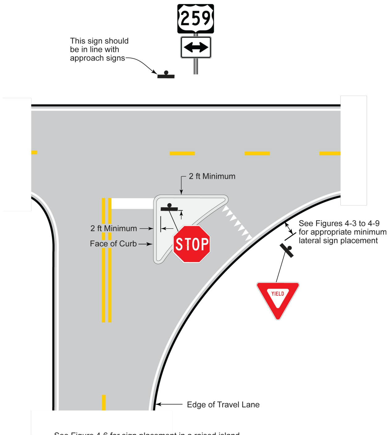
Figure 4-10. Stop/Yield Sign Lateral Placement at a Channelized Intersection
