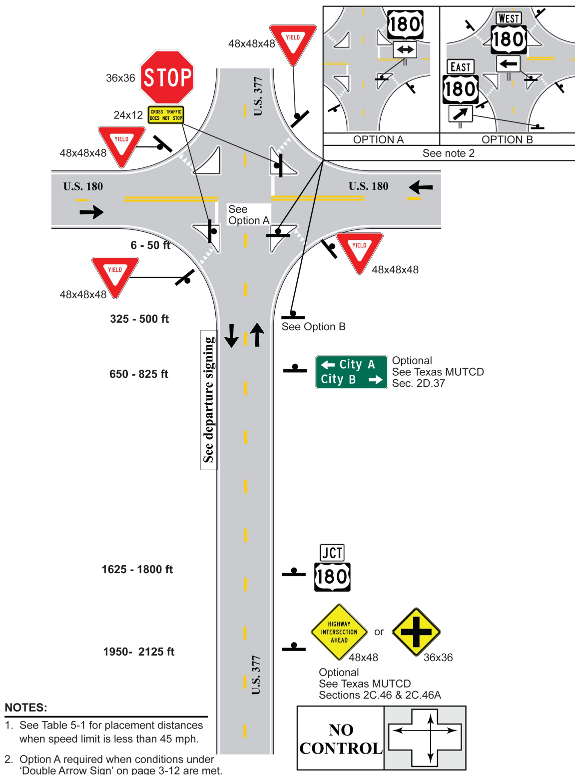
Figure 5-18. 4-Leg, 1 Approach Lane with Free Right Turn, No Control, Approach Lane Goes Through
