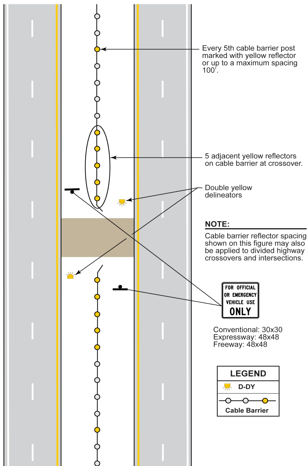
Figure 8-24. Emergency Crossover
