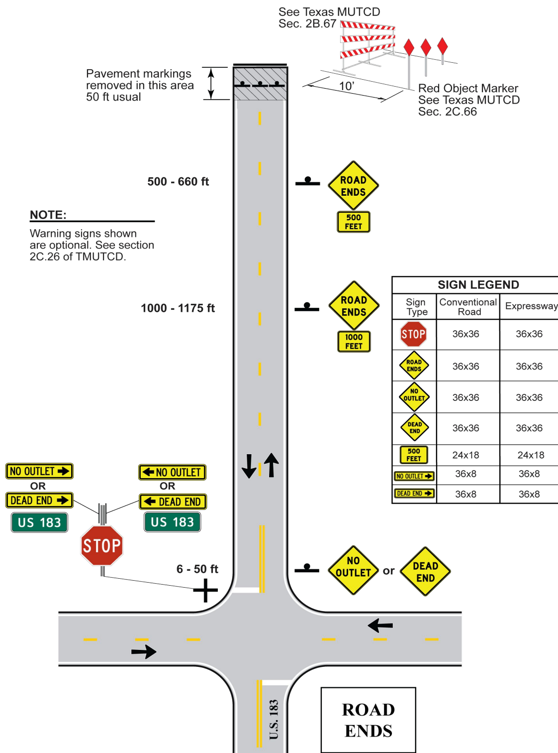
Figure 7-15. Road Ends Signing
