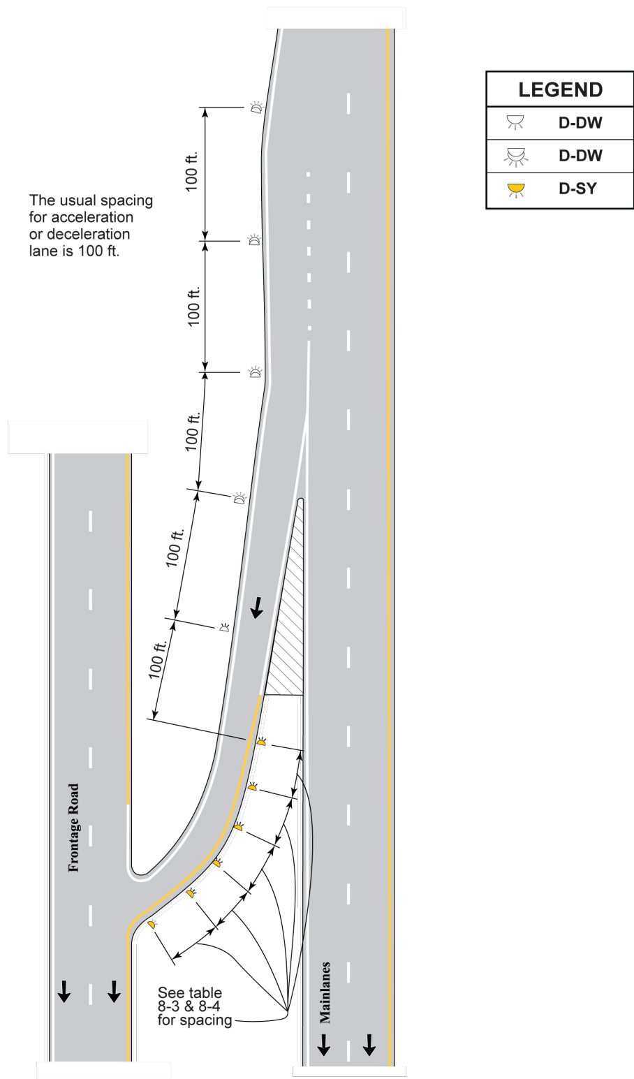
Figure 8-23. One-Way Curved Ramp Detail
