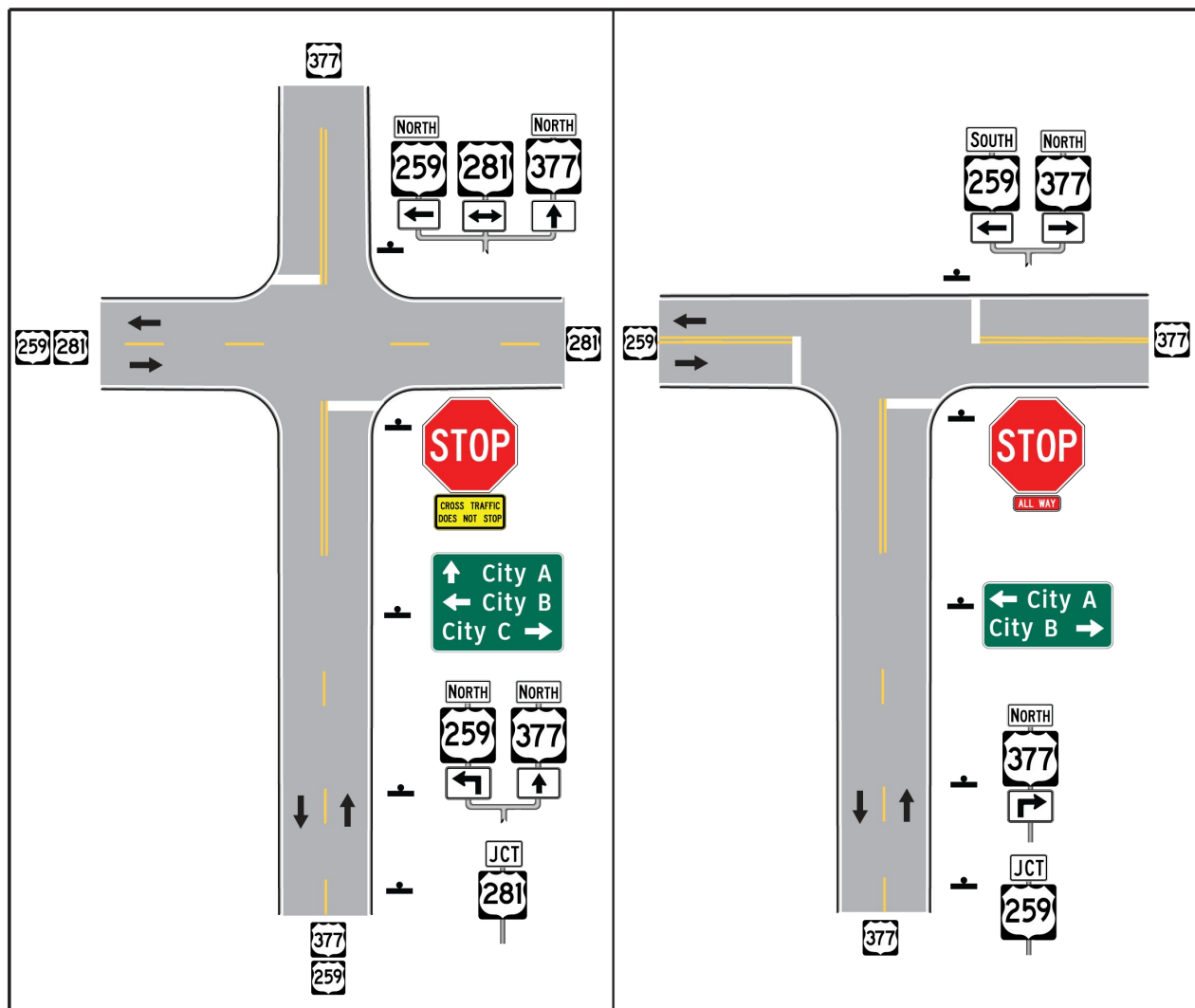
Figure 3-26. Required Applications of Advance Route Turn Assembly
