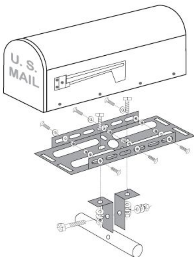
Figure 9-14. Attaching the Bracket to the Multiple Support
