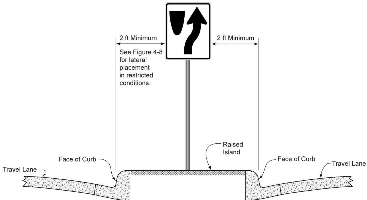
Figure 4-7. Lateral Sign Placement with Raised Island
