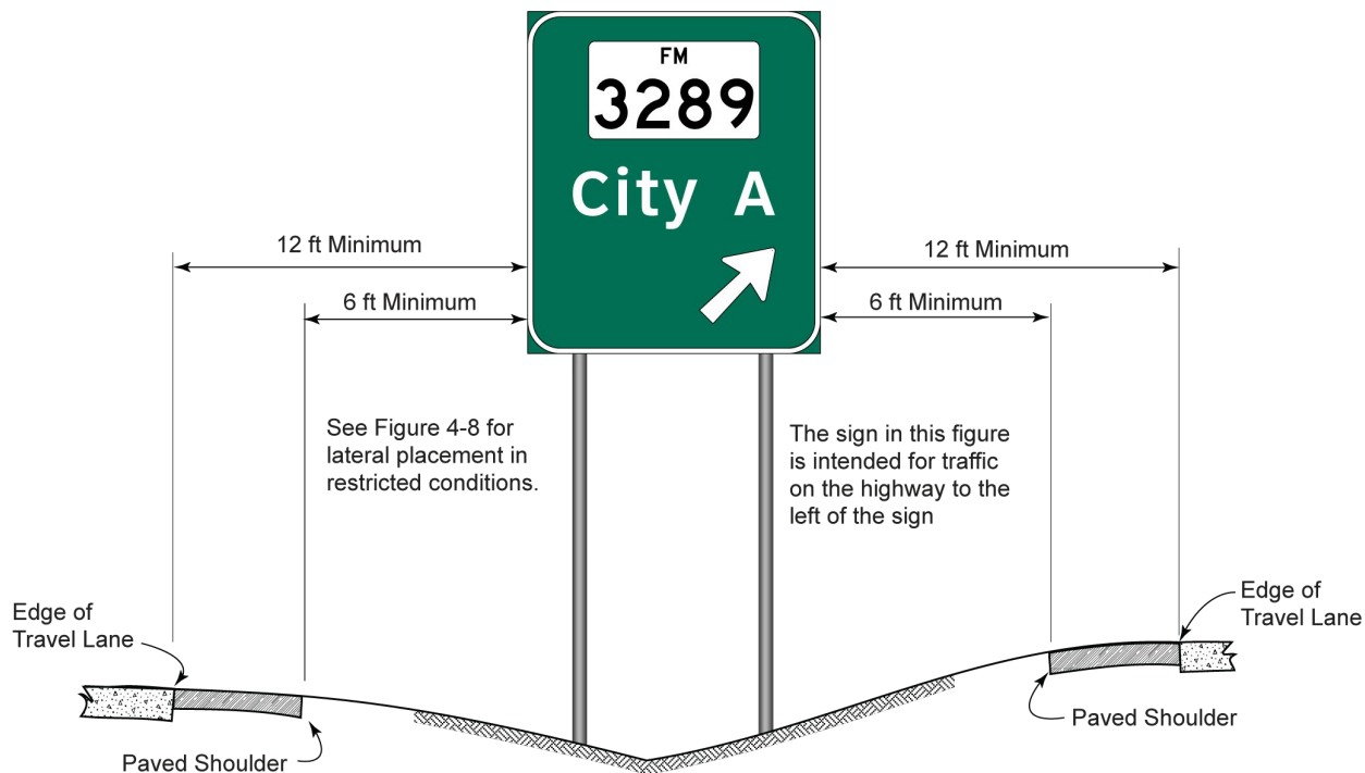
Figure 4-8. Lateral Sign Placement in Restricted Right-of-Way
