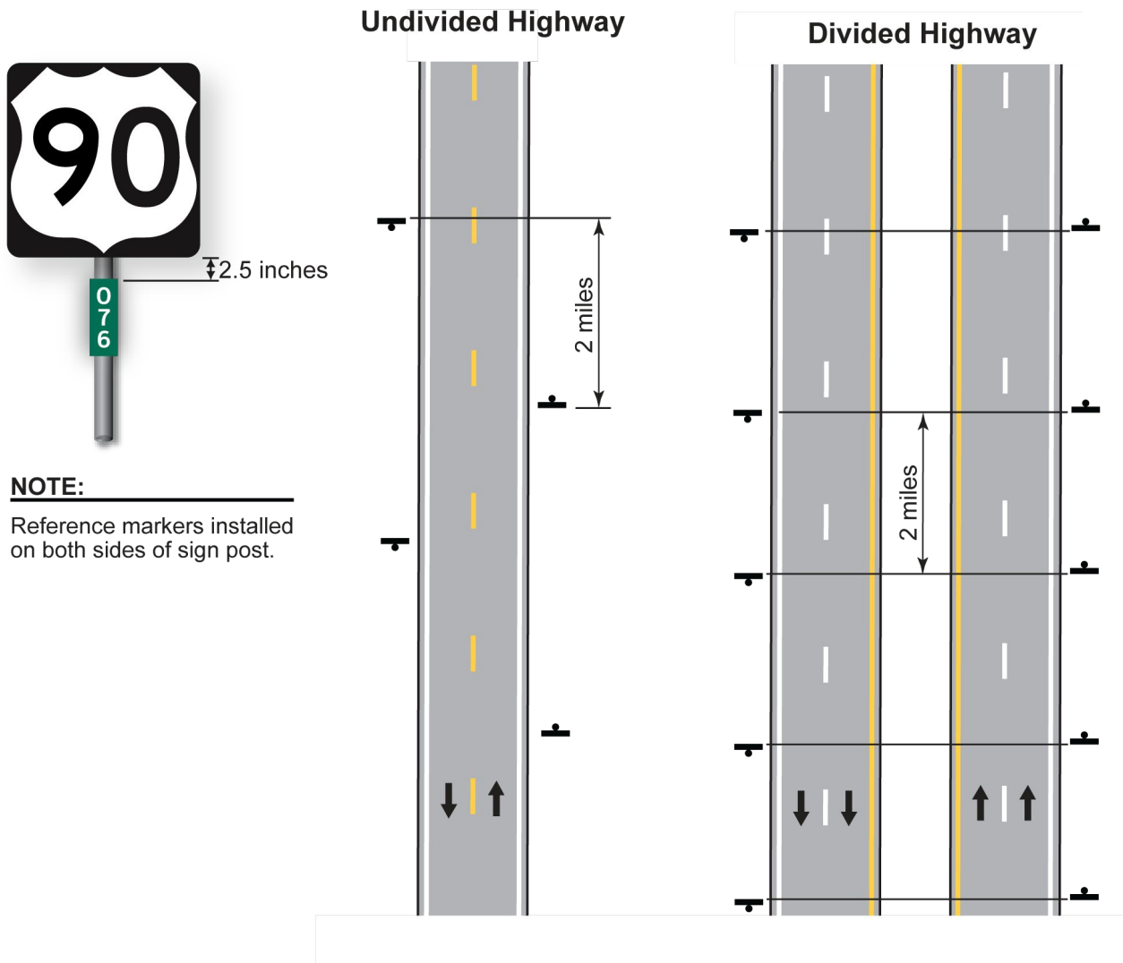
Figure 3-30. Texas Reference Marker Assembly
