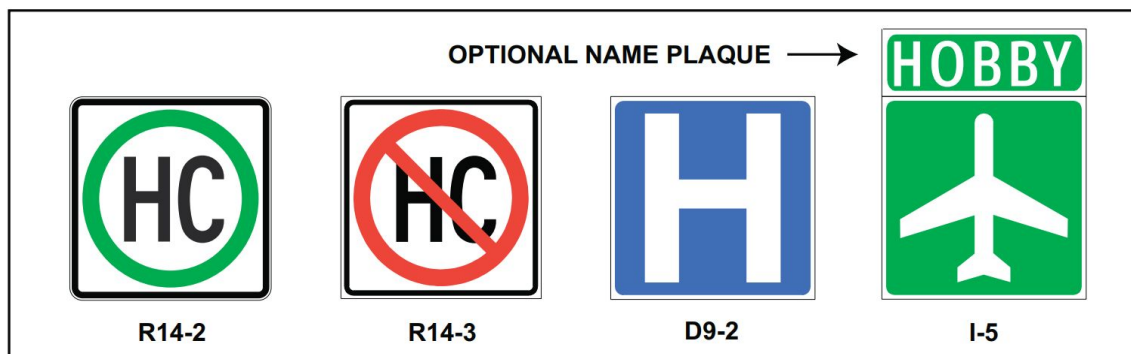
Figure 3-17. Guide Sign Routing plaques.
