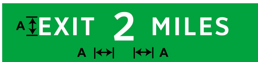
Figure 4-15. Lateral spacing between a word and a mileage numeral.
