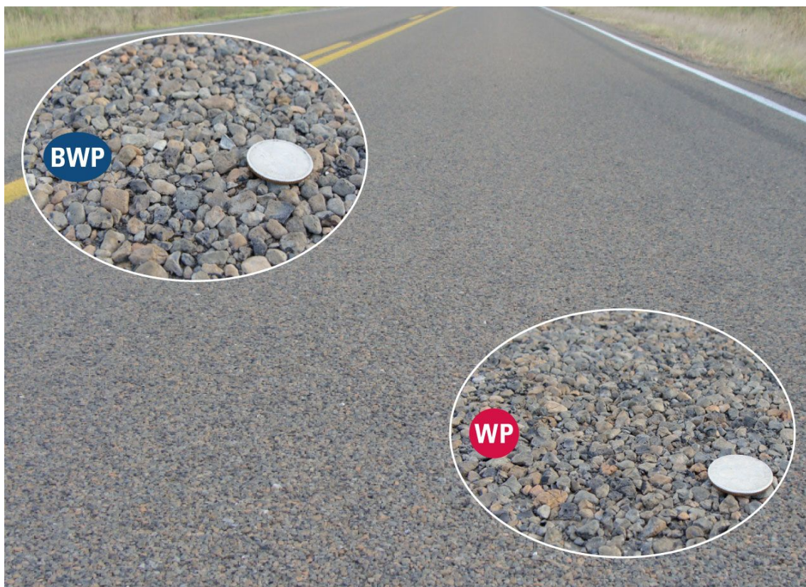
Figure 4-9. Lane with no wheel path color difference.
