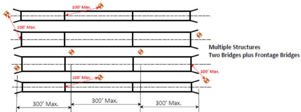
Figure 2–1. Minimum number of test holes for common types of structures
