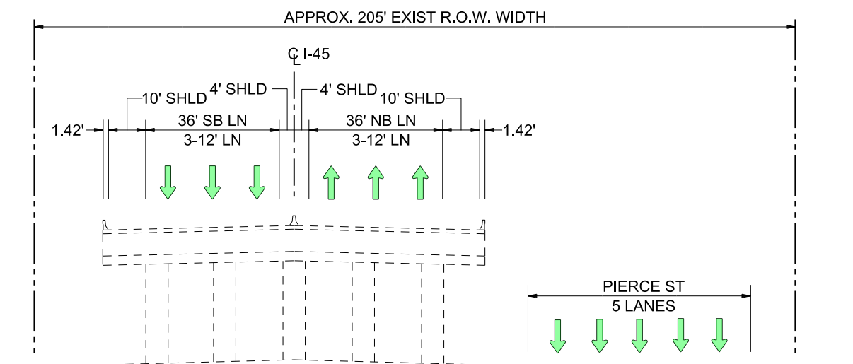
EXISTING I-45 (PIERCE ELEVATED)
