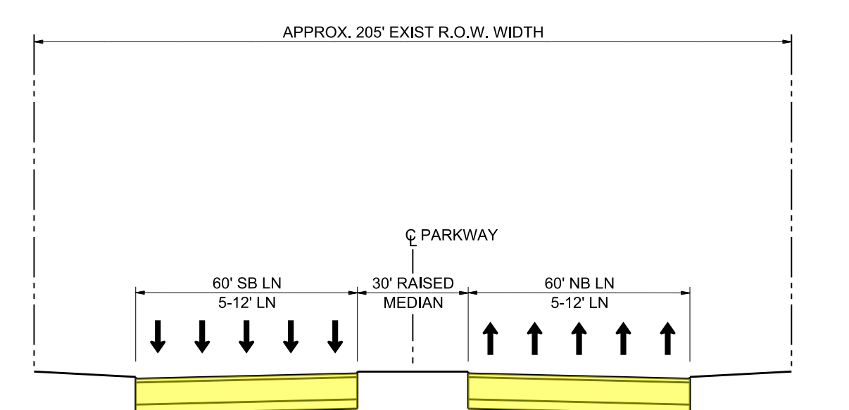
PROPOSED I-45 (PIERCE ELEVATED) SECTION C-C
