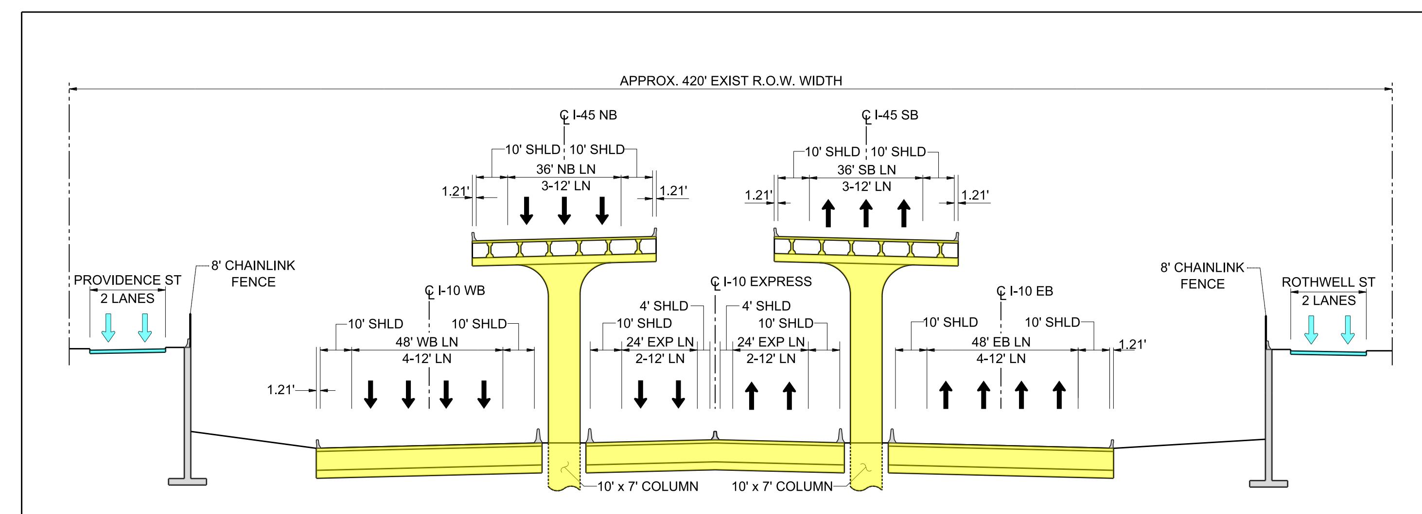
PROPOSED I-10 (DEPRESSED SECTION) SECTION A-A
