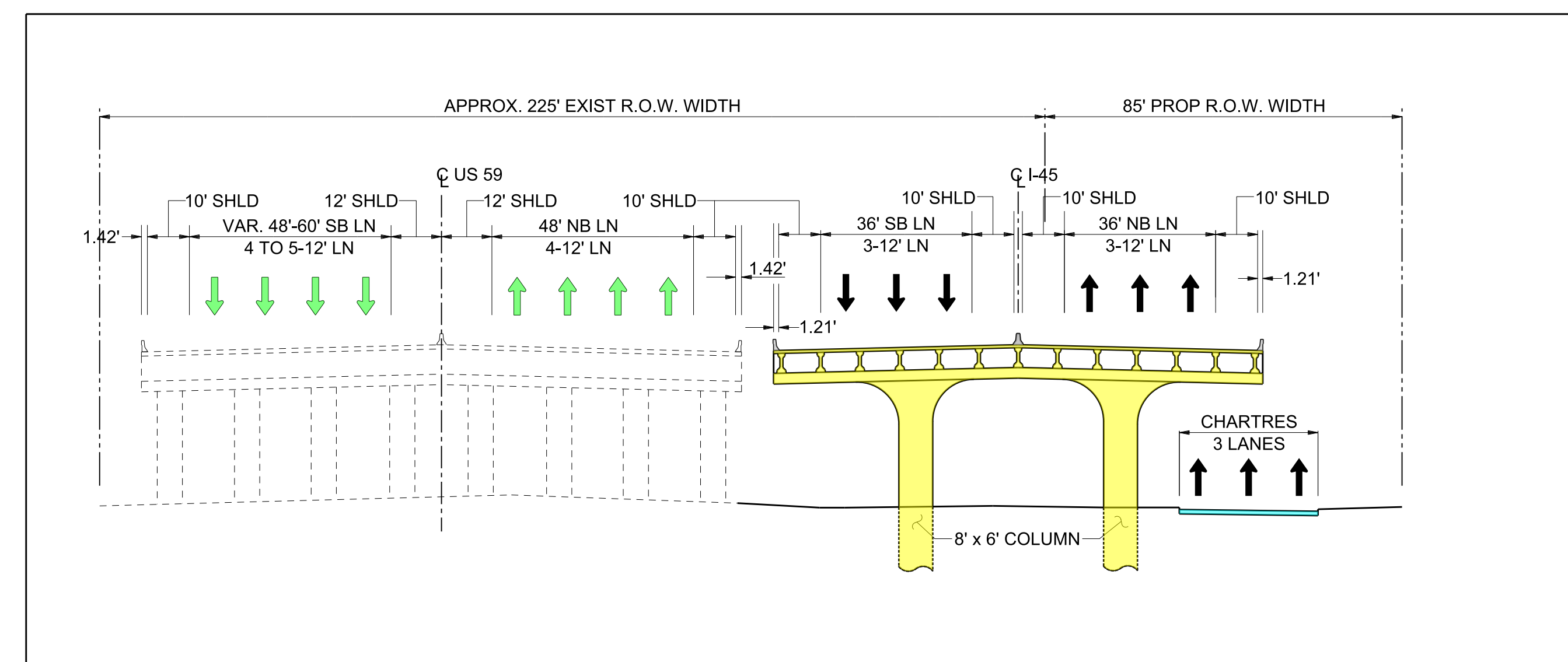
PROPOSED US 59 SECTION B-B
