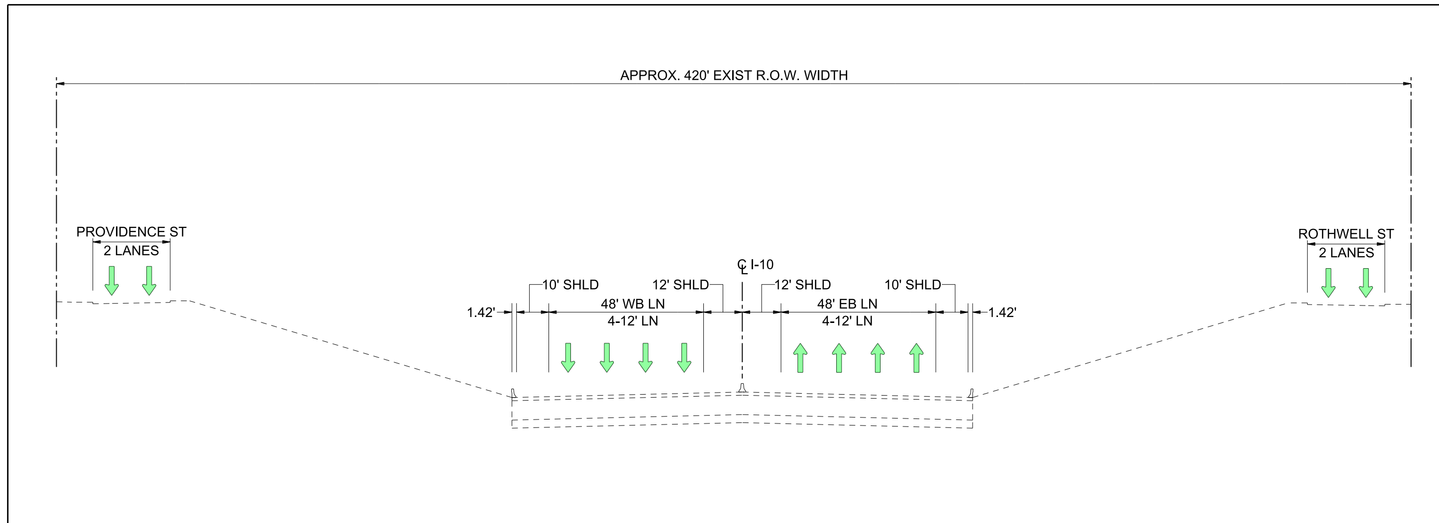
EXISTING I-10 (DEPRESSED SECTION)
