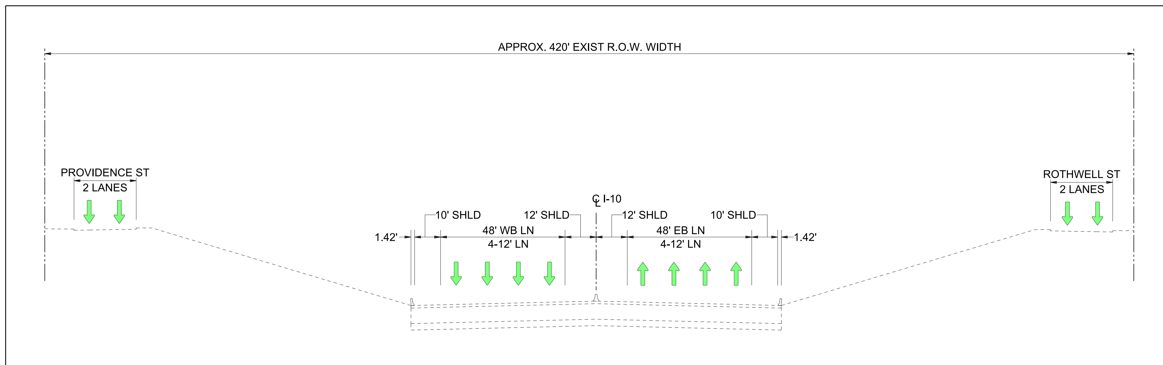
EXISTING I-10 (DEPRESSED SECTION)
