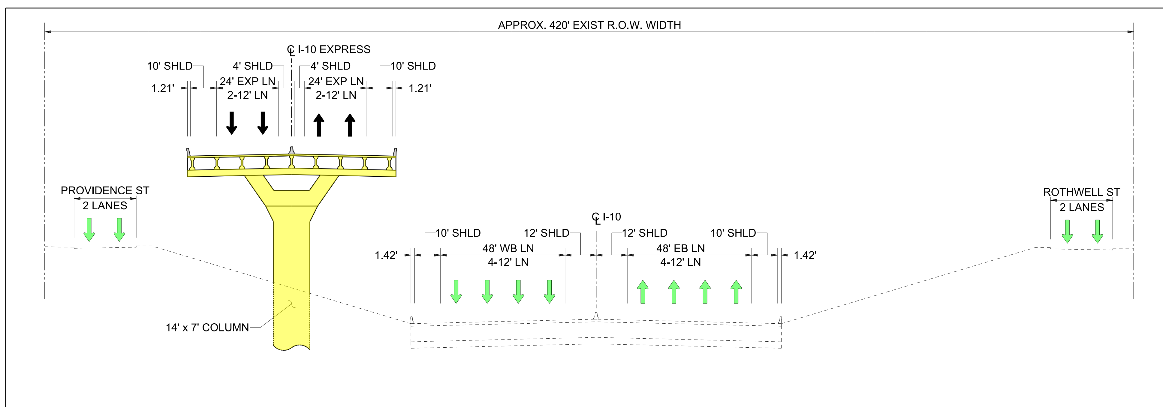
PROPOSED I-10 (DEPRESSED SECTION) SECTION B-B
