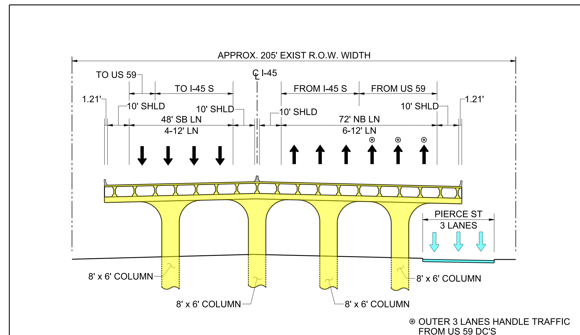
PROPOSED I-45 (PIERCE ELEVATED) SECTION A-A
