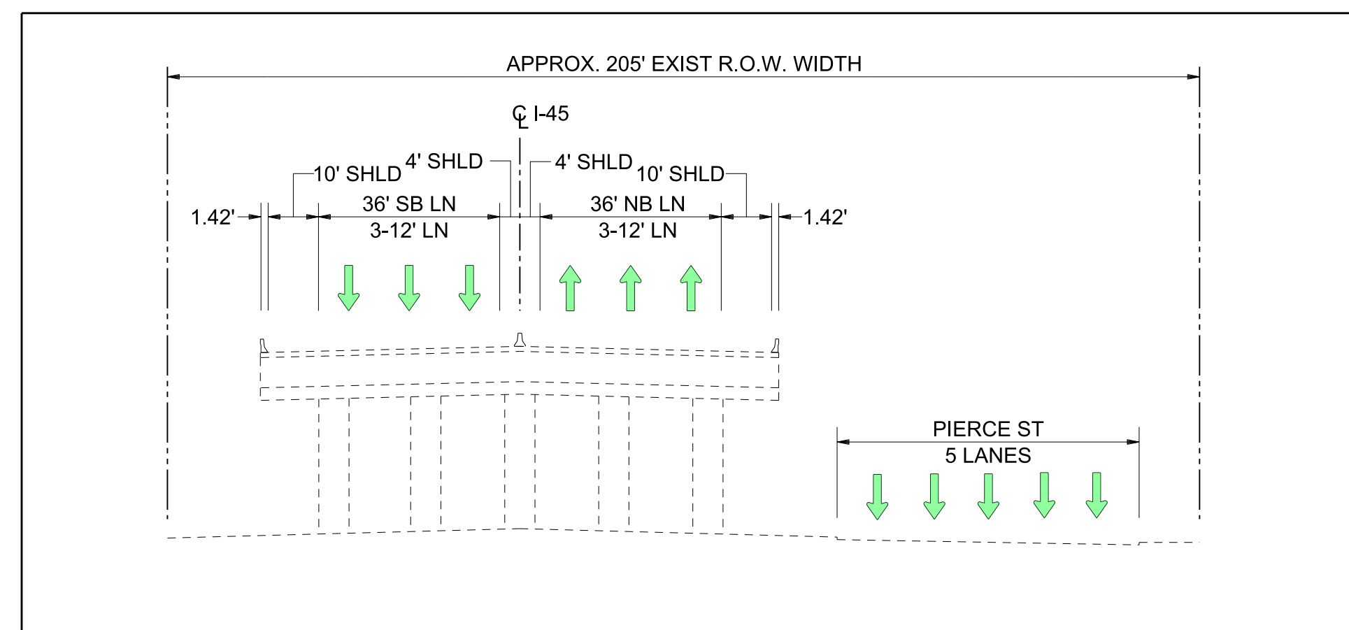
EXISTING I-45 (PIERCE ELEVATED)
