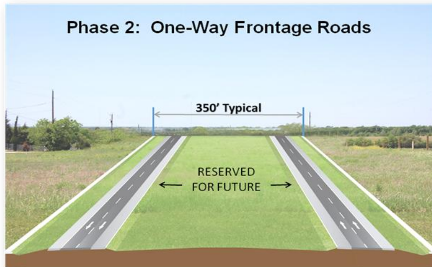
Figure 2b: Phase 2 – One-Way Frontage Roads
