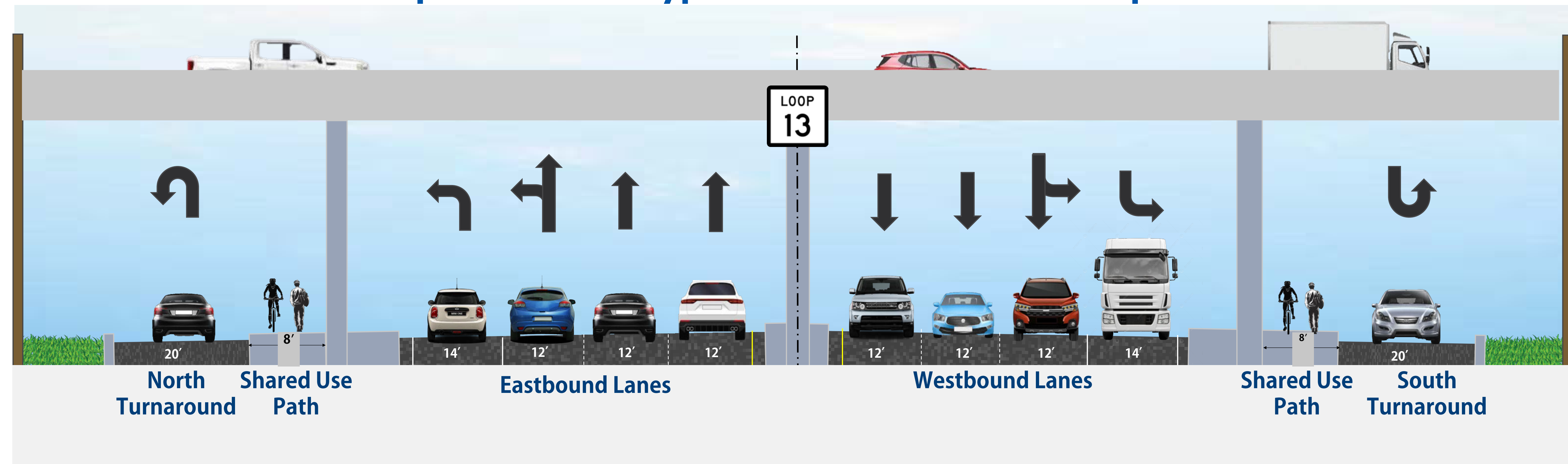
Proposed SL 13 Typical Section at I-37 Overpass
