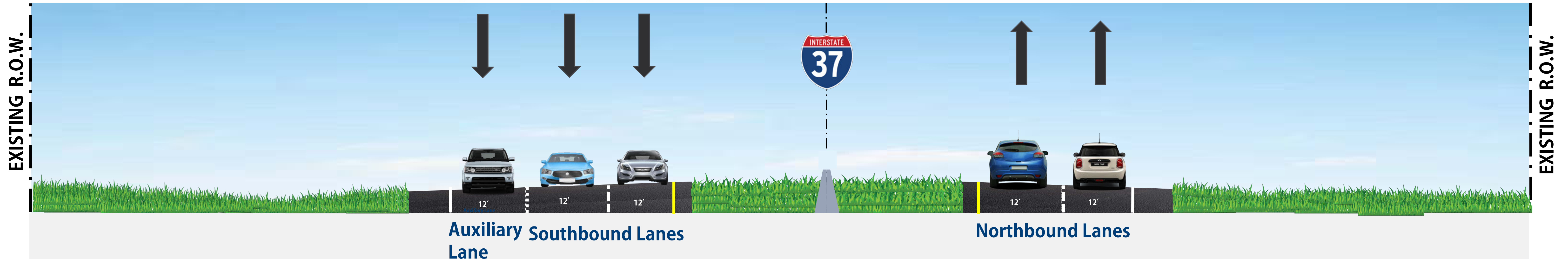
Proposed Typical Section Between SL 13 & I-410 Ramps
