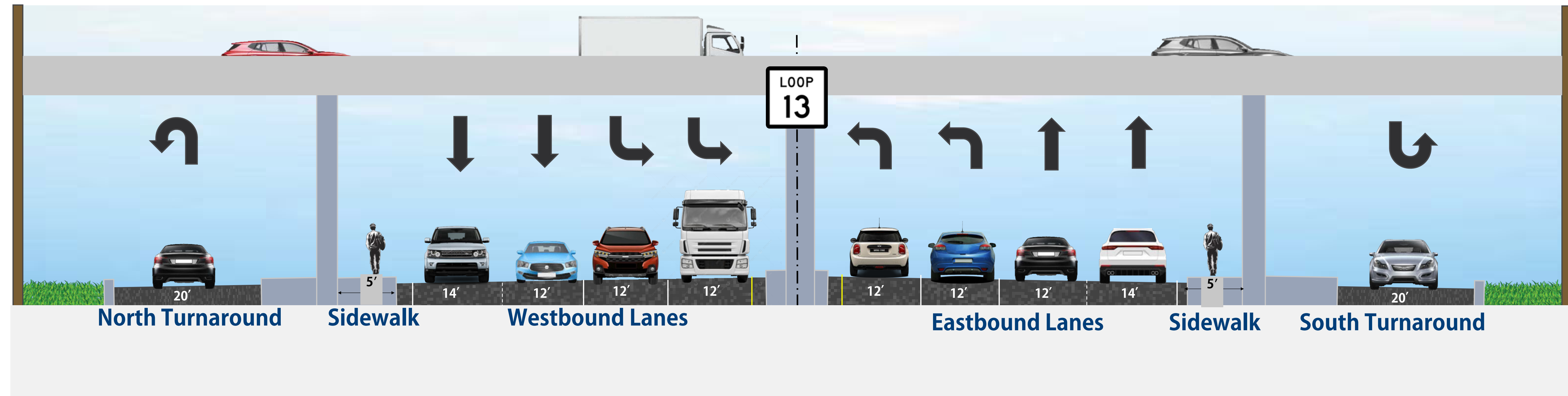
Existing SL 13 Typical Section at I-37 Overpass
