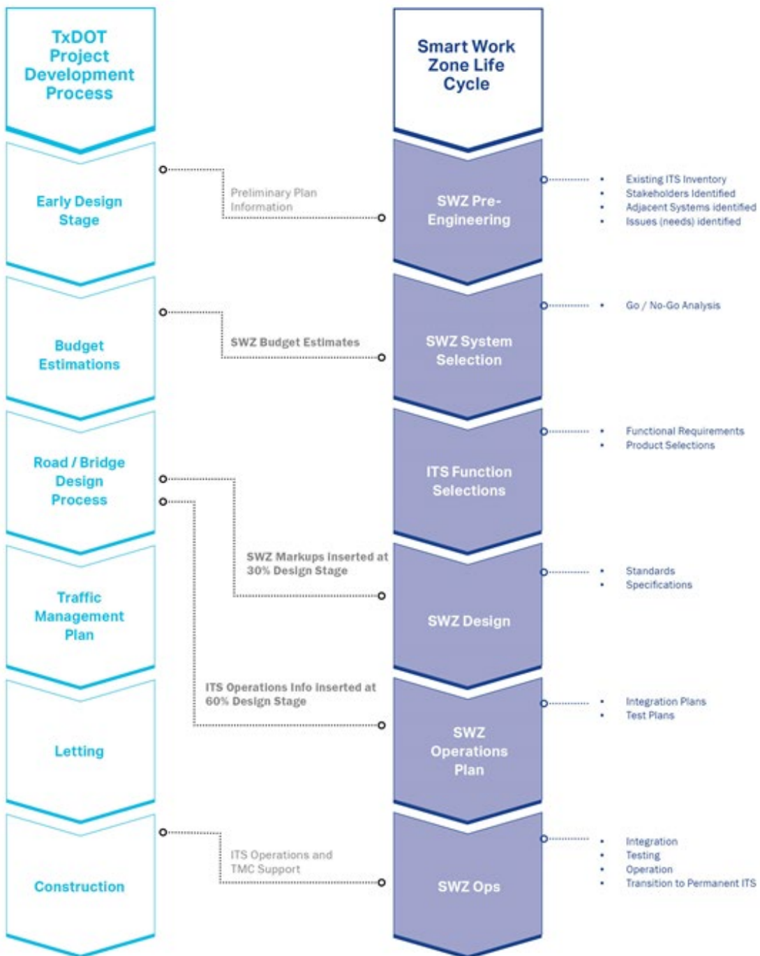
Figure 1: Timeline showing the TxDOT Construction Process and Smart Work Zone Life Cycle
