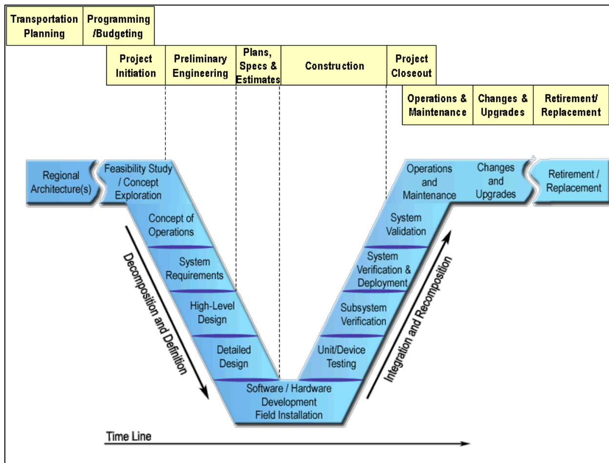
Figure 2: FHWA Systems Engineering Process “V” Diagram
