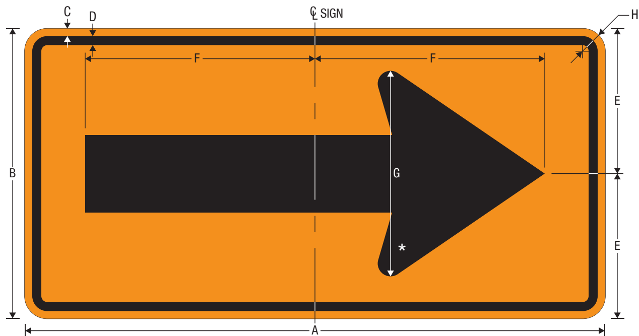
CW1-6R Large Arrow (1-Direction)
