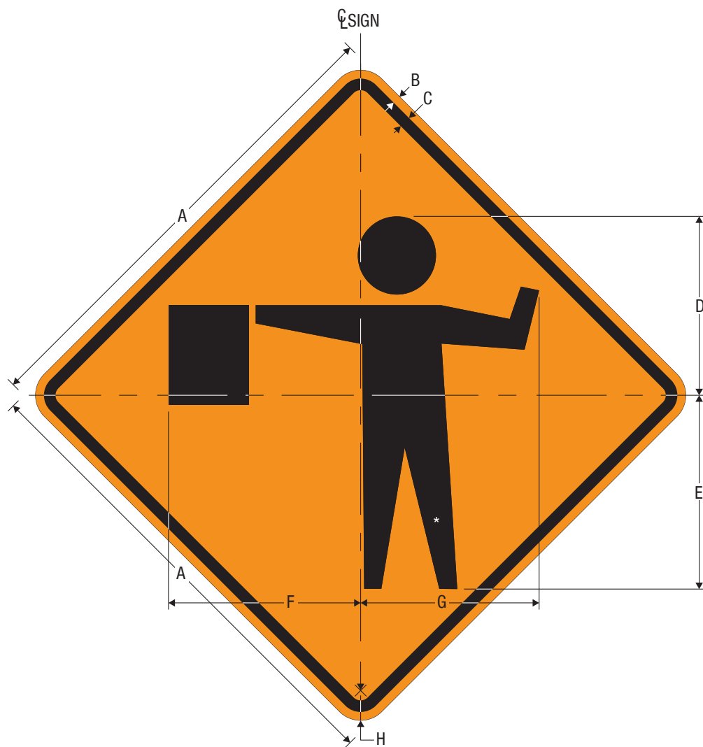
CW20-7 FLAGGER
