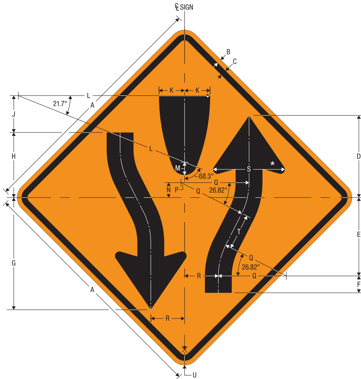
CW6-1 Divided Highway
