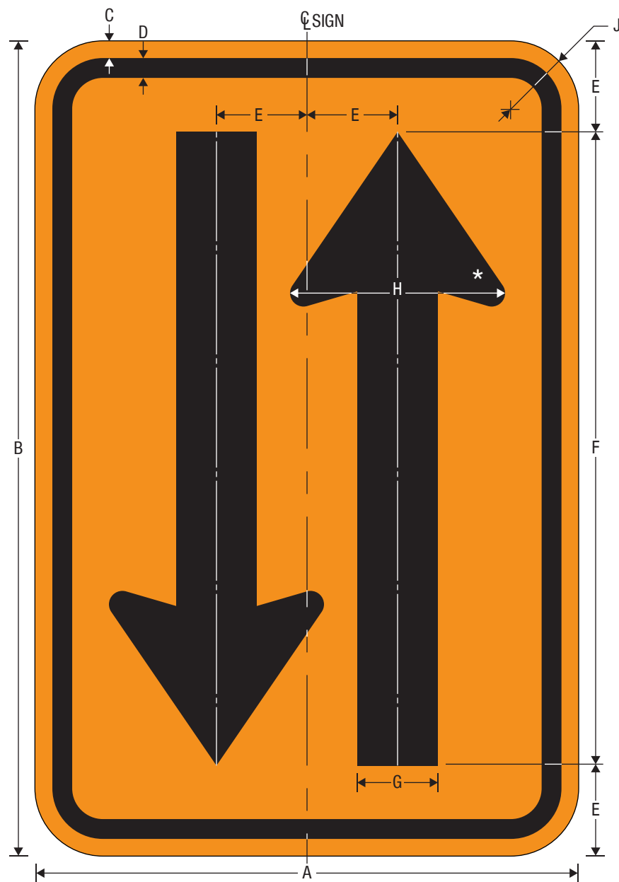
CW6-4 Narrow Two-Way Traffic
