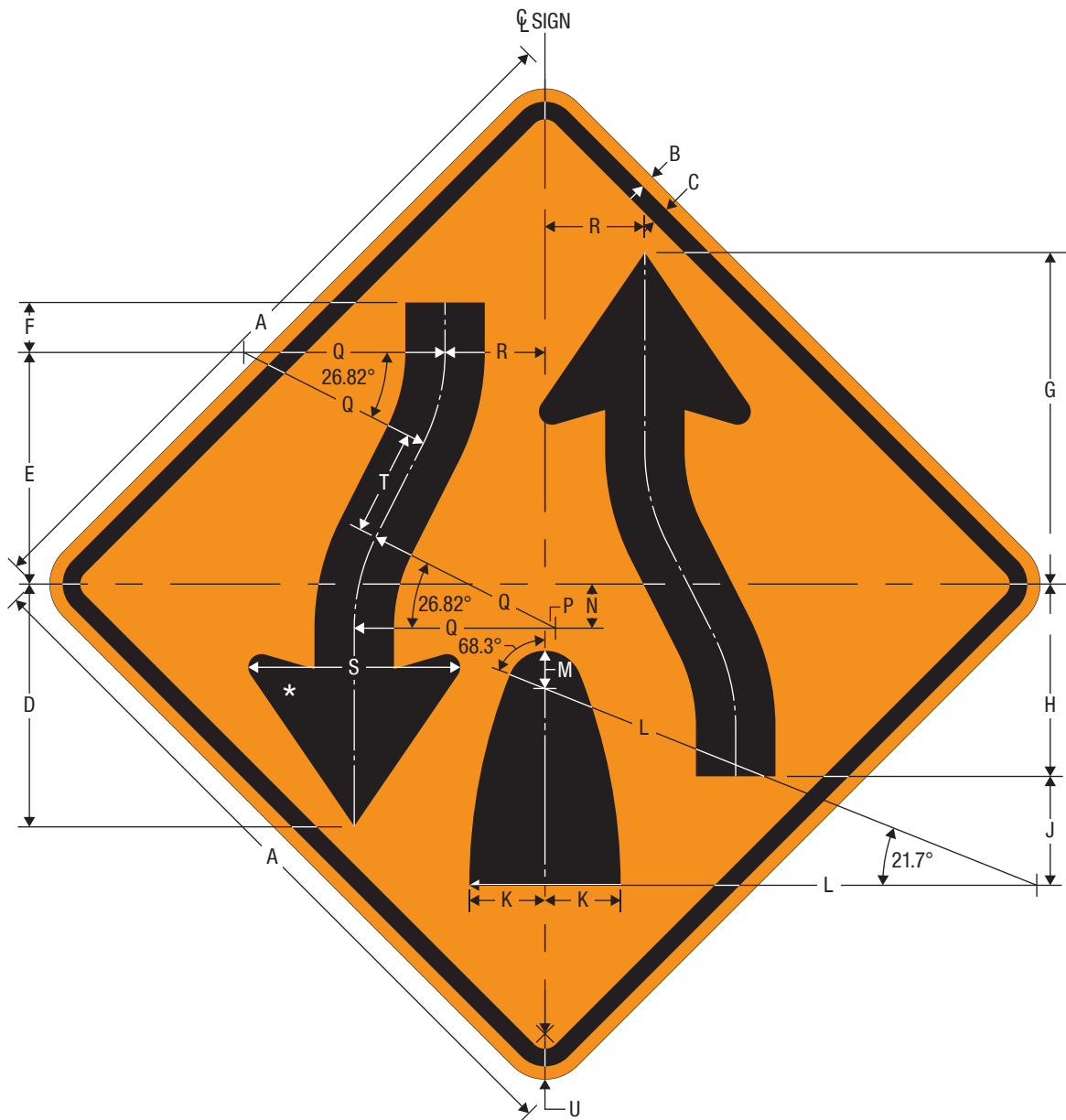
CW6-2 Divided Highway Ends
