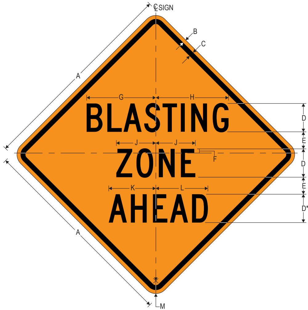
CW22-1[D] BLASTING ZONE AHEAD
