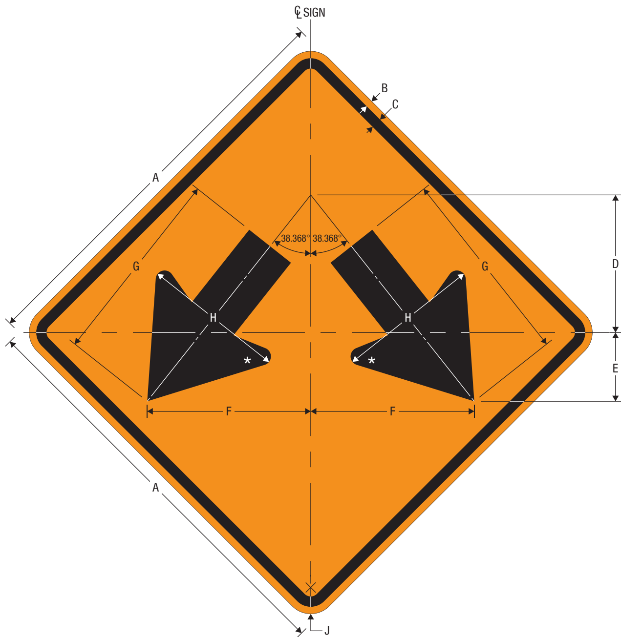
CW12-1 Double Arrow
