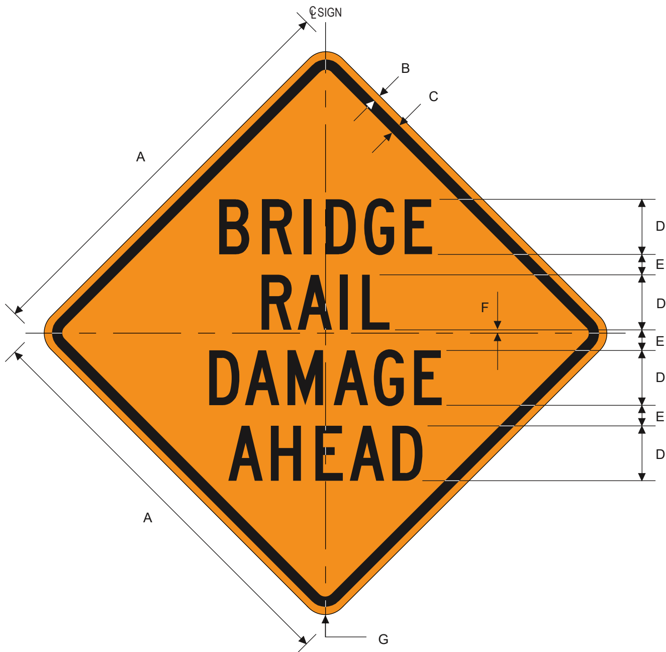
CW21-18T BRIDGE RAIL DAMAGE AHEAD
