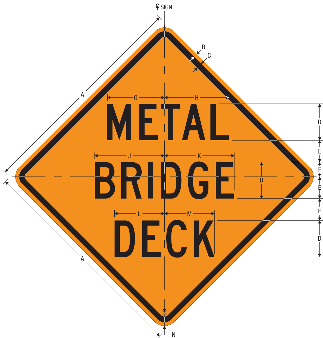
CW8-16 METAL BRIDGE DECK
