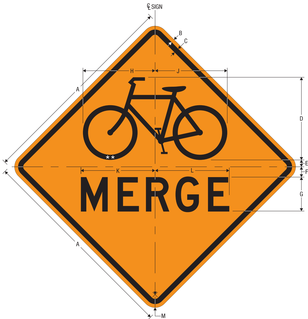
CW9-5a Bicycles Merging
