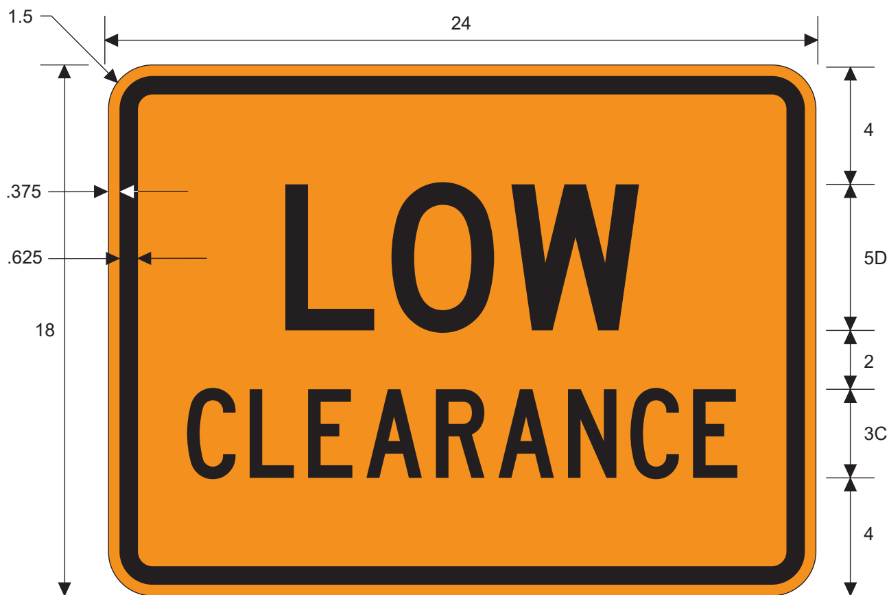
CW12-2PT Low Clearance (Plaque)
