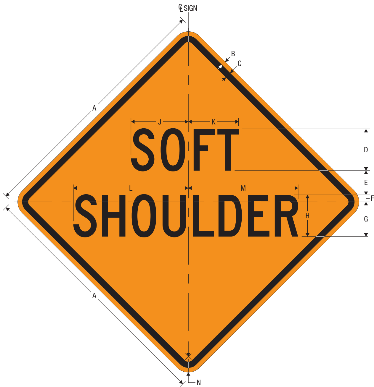
CW8-4 SOFT SHOULDER
