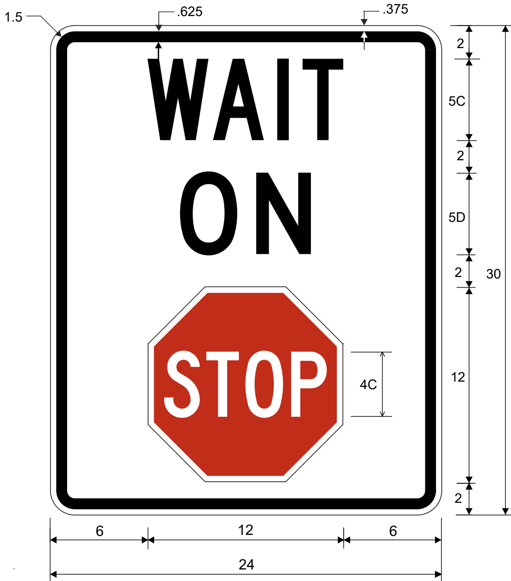
R1-7aT WAIT ON Stop
