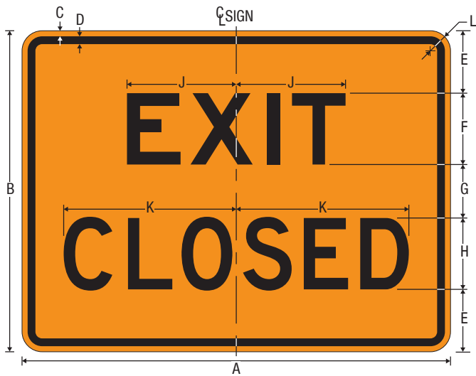
E5-2a EXIT CLOSED
