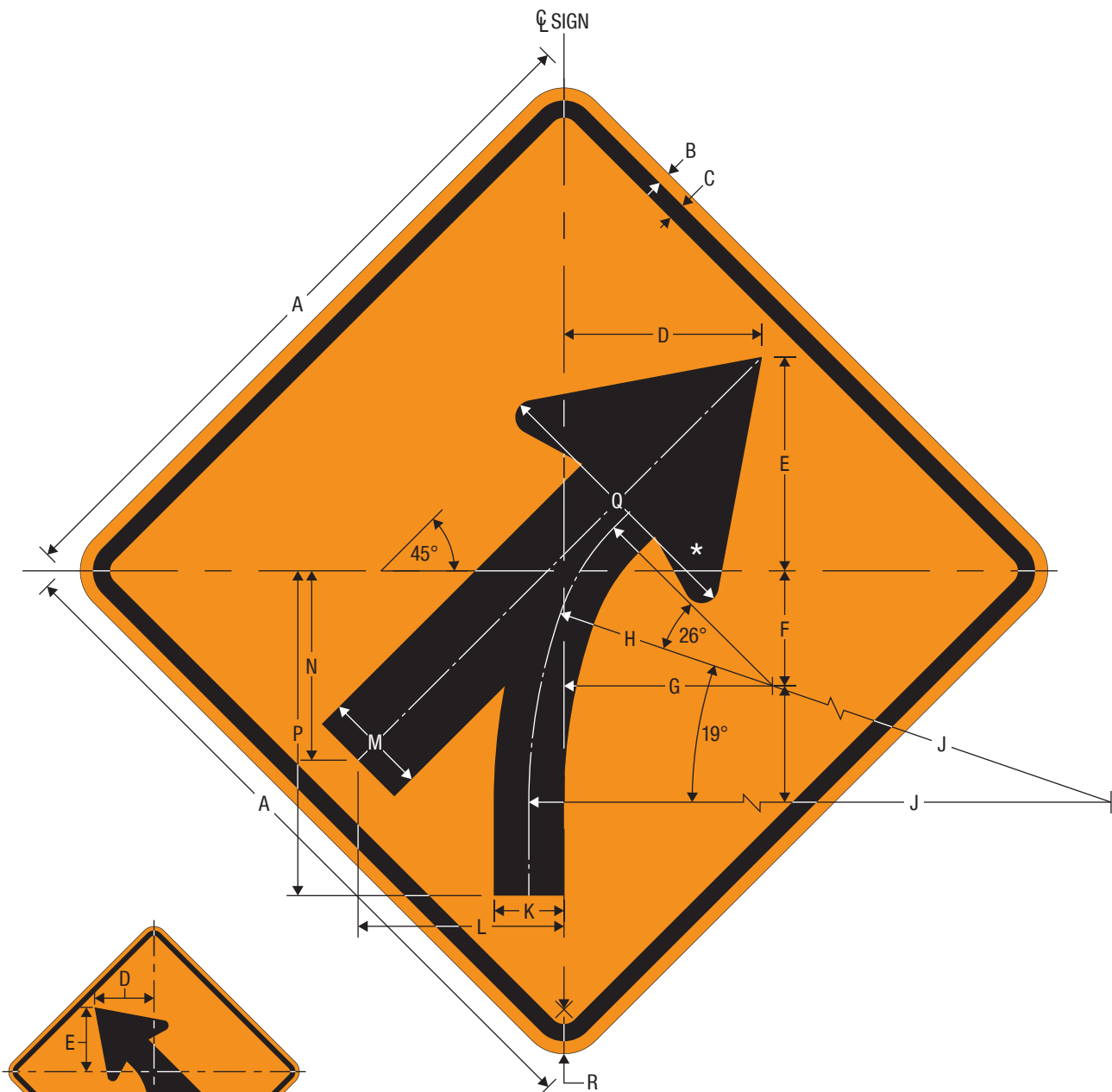
CW4-5R Entering Roadway Merge
