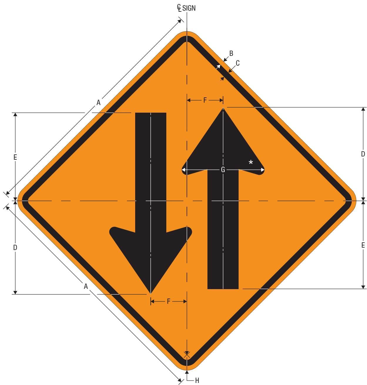
CW6-3 Two-Way Traffic
