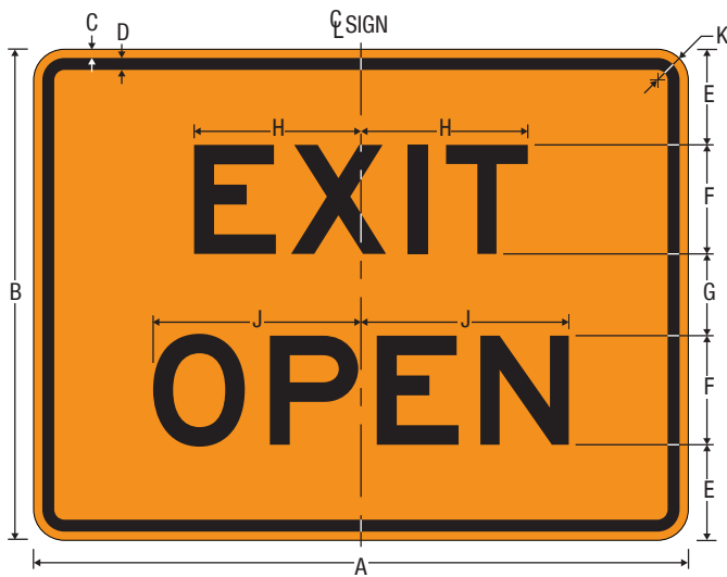
E5-2 EXIT OPEN
