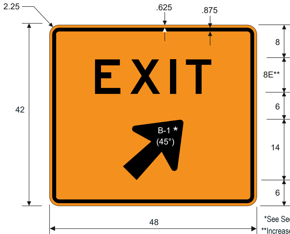
E5-4aT EXIT GORE (with 45 Degree Arrow)
