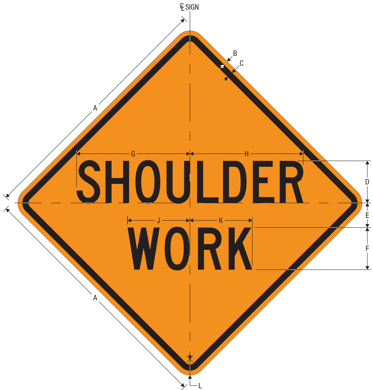
CW21-5 SHOULDER WORK
