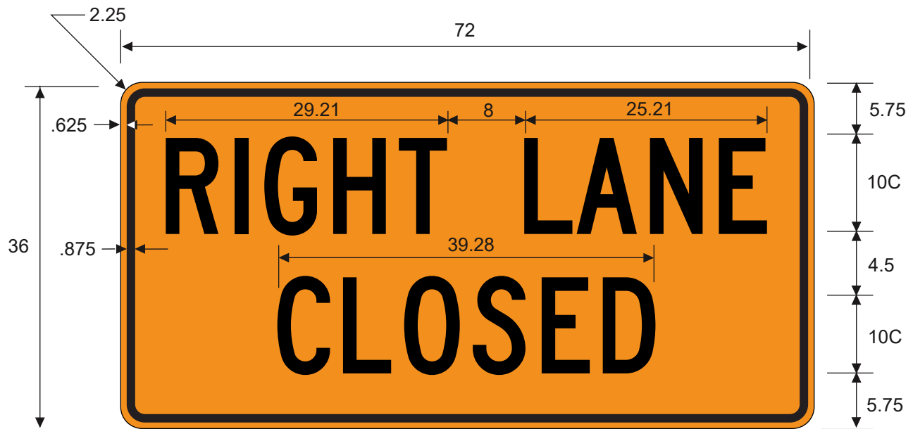
CW20-5cTR RIGHT LANE CLOSED
