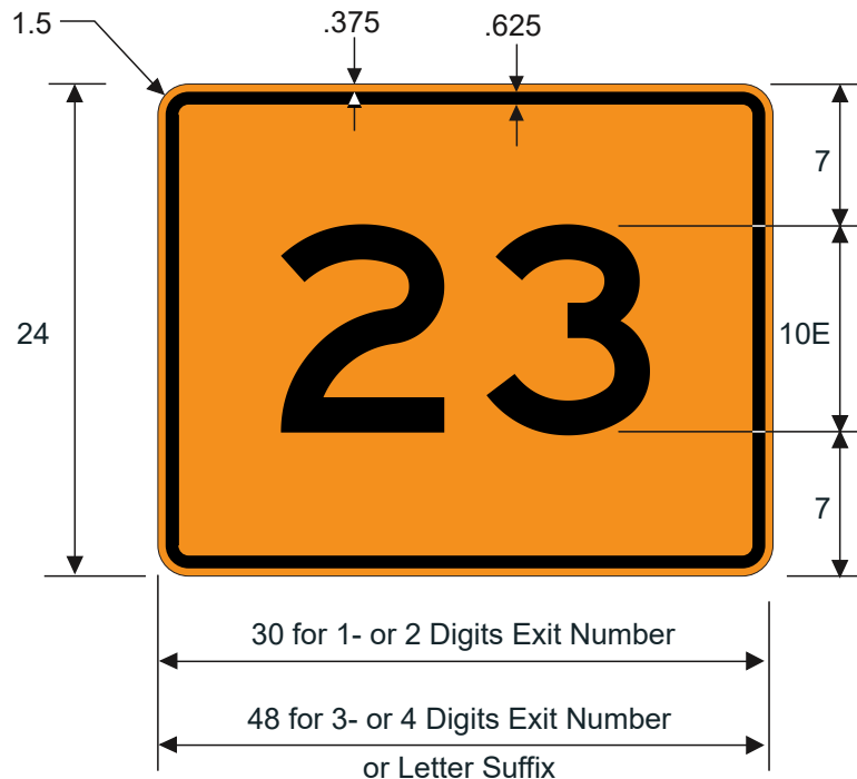
E5-4aPT Exit Number (Plaque)
