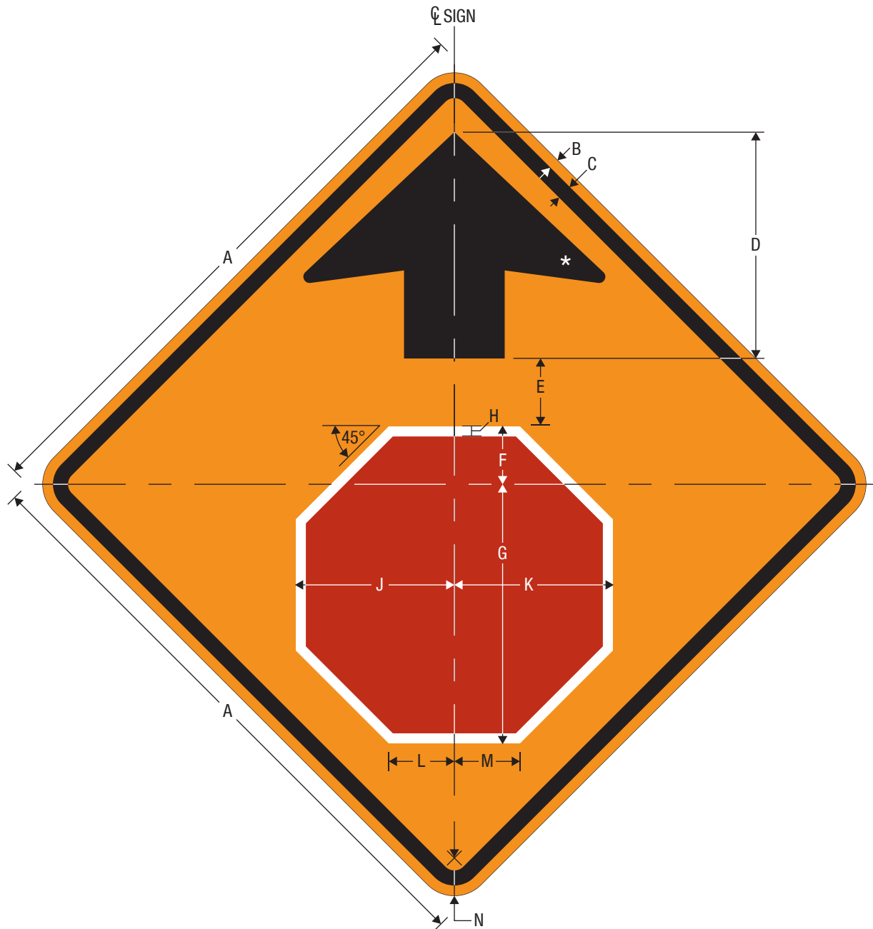
CW3-1 Stop Ahead
