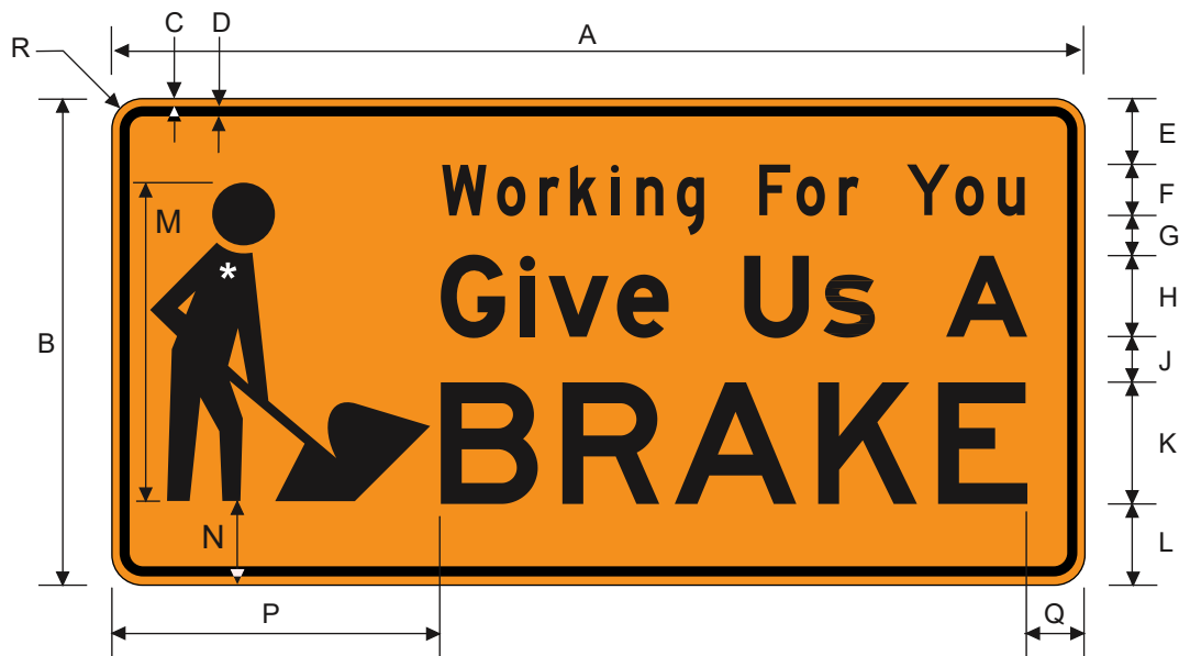
G20-7T WORKING FOR YOU GIVE US A BRAKE (with Symbol)
