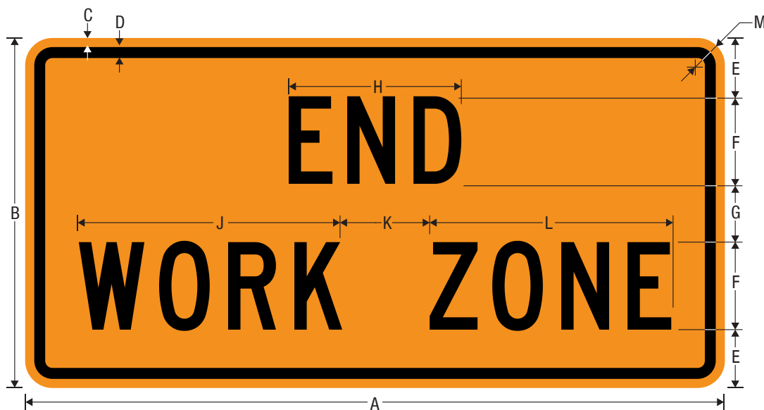
G20-2bT END WORK ZONE
