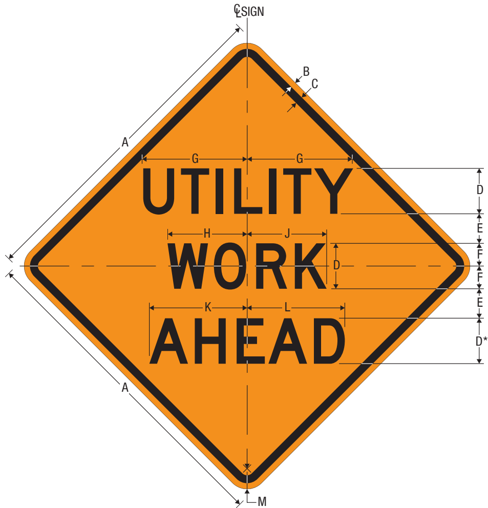
CW21-7[D] UTILITY WORK (with Distance)
