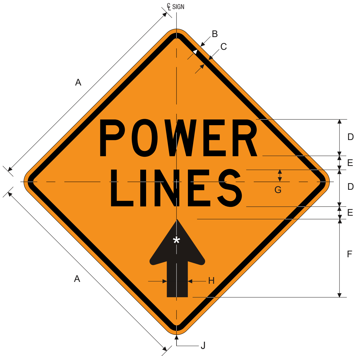
CW28-1T POWER LINES (with Arrow)
