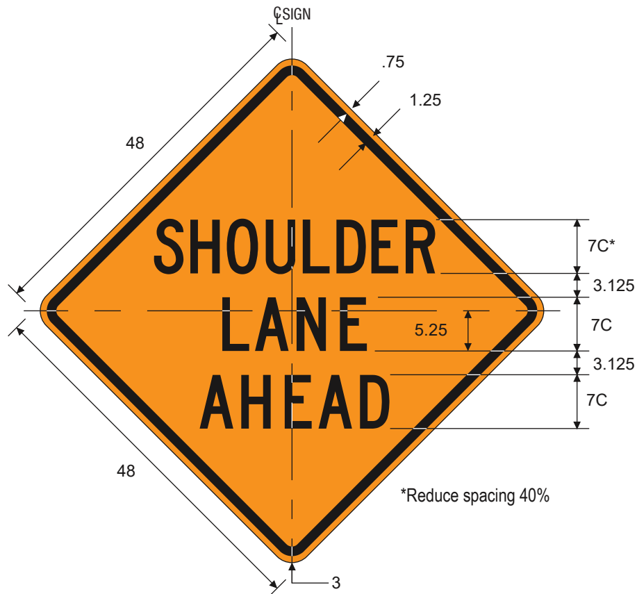
CW23-1T SHOULDER LANE AHEAD
