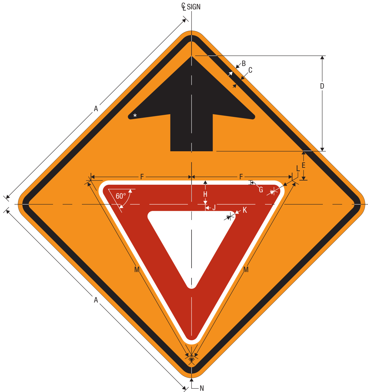
CW3-2 Yield Ahead
