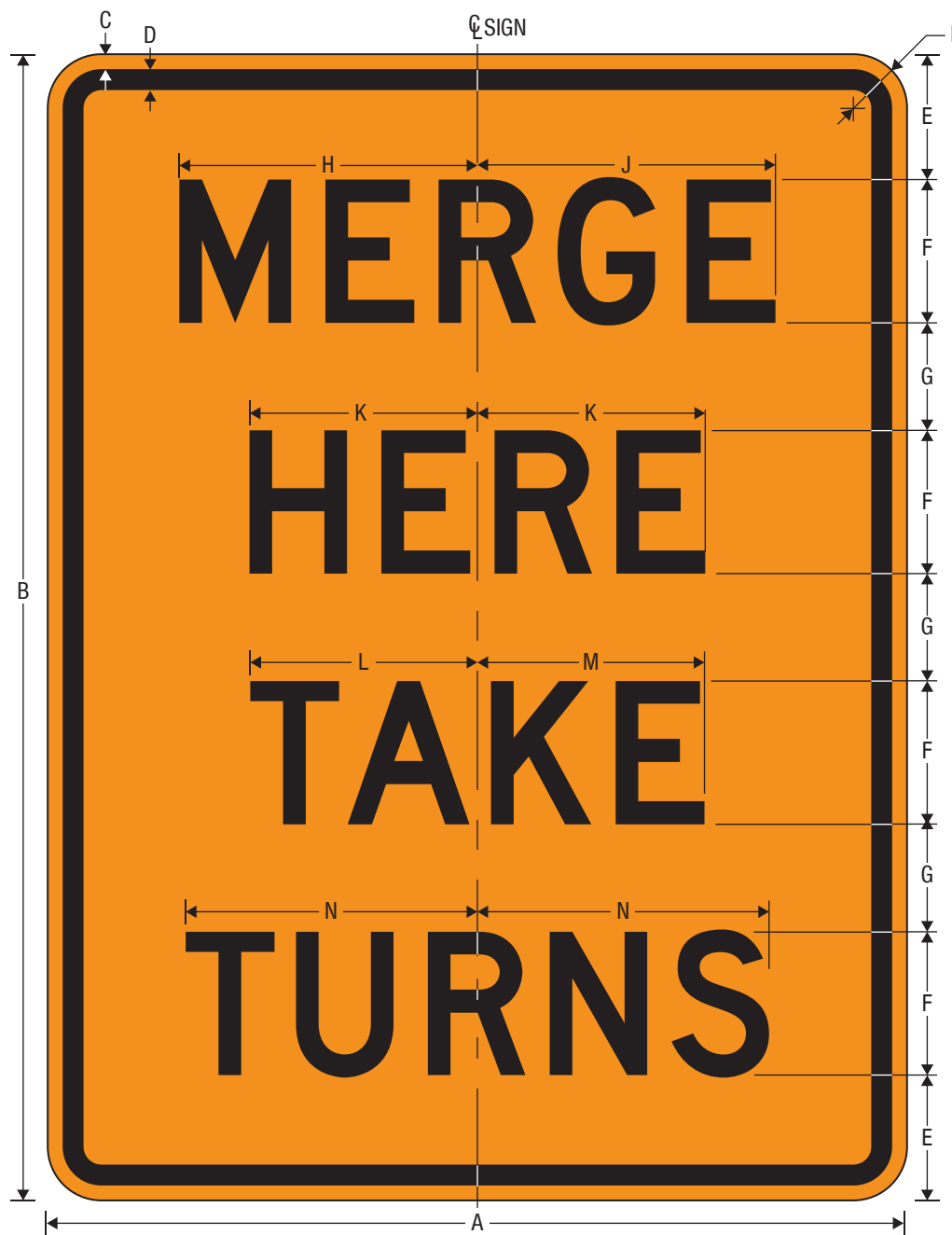
CW9-2a MERGE HERE TAKE TURNS
