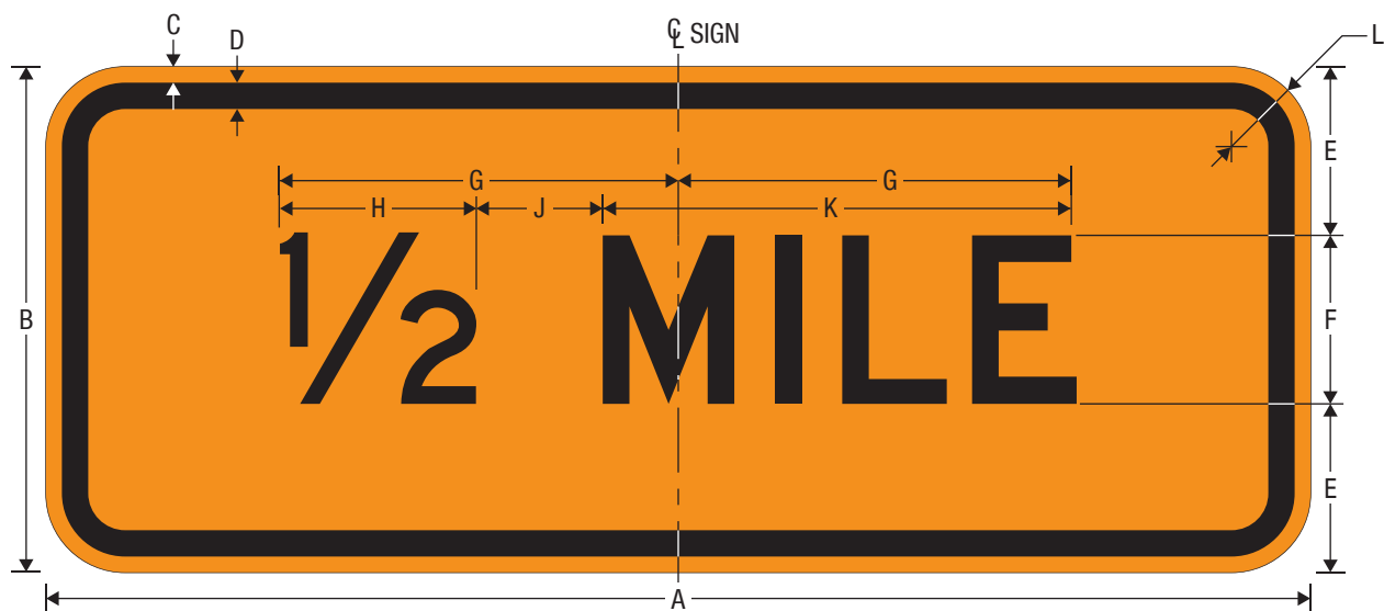
CW16-3aP [1]
