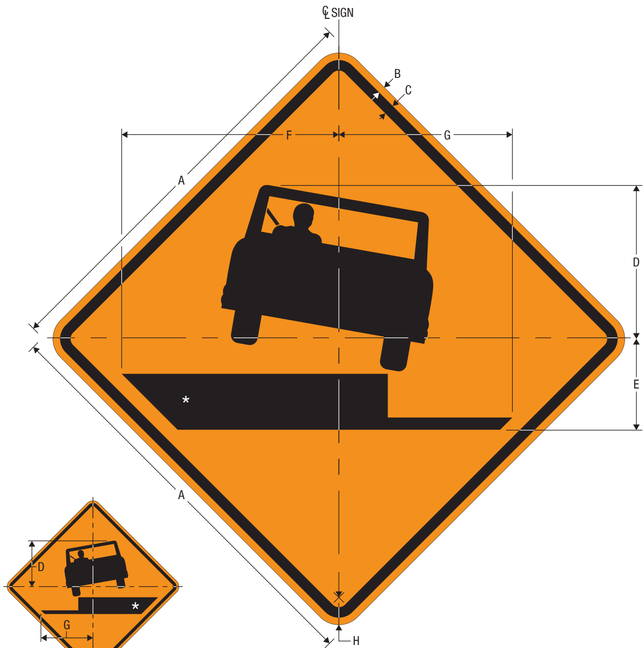
CW8-17R Shoulder Drop Off
