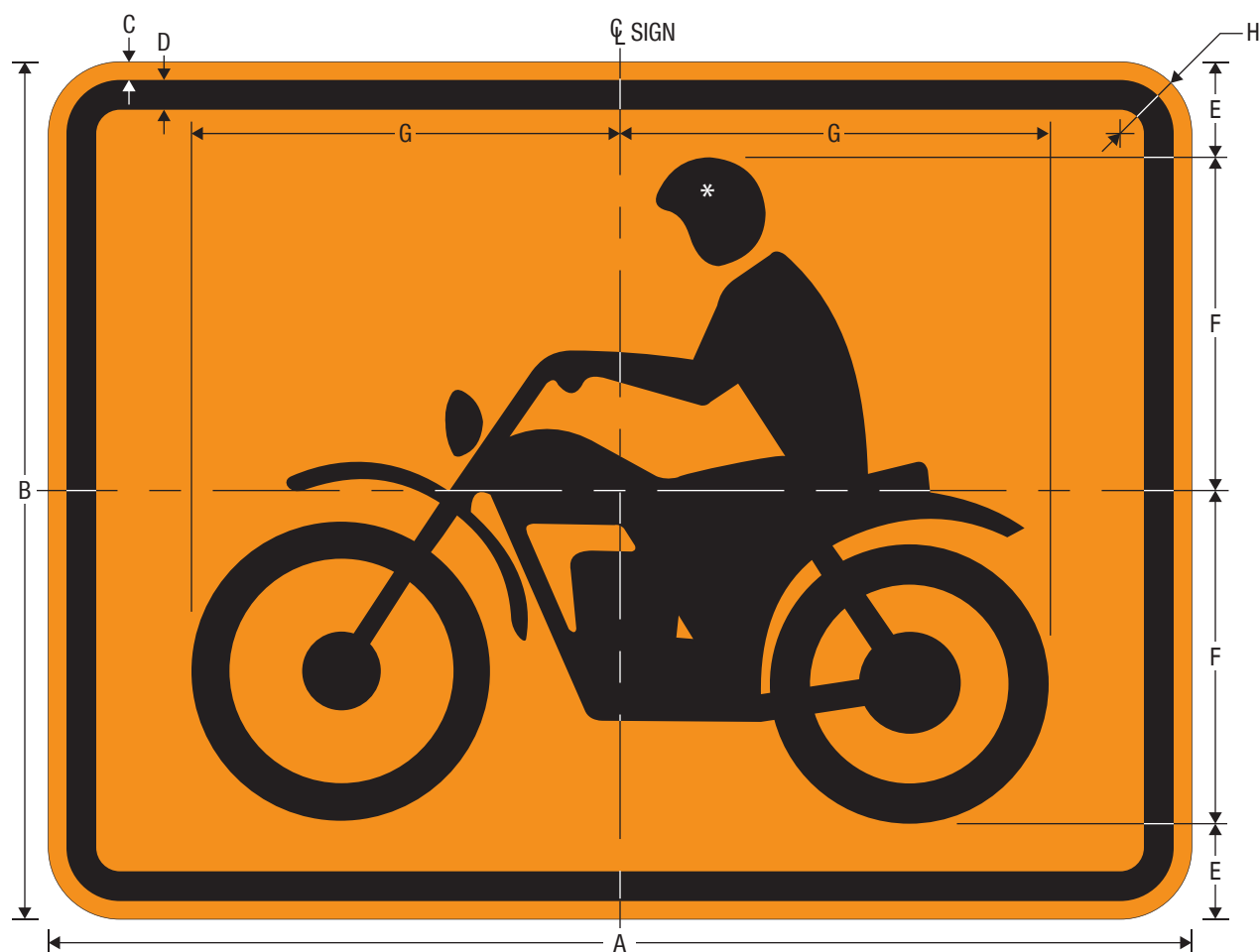
CW8-15aP Motorcycle (Plaque)
