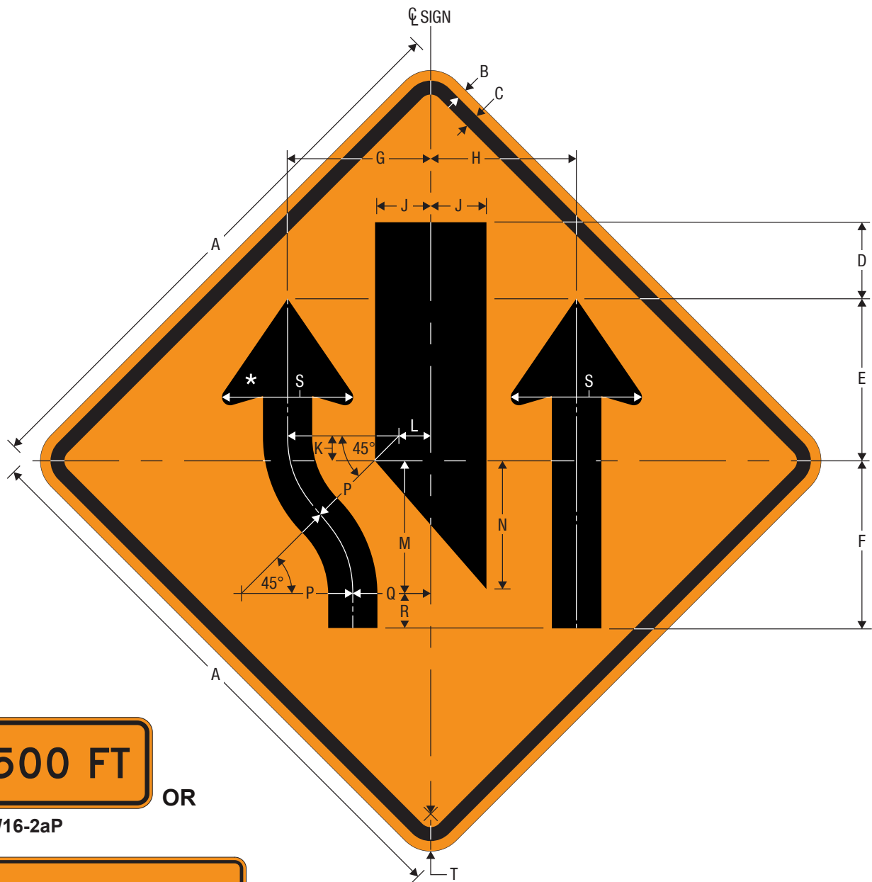
CW9-3 Interior Lane Shift Ahead
