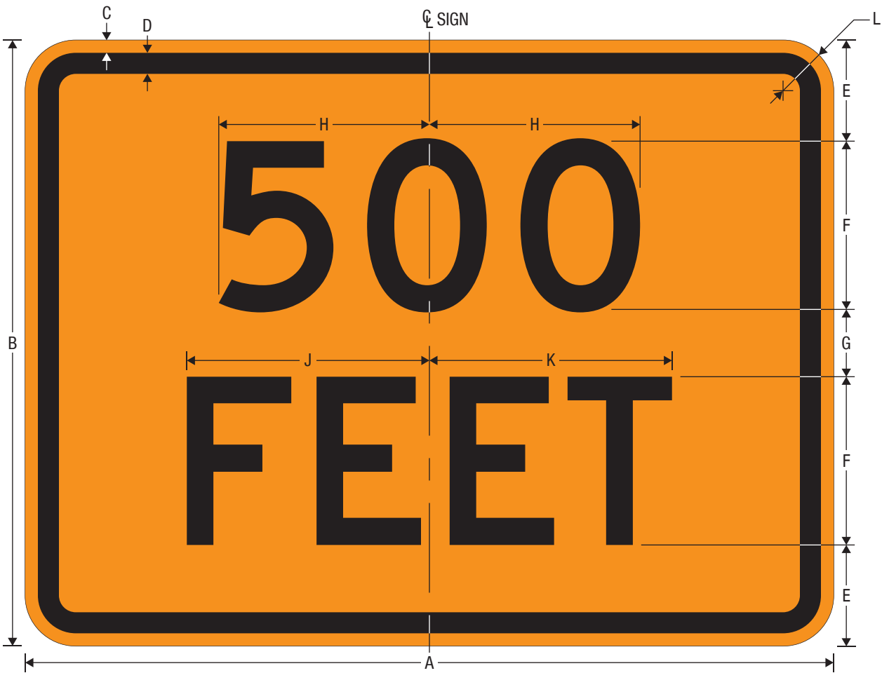
CW16-2P
