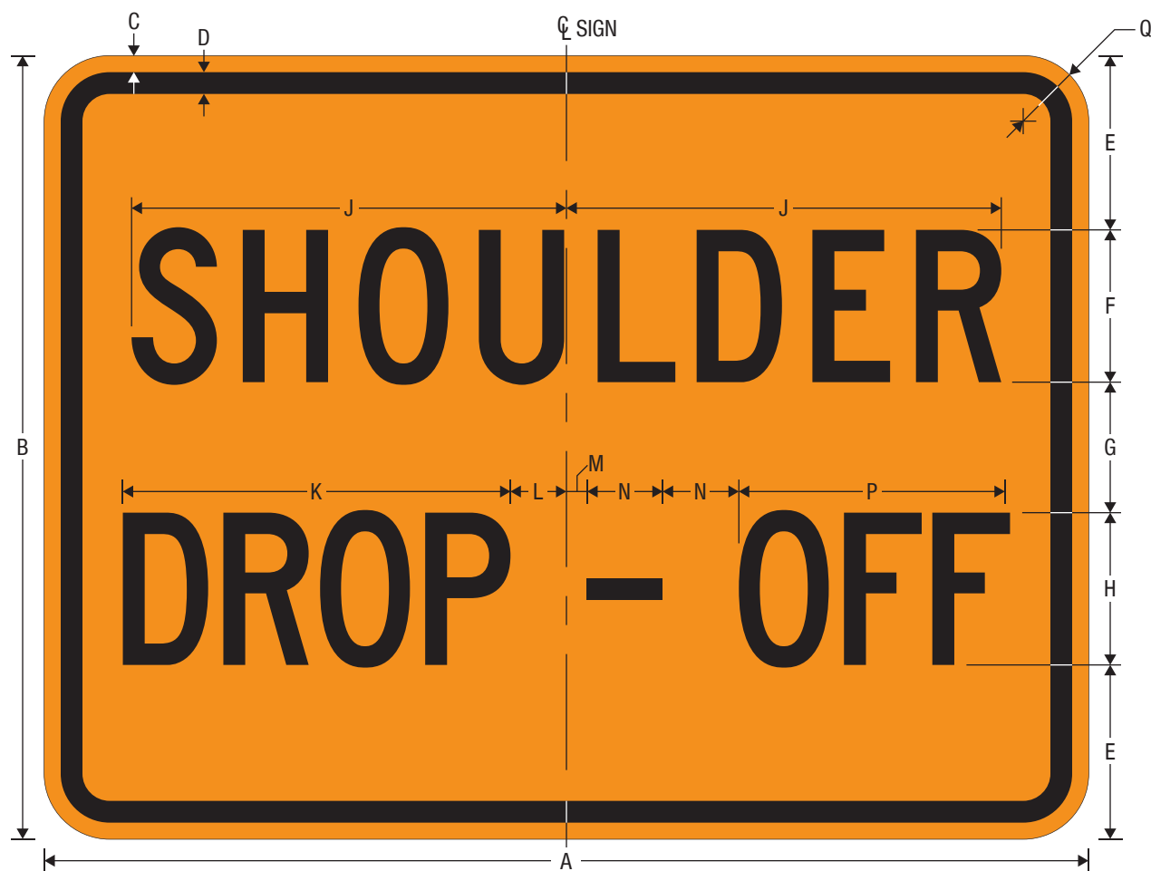
CW8-17P SHOULDER DROP-OFF (Plaque)
