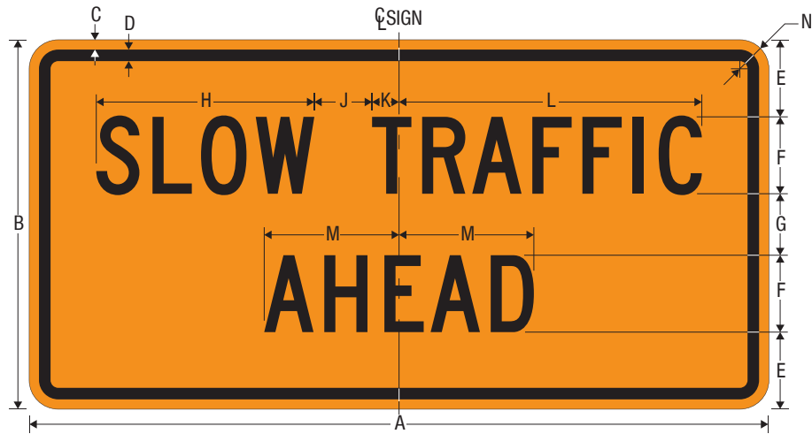
CW23-1 SLOW TRAFFIC AHEAD
