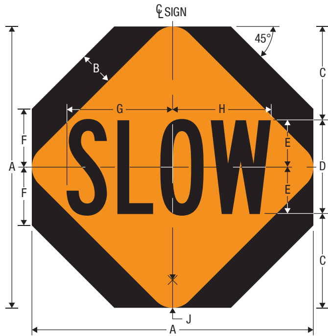
CW20-8 SLOW (On Stop/Slow Paddle)
