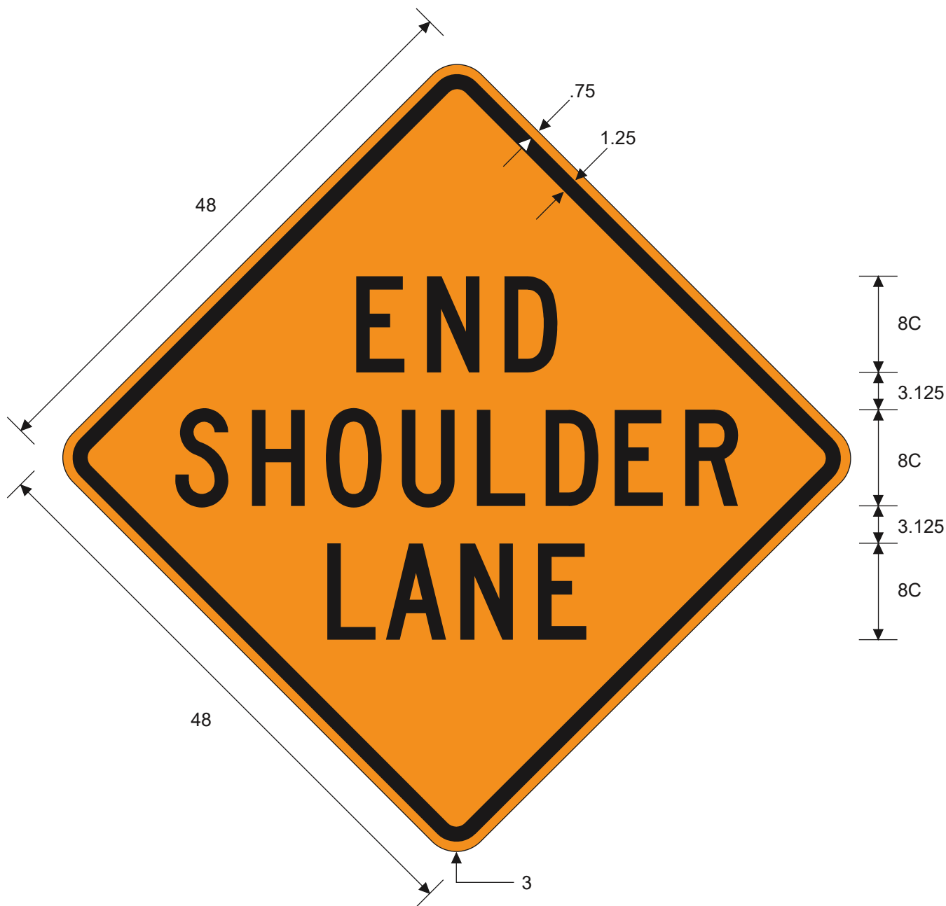
CW23-3T END SHOULDER LANE
