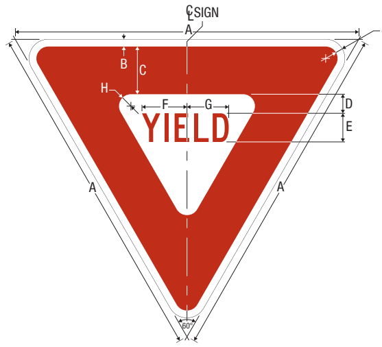
R1-2 YIELD
