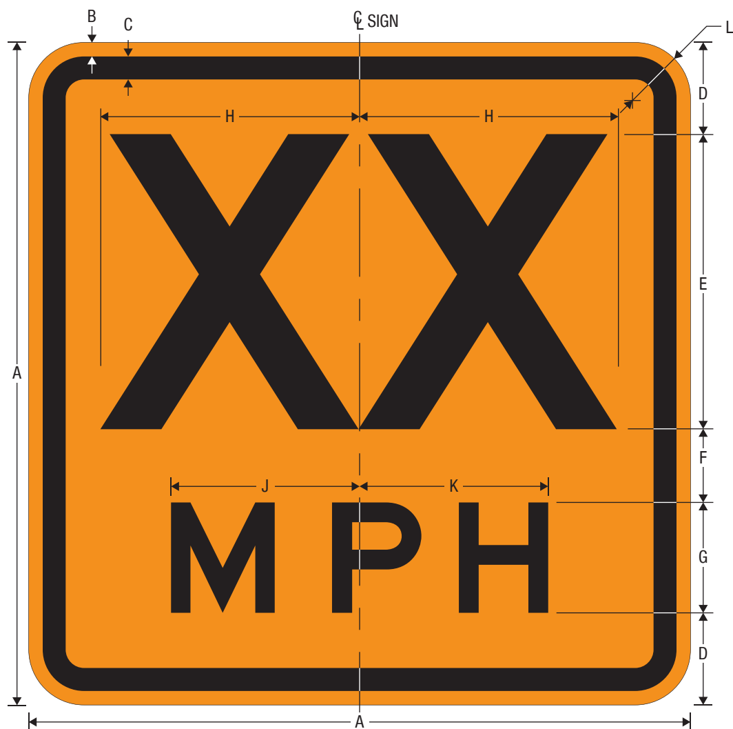
CW13-1P Advisory Speed (Plaque)
