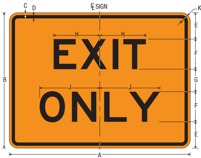
E5-3 EXIT ONLY
