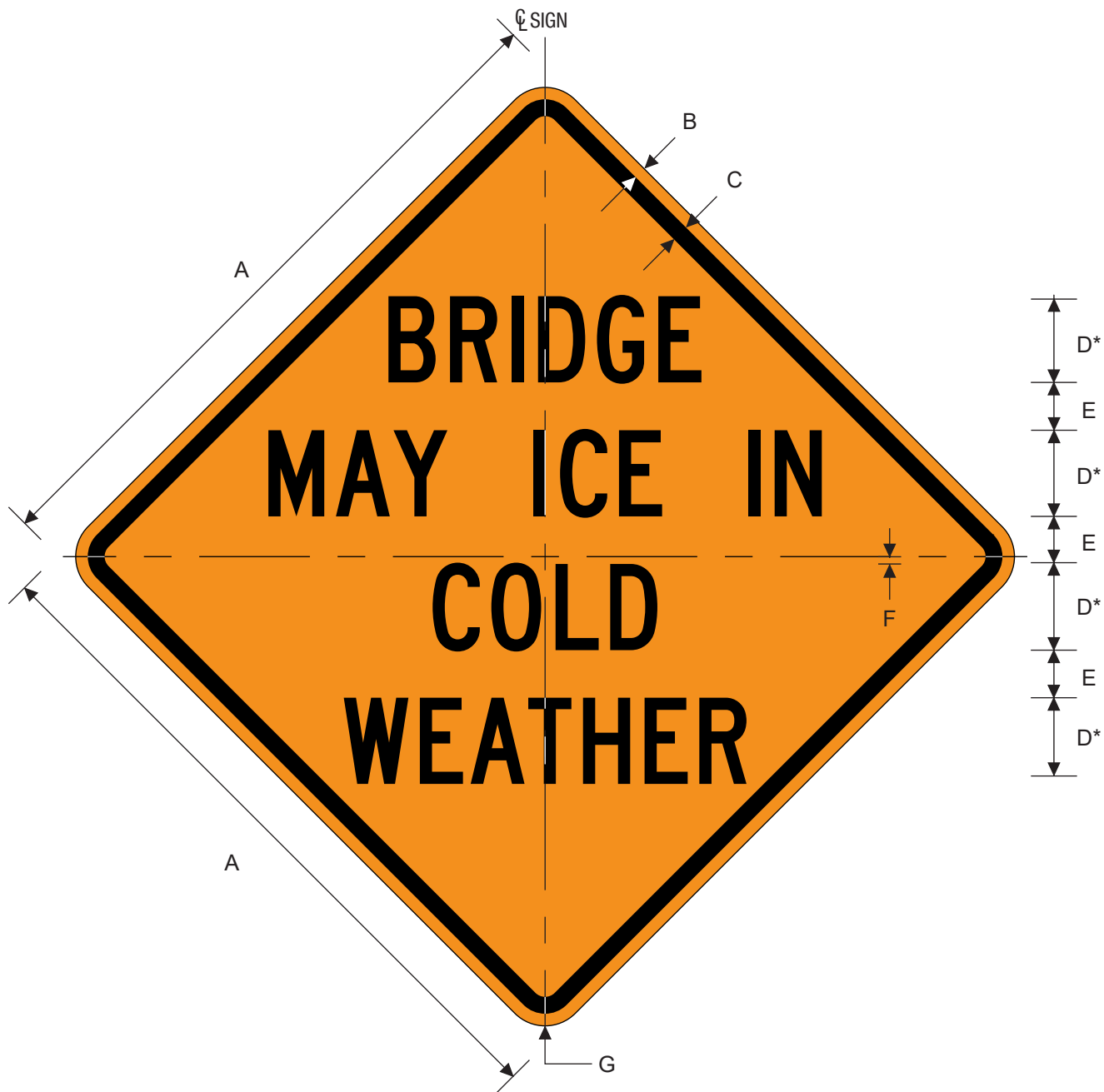
CW8-13aT BRIDGE MAY ICE IN COLD WEATHER
