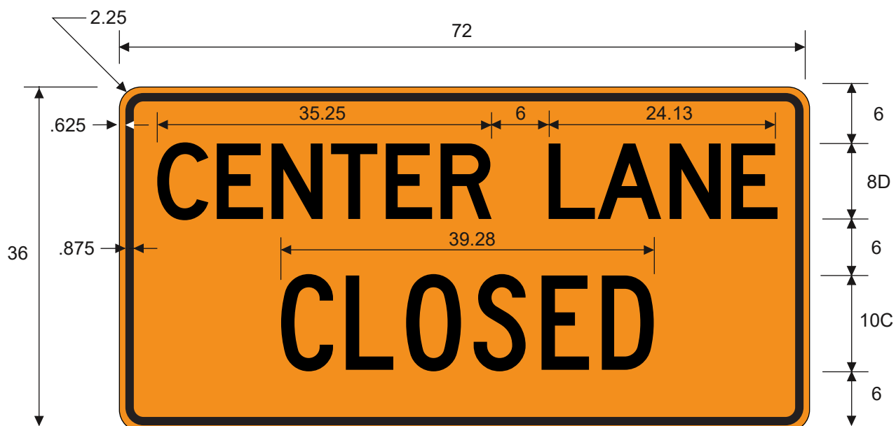
CW20-5dT CENTER LANE CLOSED
