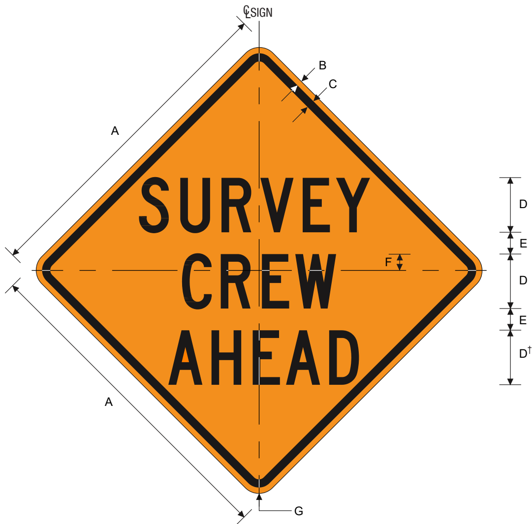
CW21-6T[D] SURVEY CREW (with Distance)
