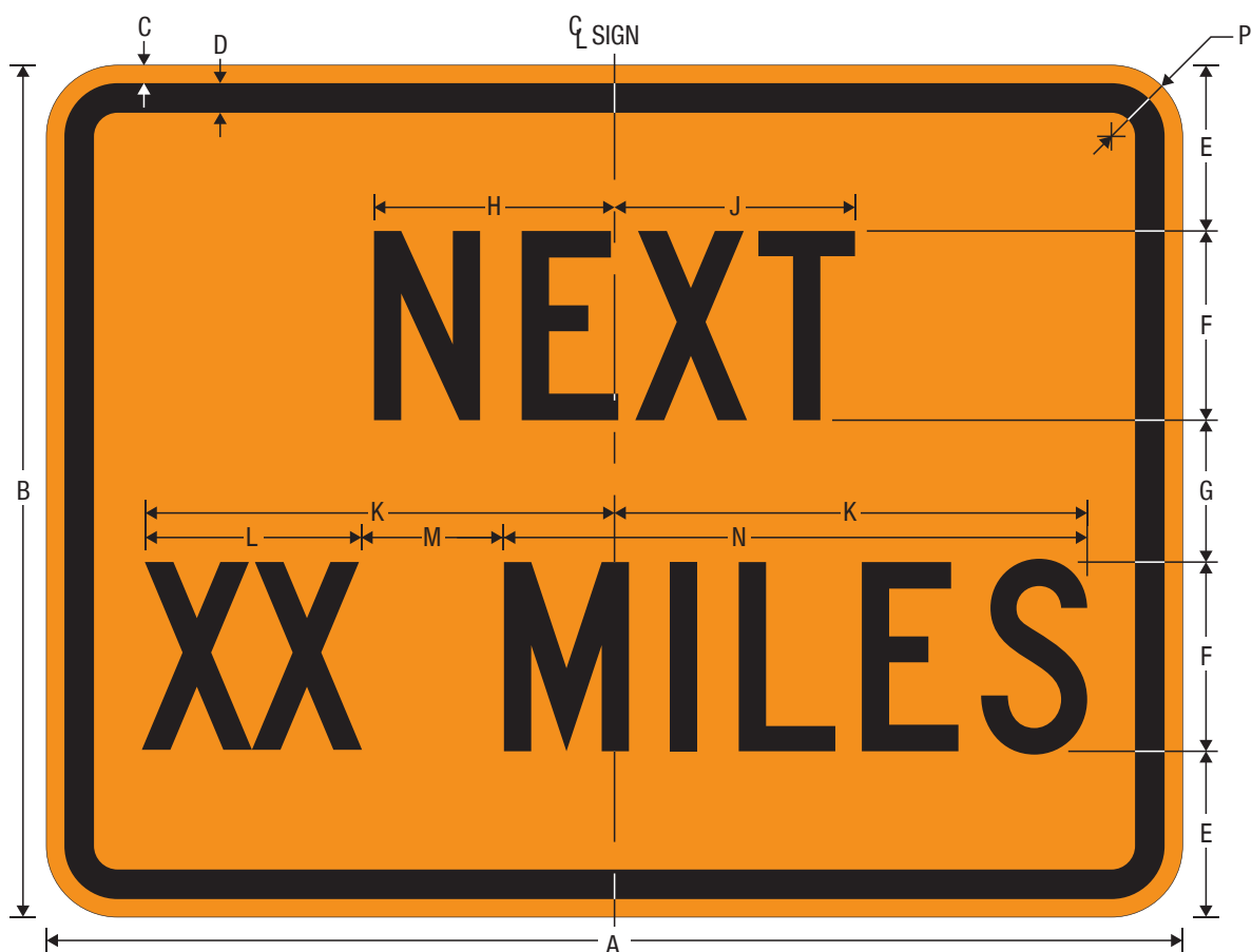
CW7-3aP NEXT XX MILES (Plaque)
