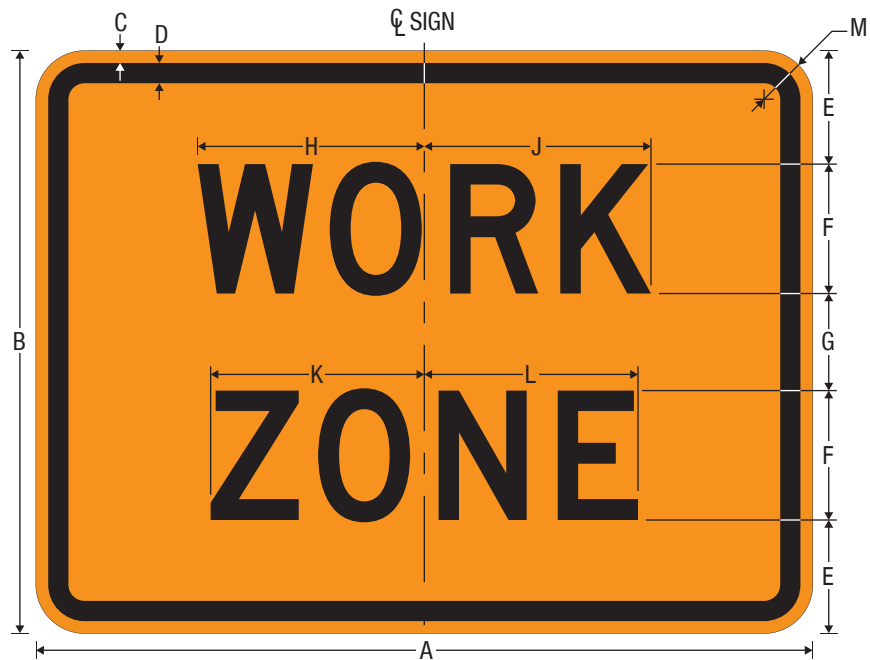
G20-5aP WORK ZONE (Plaque)
