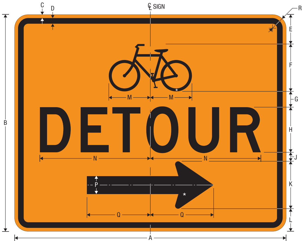
M4-9cR Bicyclist DETOUR (with Arrow)
