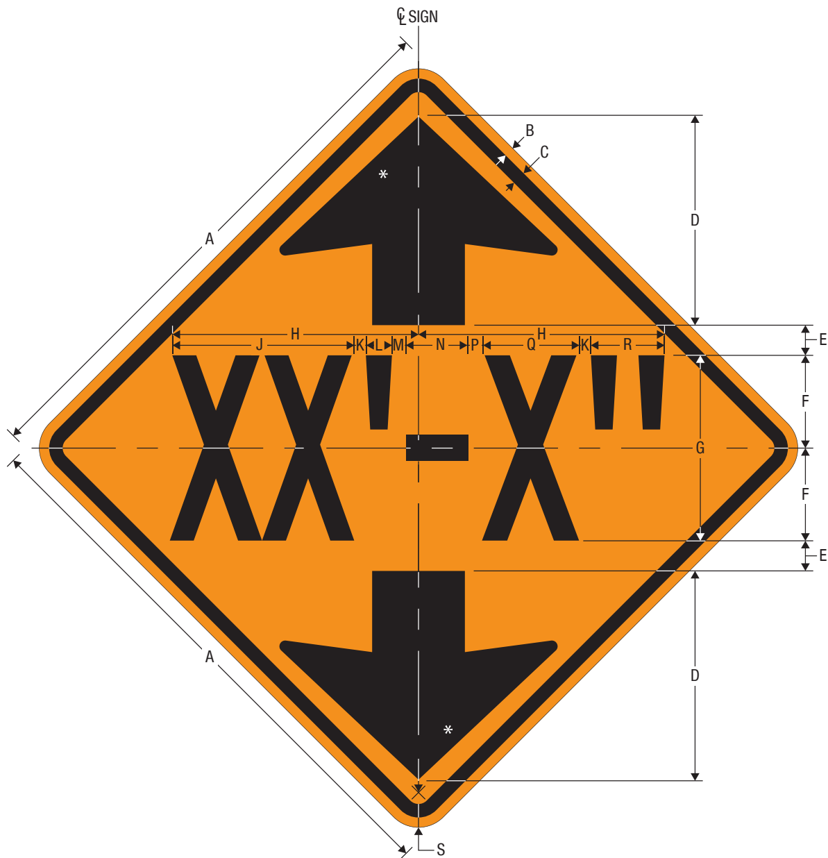
CW12-2 Clearance Advance
