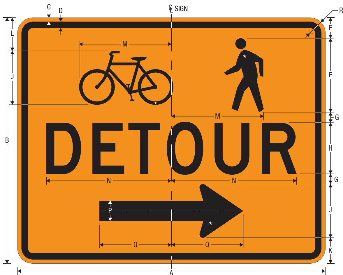
M4-9aR Bicyclist/Pedestrian DETOUR
