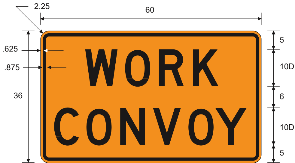
CW21-10aT WORK CONVOY
