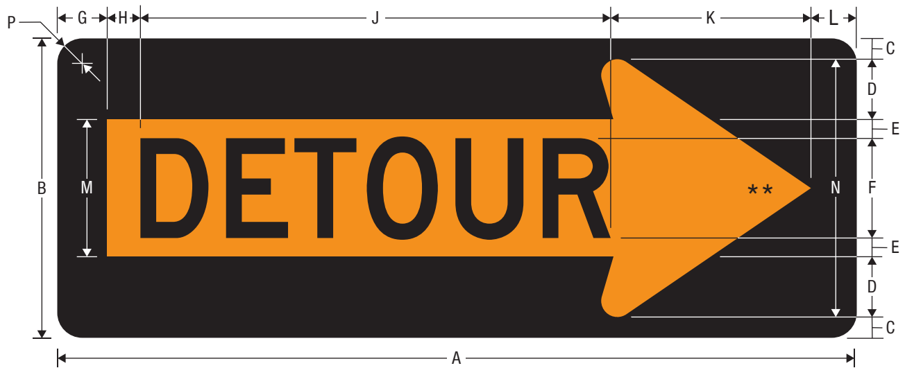
M4-10R DETOUR (Arrow)
