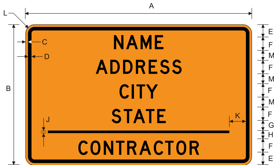
G20-6T CONTRACTOR
