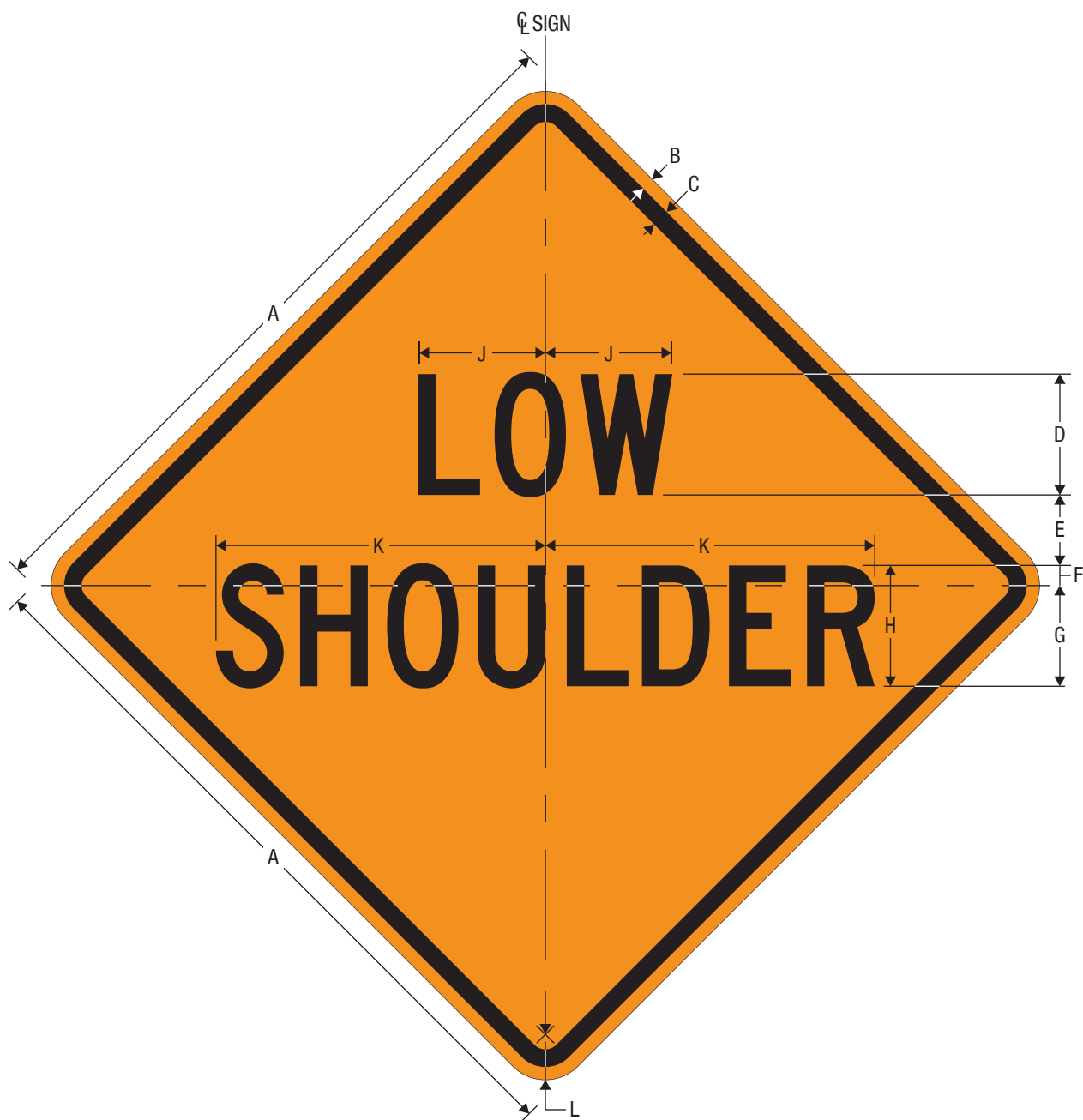
CW8-9 LOW SHOULDER
