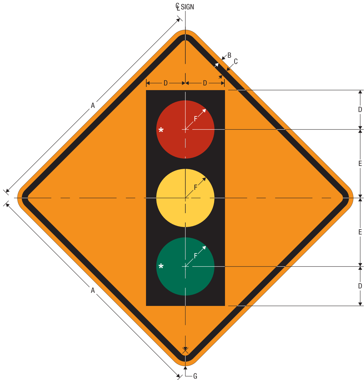
CW3-3 Signal Ahead
