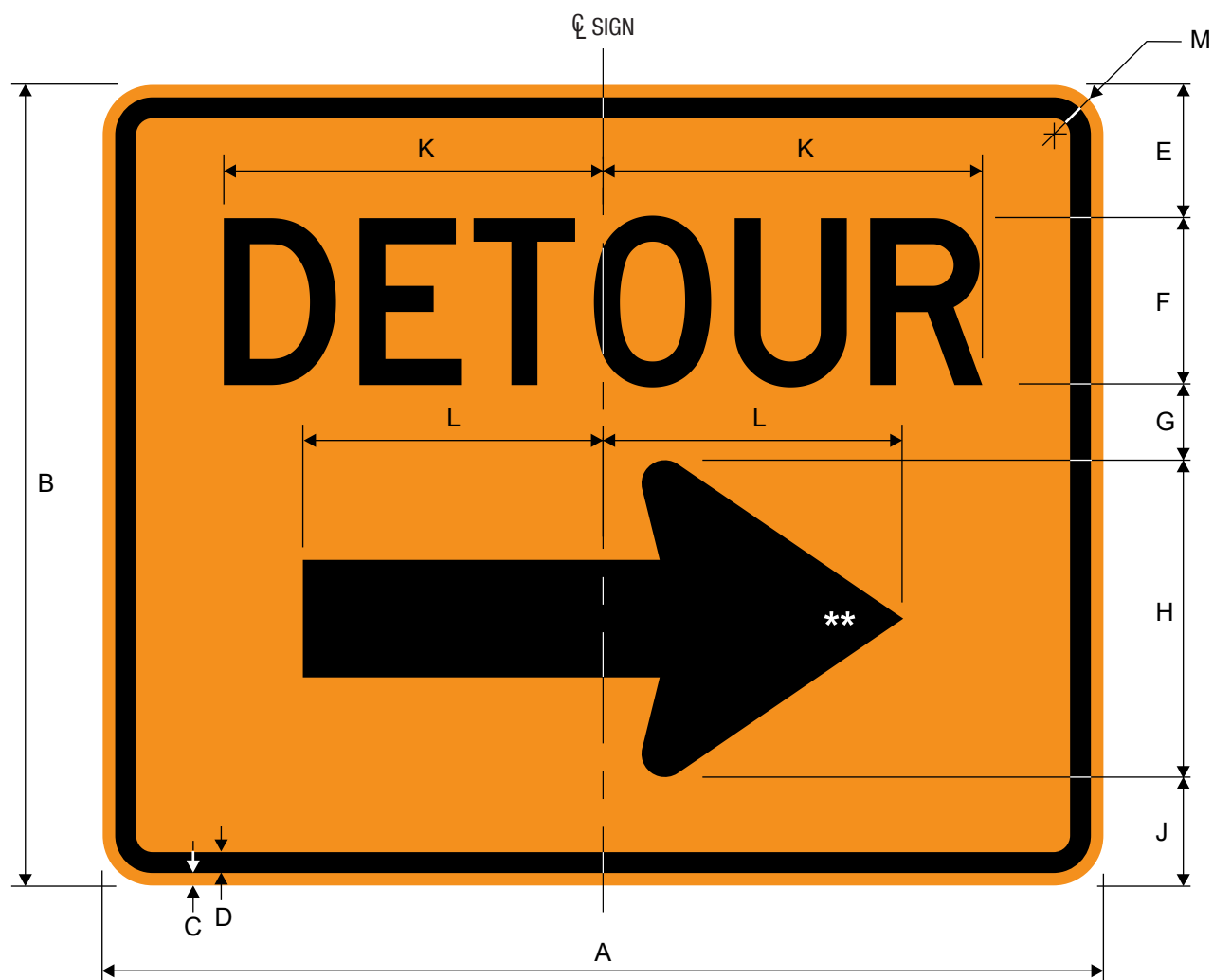
M4-9R DETOUR (Right-Arrow)
