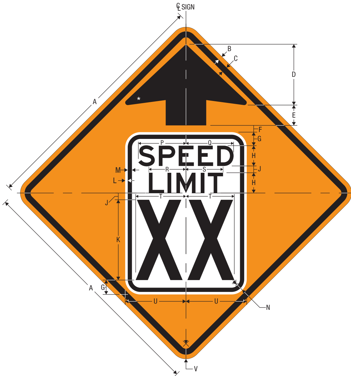
CW3-5 Reduced Speed Limit Ahead
