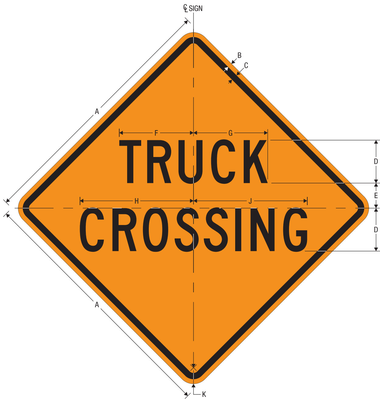
CW8-6 TRUCK CROSSING
