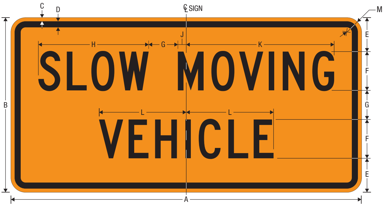
CW21-4 SLOW MOVING VEHICLE
