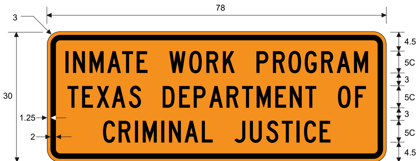
CW29-2T
