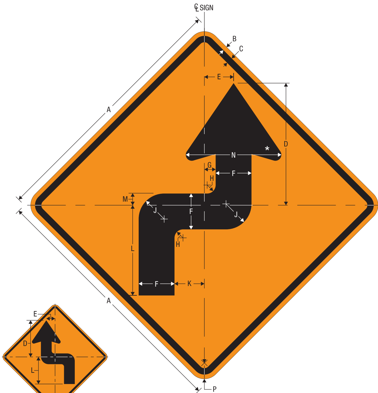
CW1-3R Horizontal Alignment - Reverse Turn
