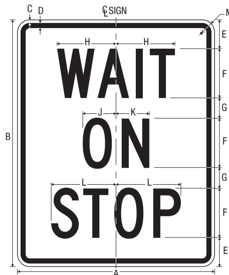
R1-7 WAIT ON STOP
