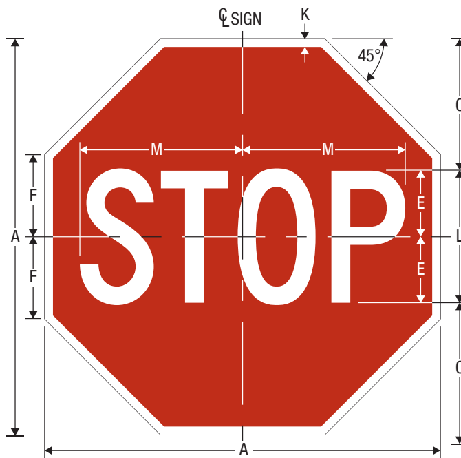
[R1-1] STOP (On Stop/Slow Paddle)
