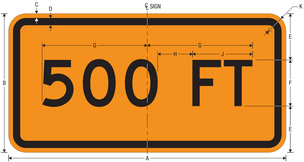
CW16-2aP [Distance Plaque] XX FT (1-Line Plaque)
