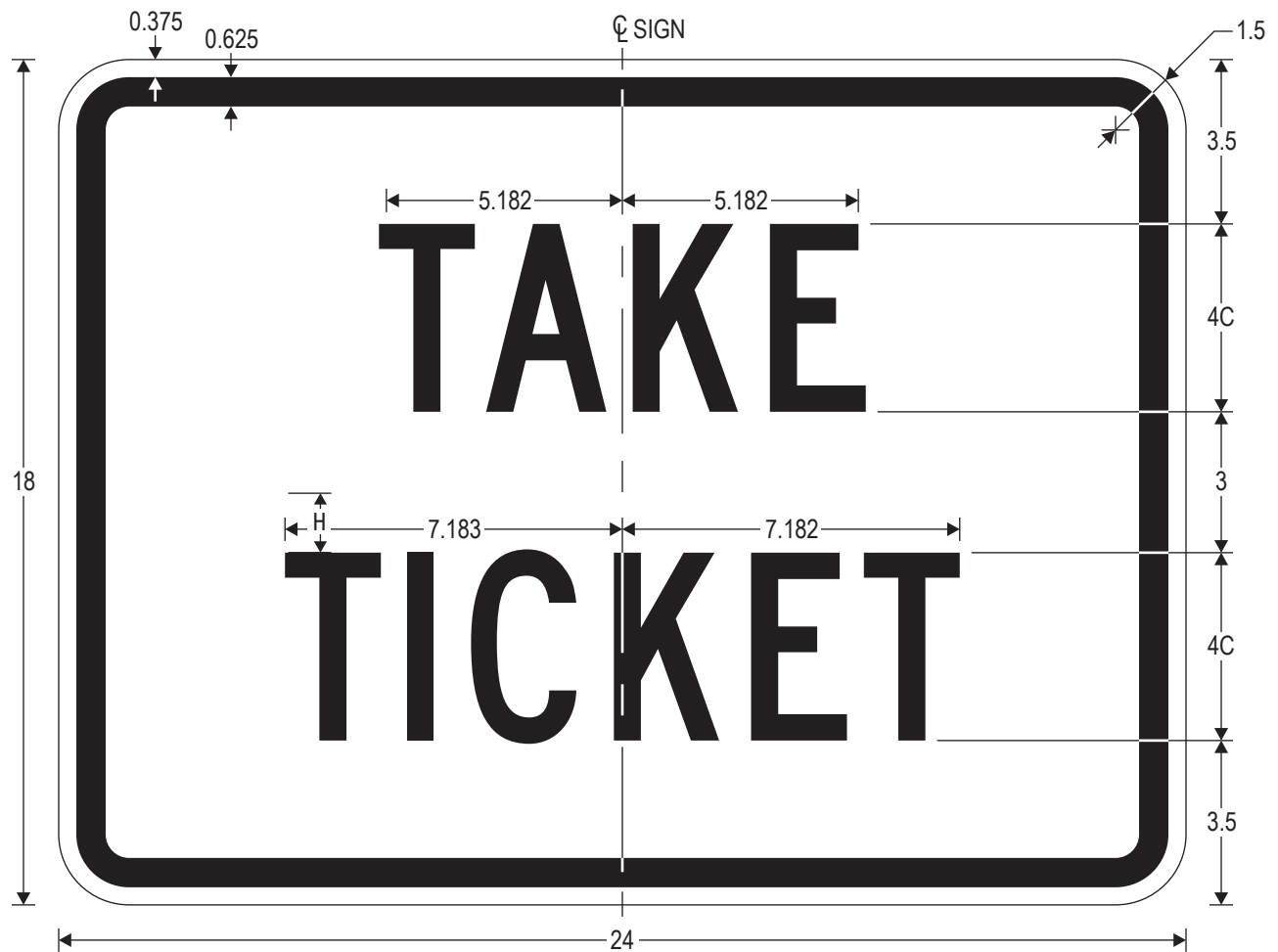
R3-30P TAKE TICKET (Plaque)
