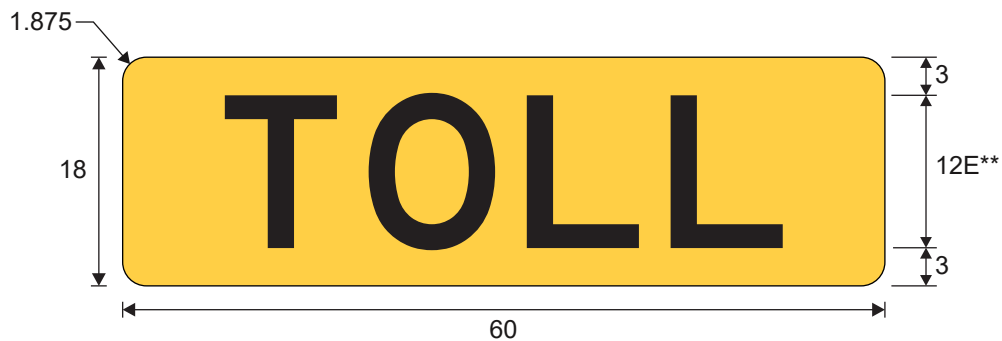
W90-12T TOLL Panel Inset
