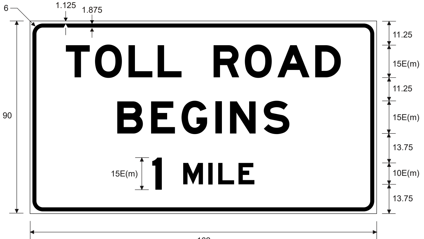
R90-1T TOLL ROAD BEGINS X MILE
