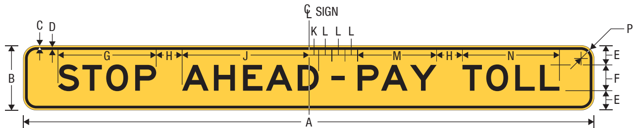
W9-6cP STOP AHEAD - PAY TOLL (Plaque)
