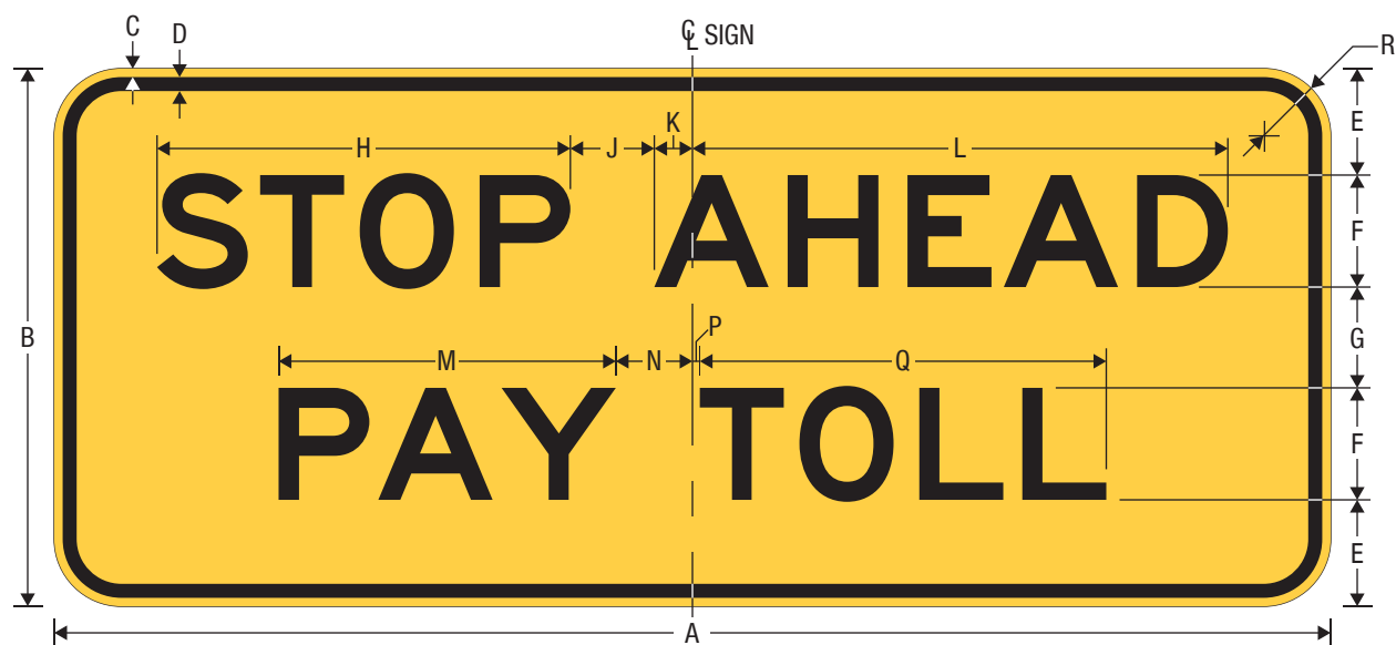
W9-6dP [STOP AHEAD] PAY TOLL (Plaque)
