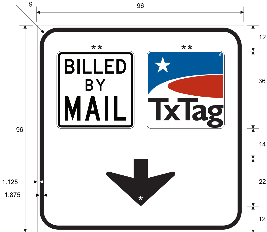
E90-6aT BILLED BY MAIL/TxTAG (Down Arrow)
