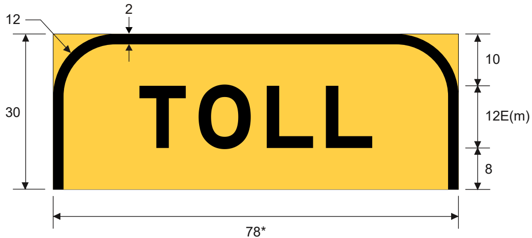
W90-11T TOLL Panel
