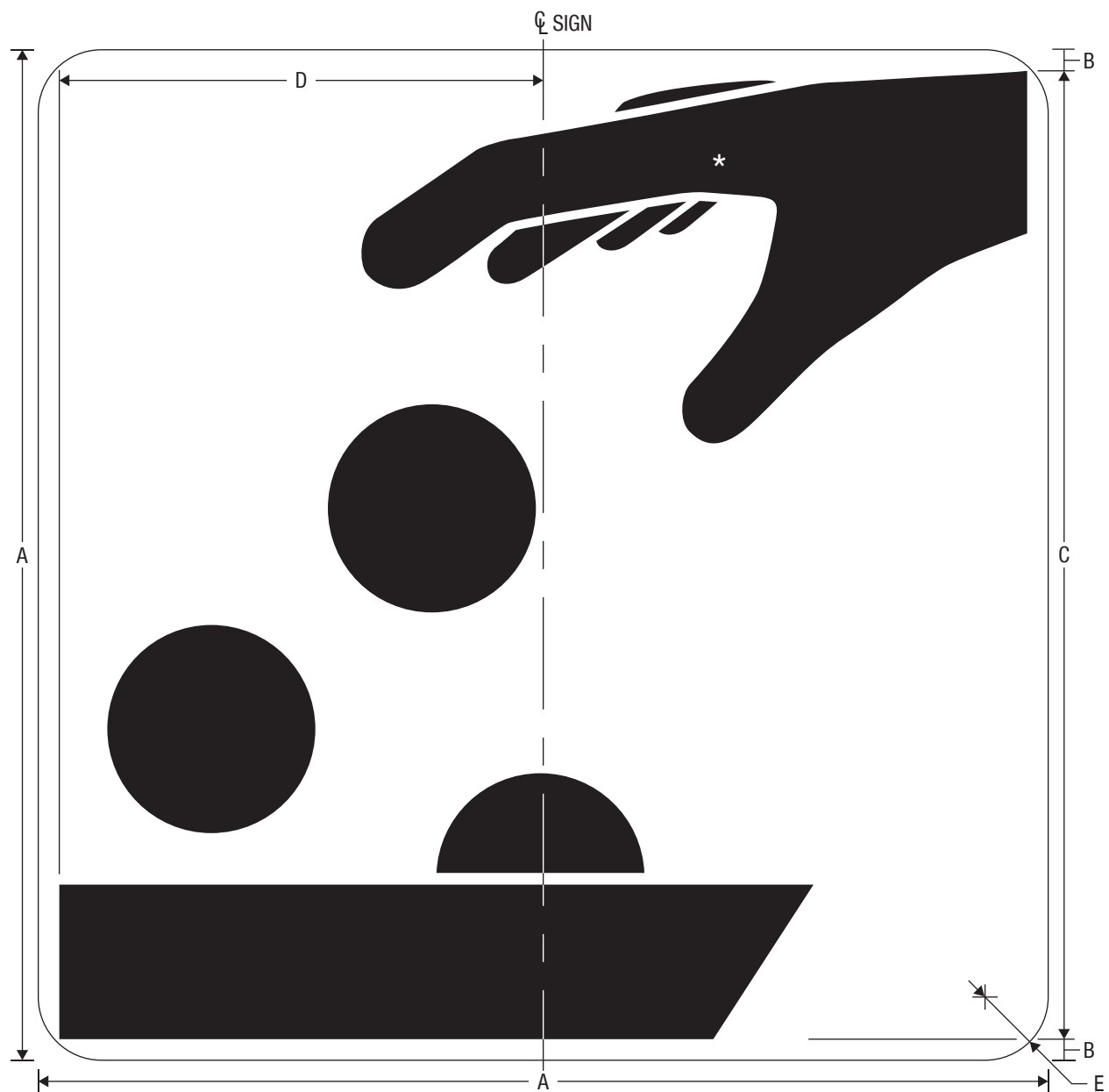
M4-18 Exact Change Symbol Panel
