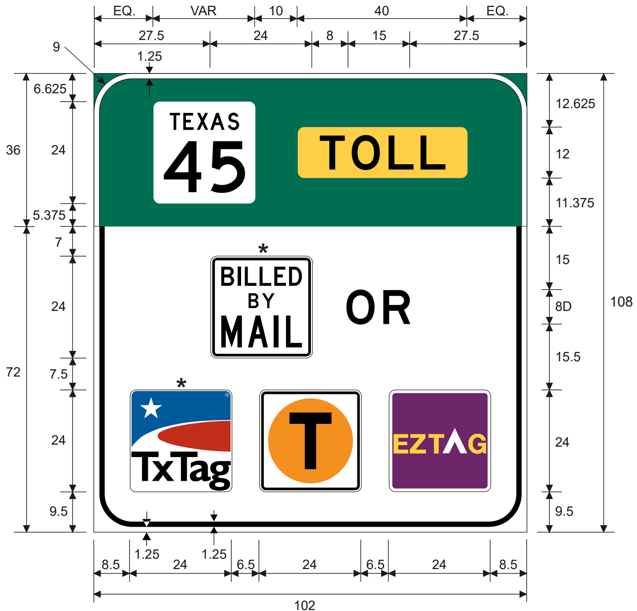
E90-13T TOLL - BILLED BY MAIL OR ETC Account Pictograph(s)
