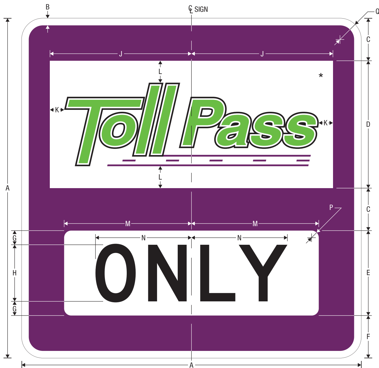
R3-31 ETC Account - ONLY
