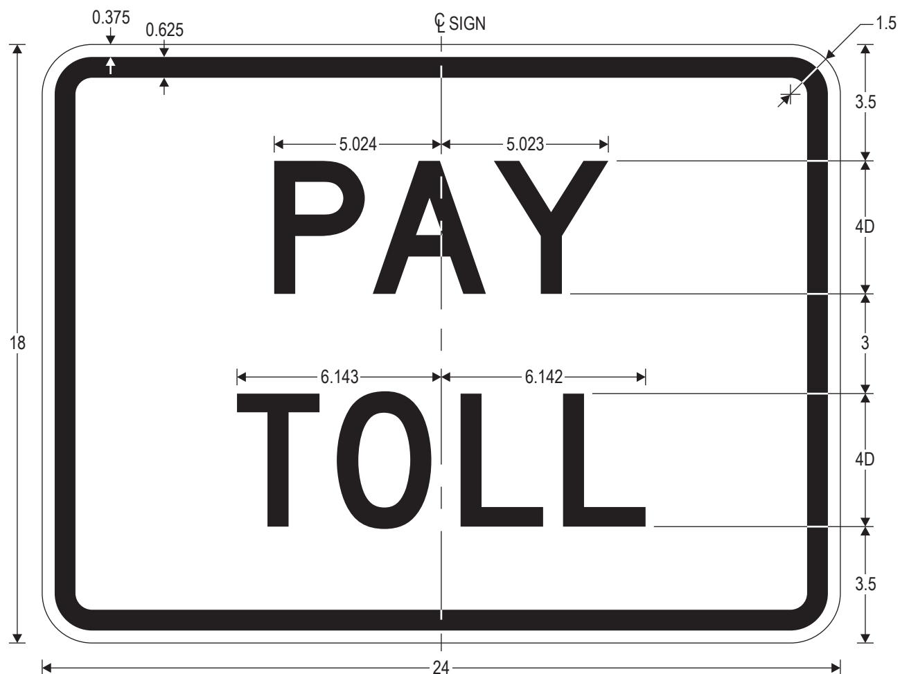
R3-29P PAY TOLL (Plaque)
