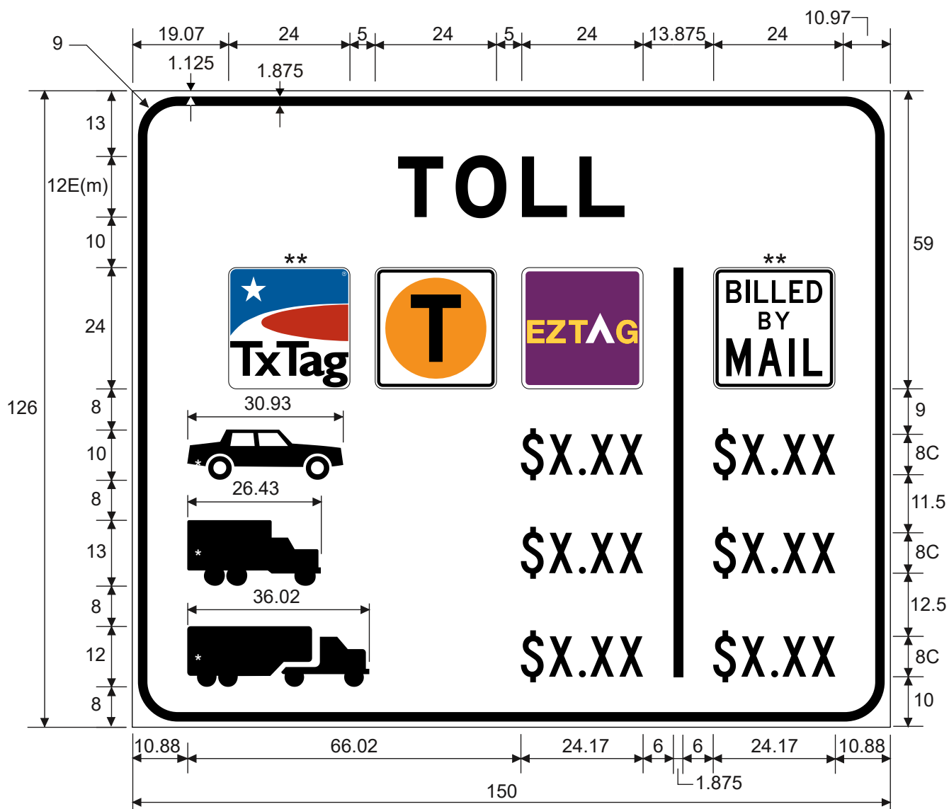
R90-2aT [ETC | BILLED BY MAIL] Toll Rate (Symbols)
