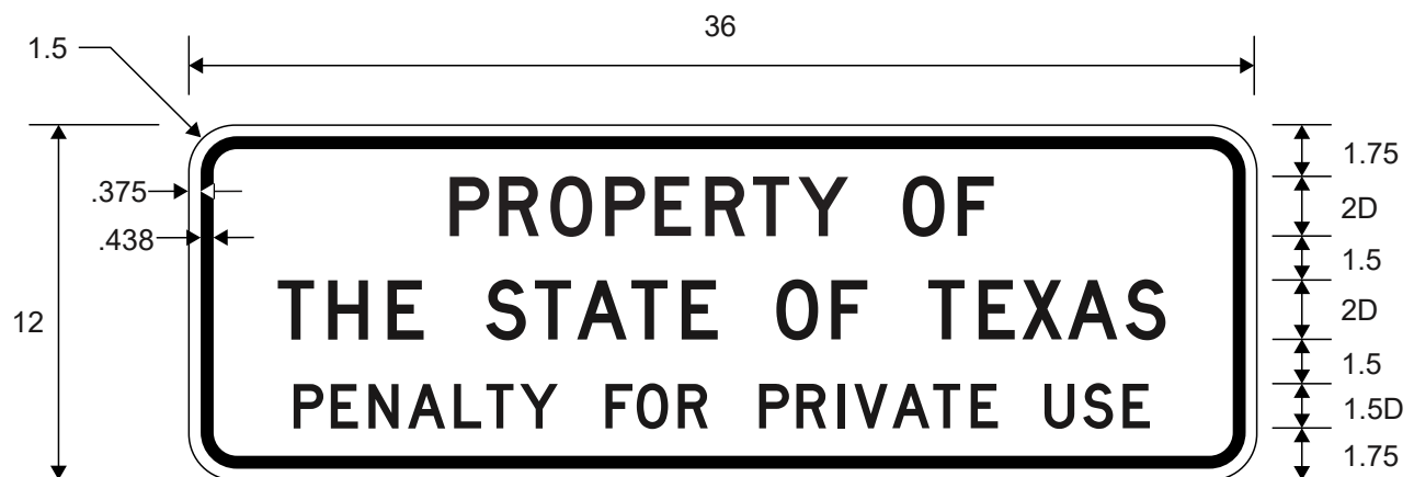
TX3-1T PROPERTY OF THE STATE OF TEXAS PENALTY FOR PRIVATE USE
