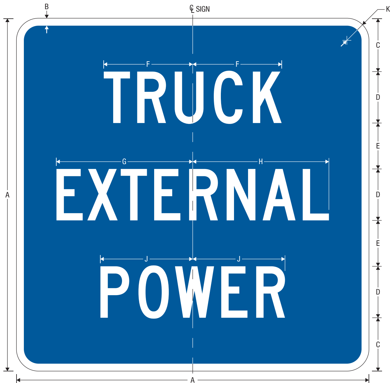
D9-16aP TRUCK EXTERNAL POWER (Plaque)
