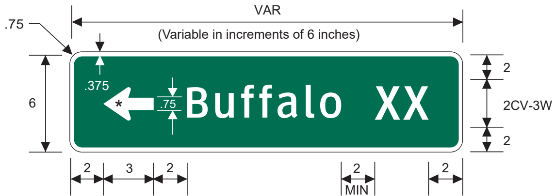
D1-1aL Destination and Distance (1 Line) (Arrow)
