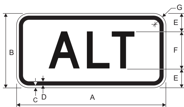
M4-1aP ALT (Plaque)
