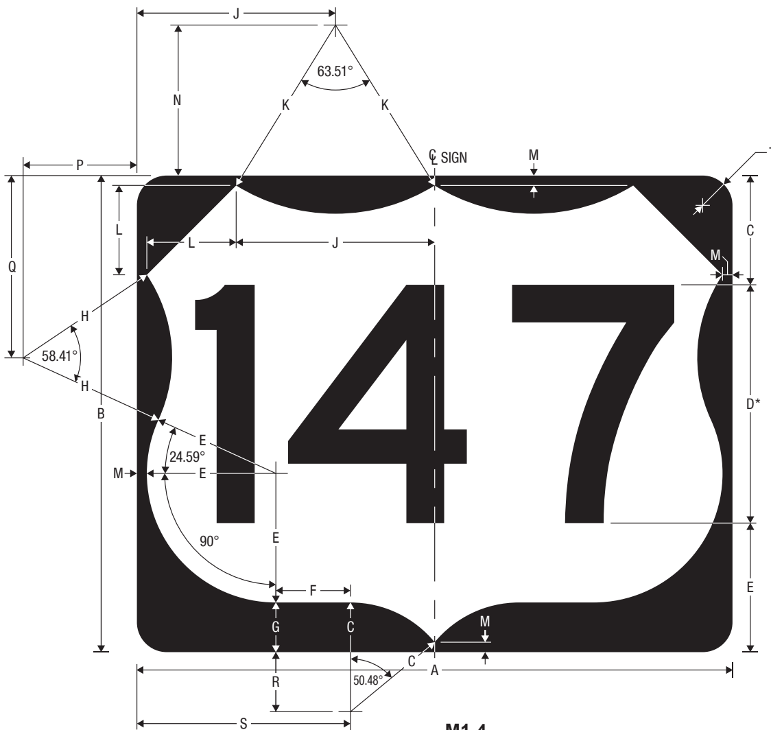
M1-4 U.S. Route - Independent Route Assembly Use (3 Digits)
