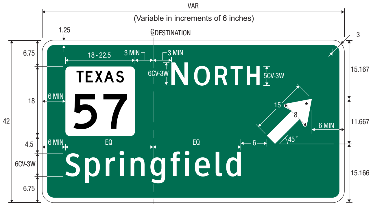
D1-1e Circular Intersection Departure Guide (Arrow)
