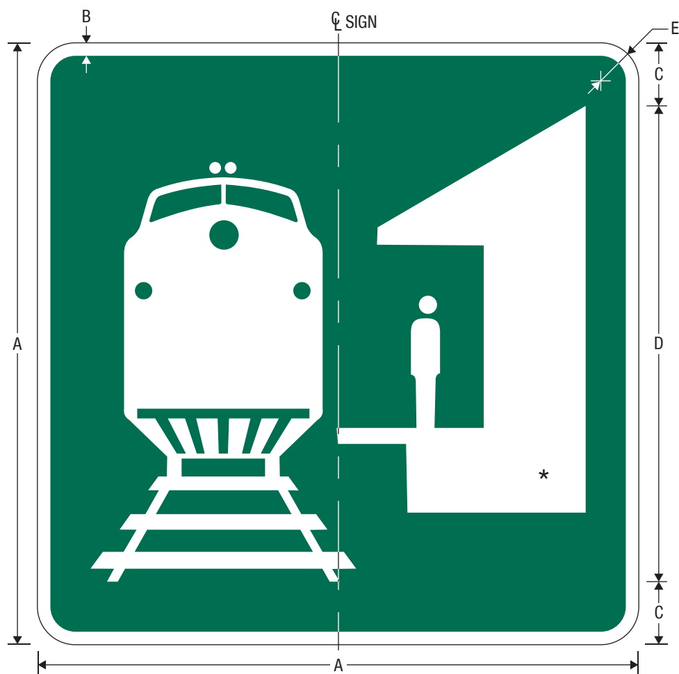
13-7 Train Station (Symbol)
