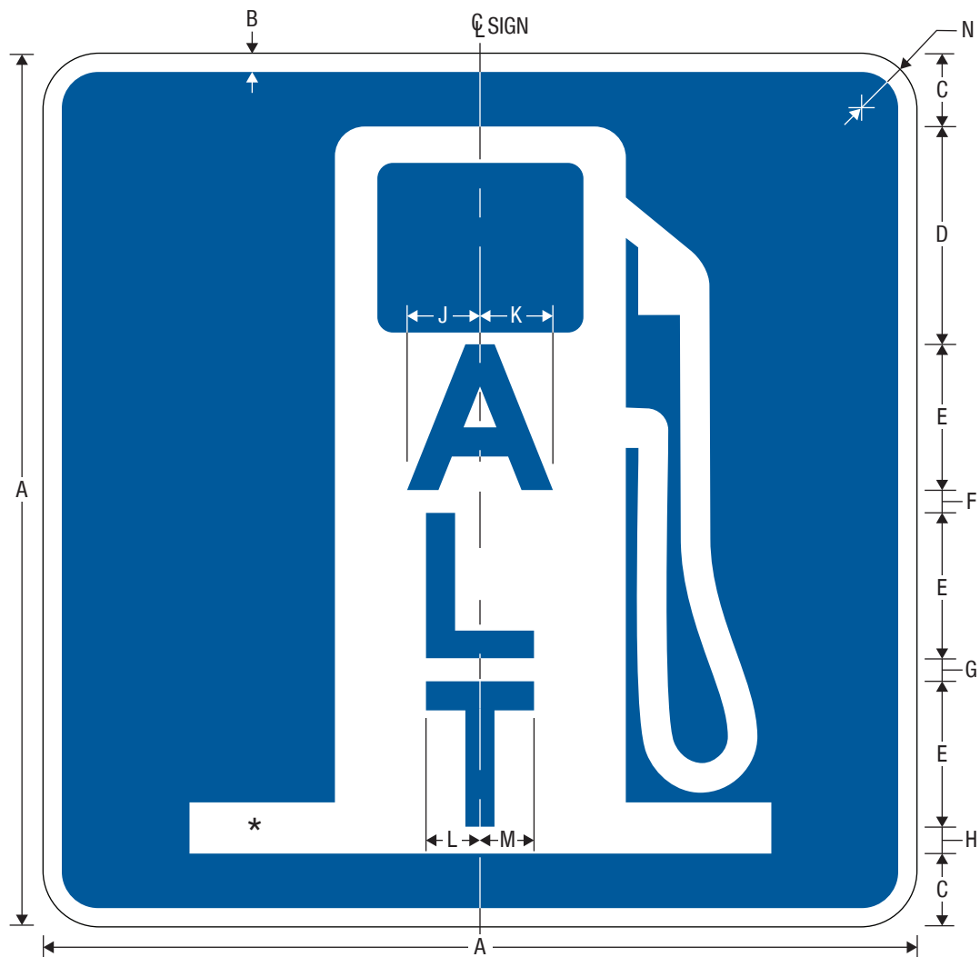
D9-11gT Alternative Fuel
