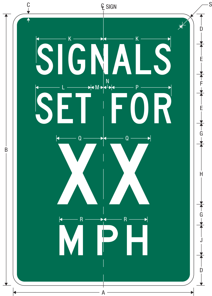
11-1 Traffic Signal Speed
