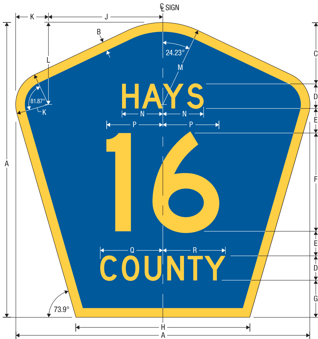
M1-6 County Route
