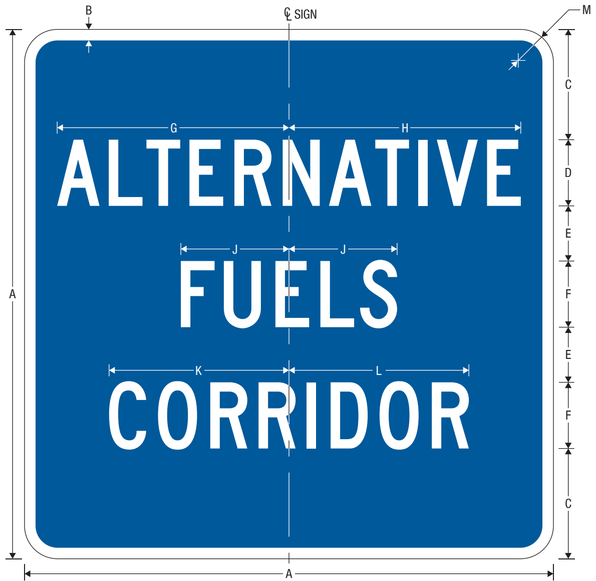
D9-19 ALTERNATIVE FUELS CORRIDOR
