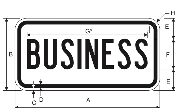
M4-3P BUSINESS (Plaque)
