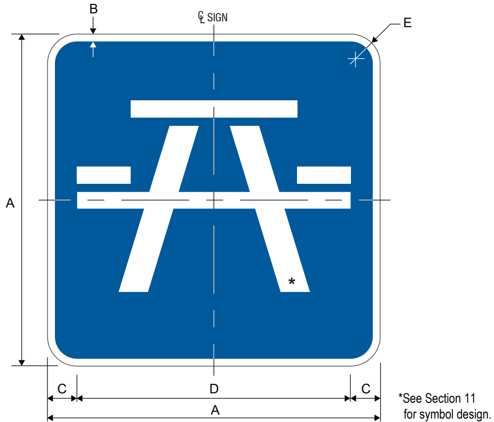
D5-5aT Picnic Table (Symbol)
