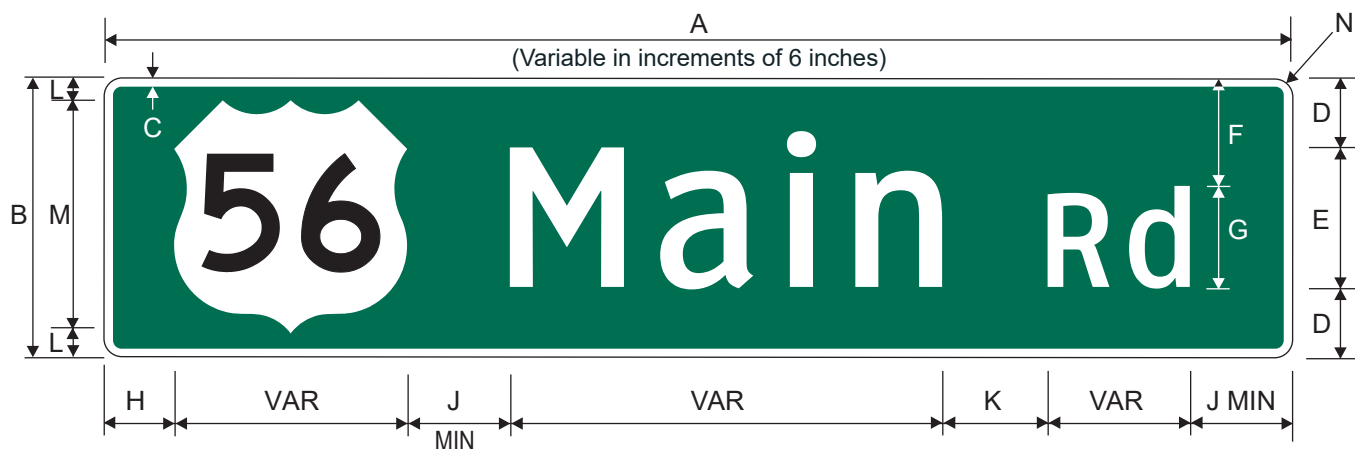
D3-1a Street Name
