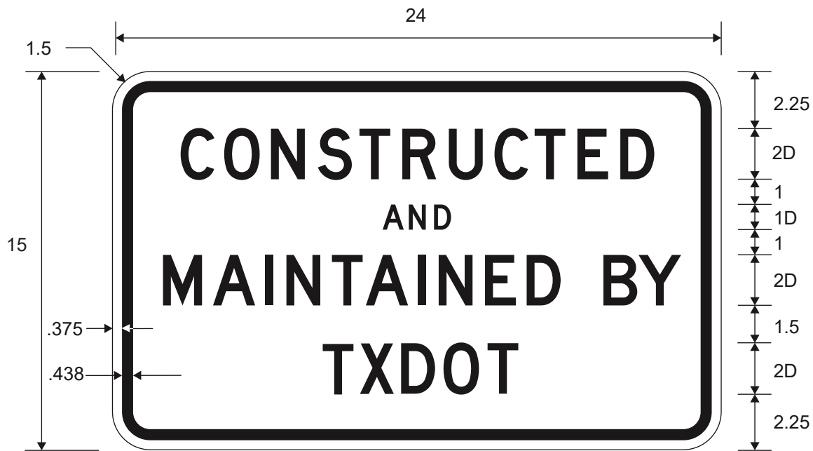
TX1-3T CONSTRUCTED AND MAINTAINED BY TXDOT
