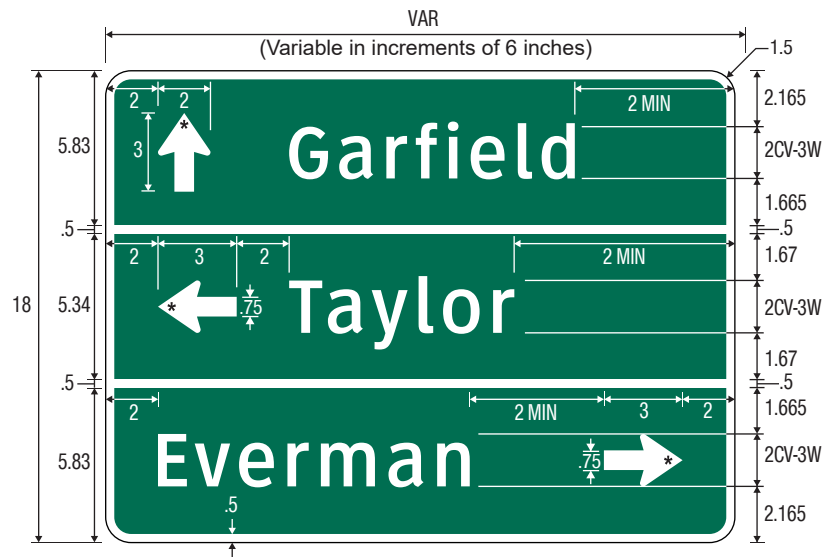
D1-3 [Bicycle] Destination (3 Lines) (Arrows)
