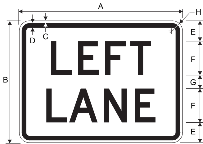
M5-4P LEFT LANE (Plaque)
