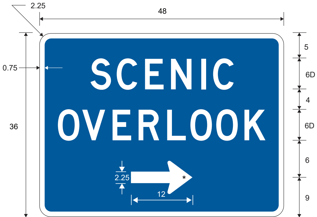
D5-11eTR SCENIC OVERLOOK (Arrow)
