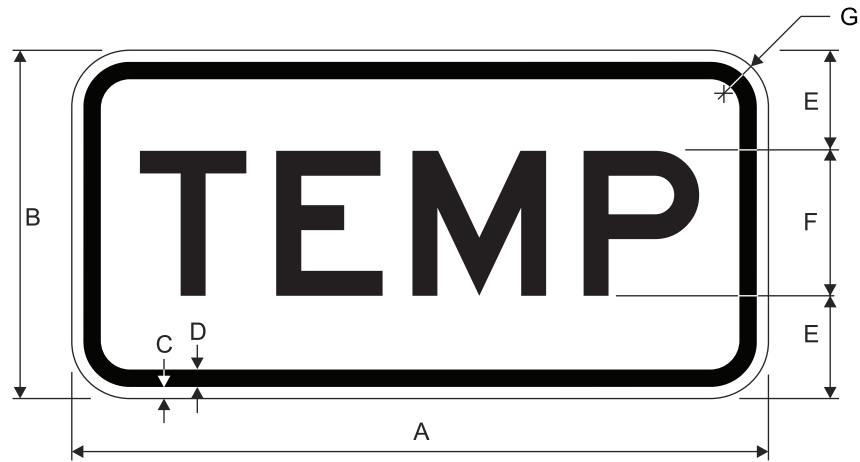
M4-7aP TEMP (Plaque)
