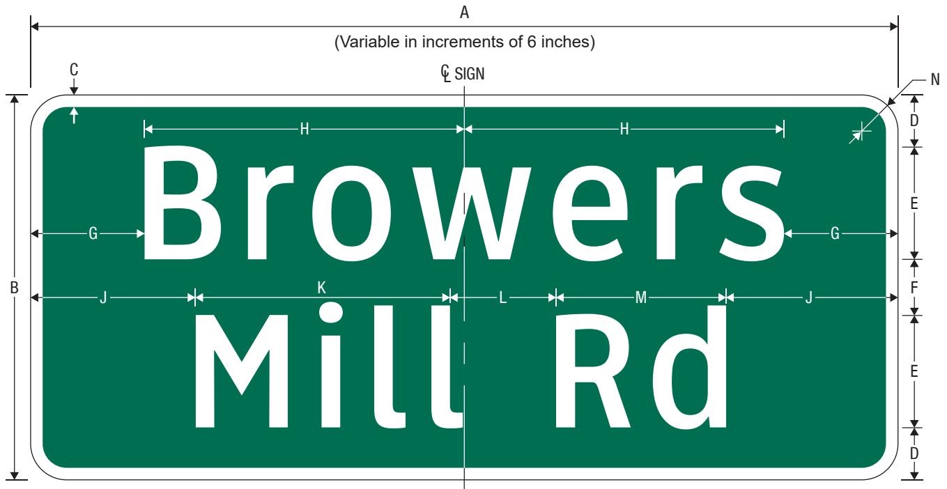
I2-3a Grade Separation Identification (2 Lines)
