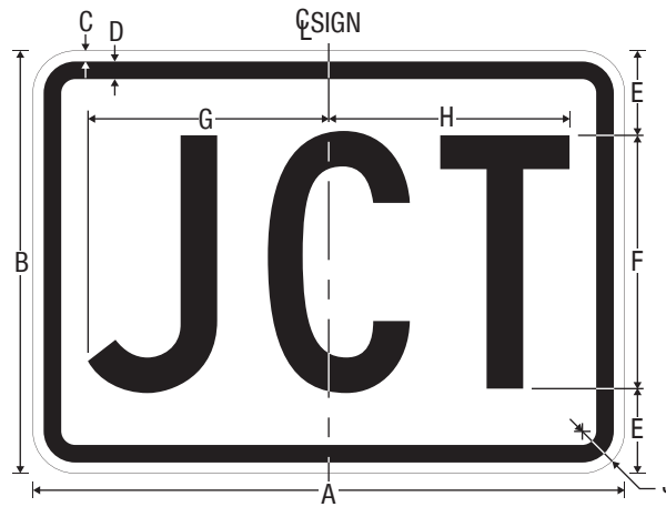
M2-1P Junction (Plaque)
