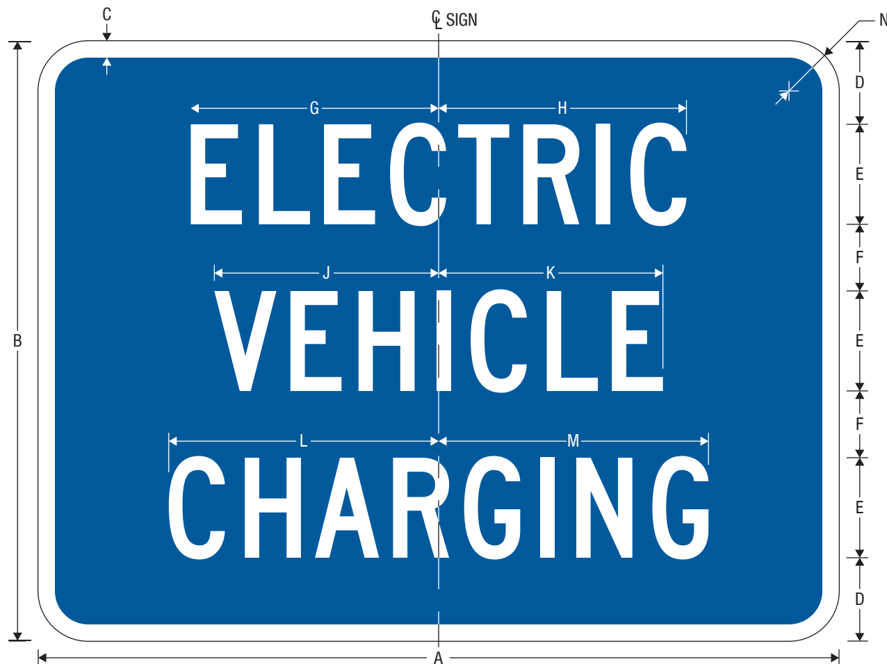
D9-11bP ELECTRIC VEHICLE CHARGING (Plaque)
