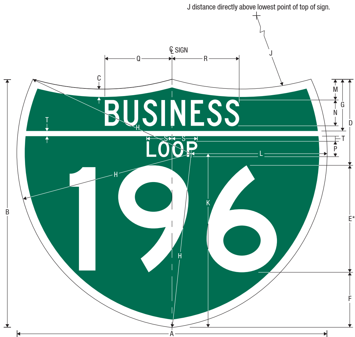
M1-2[A] Off-Interstate Route-Loop Guide Sign Attachment Use (3 Digits)
