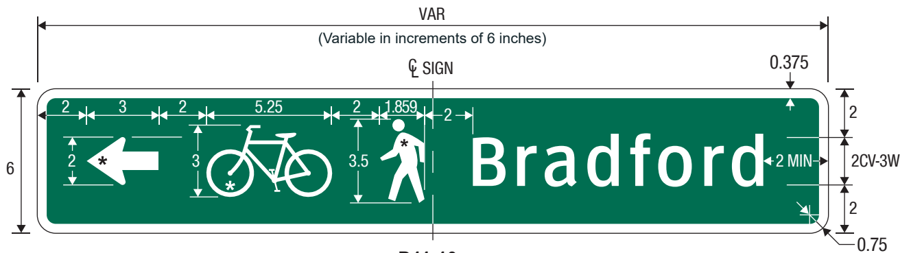
D11-10a Shared-Use Path Destination (1 Line)
