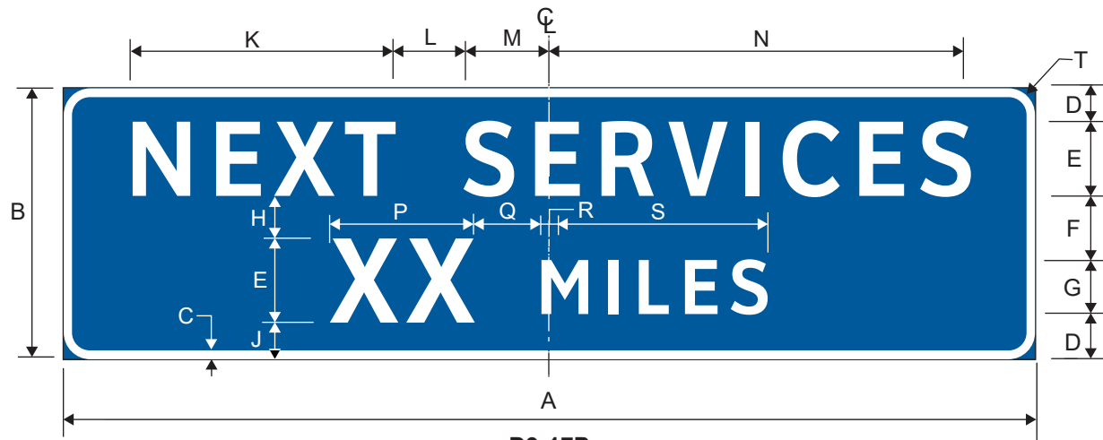
D9-17P NEXT SERVICES XX MILES
