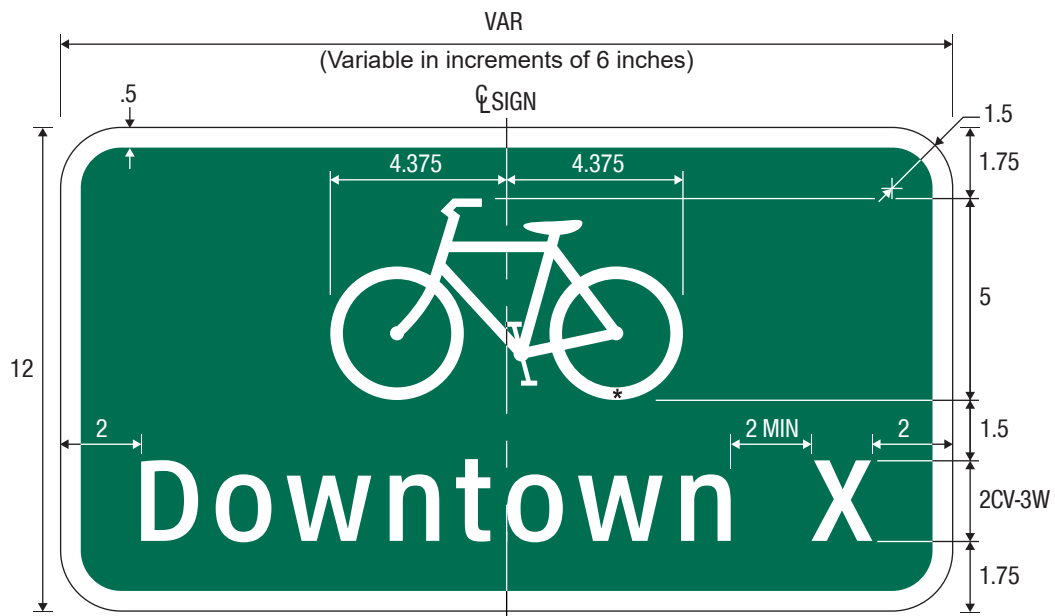
D2-1a Bike Route Destination and Distance (1 Line)
