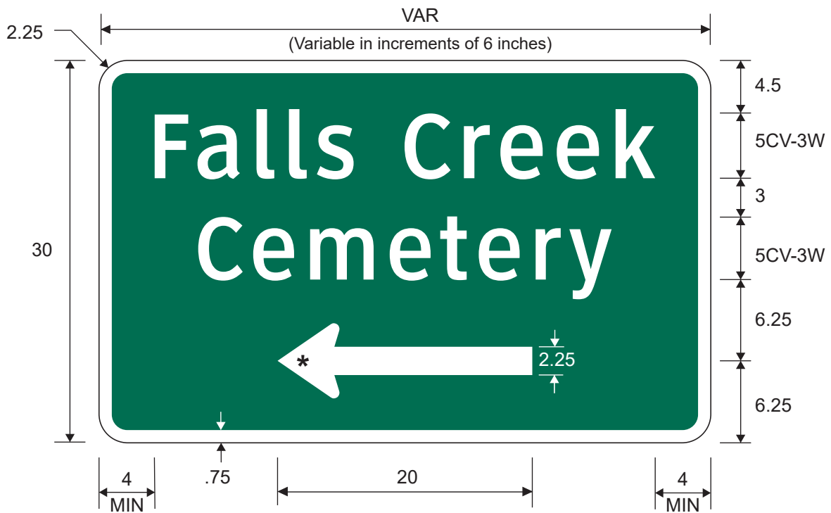
D3-3bTL CEMETERY (2 Lines) (Arrow)
