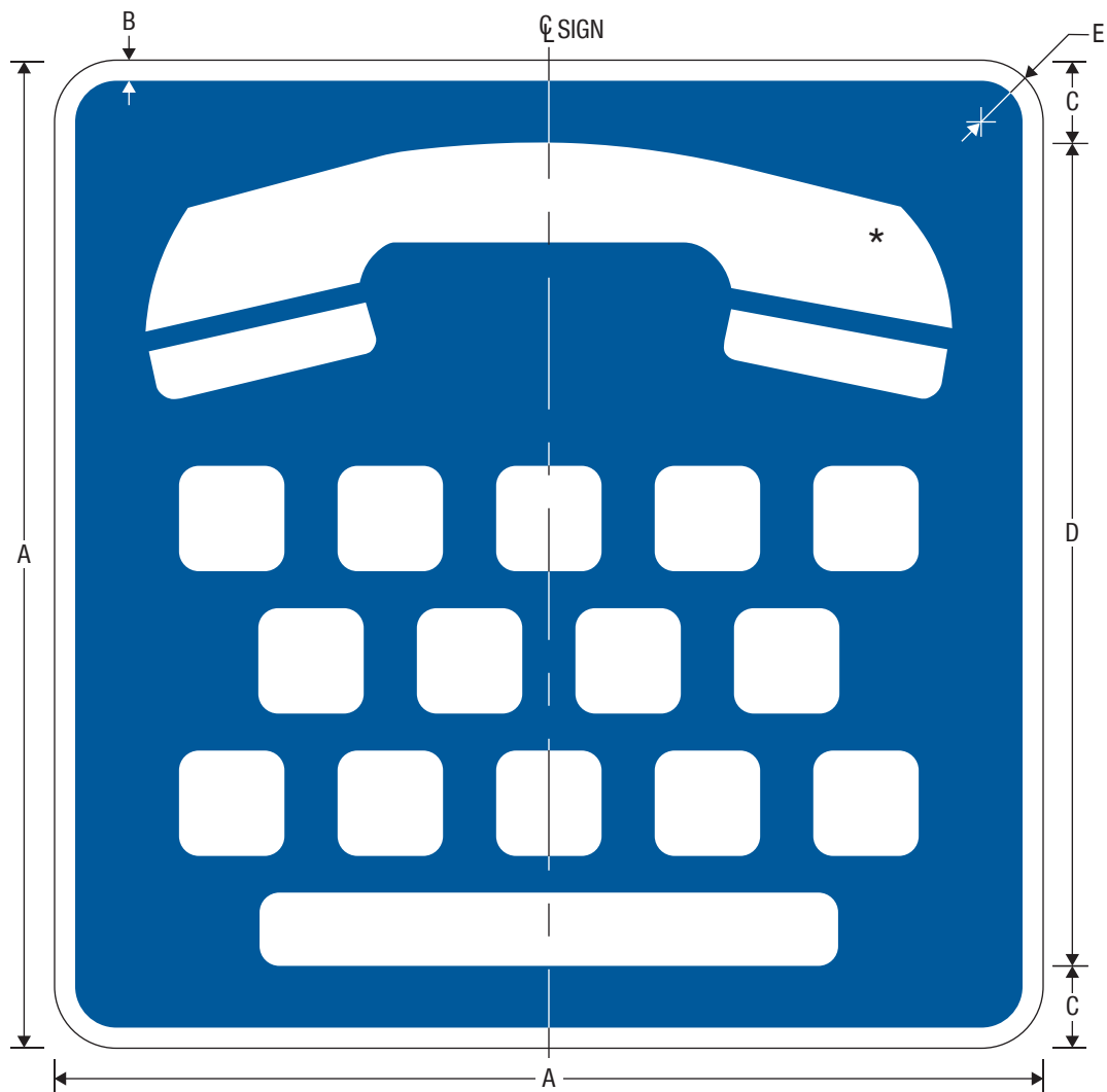
D9-21 Telecommunications Device for the Deaf
