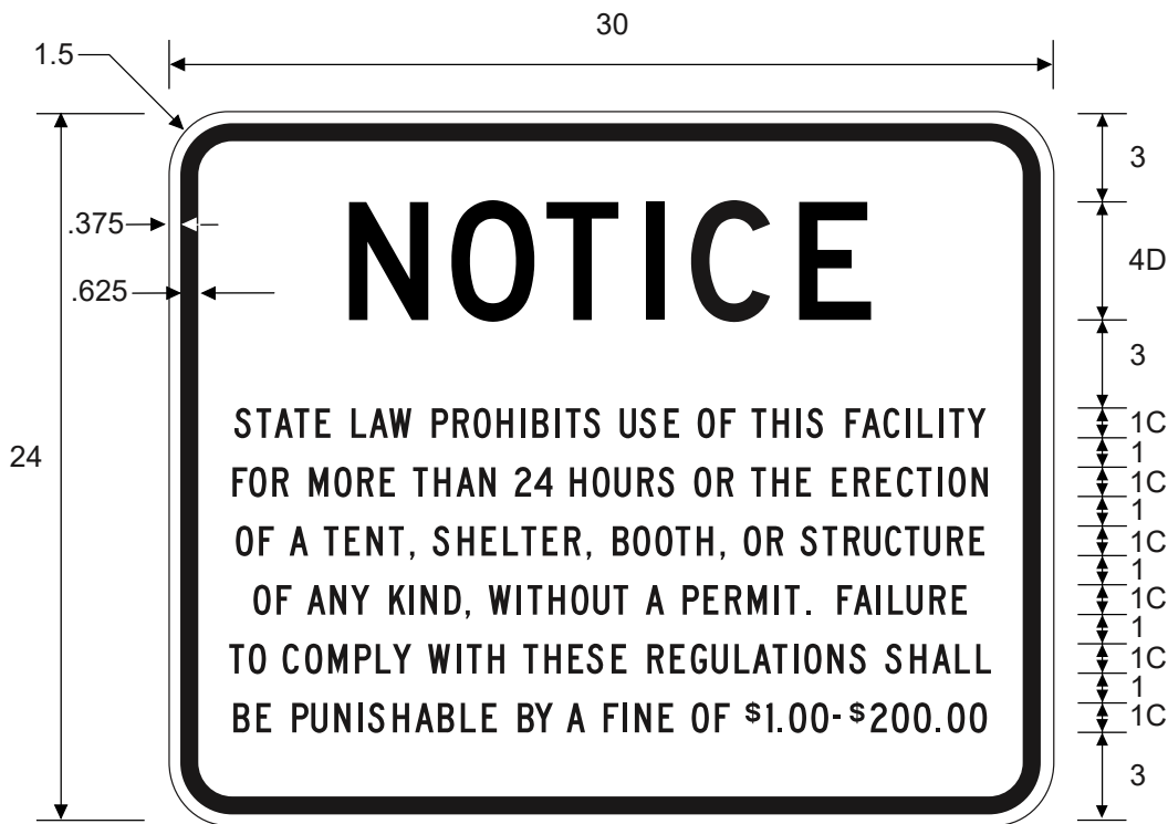
TX2-1T NOTICE STATE LAW USE OF FACILITY
