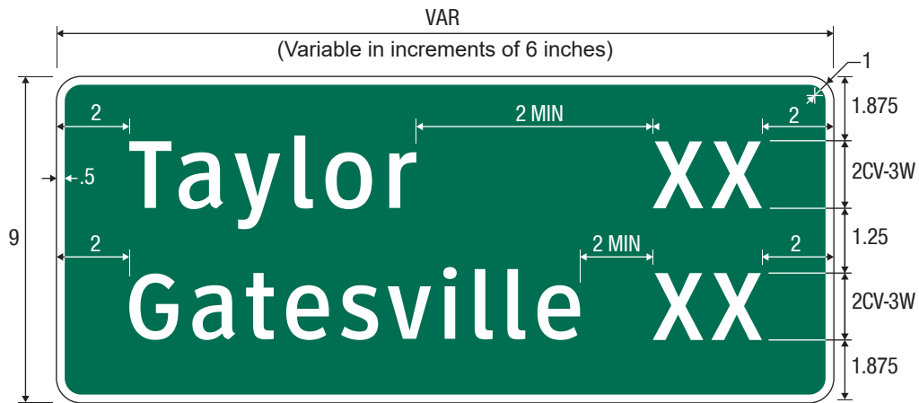
D2-2 [Bicycle] Destination and Distance (2 Lines)
