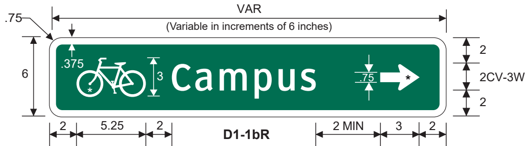
Bicycle Destination (1 Line) (Arrow)
