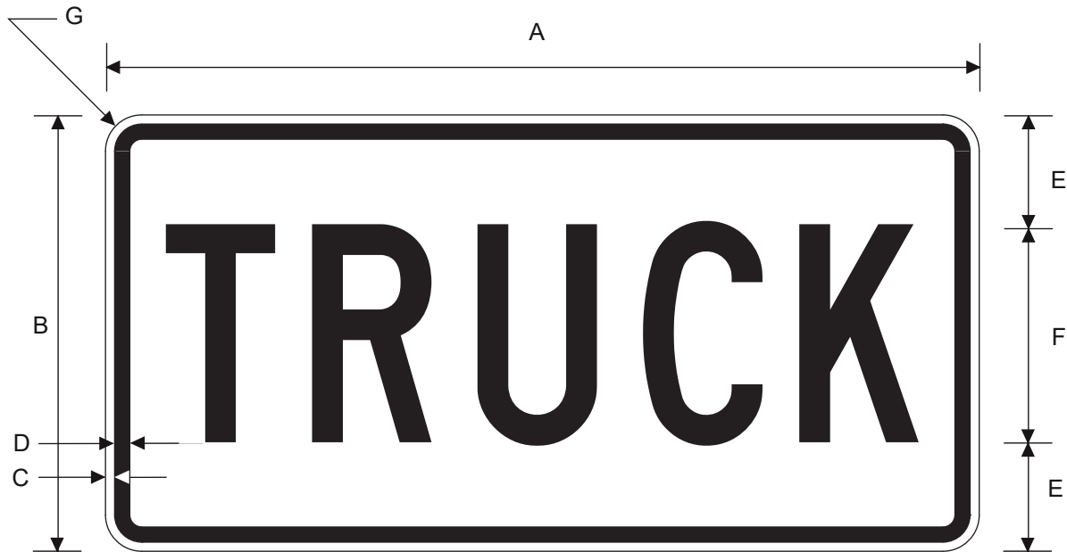
M4-4P TRUCK (Plaque)
