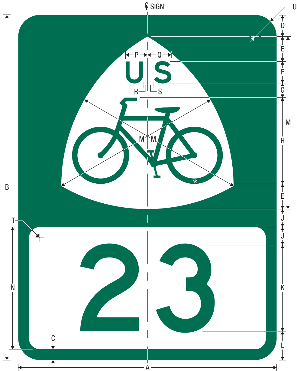
M1-9 U.S. Bicycle Route
