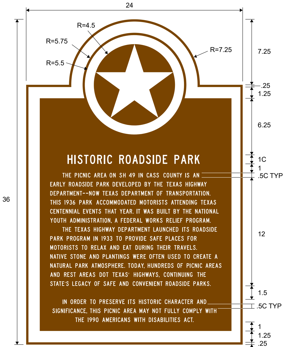
D7-10T HISTORIC ROADSIDE PARK
