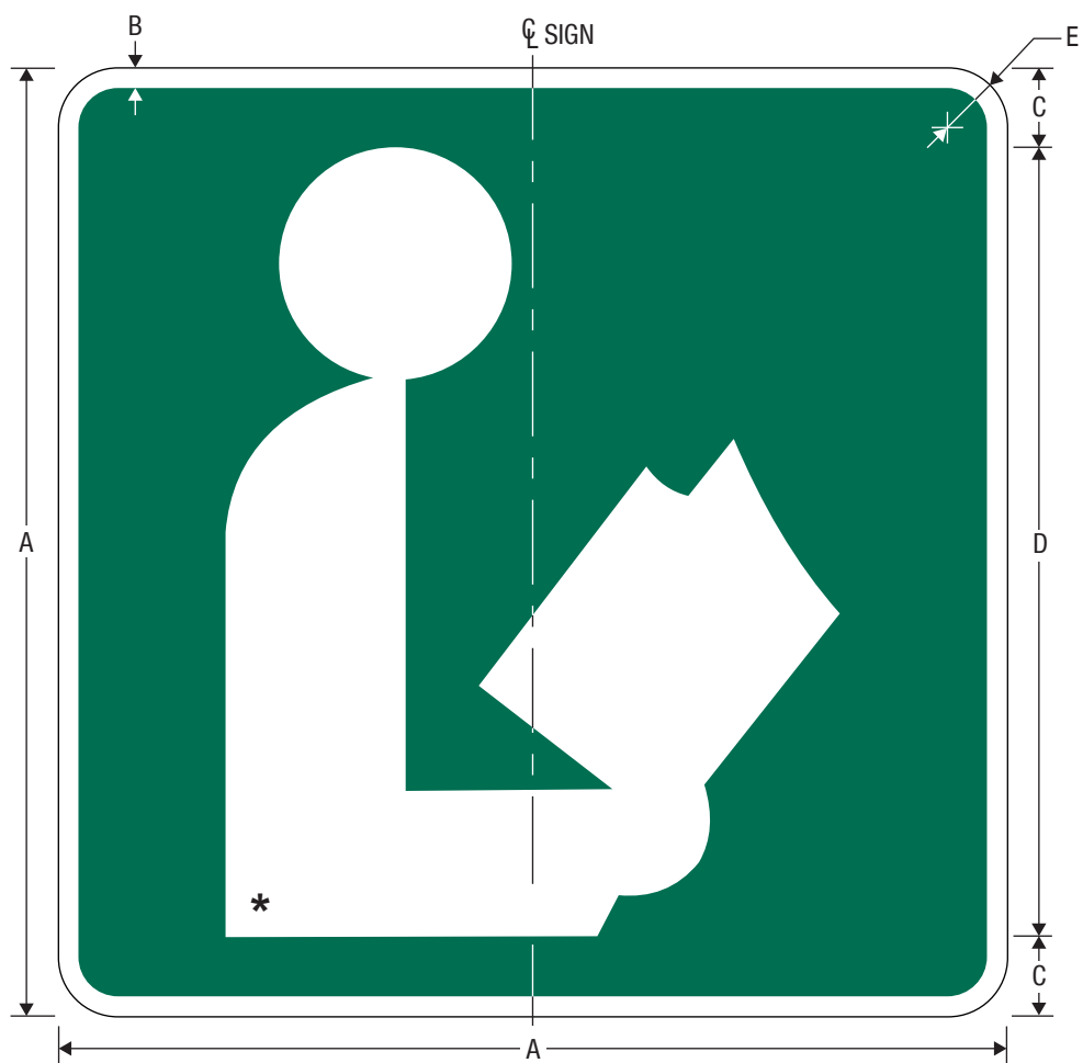
I4-1 Library (Symbol)
