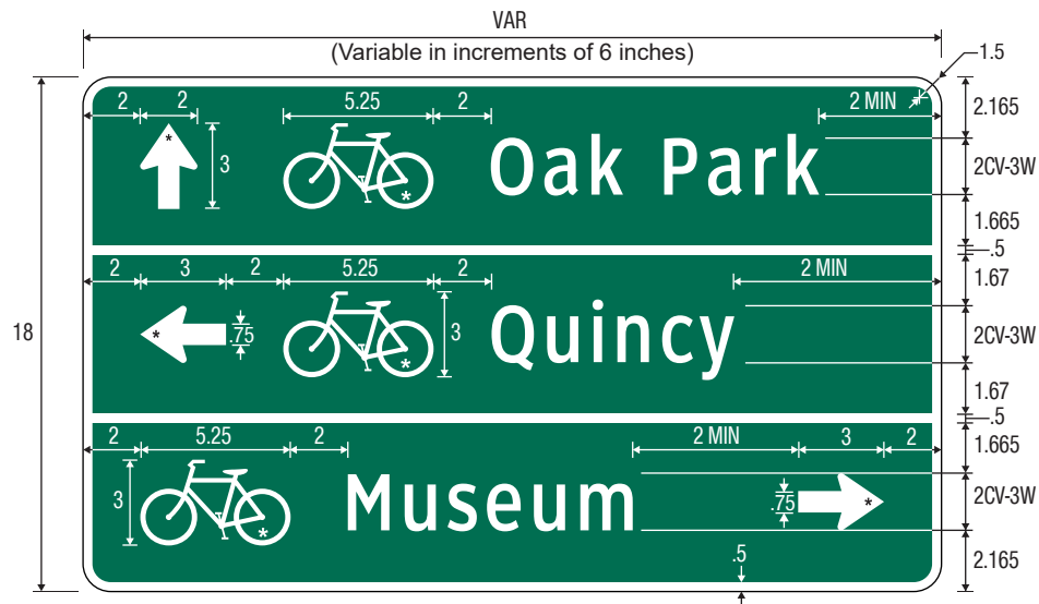
D1-3b Bicycle Destination (3 Lines) (Arrows)
