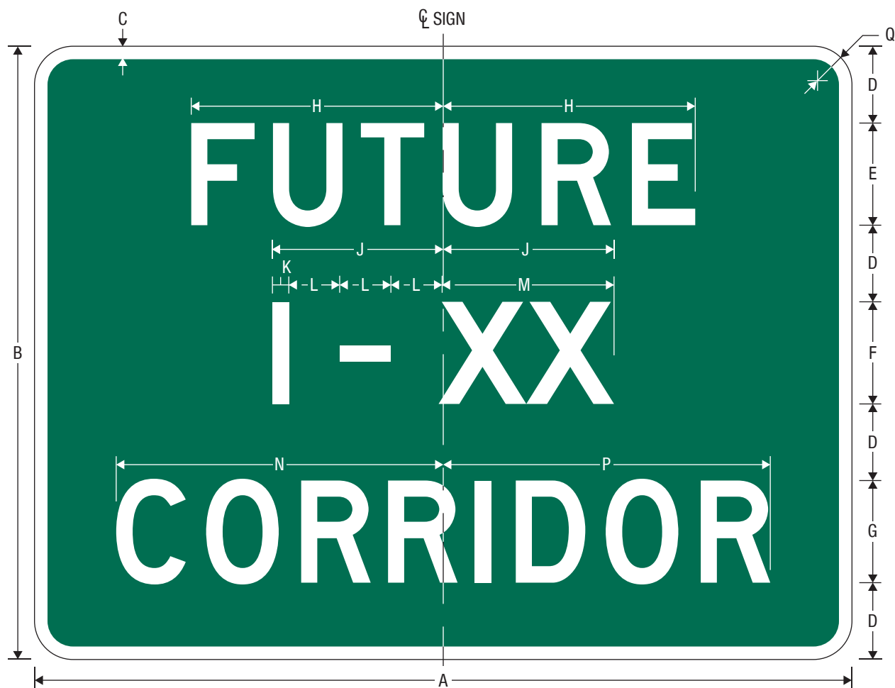
I2-4a FUTURE I-XX CORRIDOR
