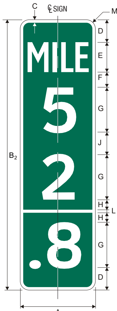
D10-2a Intermediate Reference Location (2 Digits with decimal)
