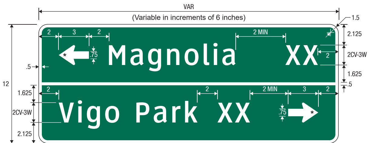
D1-2a [Bicycle] Destination and Distance (2 Lines) (Arrows)
