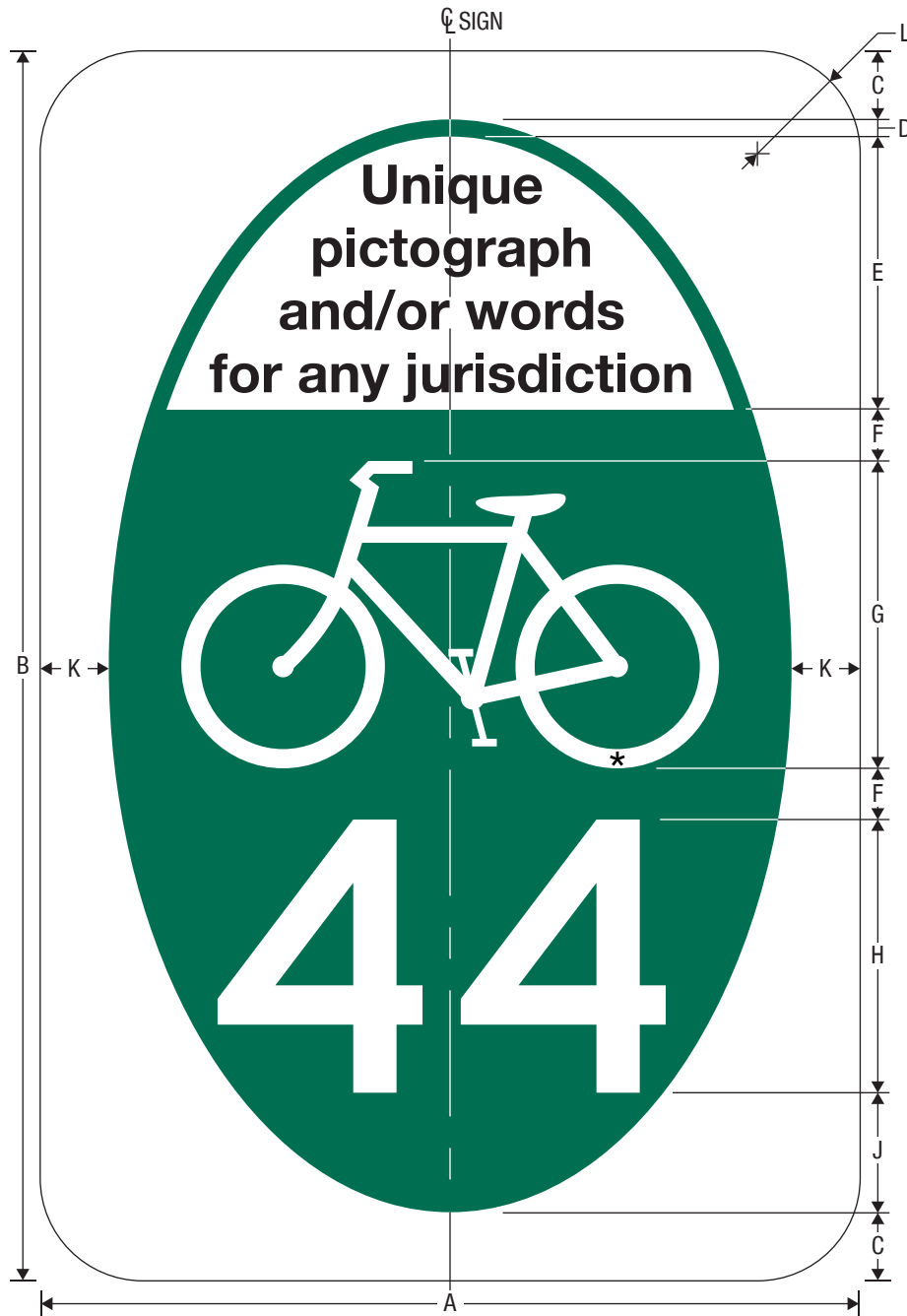
M1-8a State or Local Bicycle Route
