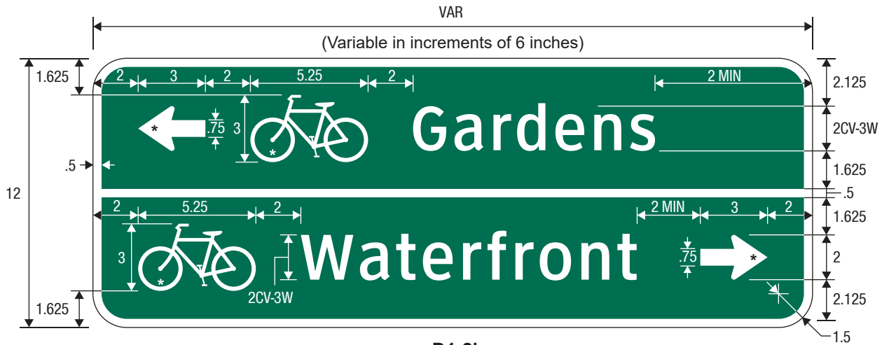
D1-2b Bicycle Destination (2 Lines) (Arrows)
