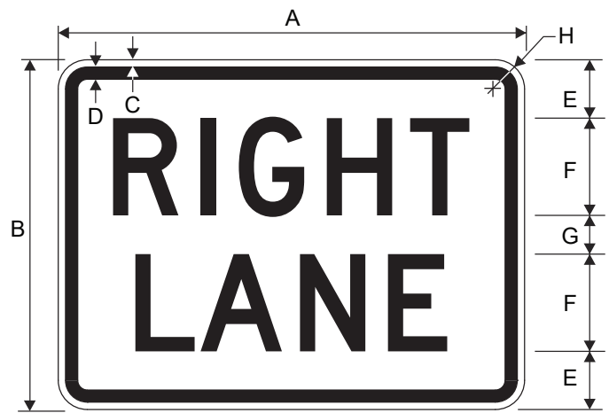
M5-6P RIGHT LANE (Plaque)
