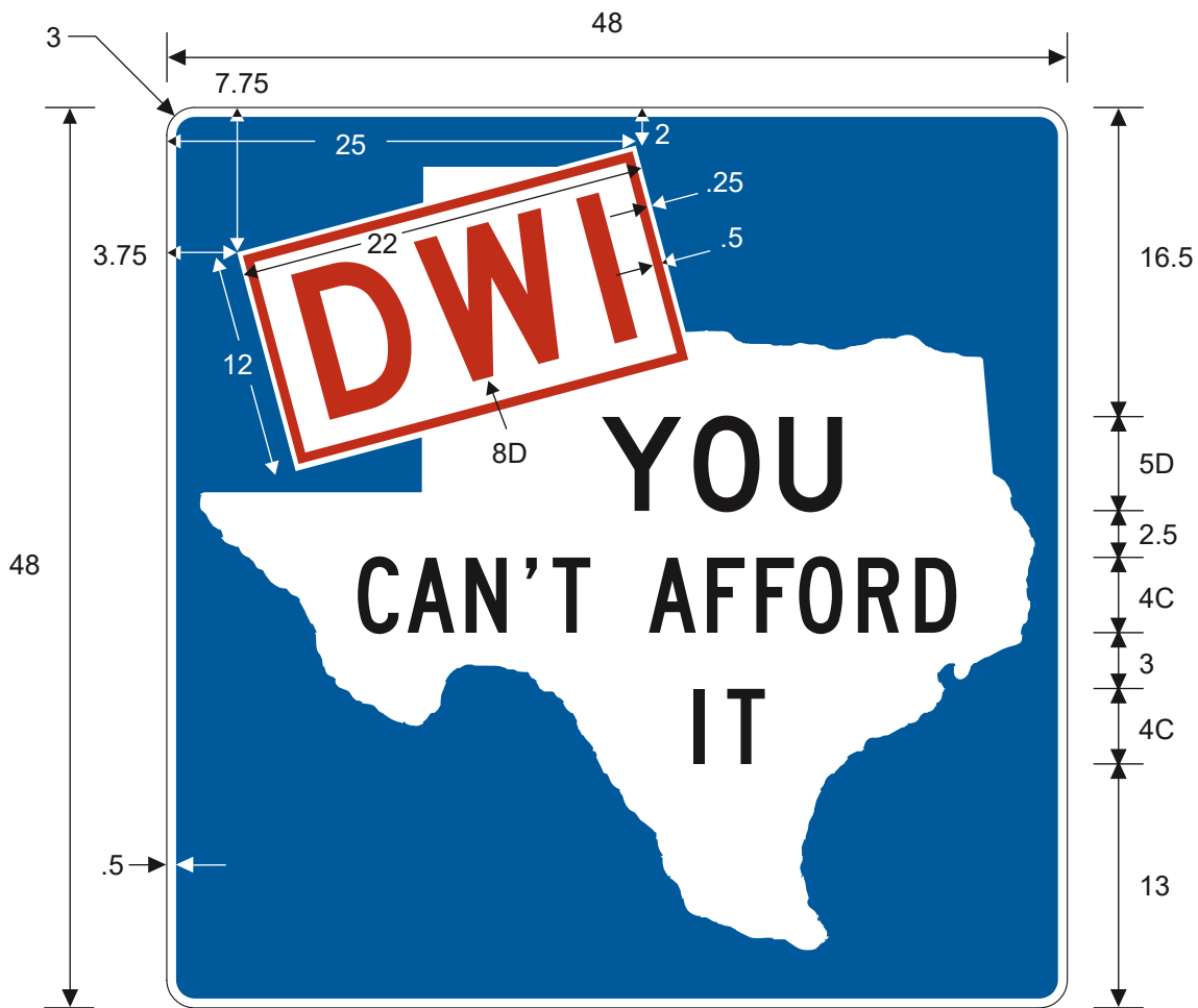
D12-7T DWI YOU CAN'T AFFORD IT
