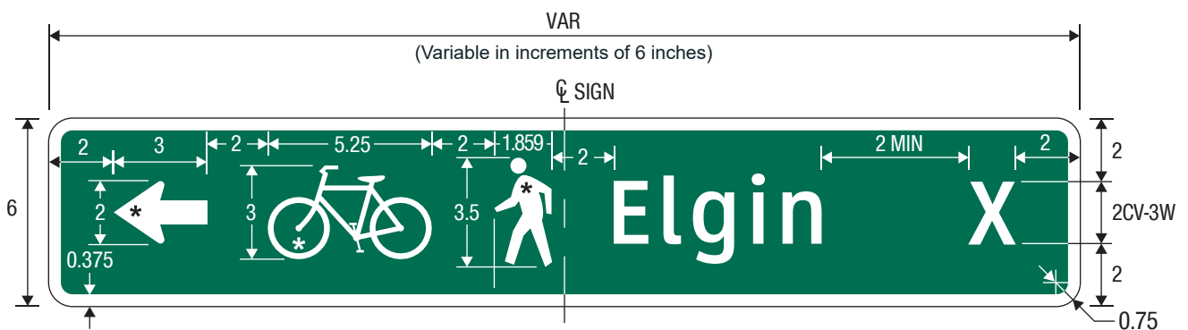
D11-10d Shared-Use Path Destination and Distance (1 Line)
