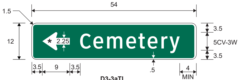
D3-3aTL CEMETERY (1 Line) (Arrow)
