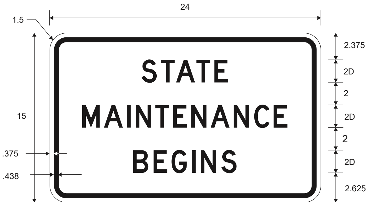
TX1-2T STATE MAINTENANCE BEGINS
