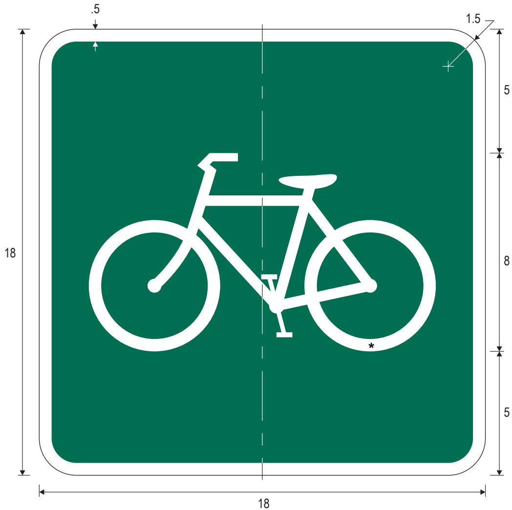
D11-11 Bicycles Directional (Symbol)
