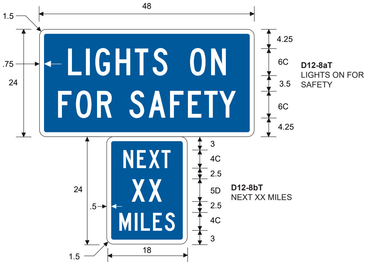
D12-8T LIGHTS ON FOR SAFETY TURN ON HEADLIGHTS NEXT XX MILES
