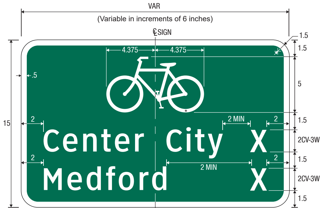
D2-2a Bike Route Destination and Distance (2 Lines)
