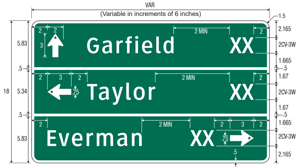
D1-3a [Bicycle] Destination and Distance (3 Lines) (Arrows)
