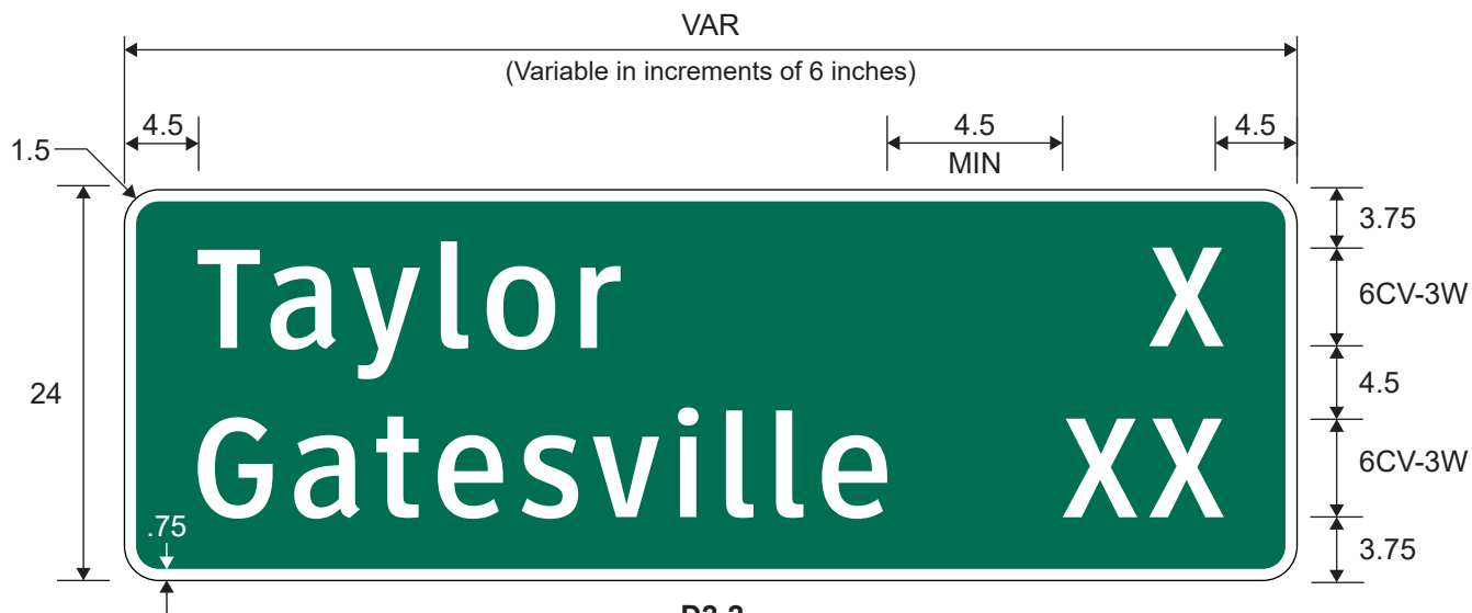
D2-2 Destination and Distance (2 Lines)
