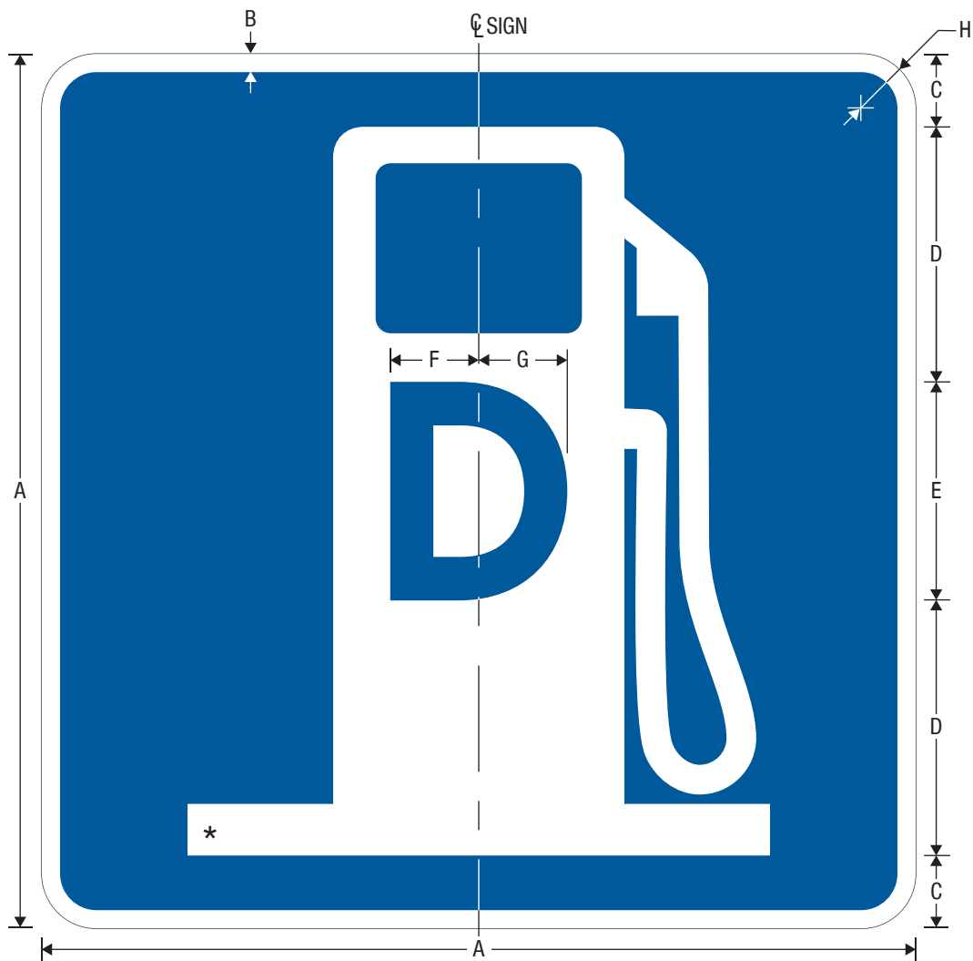
D9-11 Diesel Fuel
