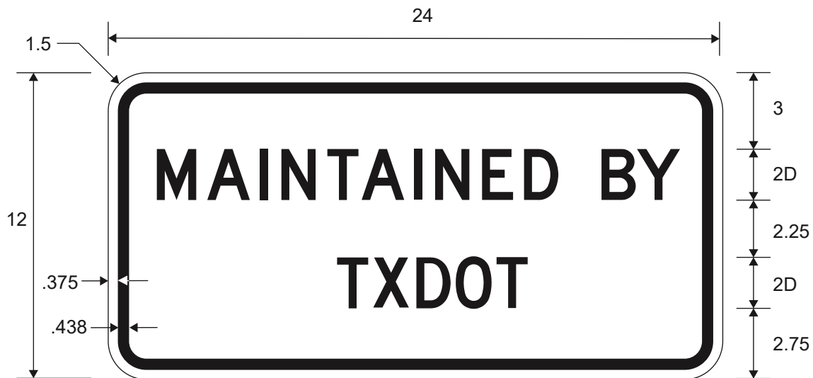
TX1-4T MAINTAINED BY TXDOT
