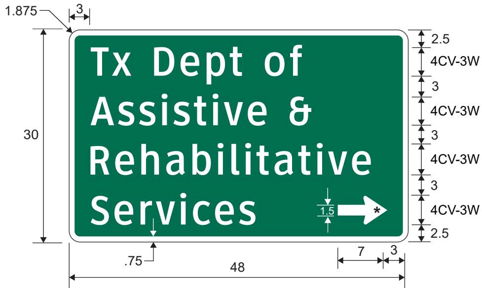
D26-6TR TEXAS DEPARTMENT OF ASSISTIVE AND REHABILITATIVE SERVICES (Arrow)
