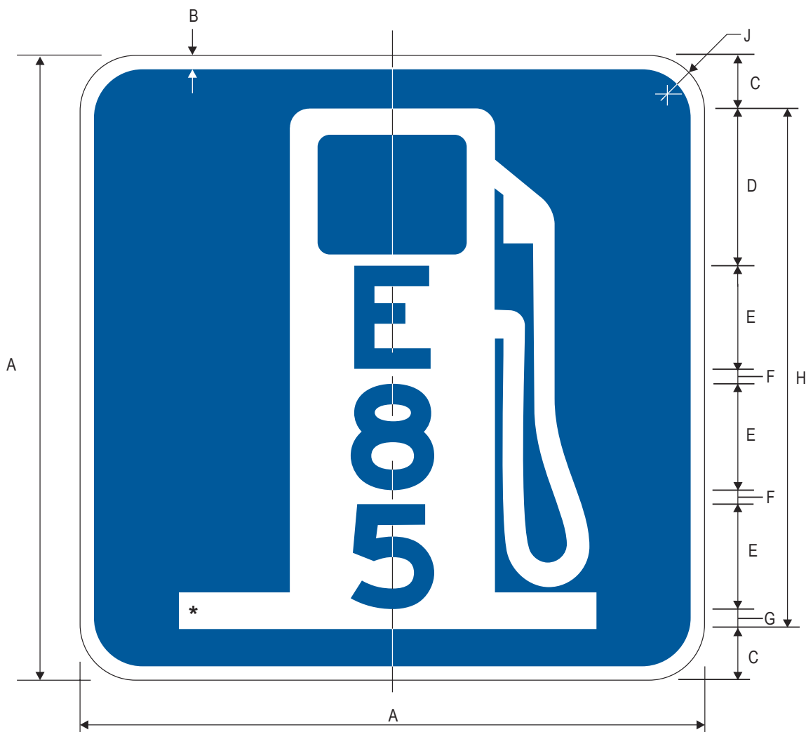
D9-11c Alternative Fuel (Ethanol)
