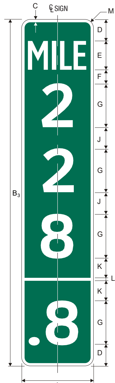
D10-3a Intermediate Reference Location (3 Digits with decimal)
