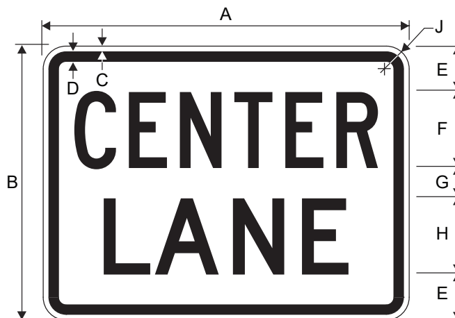
M5-5P CENTER LANE (Plaque)
