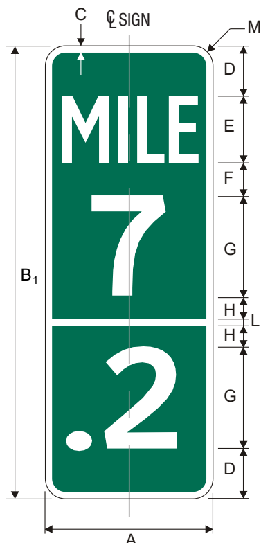
D10-1a Intermediate Reference Location (1 Digit with decimal)
