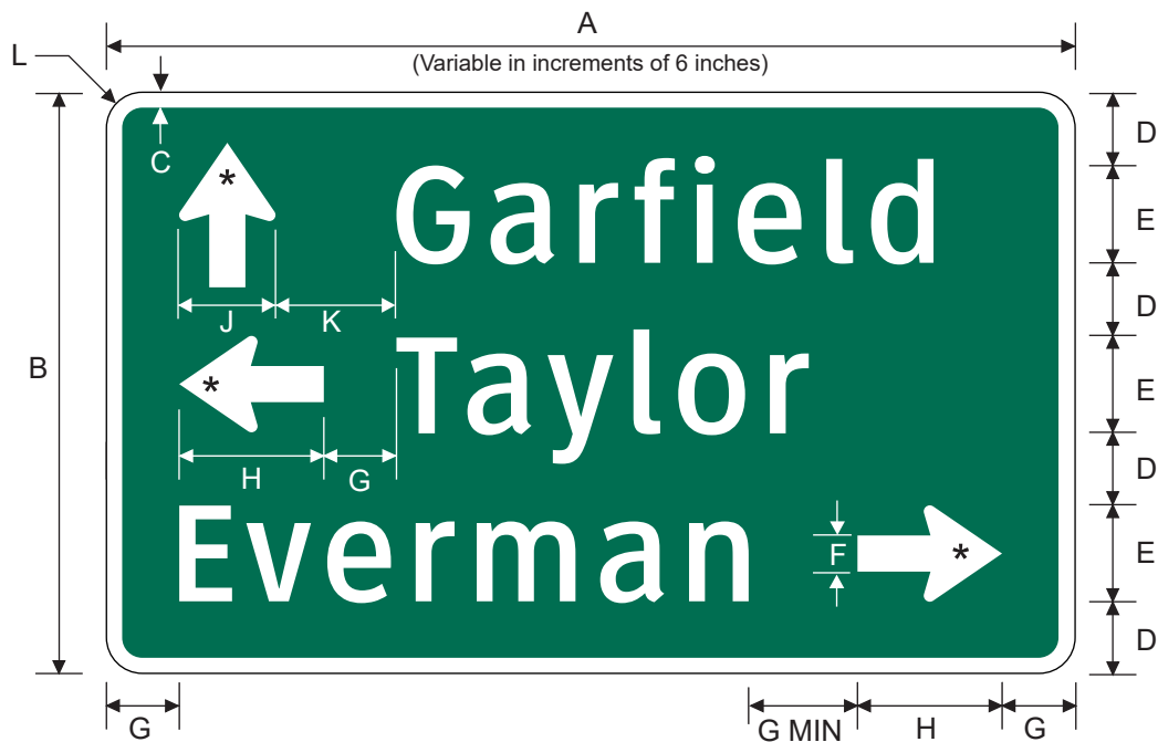
D1-3 Destination (3 Lines) (Arrows)
