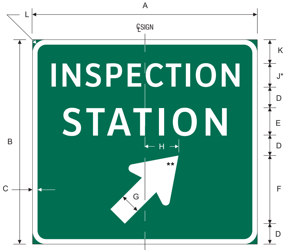
D8-3aT INSPECTION STATION (Arrow)
