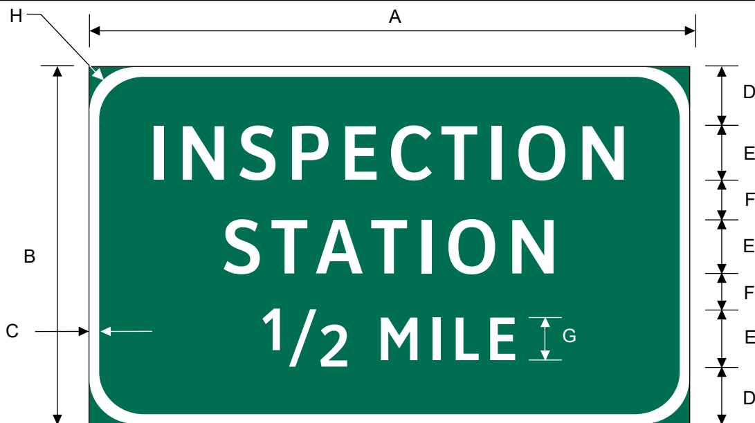
D8-2aT INSPECTION STATION 1/2 MILE
