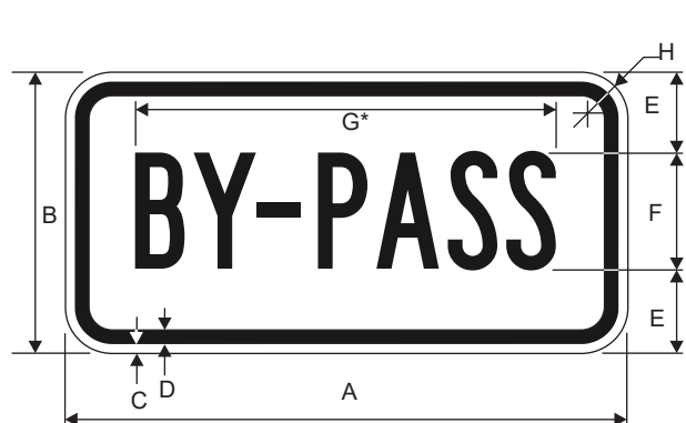
M4-2P BY-PASS (Plaque)
