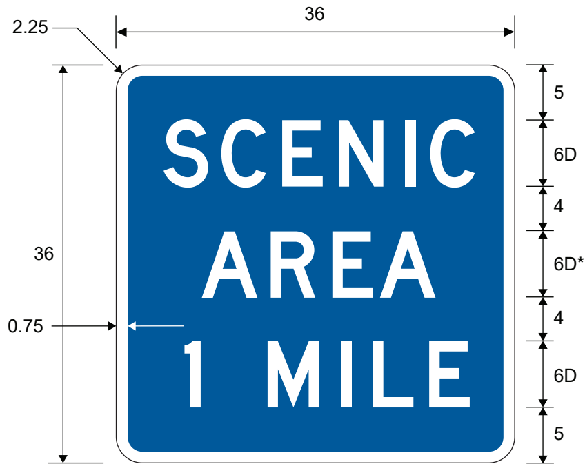
D5-11T[A] SCENIC AREA X MILE
