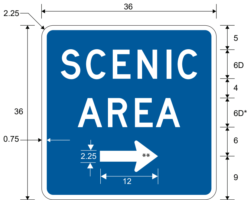
D5-11cTR SCENIC AREA (VIEW) (Arrow)
