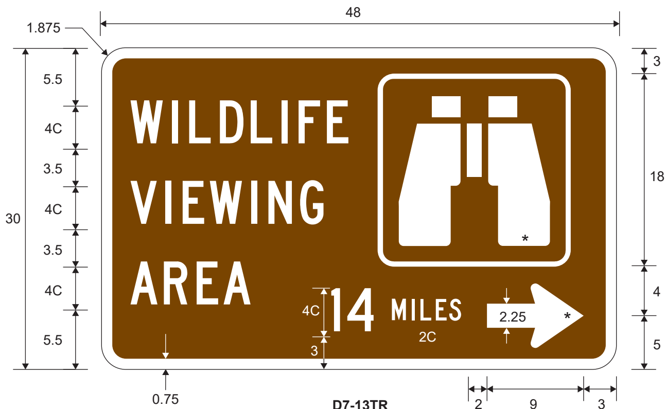
D7-13TR WILDLIFE VIEWING AREA (with Distance and Binoculars Symbol attached (Arrow))
