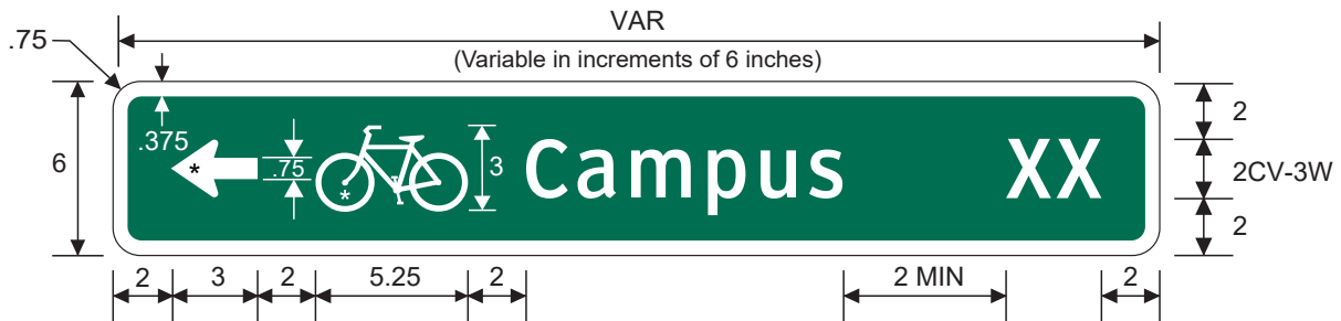
Bicycle Destination and Distance (1 Line) (Arrow)
