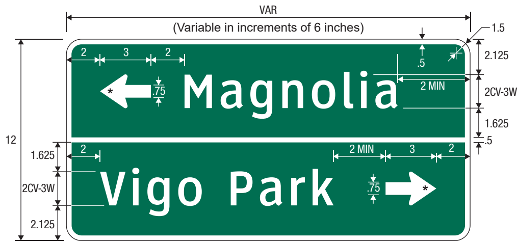
D1-2 [Bicycle] Destination (2 Lines) (Arrows)
