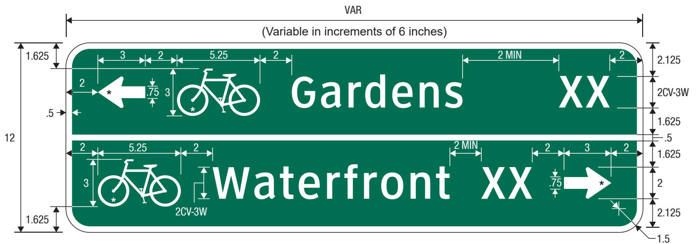
D1-2c Bicycle Destination and Distance (2 Lines) (Arrows)
