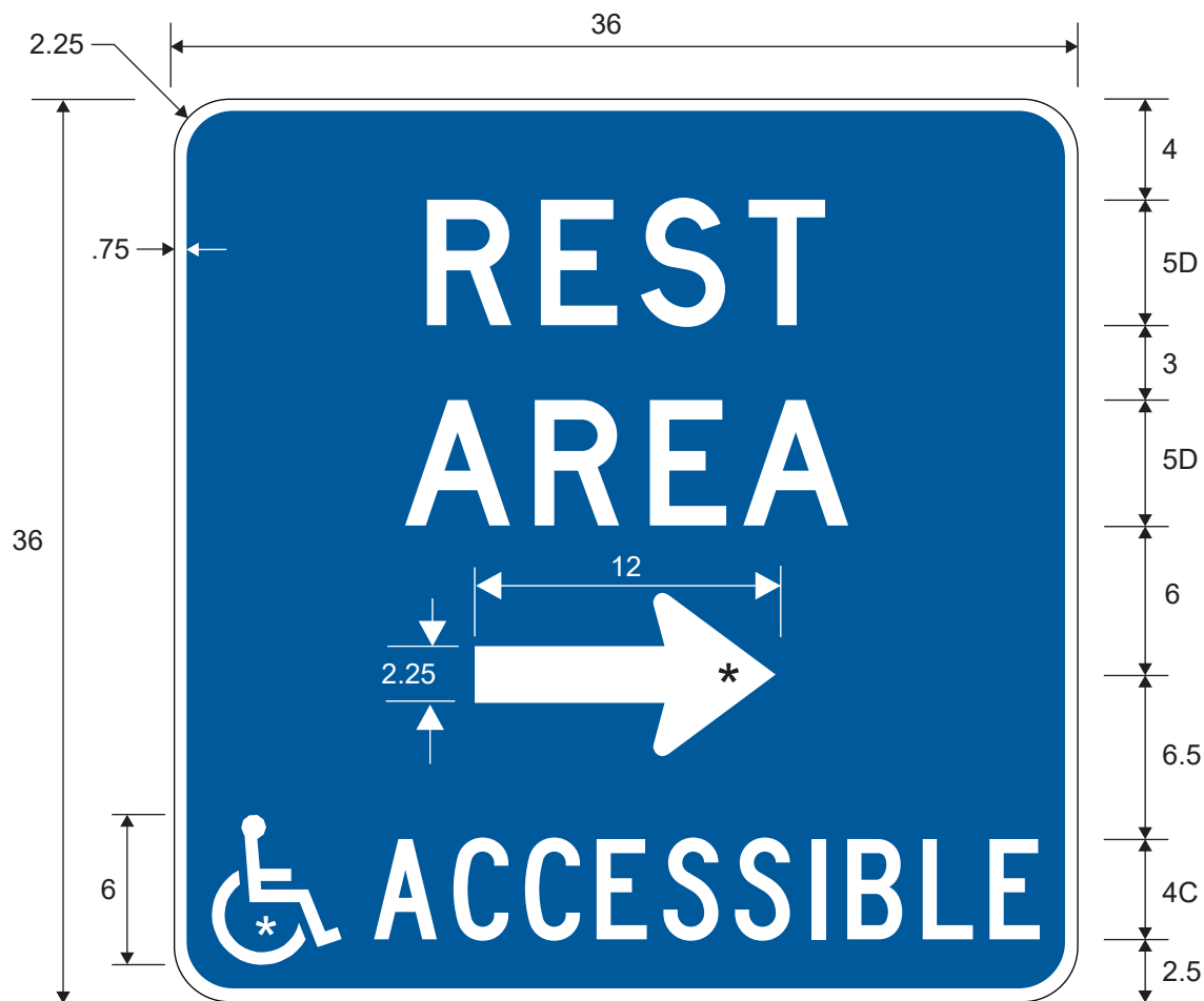
D5-5TR REST AREA ACCESSIBLE (with Arrow and Symbol)
