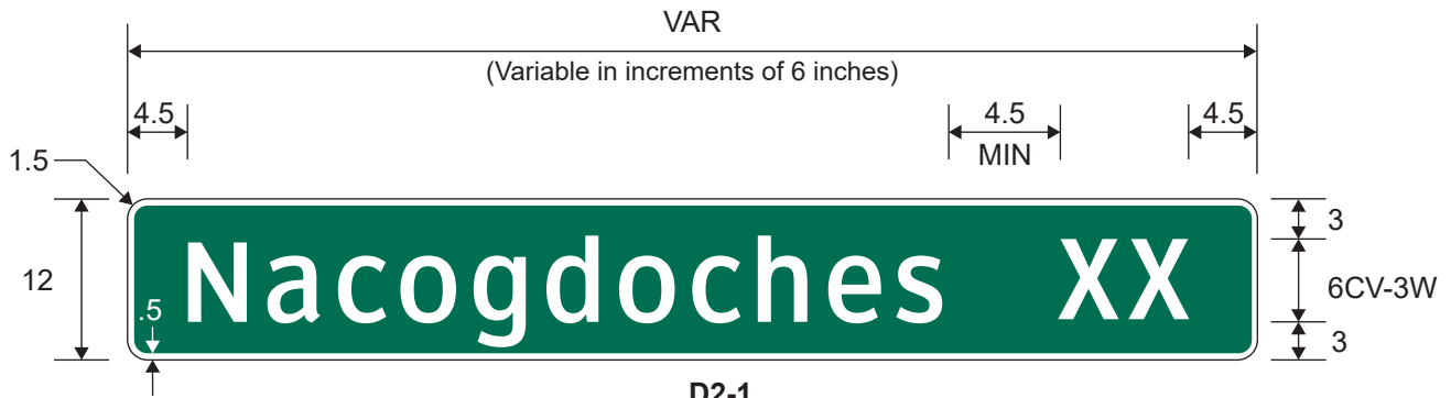
Destination and Distance (1 Line)
