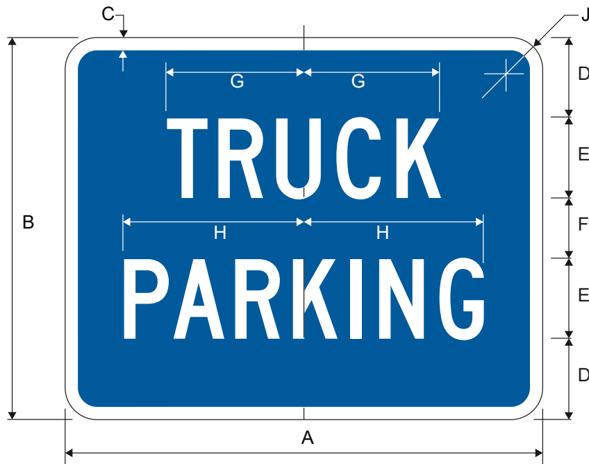
D9-16PT TRUCK PARKING
