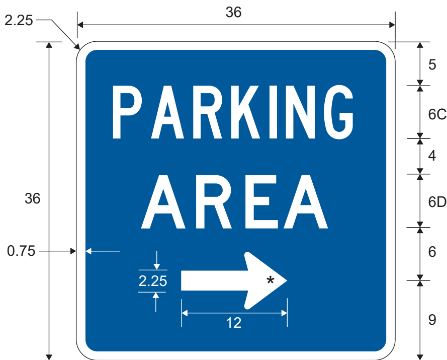
D5-9cTR PARKING AREA (Arrow)
