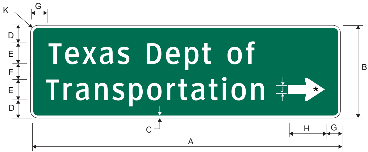
D26-10TR TEXAS DEPT OF TRANSPORTATION (Arrow)
