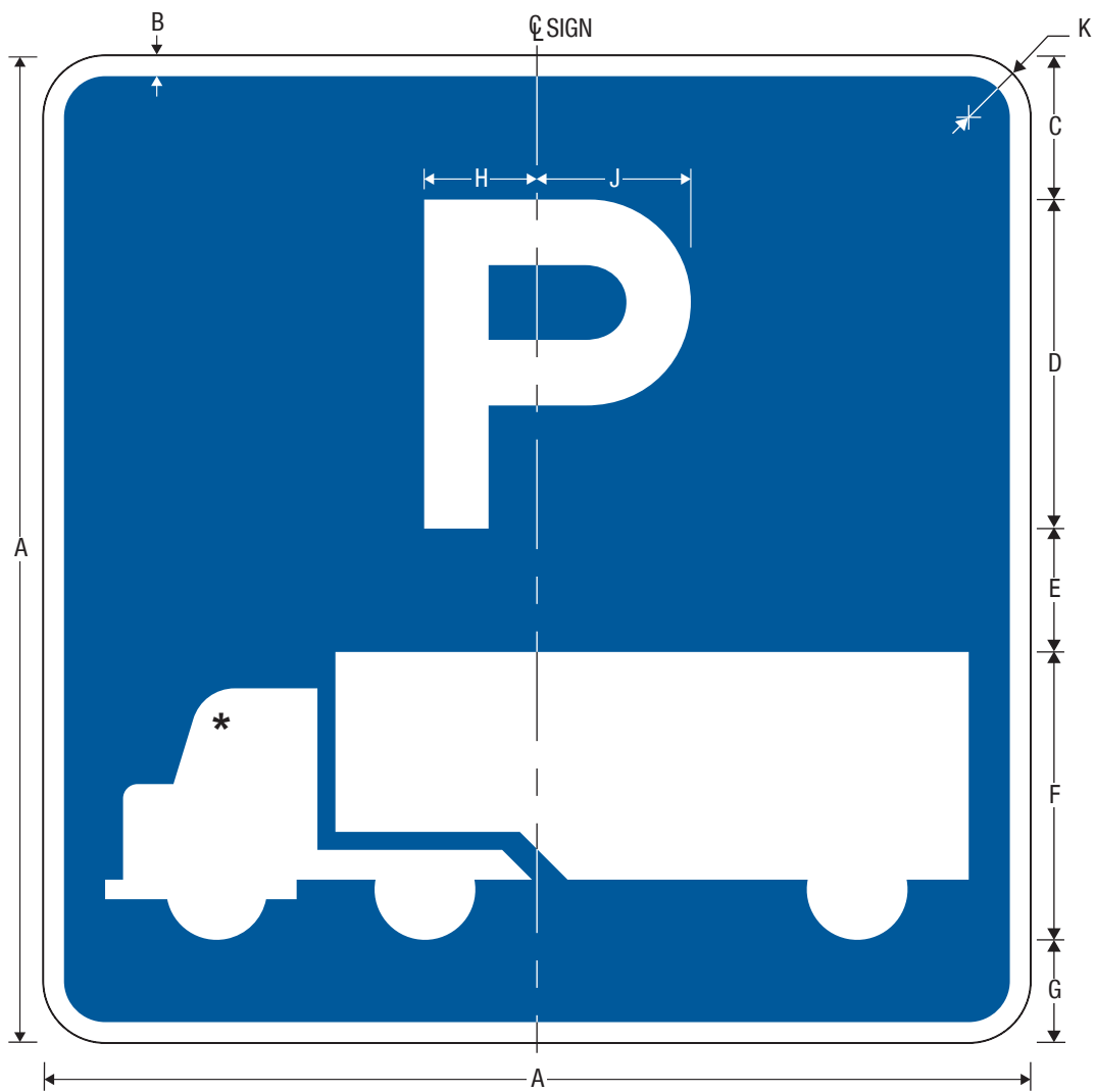
D9-16 Truck Parking
