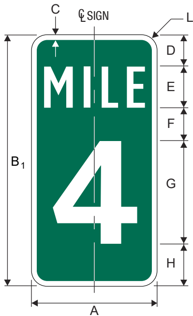
D10-1 Reference Location (1 Digit)
