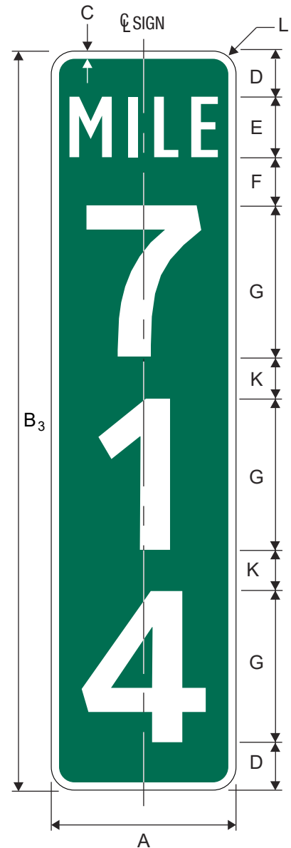
D10-3 Reference Location (3 Digits)
