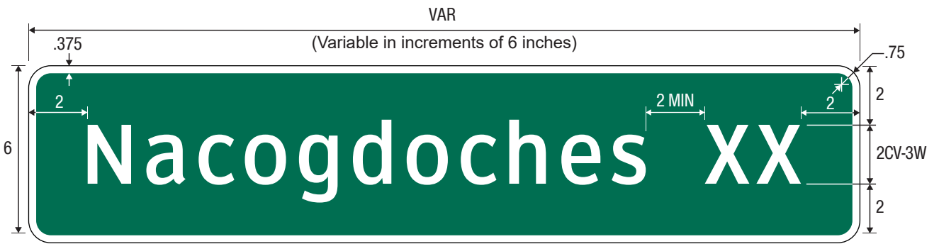
D2-1 [Bicycle] Destination and Distance (1 Line)
