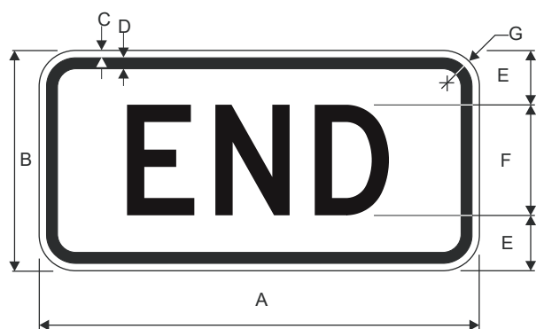
M4-6P END (Plaque)
