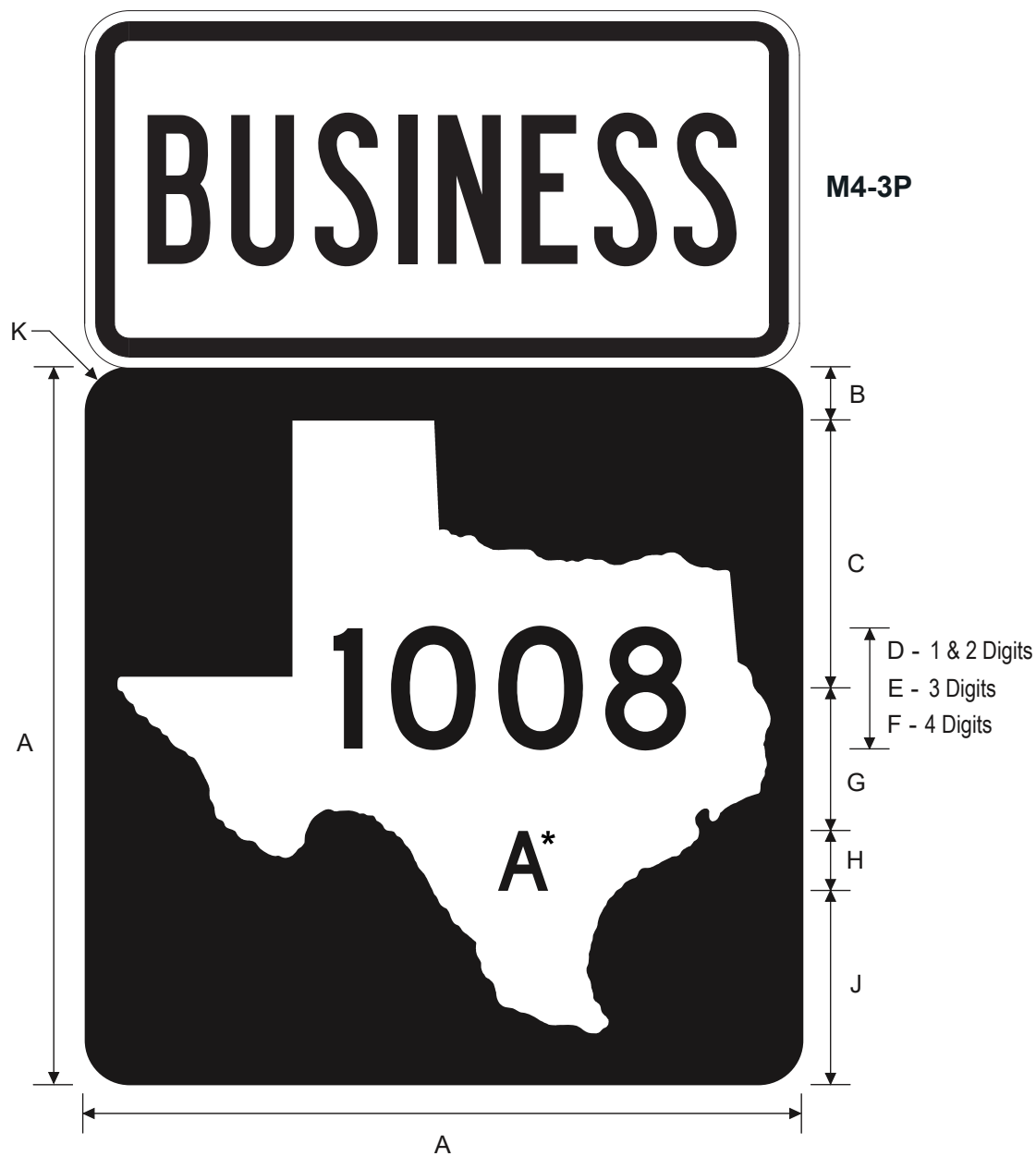
M1-5FB Texas Business Assembly Road Route Marker (Independent)
