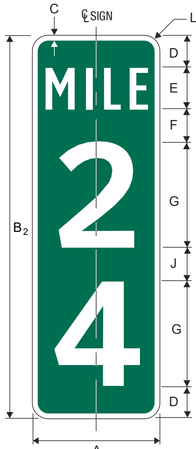
D10-2 Reference Location (2 Digits)
