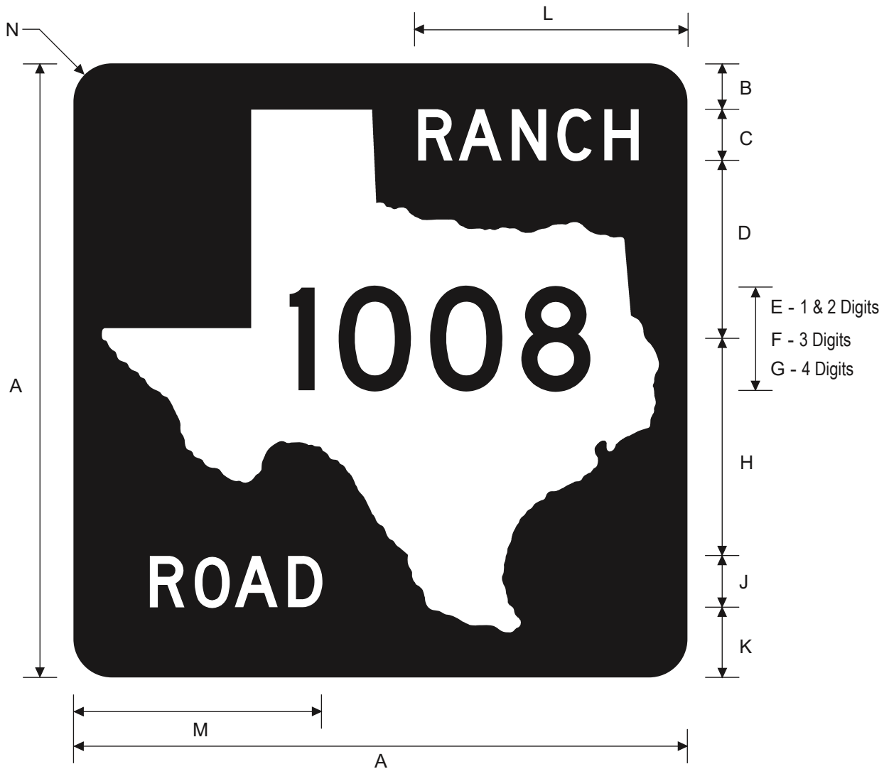
M1-5R Texas RANCH ROAD Route Marker (Independent)
