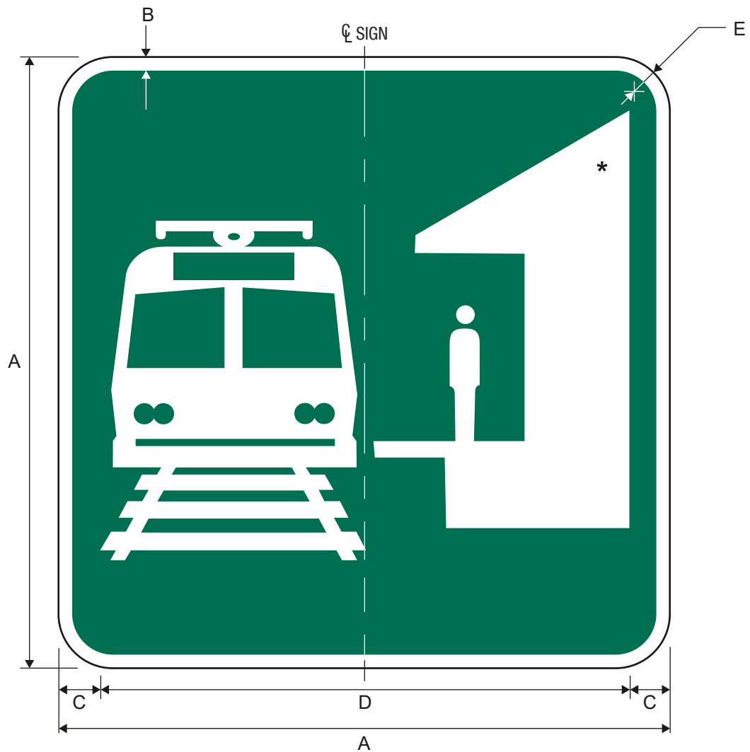
I3-8 Light Rail Transit Station (Symbol)
