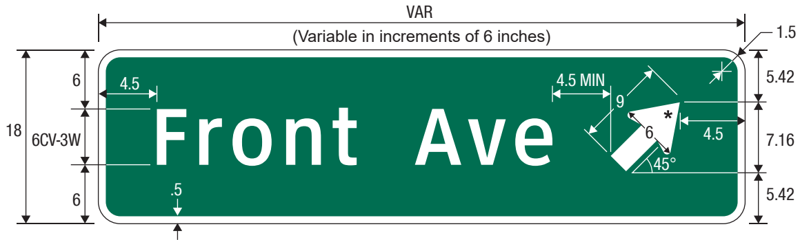
D1-1d Circular Intersection Destination (1 Line) (Arrow)
