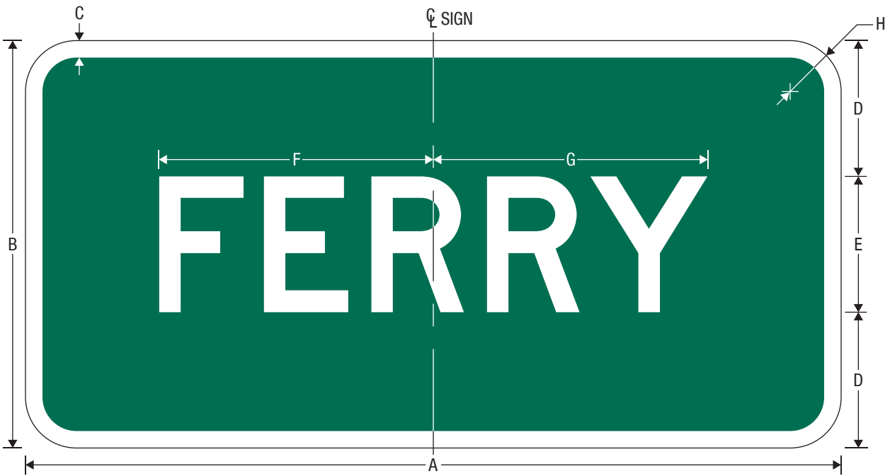
13-10P Ferry (Plaque)
