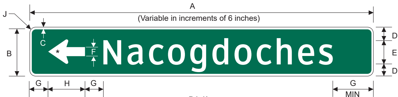
D1-1L Destination (1 Line) (Arrow)
