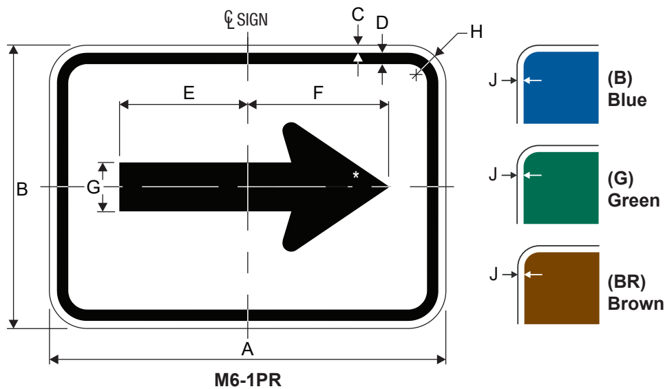
Directional Arrow - Single Head Horizontal (Plaque)
