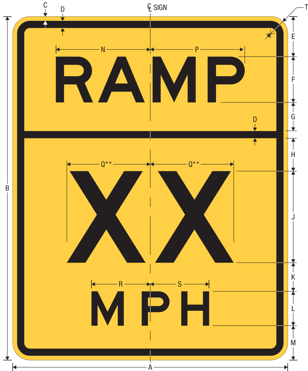
W13-3 Advisory Ramp Speed *Increase Spacing 100%. **Optically space numerals about centerline.
