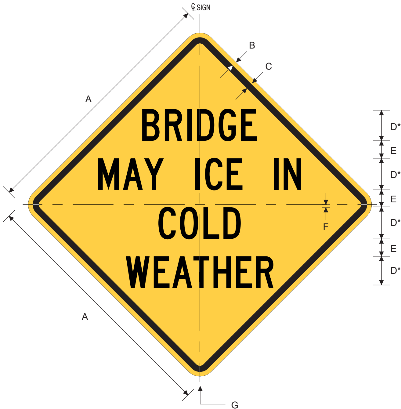
W8-13aT BRIDGE MAY ICE IN COLD WEATHER
