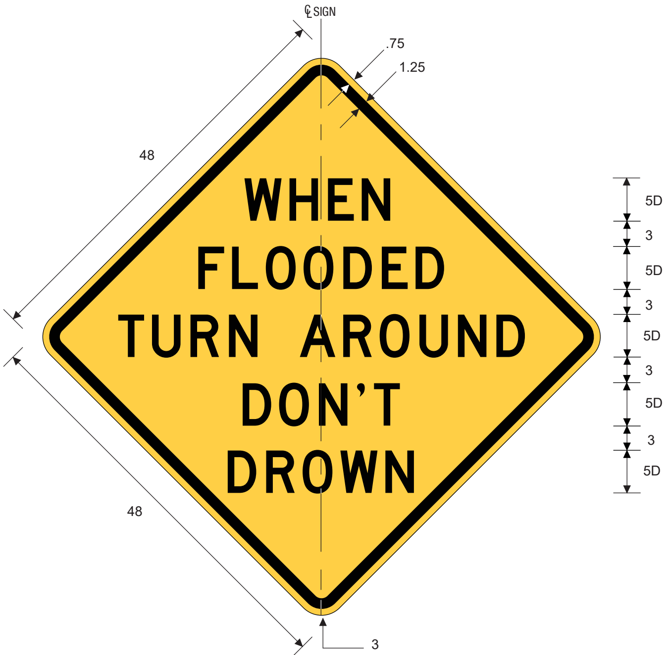
W8-18bT WHEN FLOODED TURN AROUND DON'T DROWN
