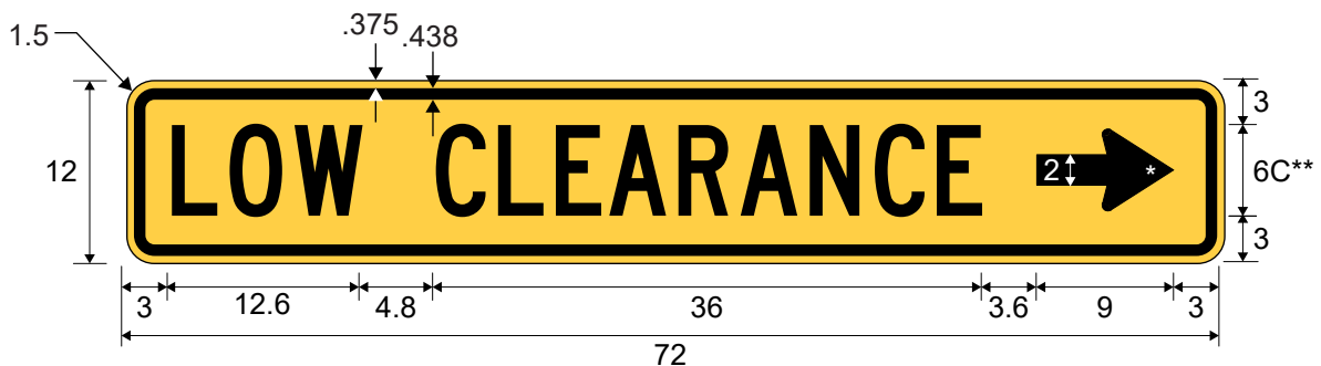
W12-3PTR LOW CLEARANCE (Plaque)
