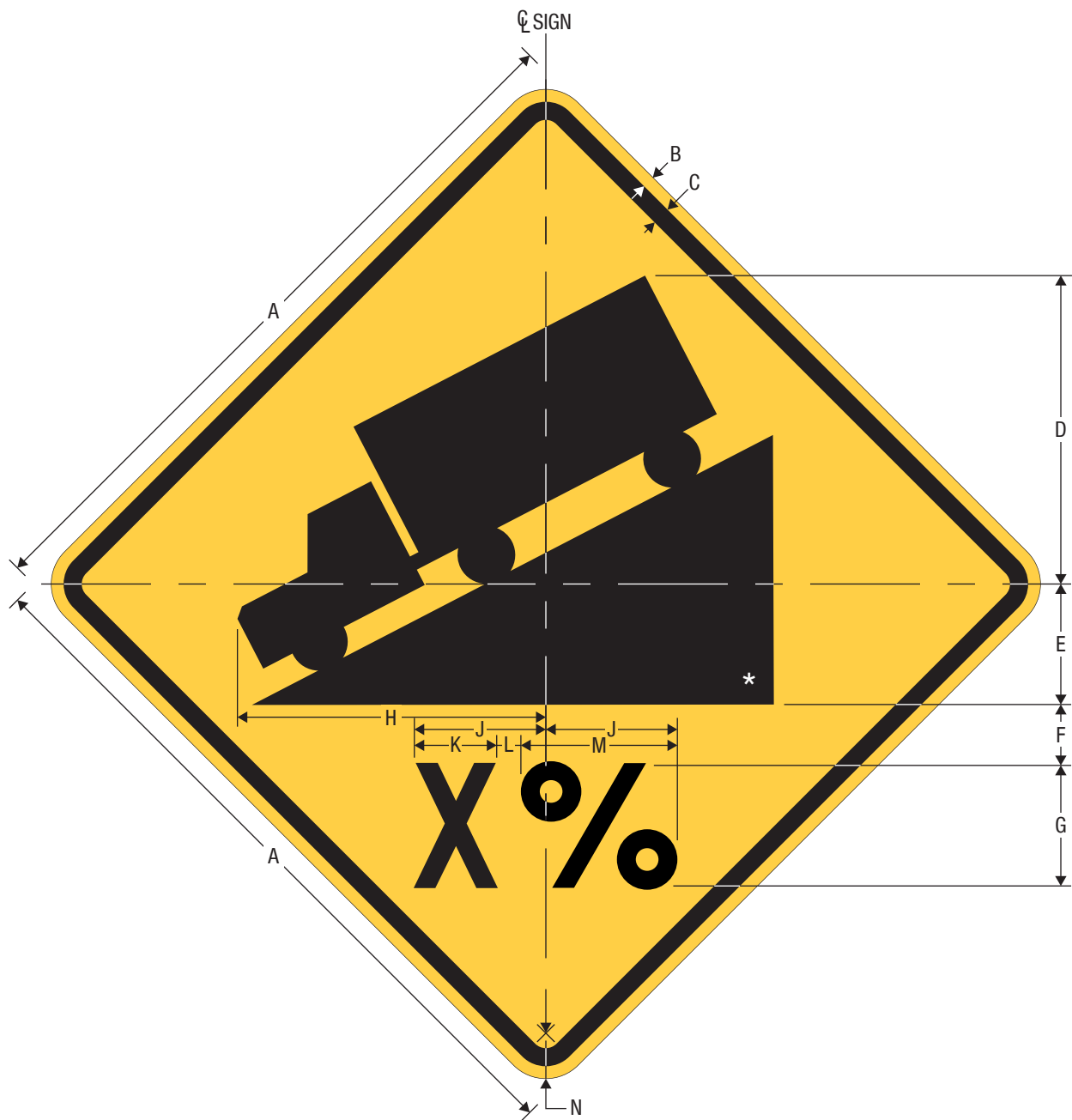
W7-1a Hill with Grade
