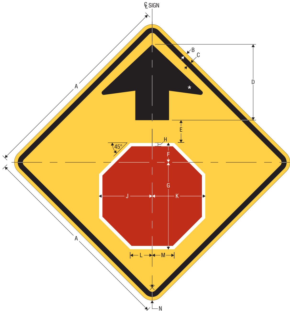
W3-1 Stop Ahead
