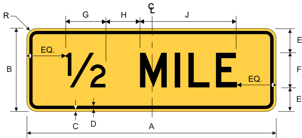
W16-3aP [1] [Distance Plaque] XX MILES (1-Line Plaque)
