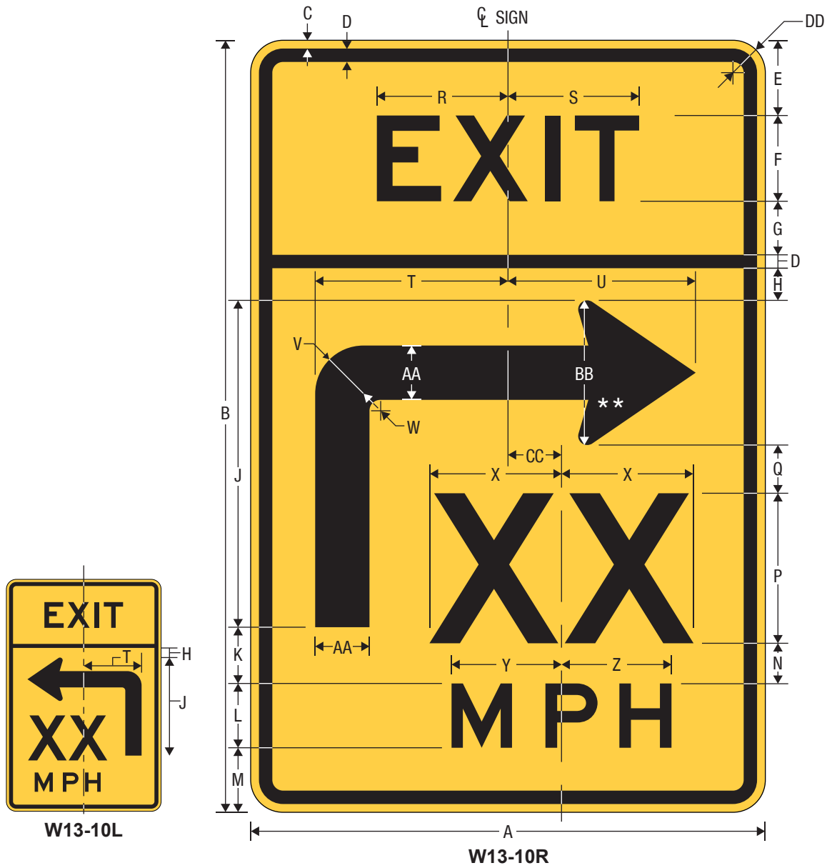
Combination Horizontal Alignment / Advisory Exit Speed - Turn
