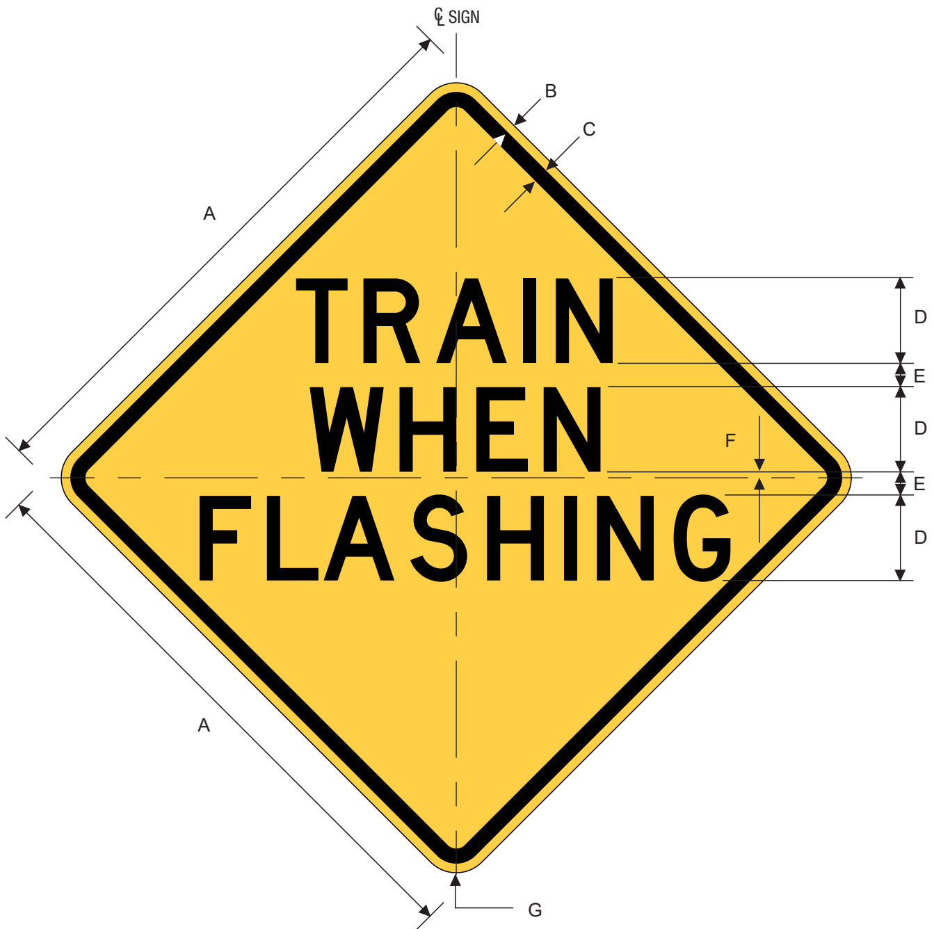
W10-17T TRAIN WHEN FLASHING
