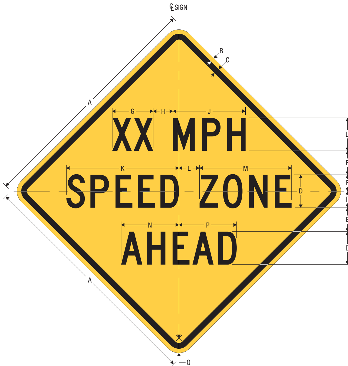
W3-5a XX MPH SPEED ZONE AHEAD
