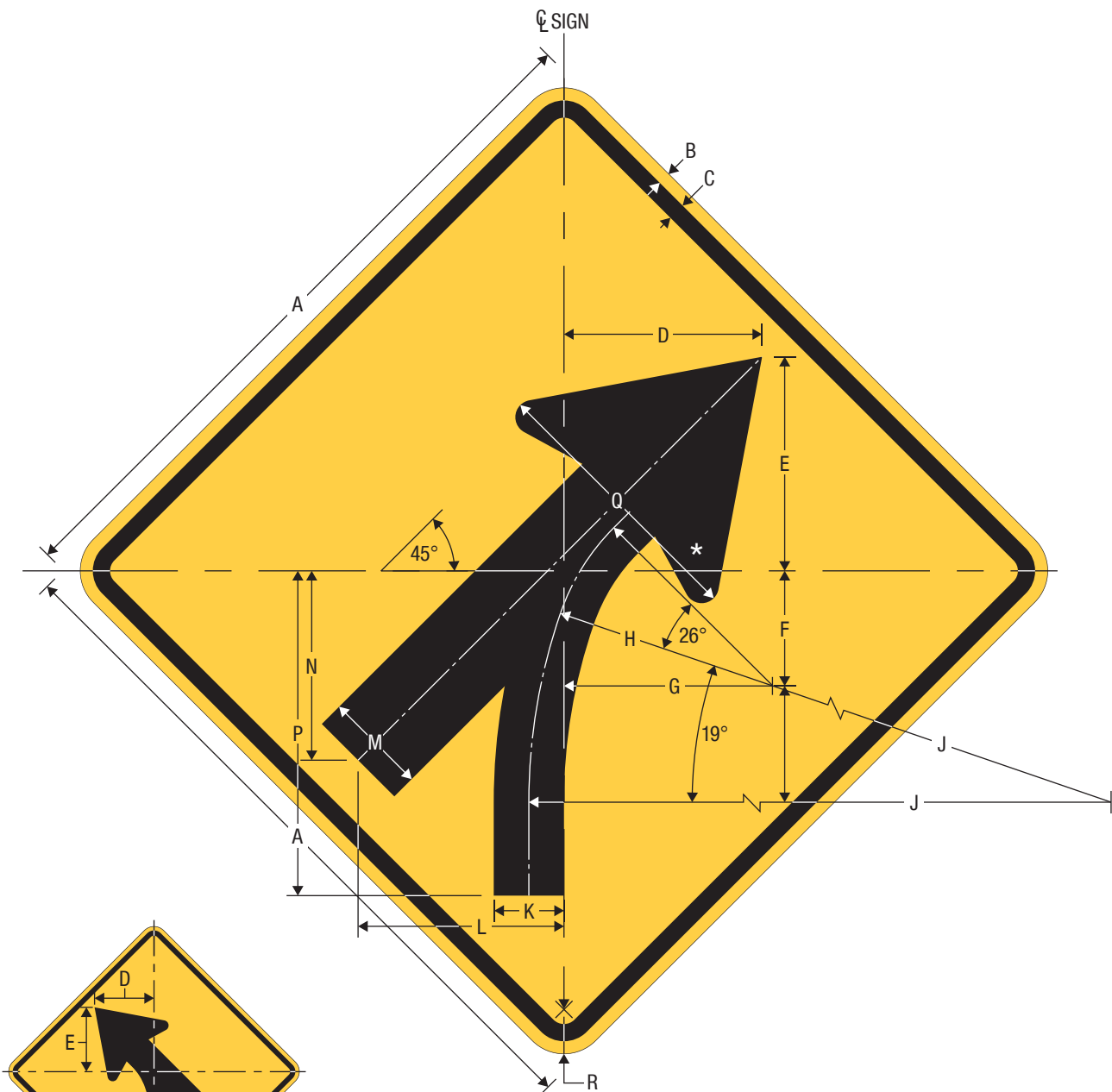
W4-5R Entering Roadway Merge
