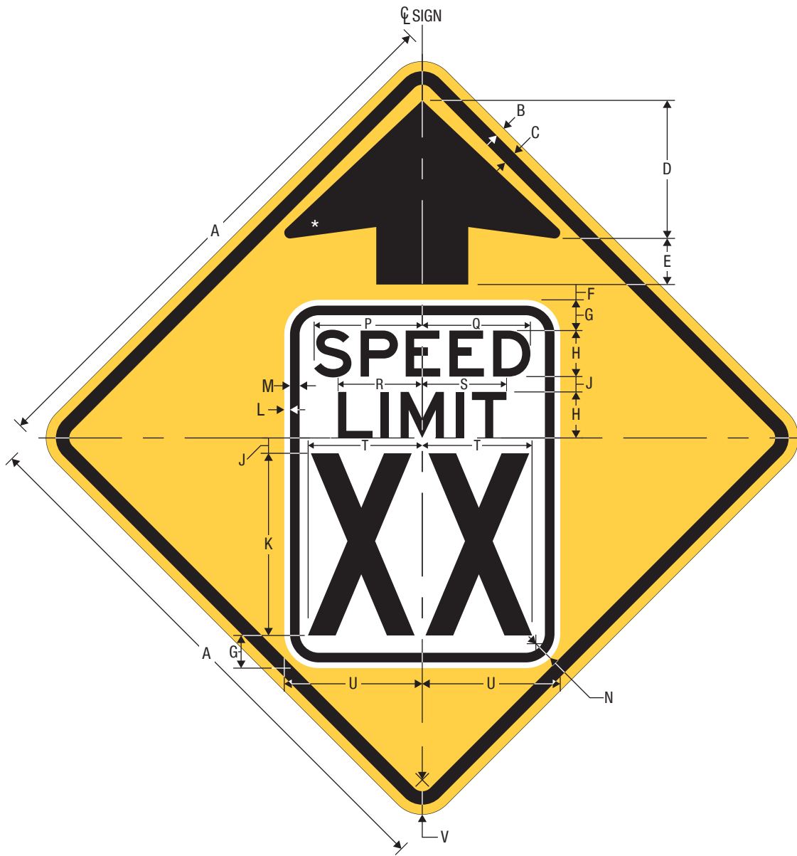
W3-5 Reduced Speed Limit Ahead
