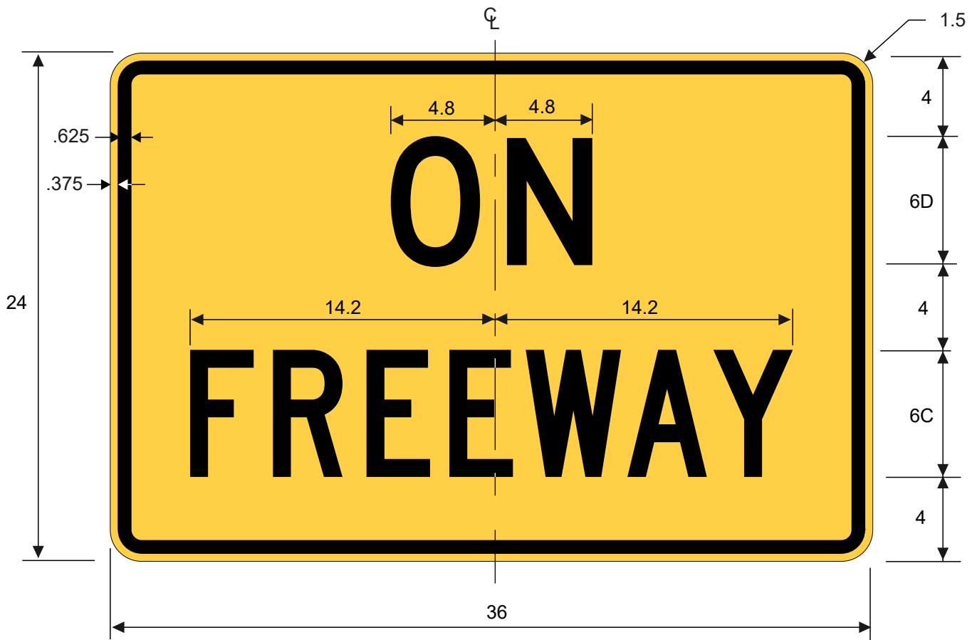
W13-4bPT ON FREEWAY (Plaque)
