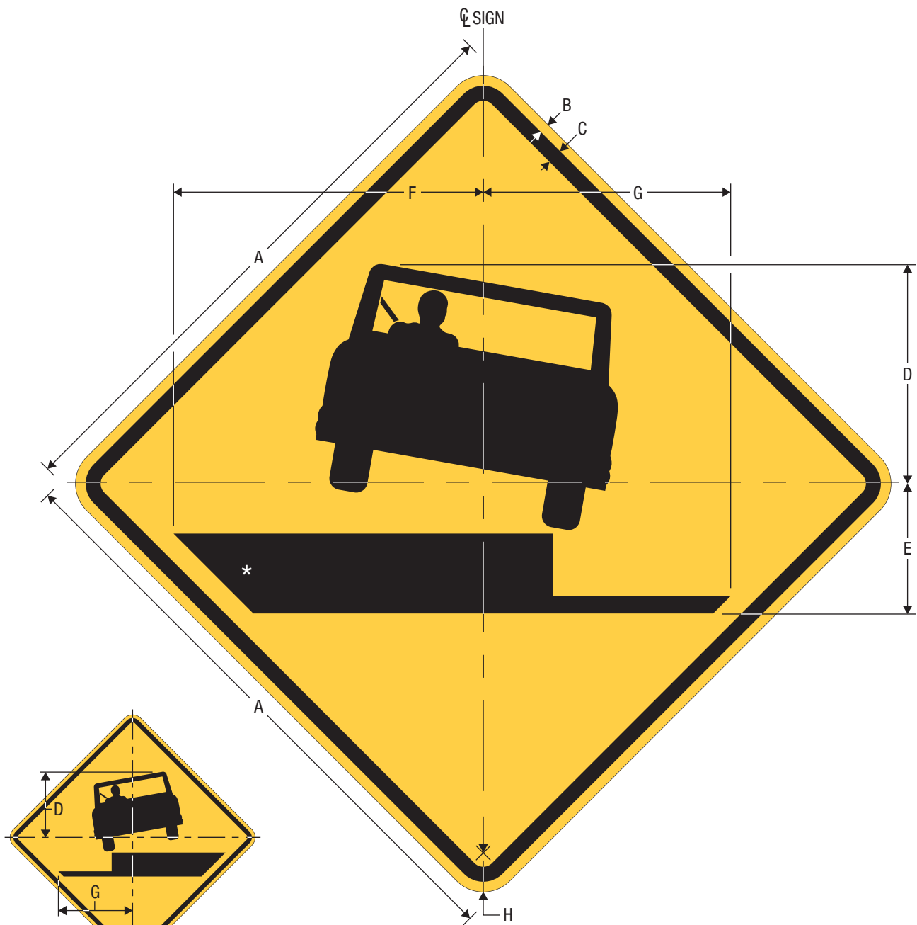
W8-17R Shoulder Drop Off
