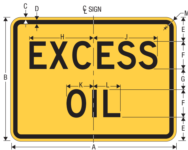
W8-5cP EXCESS OIL (Plaque)
