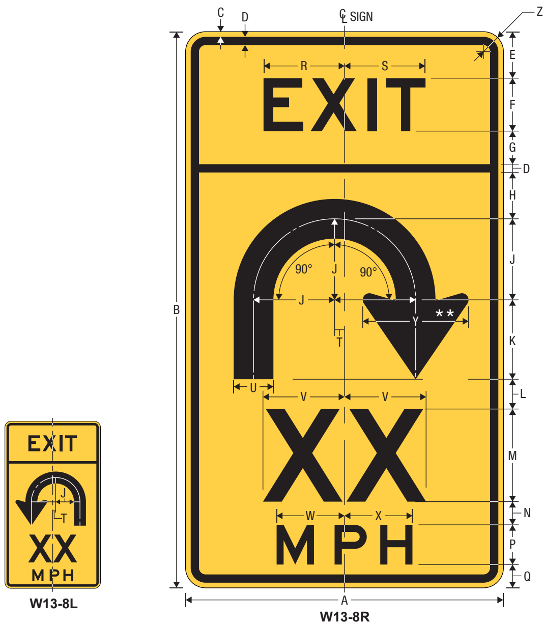
Combination Horizontal Alignment / Advisory Exit Speed - 180-Degree Loop
