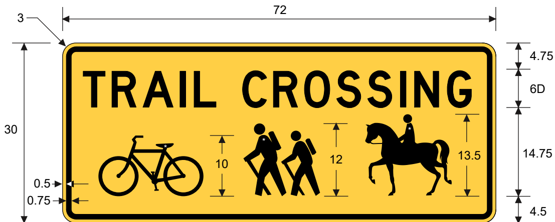
W11-15bT TRAIL CROSSING (with combined symbols)
