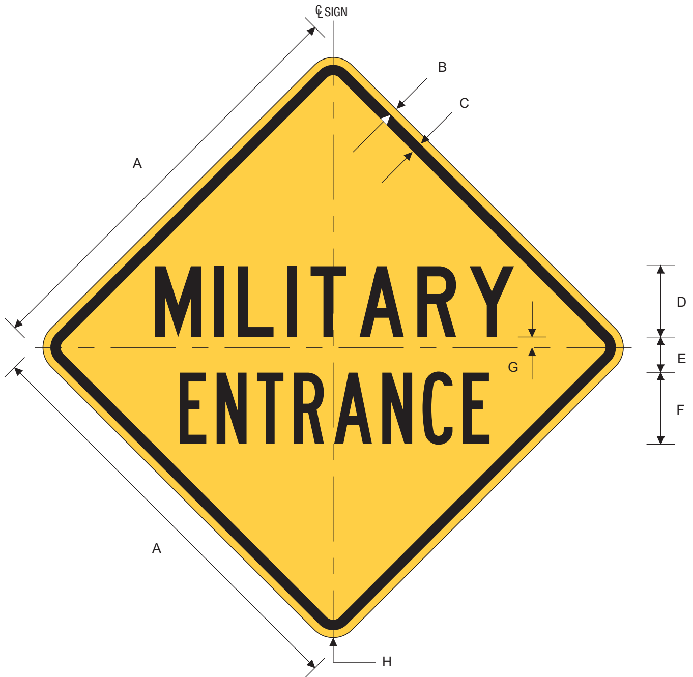
W17-6T MILITARY ENTRANCE
