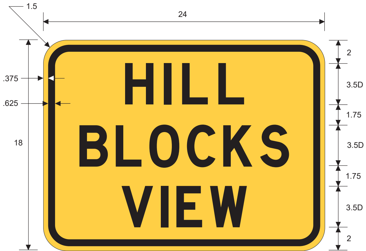
W7-6PT HILL BLOCKS VIEW (Plaque)
