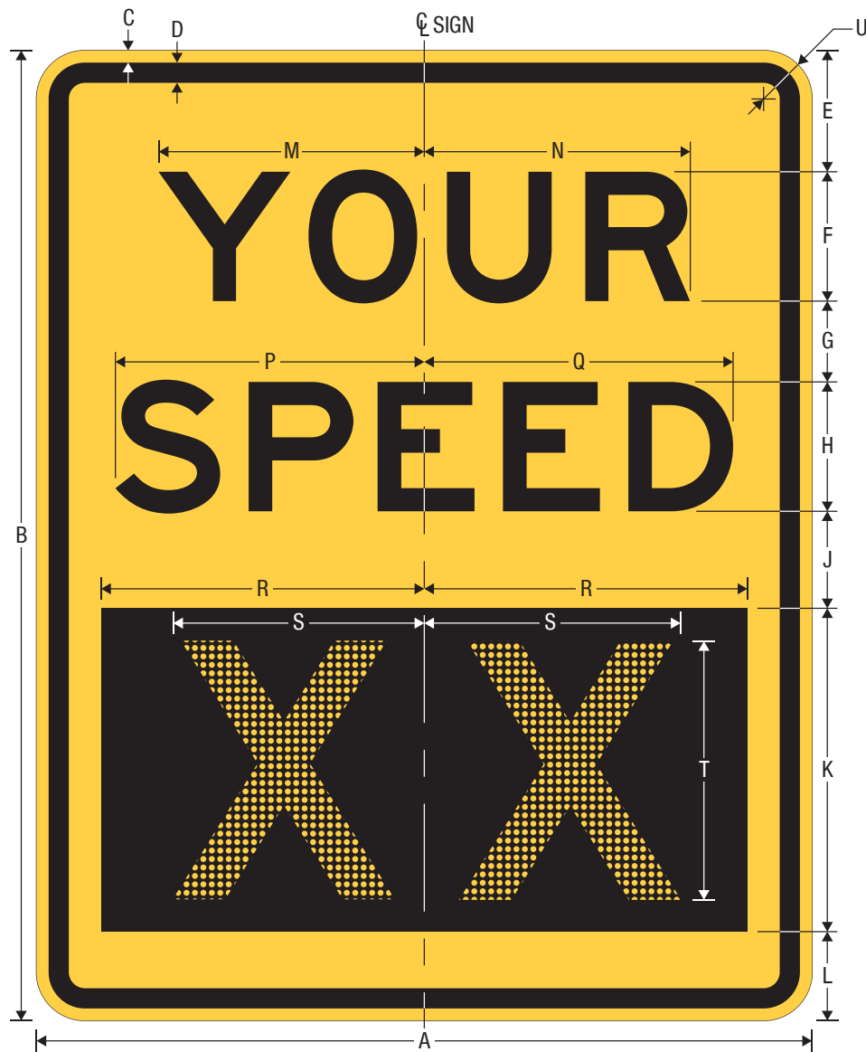
W13-20 Vehicle Speed Feedback
