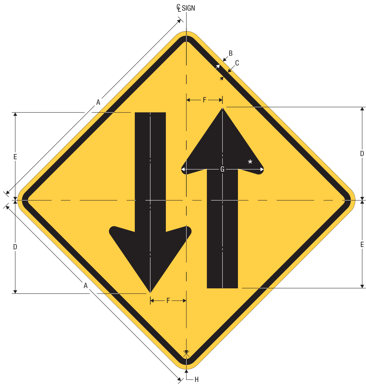
W6-3 Two-Way Traffic
