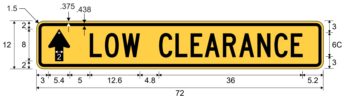
W12-3PTS LOW CLEARANCE (Plaque)
