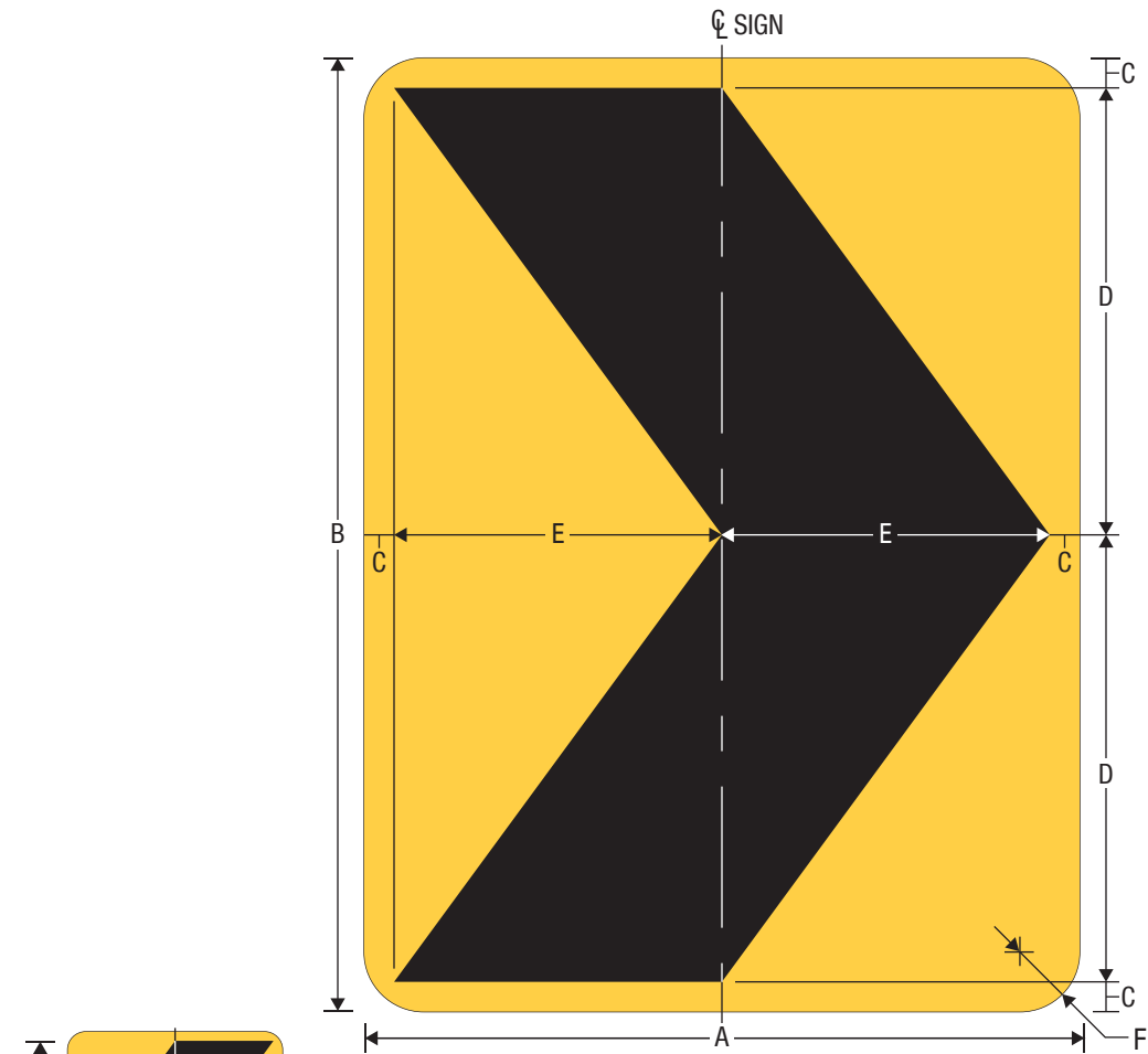
W1-8R Chevron Alignment
