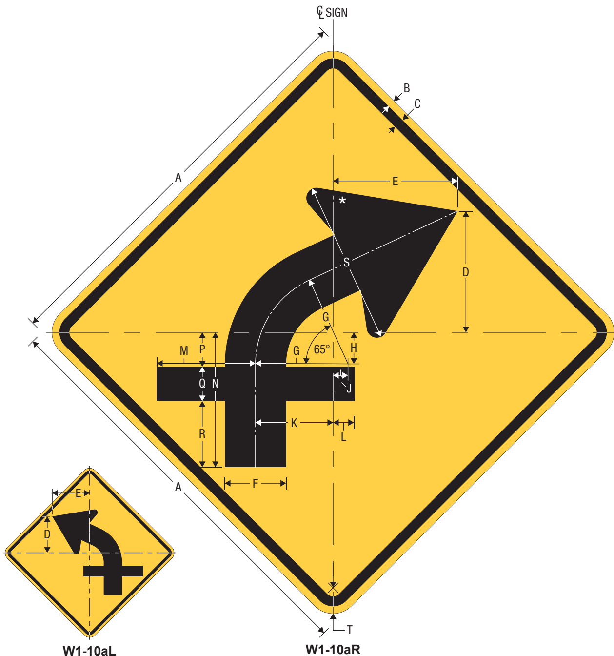
Combination Horizontal Alignment/Intersection
