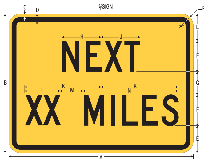
W7-3aP NEXT XX MILES (Plaque)
