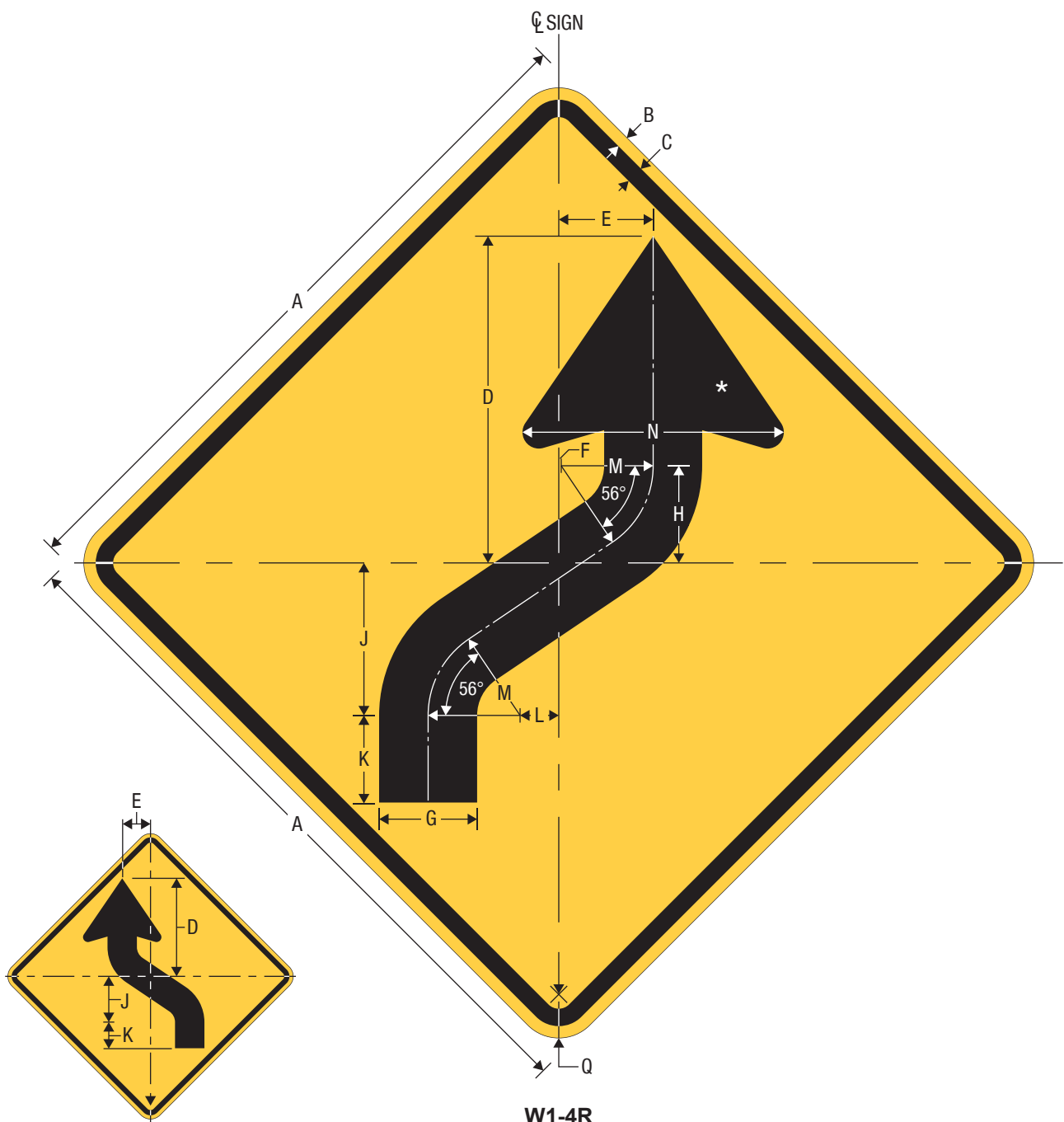
Horizontal Alignment - Reverse Curve
