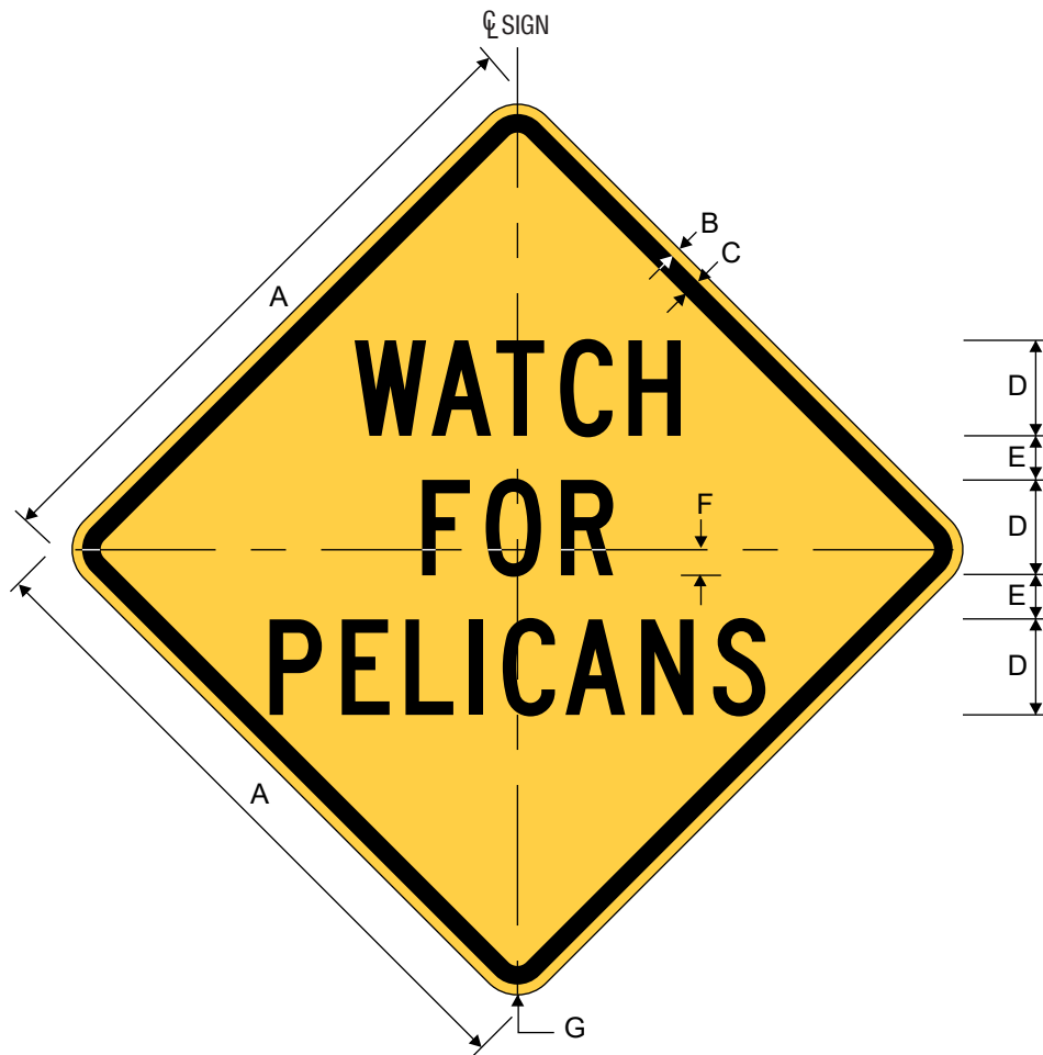
W11-26aT WATCH FOR PELICANS
