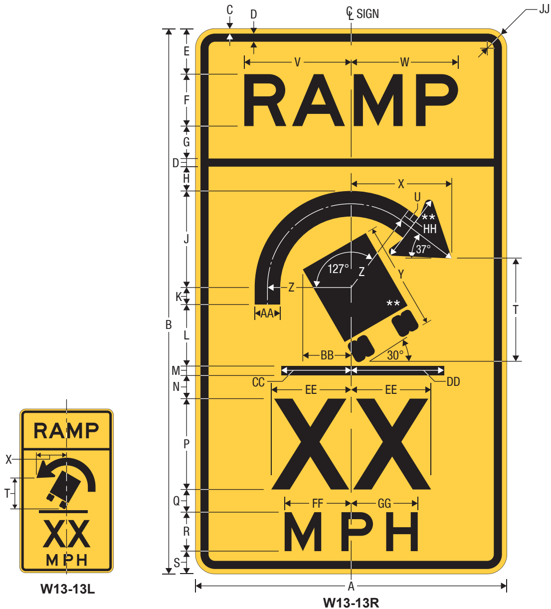
Combination Horizontal Alignment / Advisory Ramp Speed-Truck Rollover
