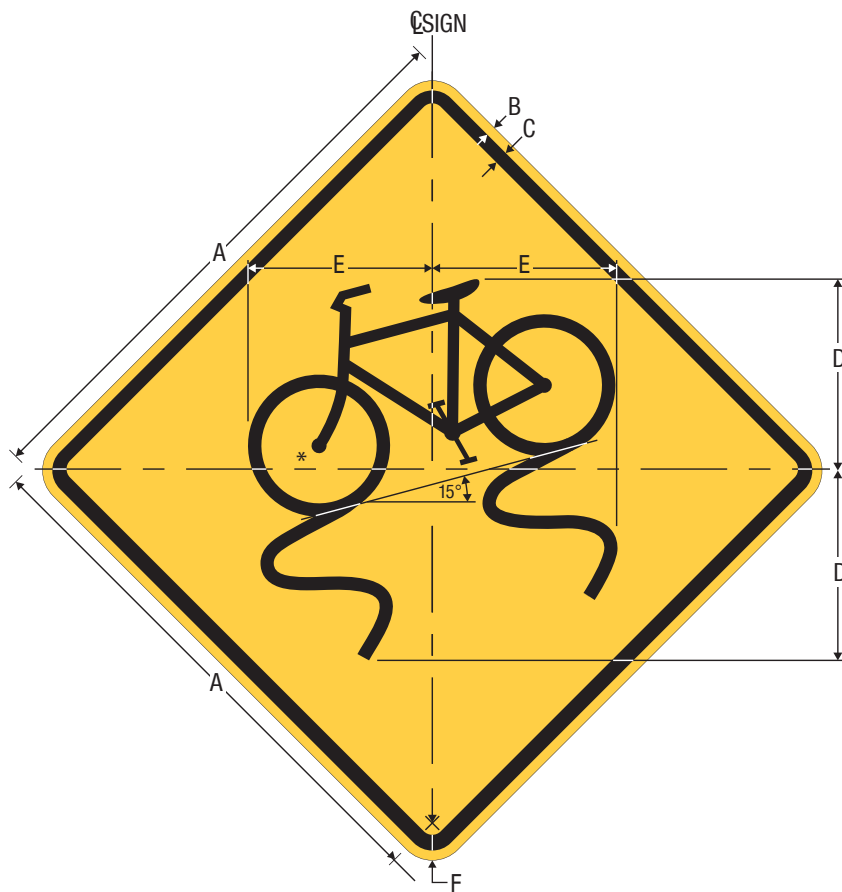
W8-10 Bicycle Surface Condition
