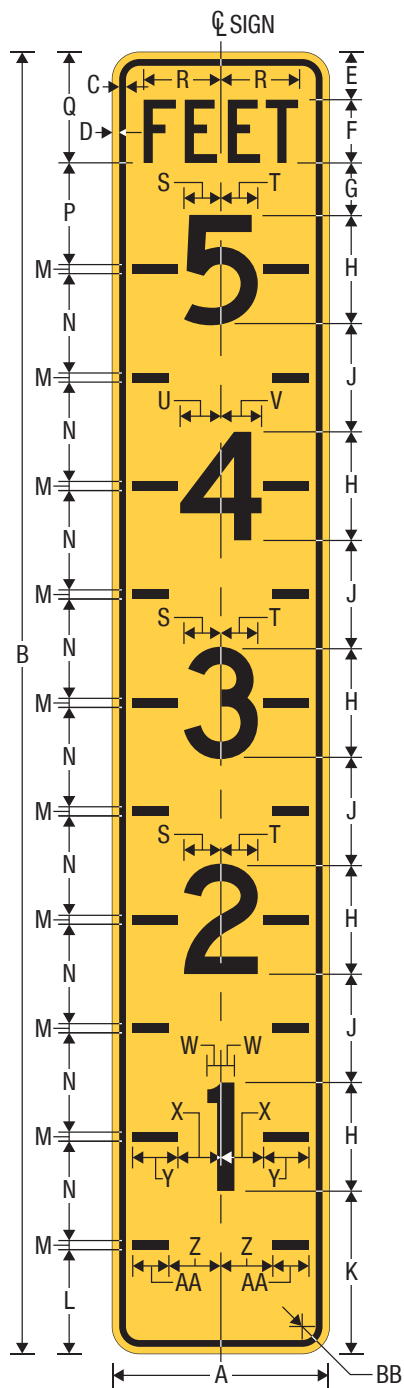
W8-19 Depth [Flood] Gauge
