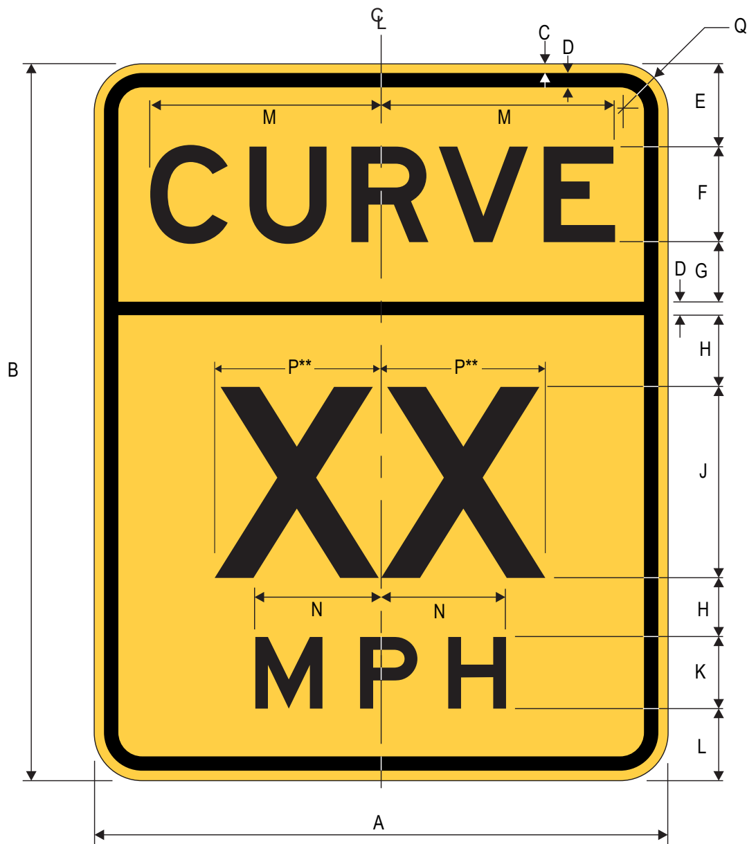
W13-5T CURVE Advisory Speed
