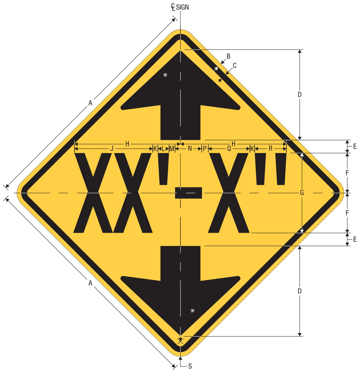
W12-2 Clearance Advance
