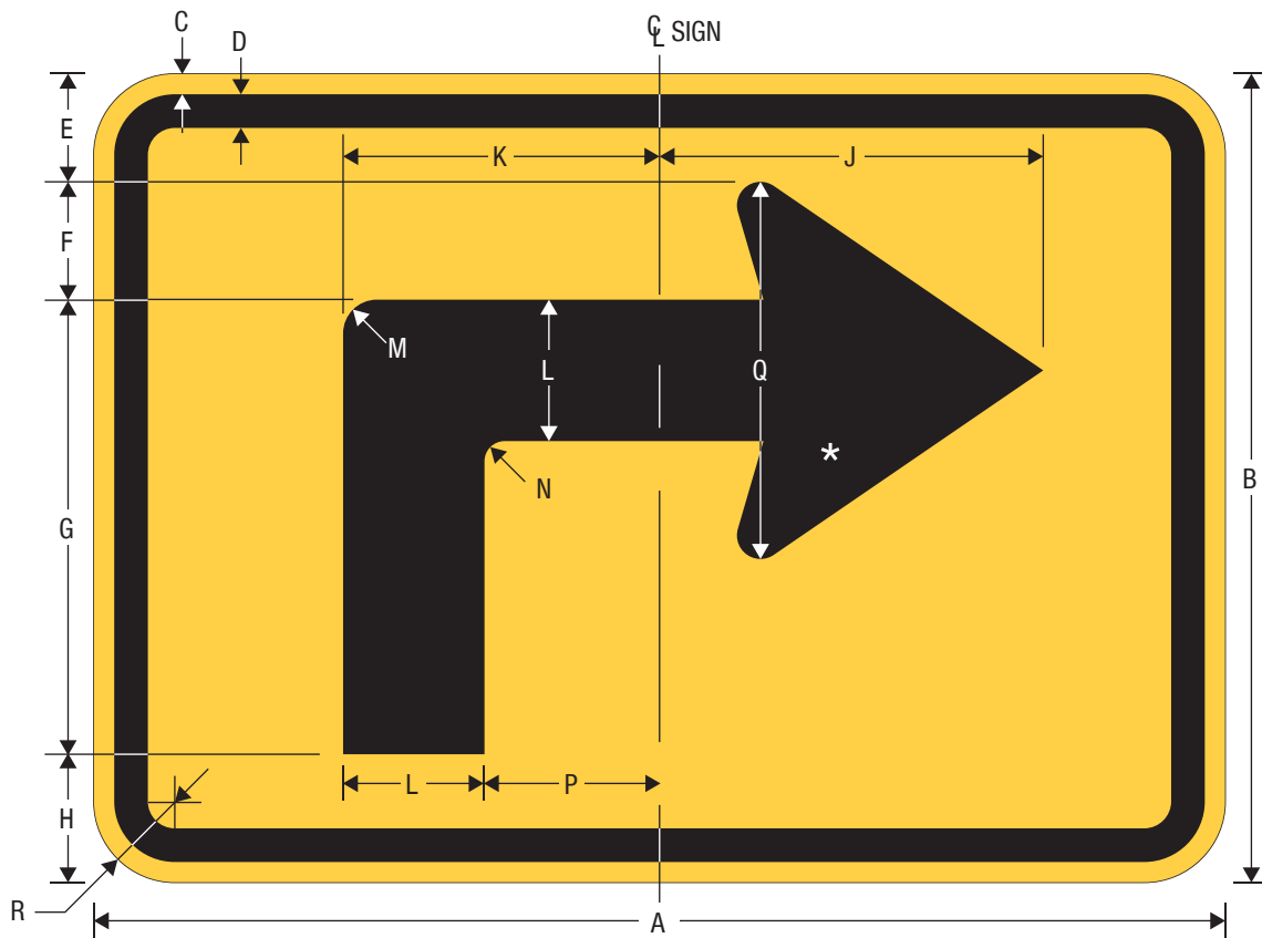
W16-6PR Advance Turn Arrow (Plaque)
