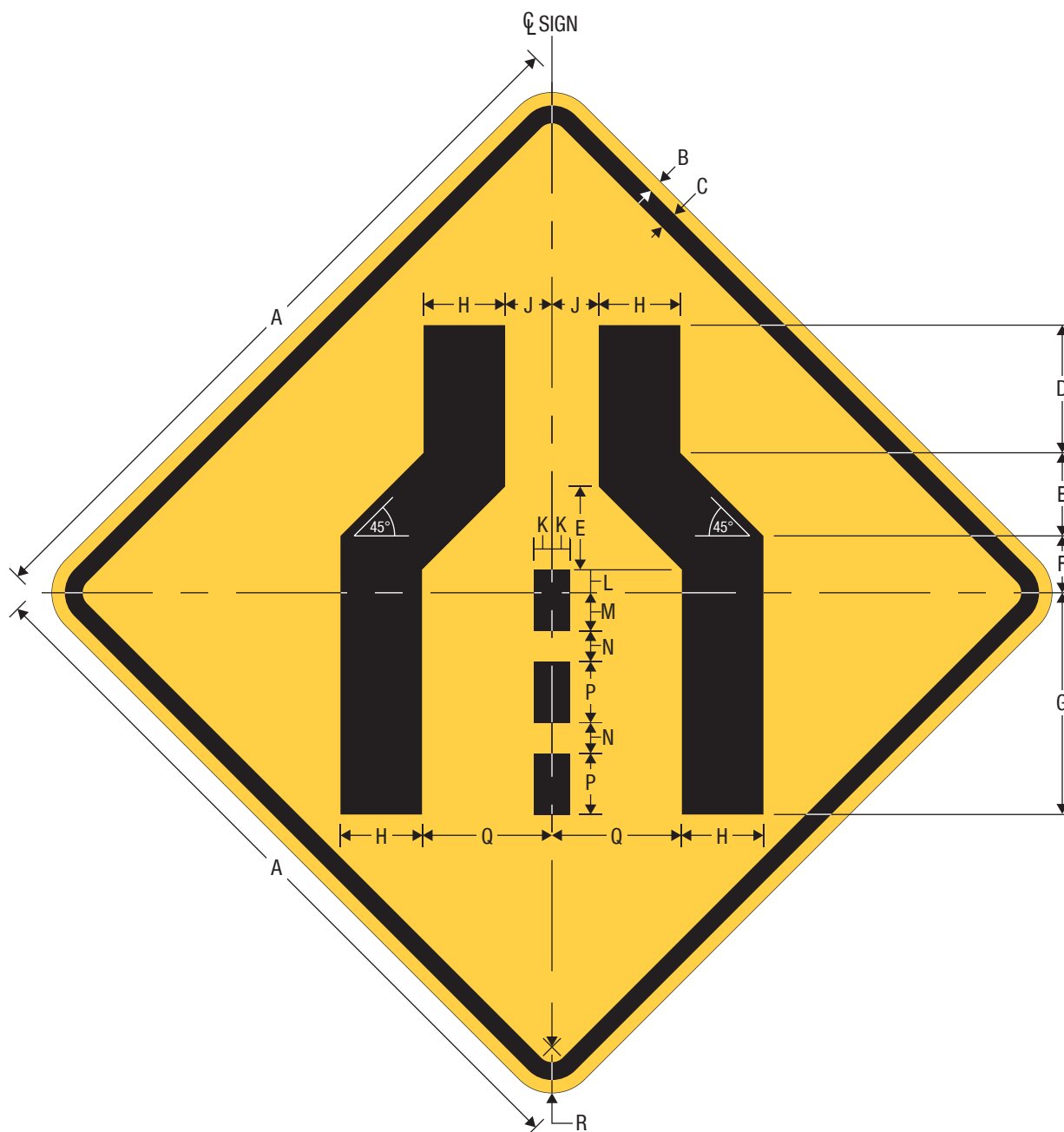
W4-8 Single-Lane Transition
