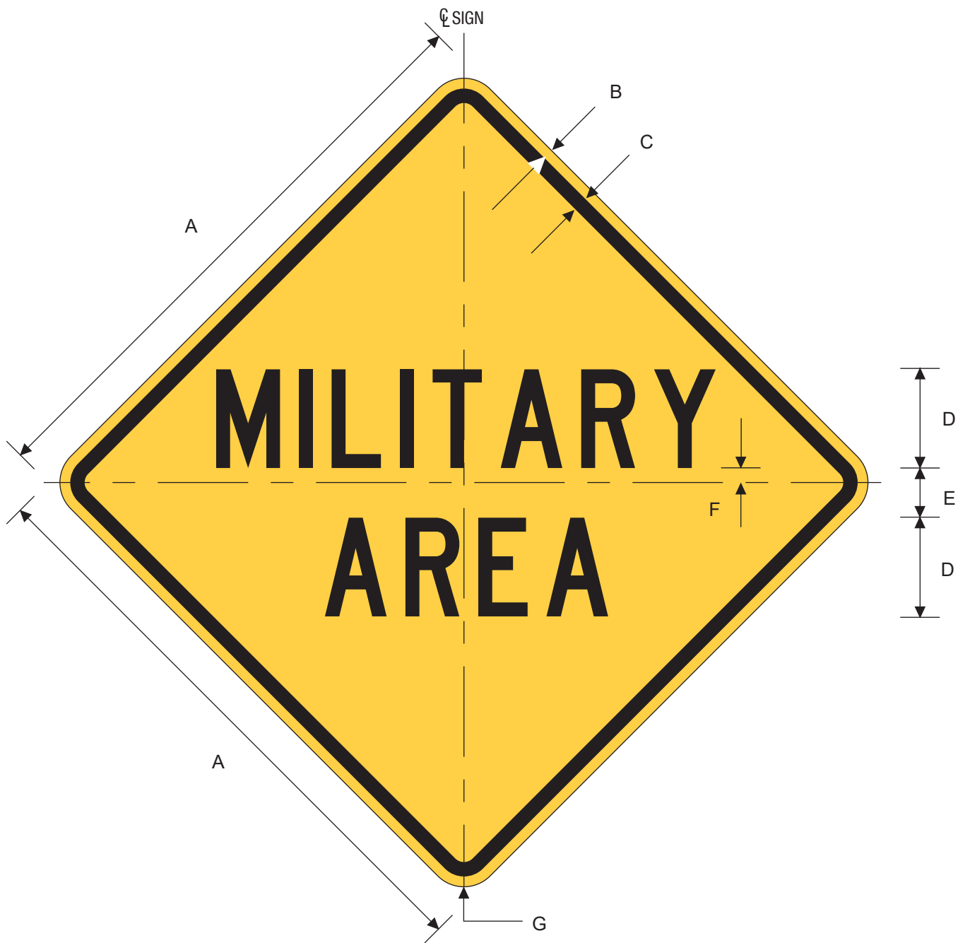
W17-7T MILITARY AREA
