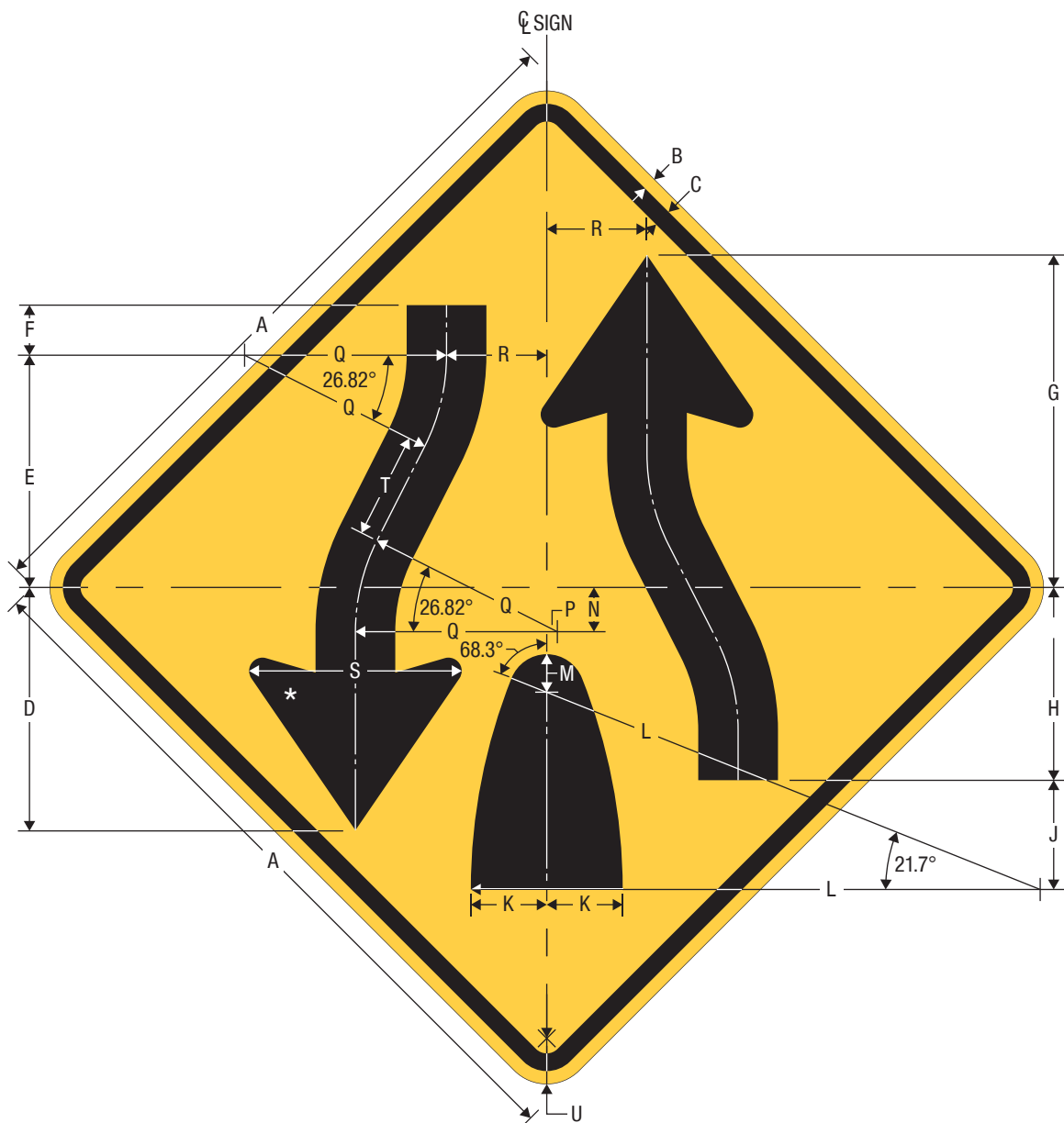
W6-2 Divided Highway Ends
