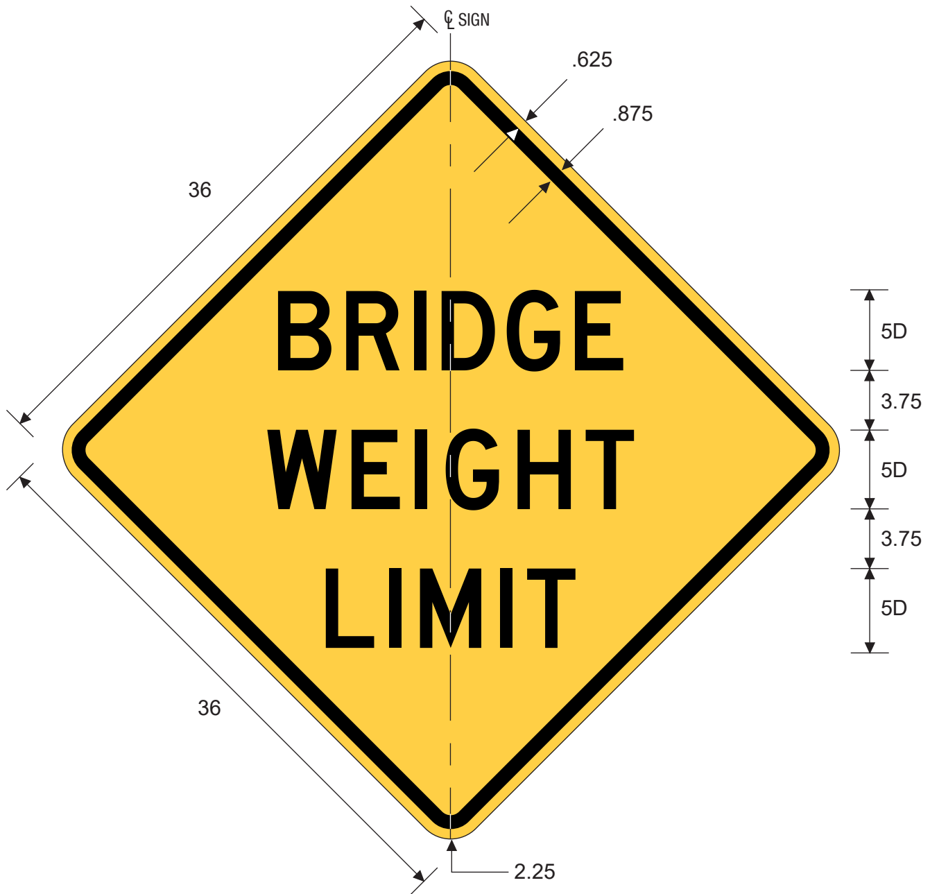
W12-5T BRIDGE WEIGHT LIMIT
