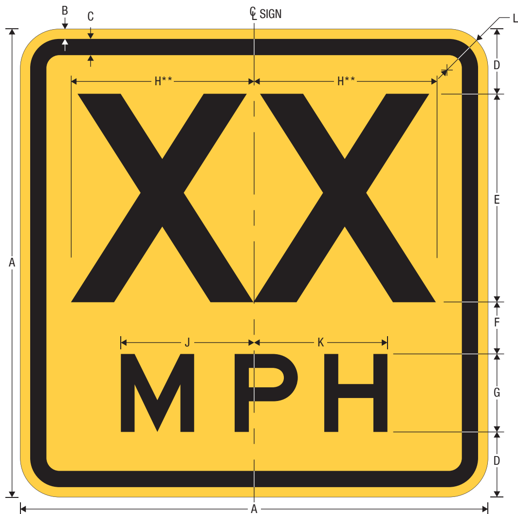
W13-1P Advisory Speed (Plaque)
