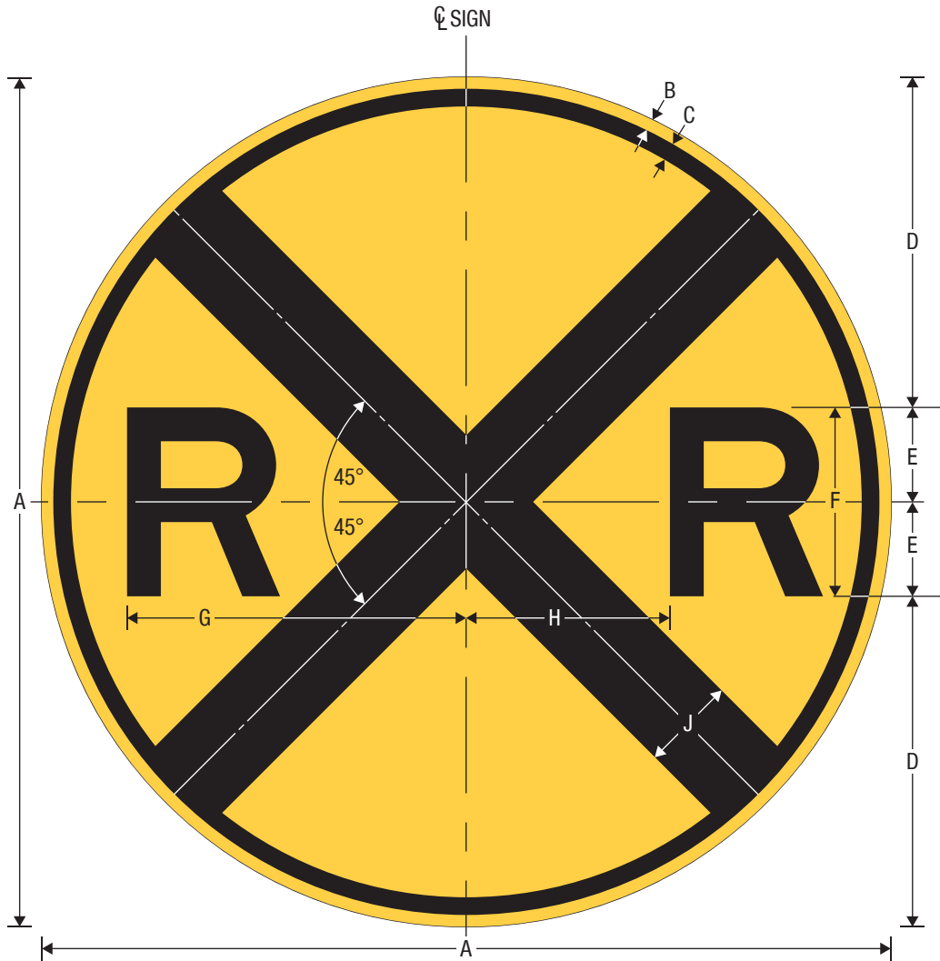
W10-1 Grade Crossing Advance Warning
