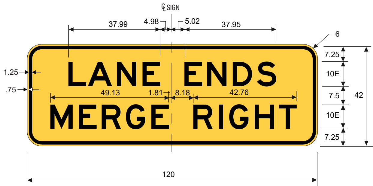
W9-5TR LANE ENDS MERGE RIGHT
