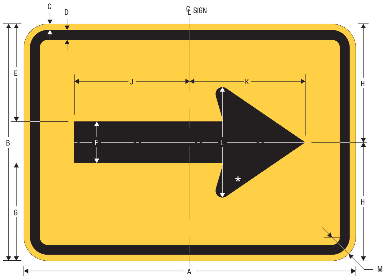
W16-5PR Directional Arrow (Plaque)
