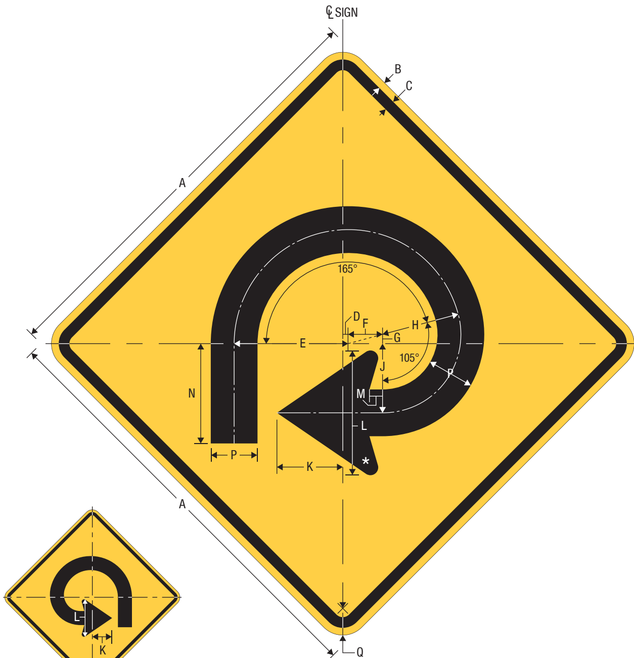
W1-15R 270-Degree Curve
