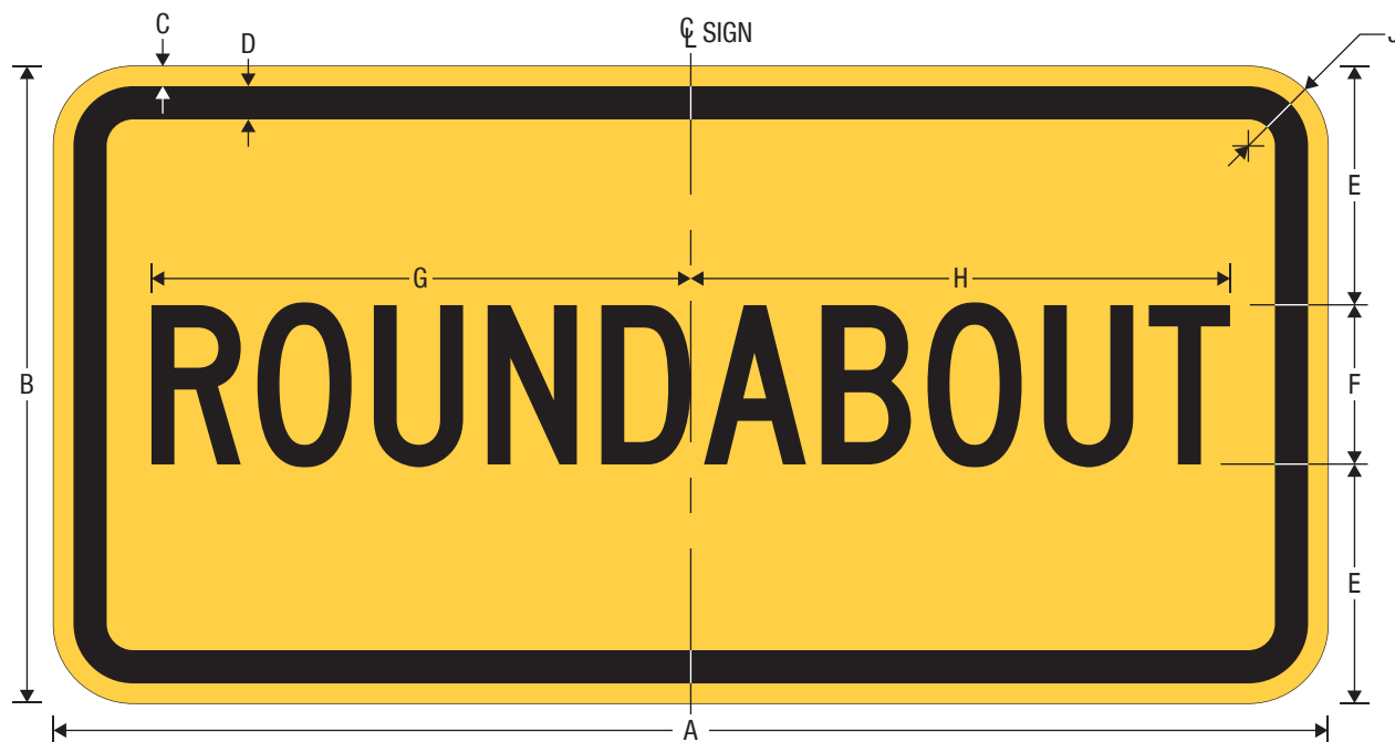
W16-12aP ROUNDABOUT (Plaque)
