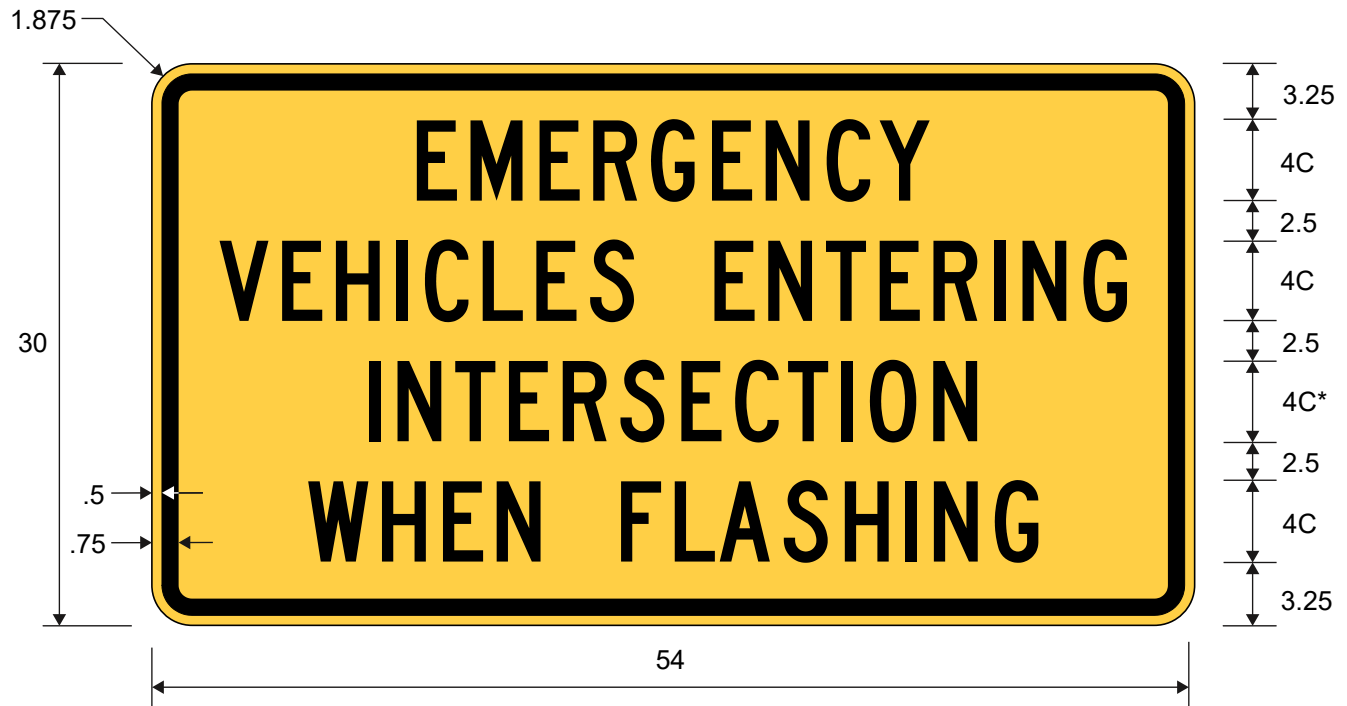
W11-12aT EMERGENCY VEHICLES ENTERING INTERSECTION WHEN FLASHING
