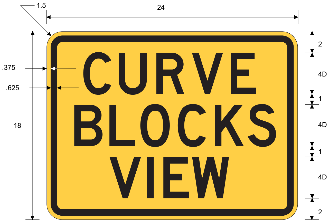
W1-11PT CURVE BLOCKS VIEW (Plaque)
