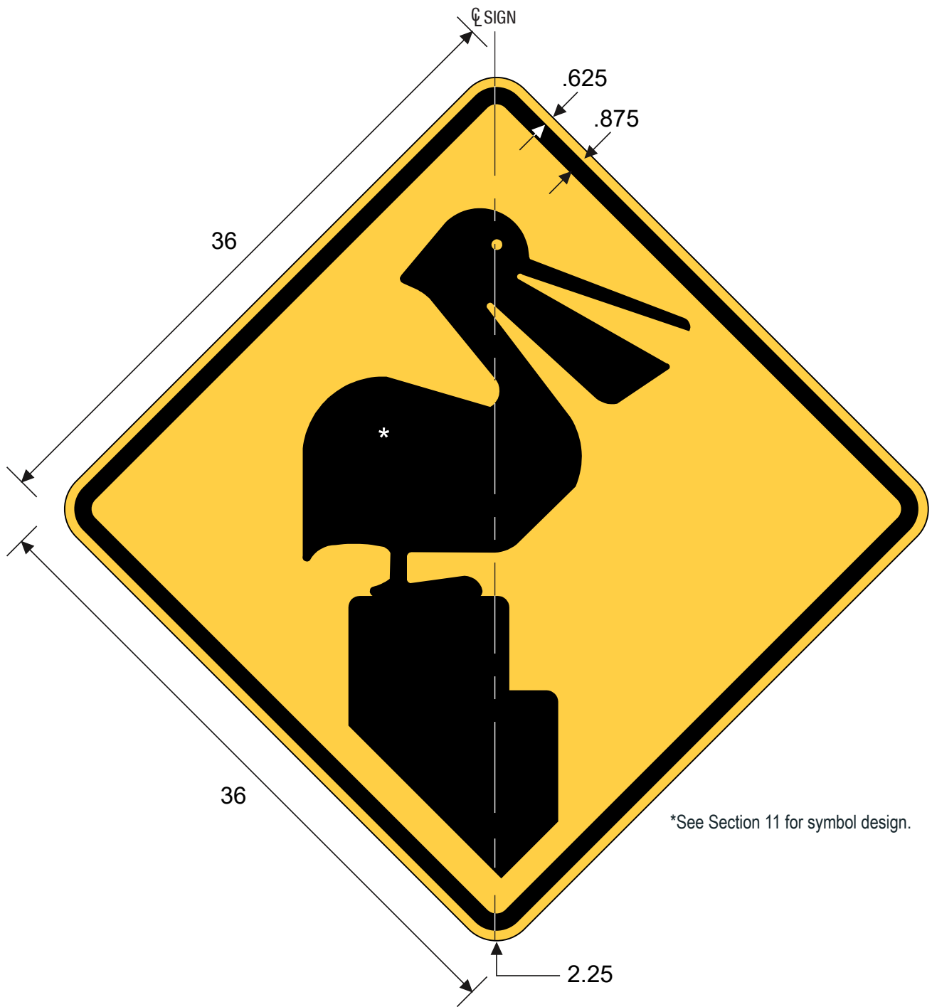
W11-26T Pelican (Symbol)
