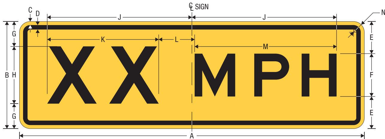
W13-1aP Confirmation Advisory Speed (Plaque)
