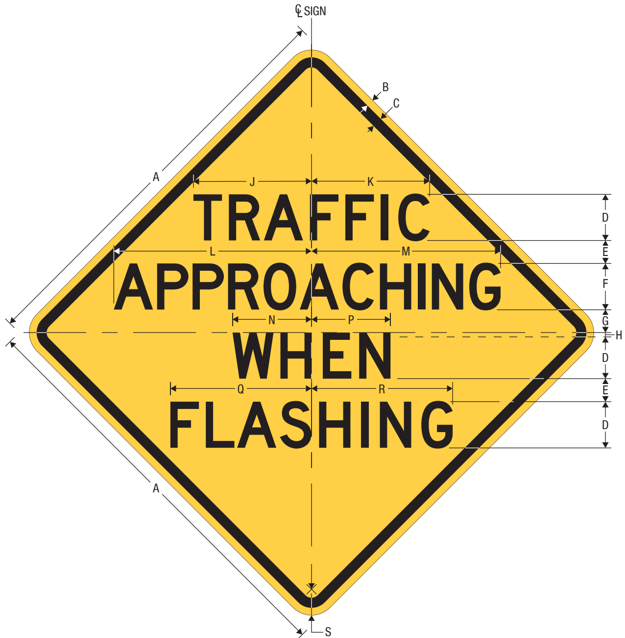
W2-11 TRAFFIC APPROACHING WHEN FLASHING
