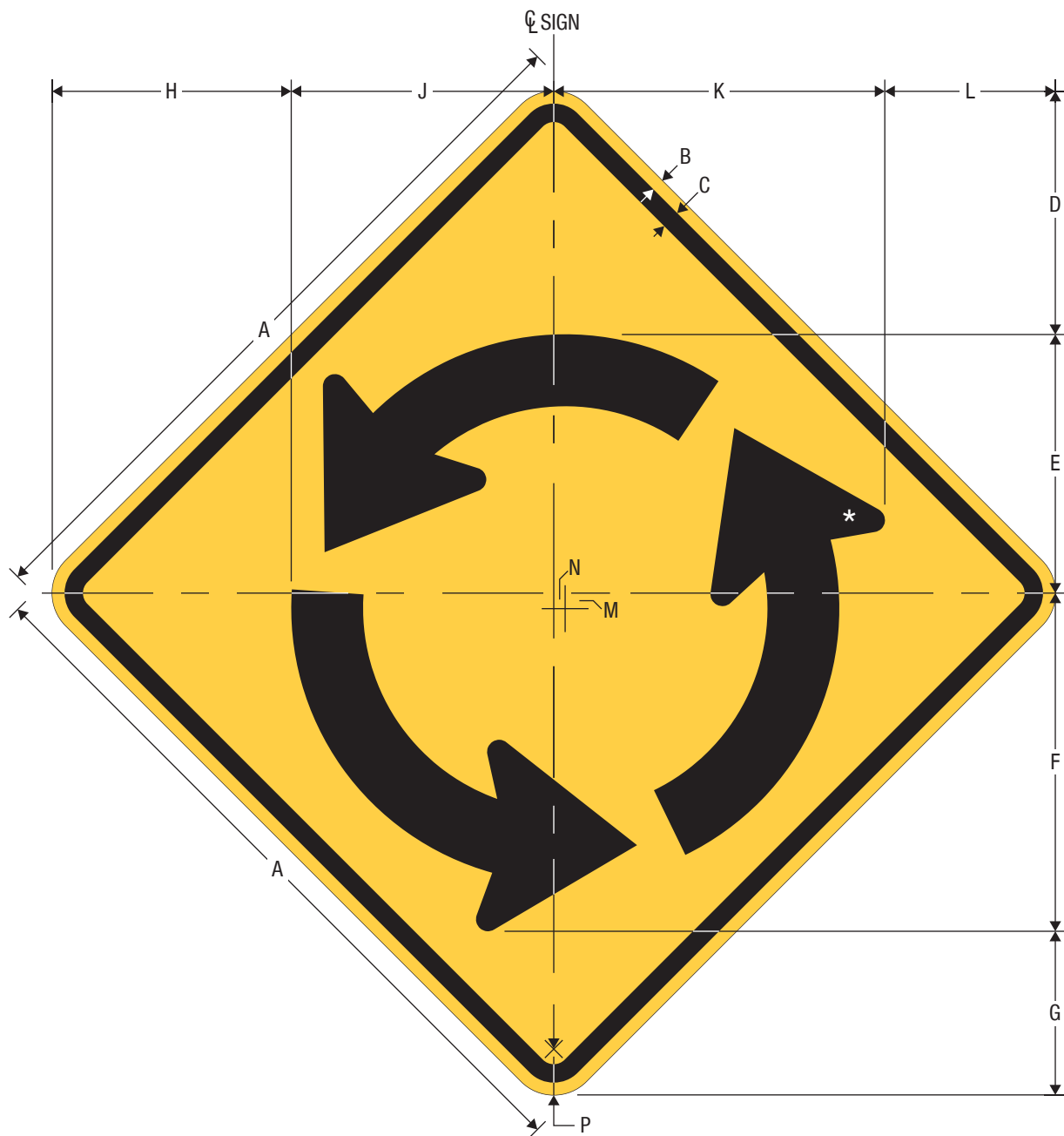
W2-6 Intersection Warning - Circular
