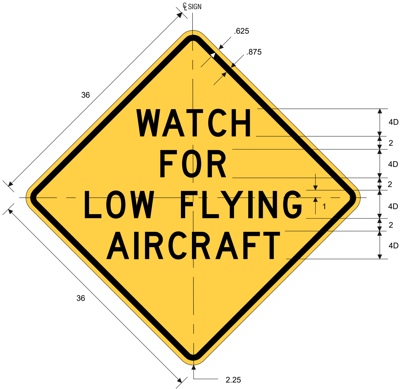
W17-10T WATCH FOR LOW FLYING AIRCRAFT
