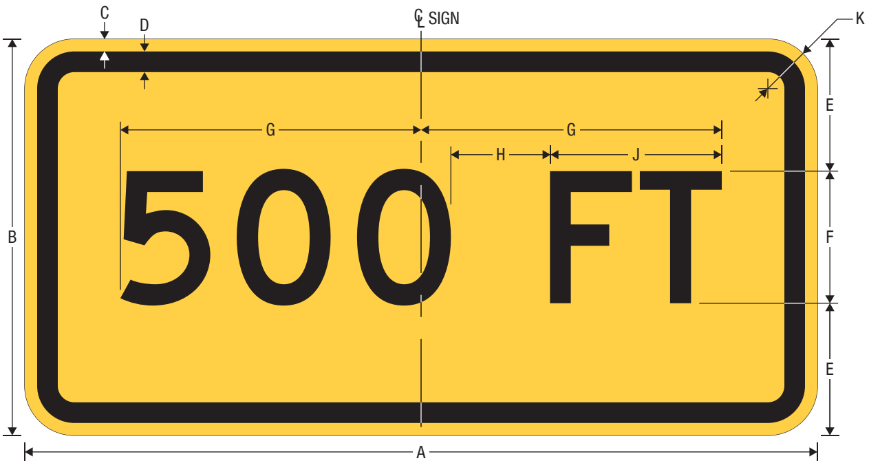
W16-2aP [Distance Plaque] XX FT (1-Line Plaque)
