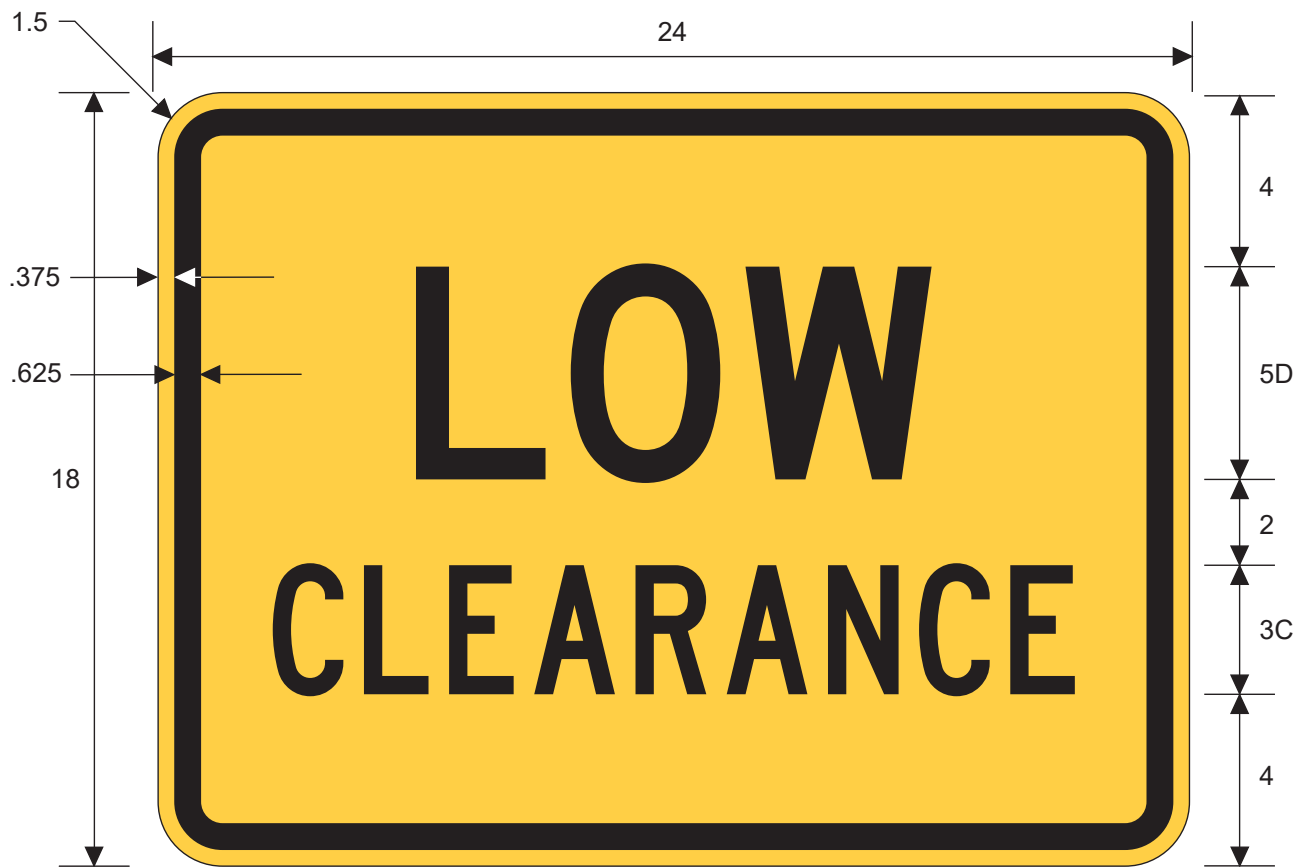
W12-2PT LOW CLEARANCE (Plaque)
