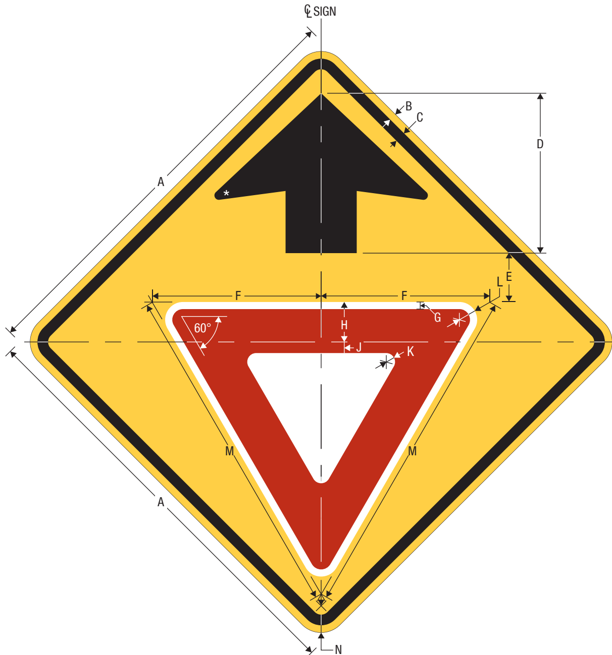
W3-2 Yield Ahead
