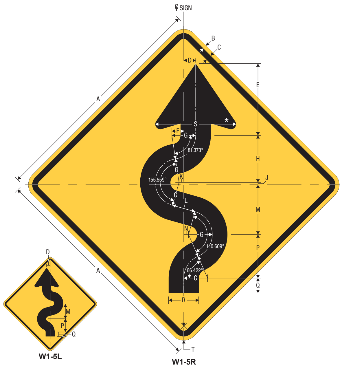
Horizontal Alignment - Winding Road
