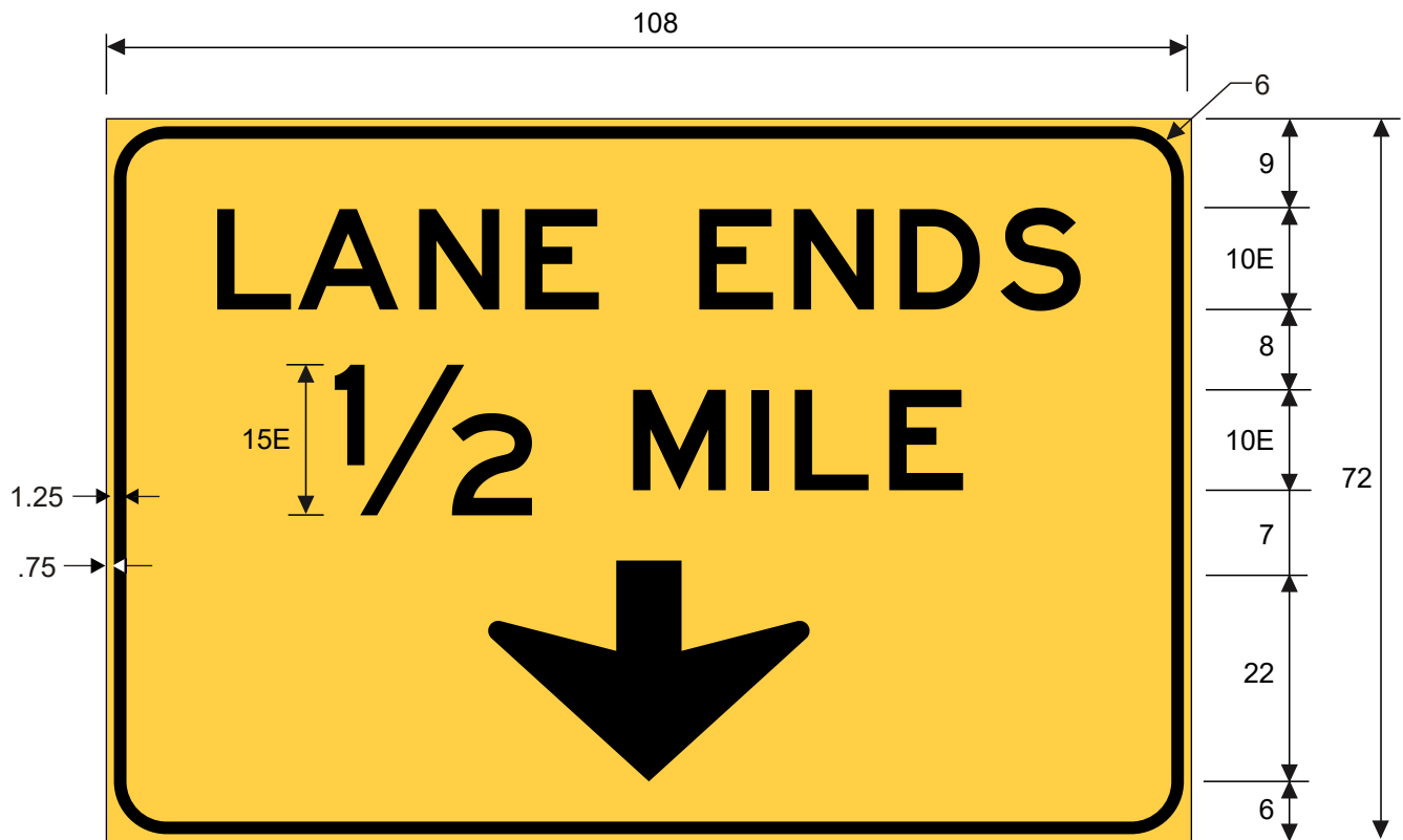
W9-1aT LANE ENDS 1/2 MILE
