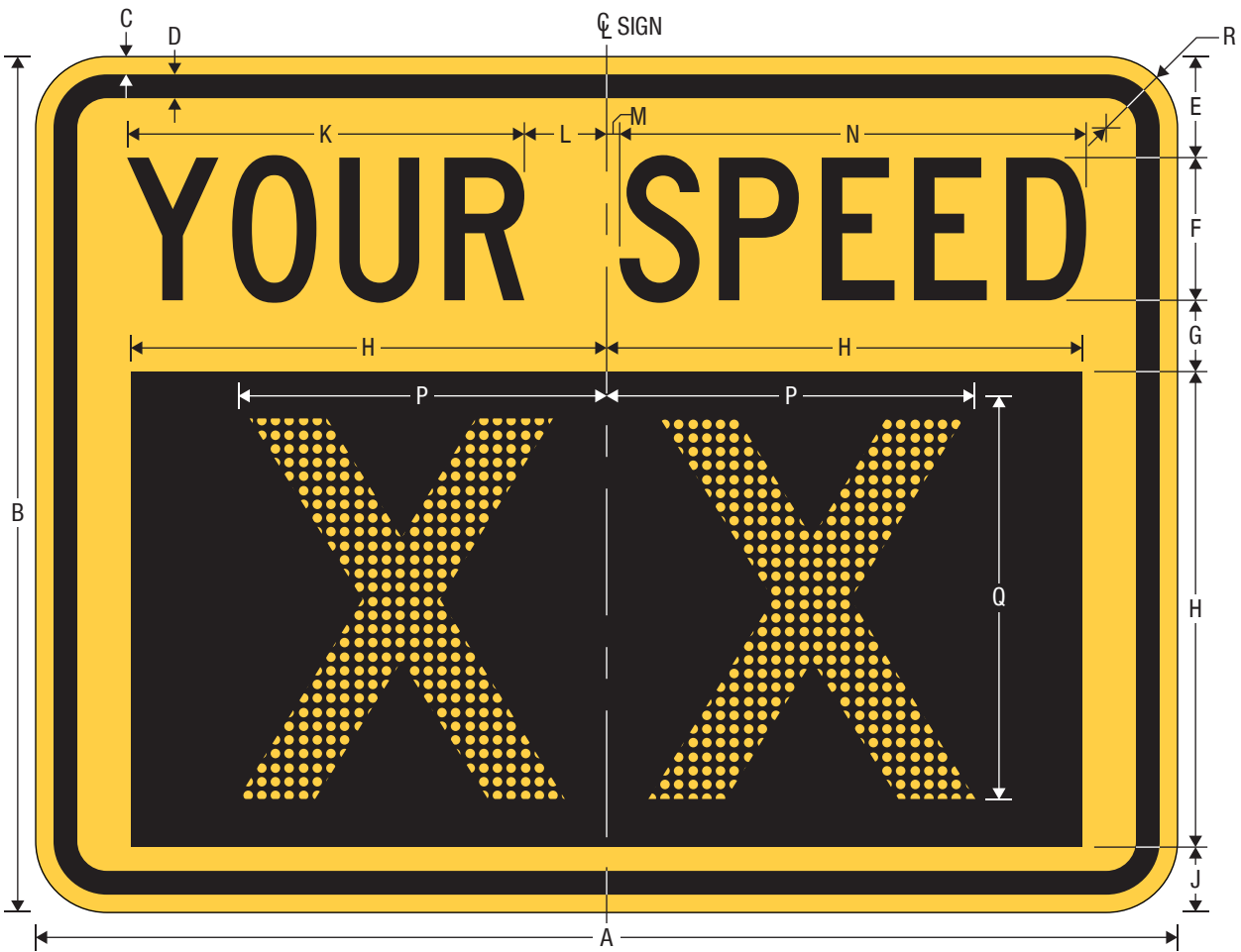
W13-20aP Vehicle Speed Feedback (Plaque)
