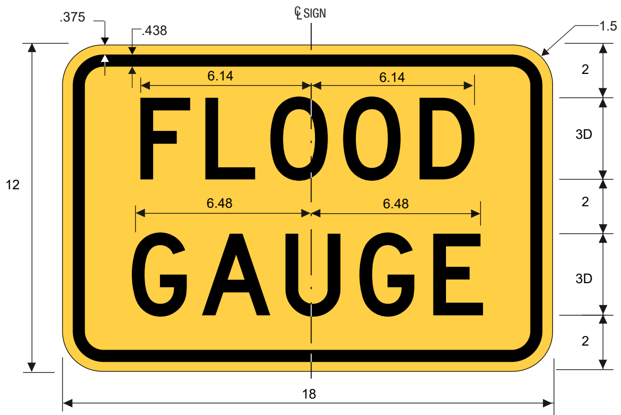
W8-19aPT FLOOD GAUGE (Plaque)
