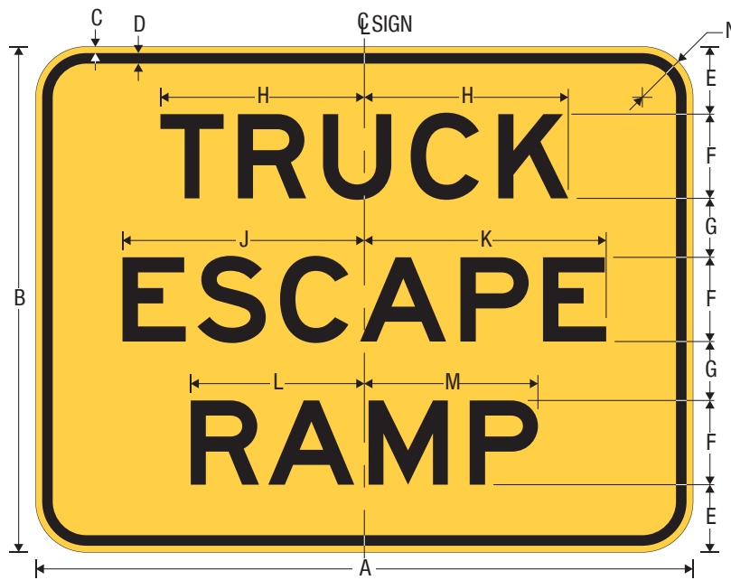
W7-4c TRUCK ESCAPE RAMP
