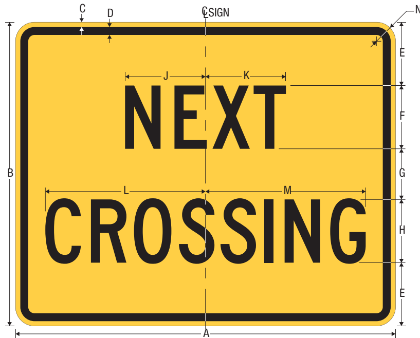
W10-14P NEXT CROSSING (Plaque)
