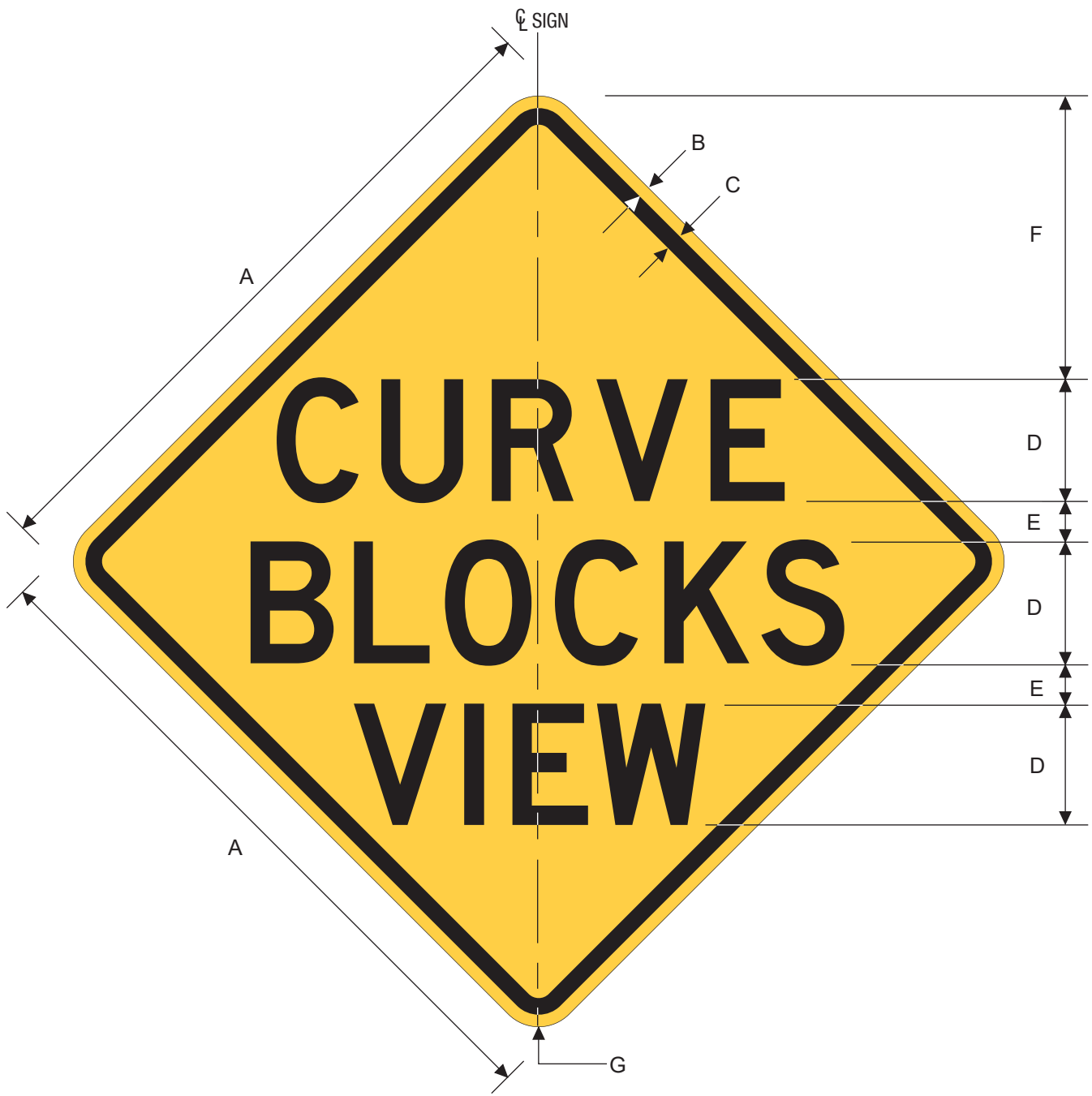
W1-11T CURVE BLOCKS VIEW
