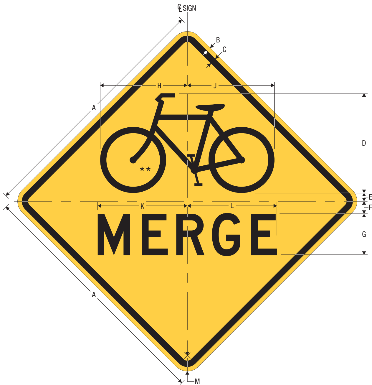
W9-5a Bicycles MERGE
