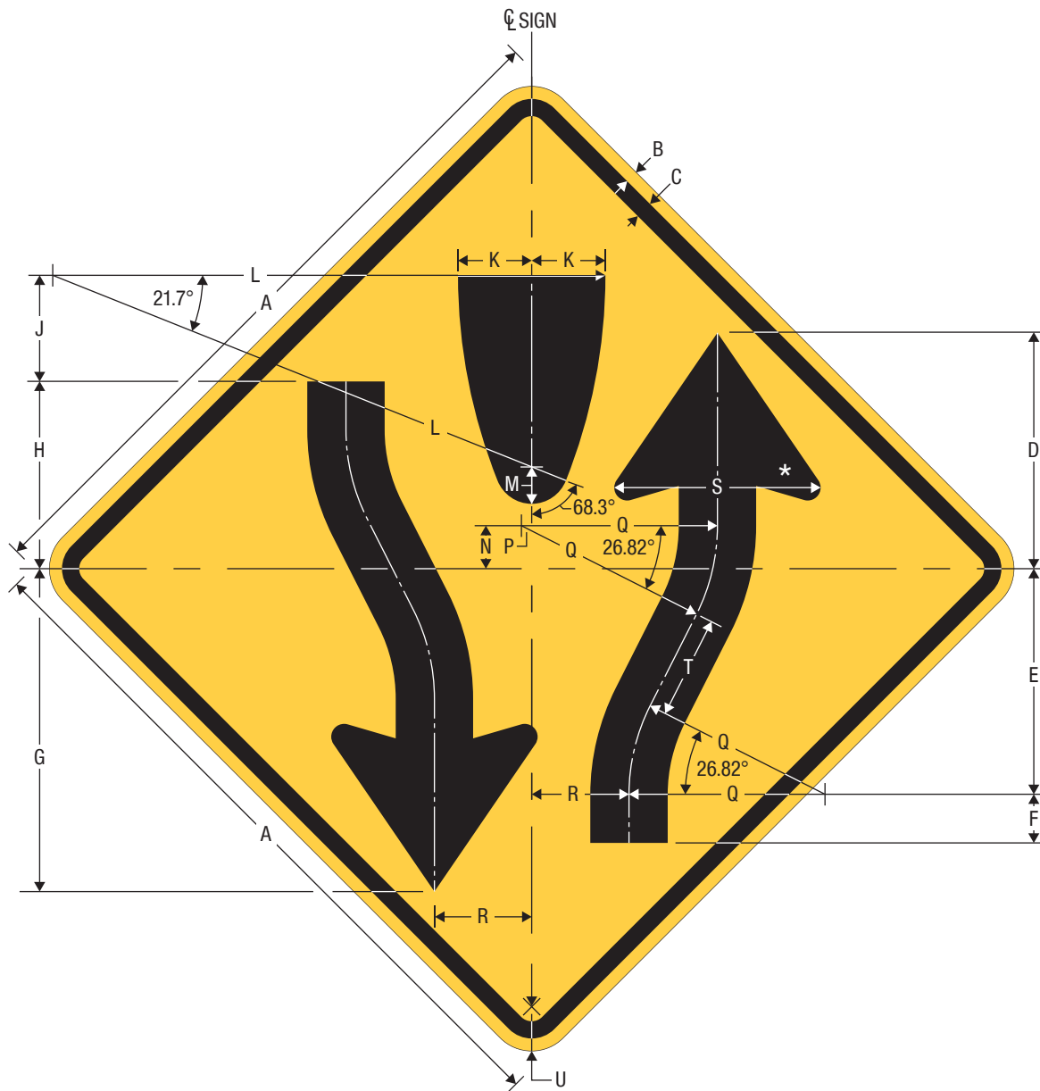
W6-1 Divided Highway
