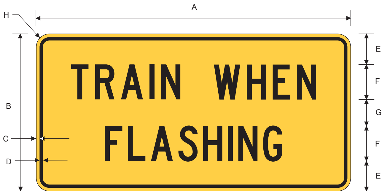
W10-17PT TRAIN WHEN FLASHING (Plaque)
