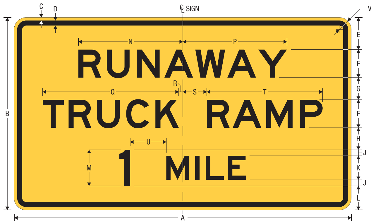
W7-4 RUNAWAY TRUCK RAMP XX MILES
