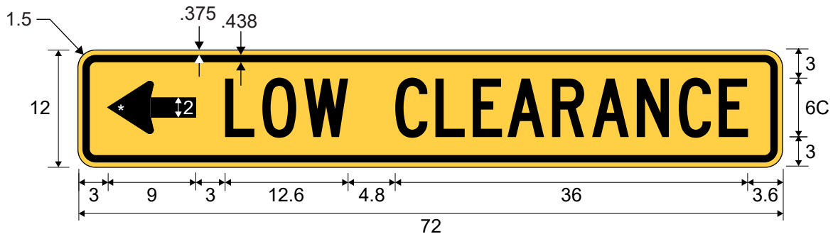
W12-3PTL LOW CLEARANCE (Plaque)
