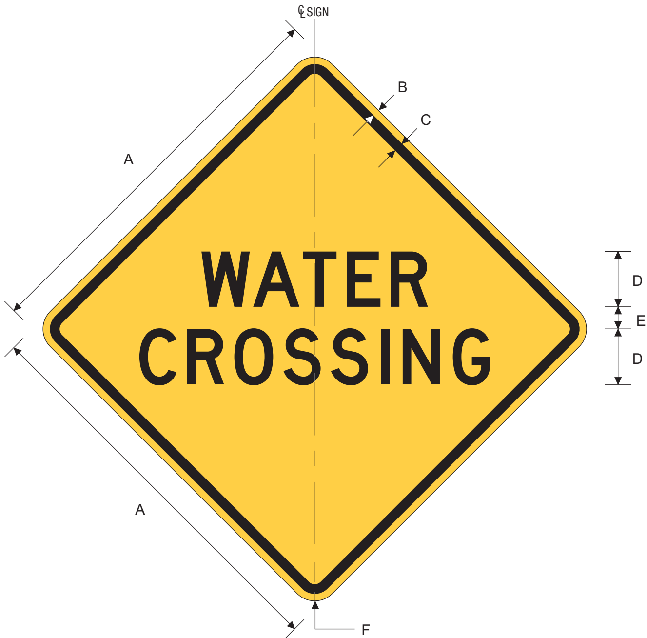
W8-18aT WATER CROSSING
