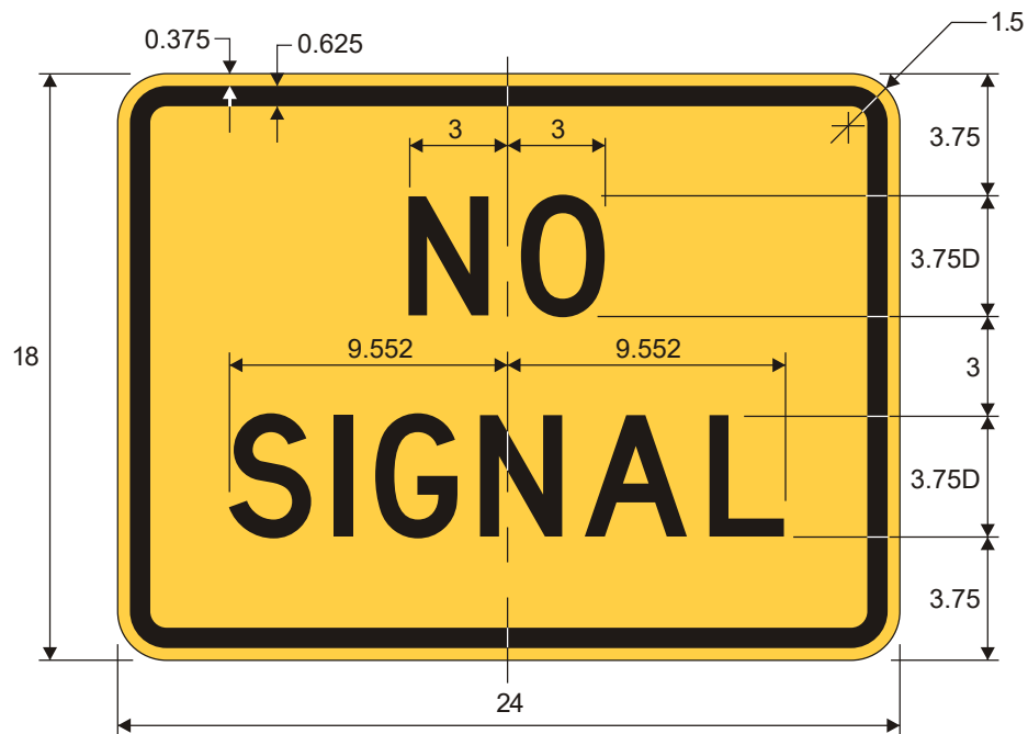
W10-10T NO SIGNAL
