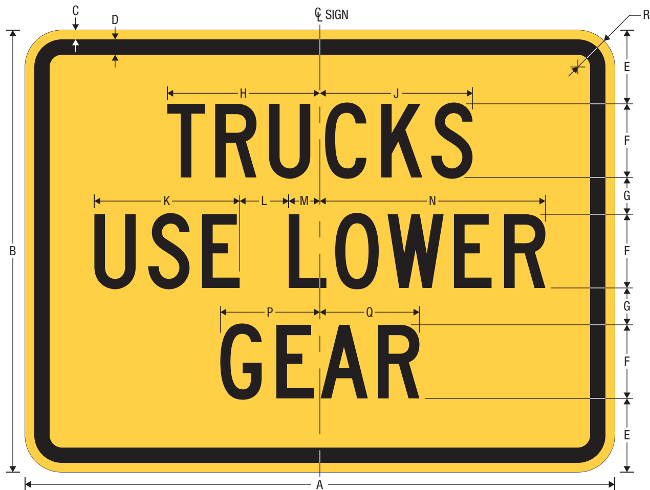
W7-2bP TRUCKS USE LOWER GEAR (Plaque)
