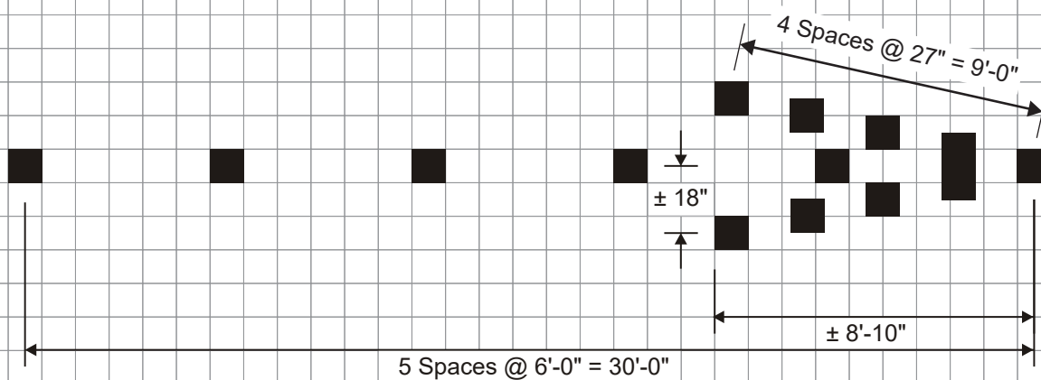
4-inch Stripe Arrow Marking
