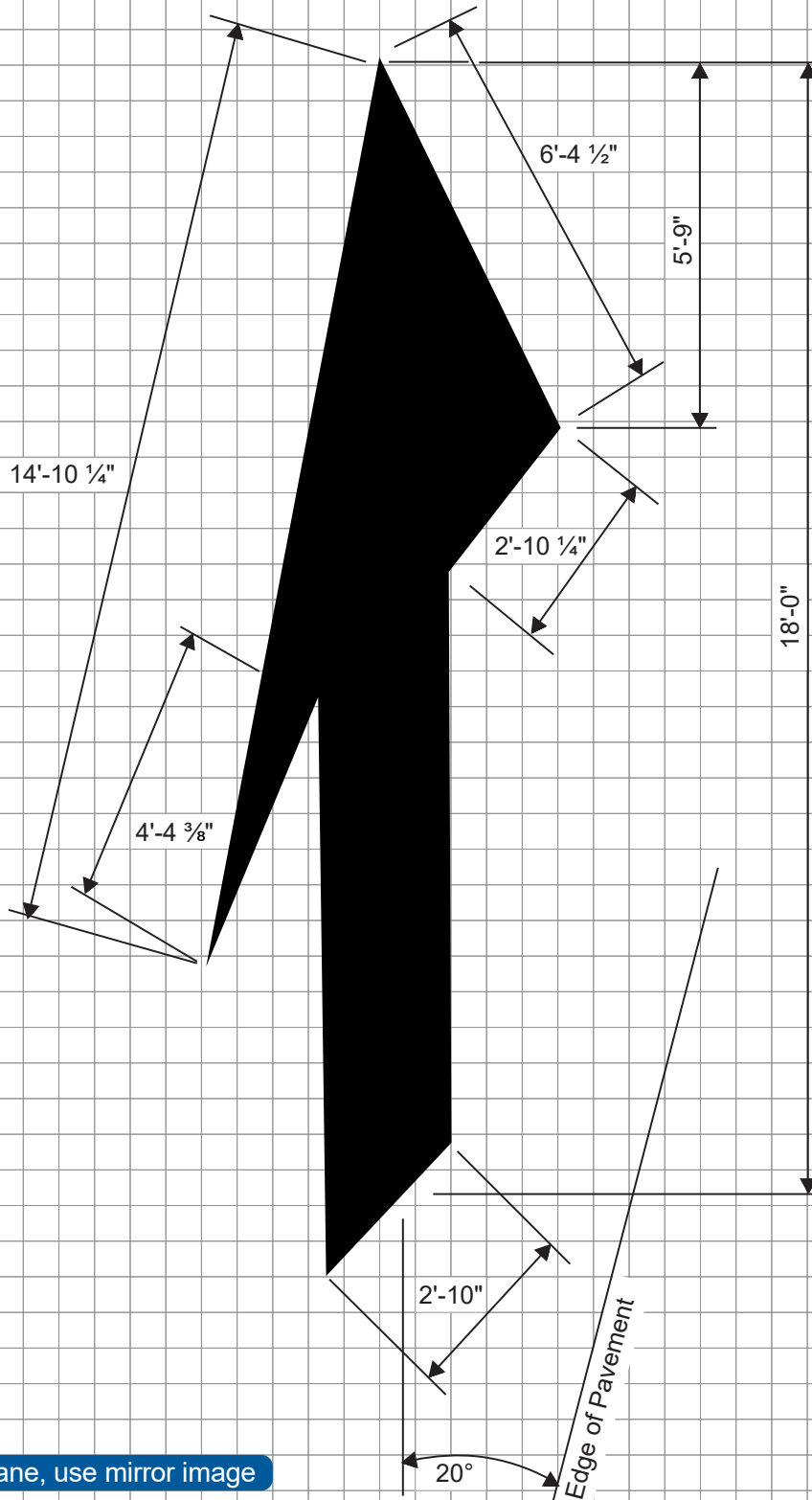
18' Lane Drop Arrow Marking (Right)
