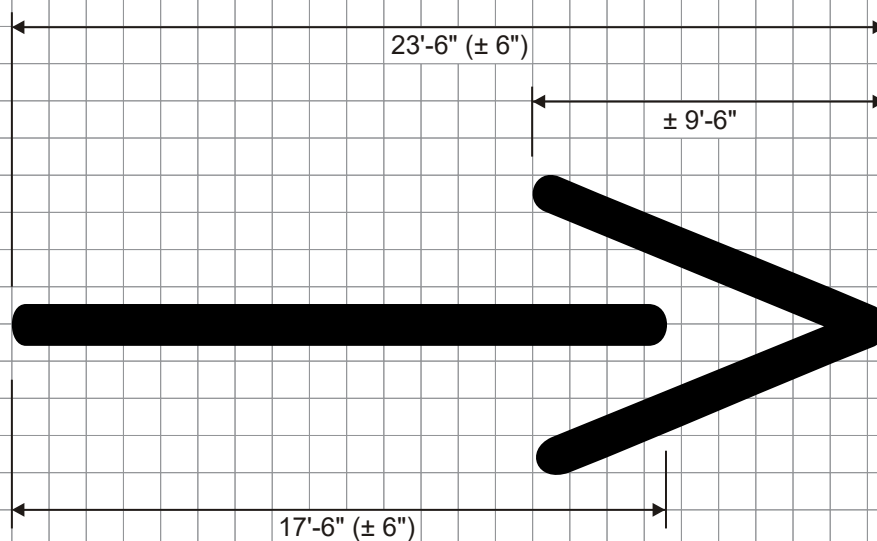
Wrong Way Arrow Marking
