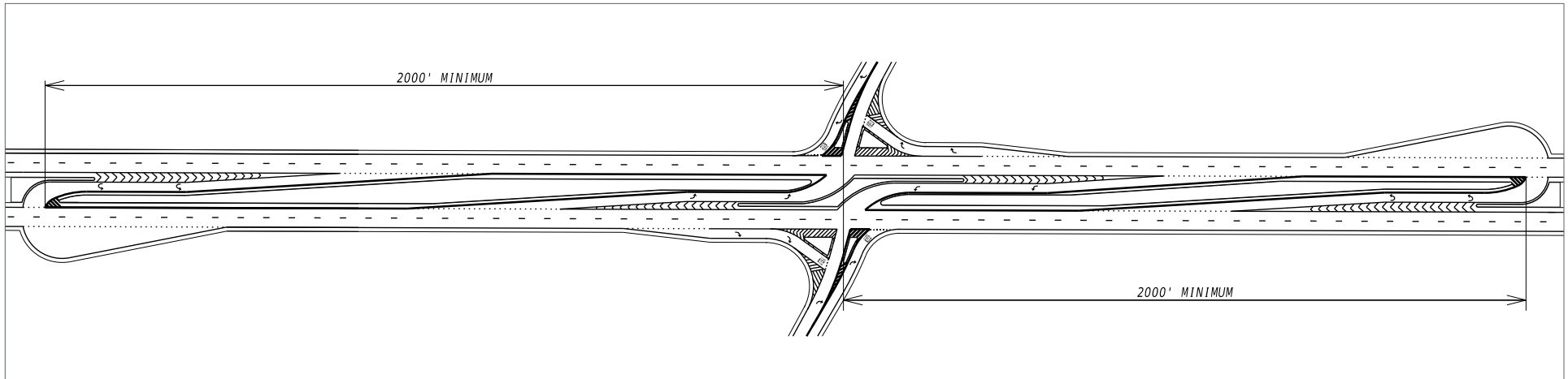
» FIGURE 4 – Non-Compact U-turn Concept Overview
