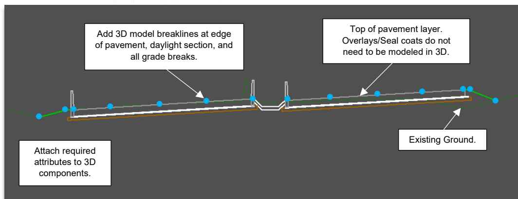
Figure 3.3 – Modeling Criteria for Roadway Full Depth Pavement
