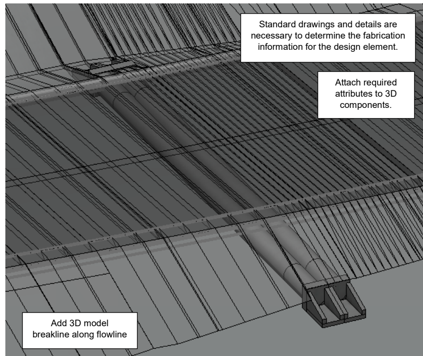
Figure 2.6 – Graphical Example for LOD 300 Design Element (Drainage Pipe)
