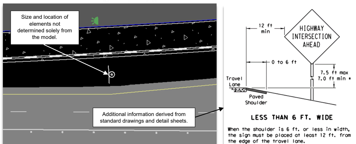
Figure 2.1 – Graphical Example for LOD 100 Design Element (Sign and Post)
