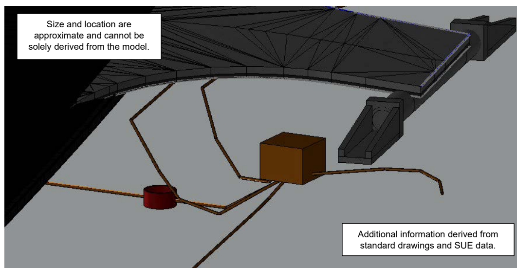
Figure 2.2 – Graphical Example for LOD 100 Design Element (Utilities – Fiber, Telecom)
