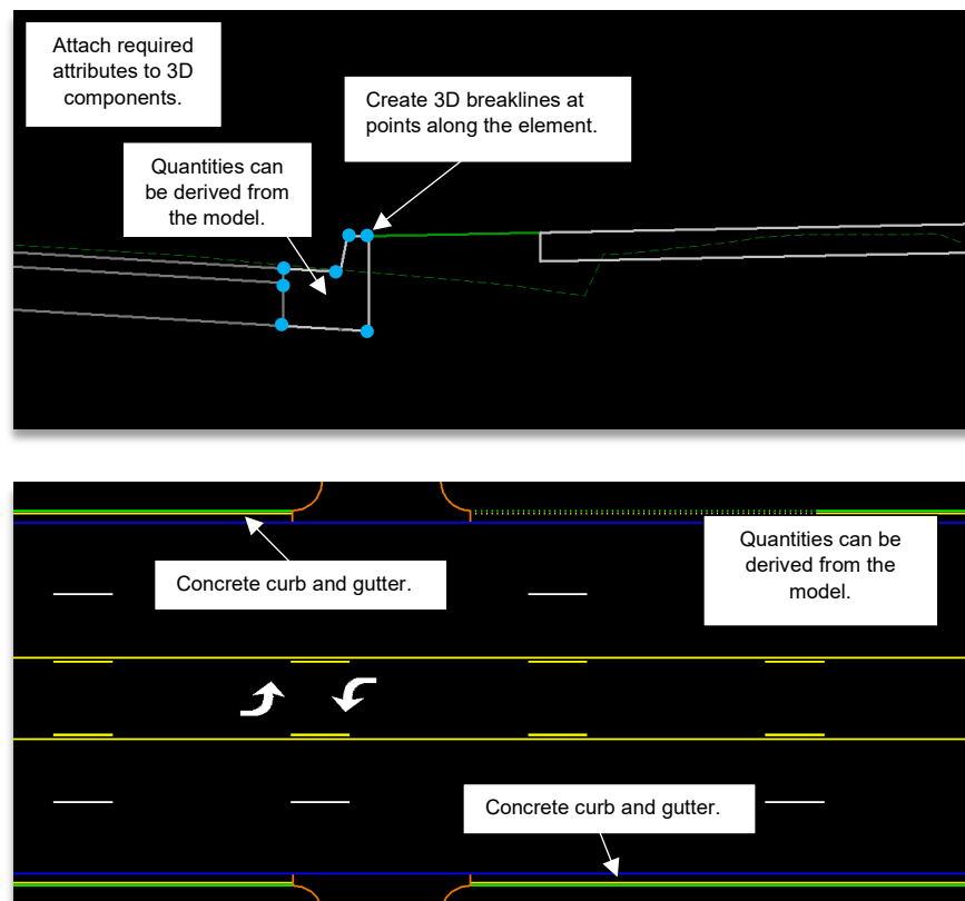
Figure 3.5 – Modeling Criteria for Curb and Gutter
