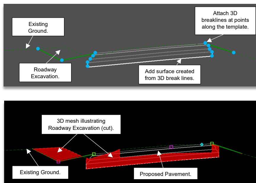
Figure 3.2 – Modeling Criteria for Roadway and/or Ditch Excavation
