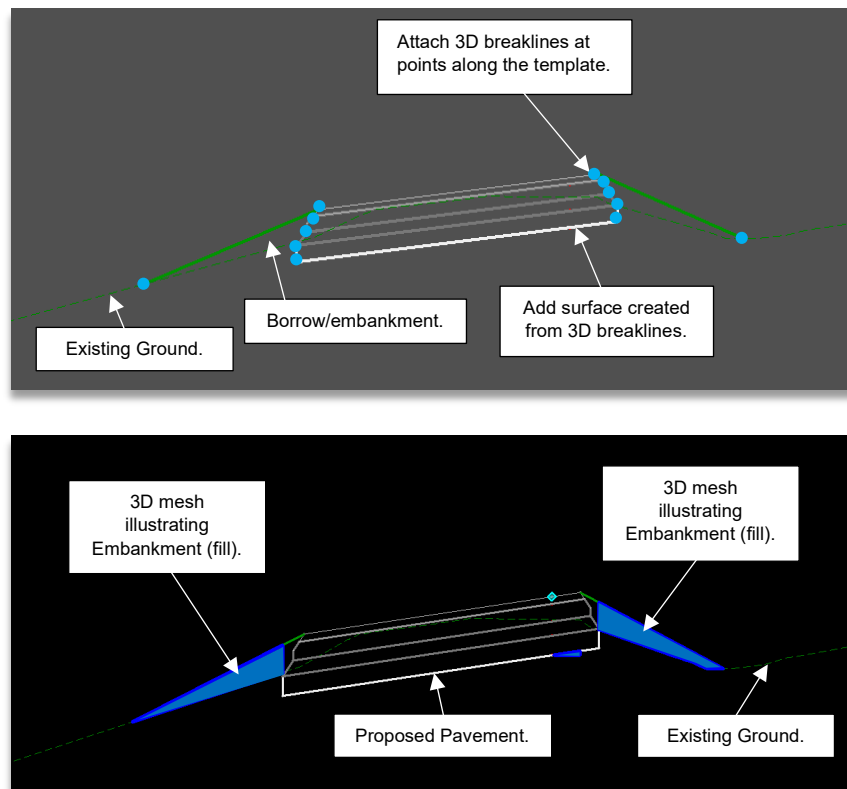
Figure 3.1 – Modeling Criteria for Roadway Embankment and Backfill
