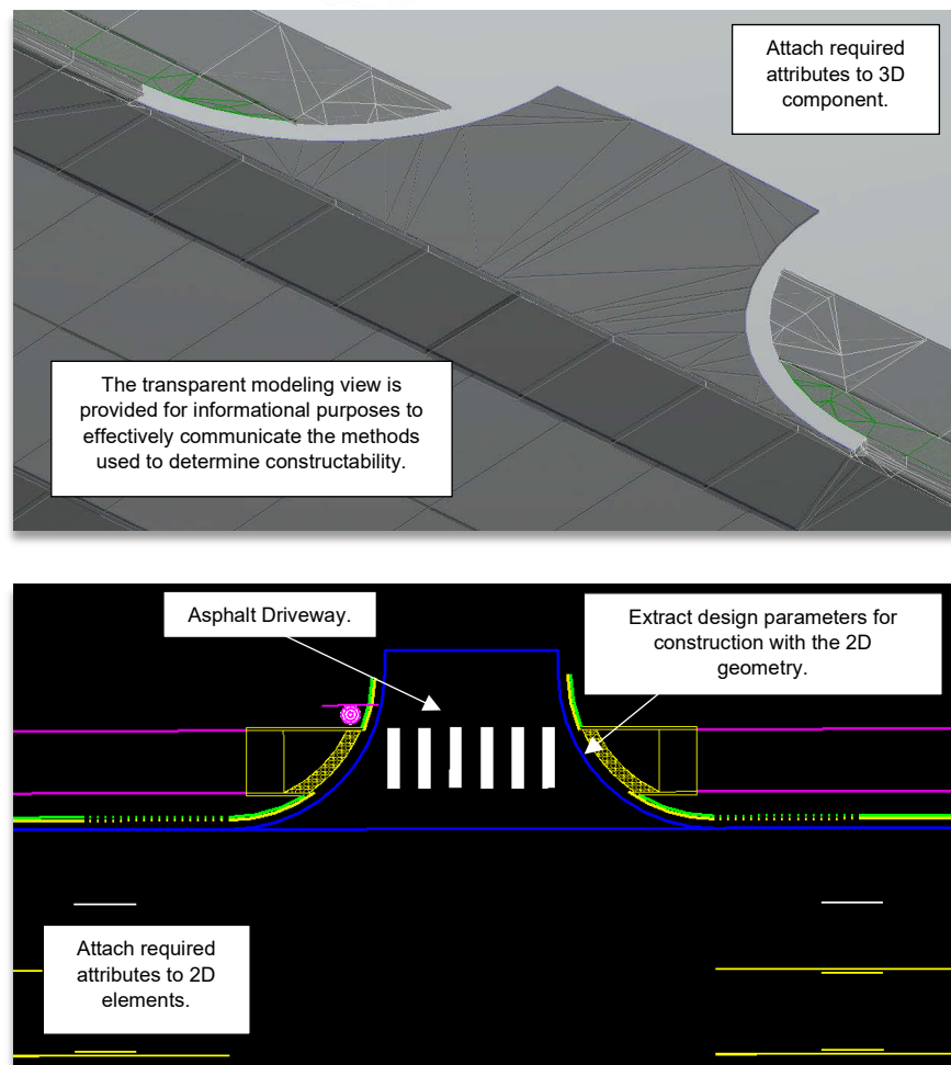
Figure 3.6 – Modeling Criteria for Driveways
