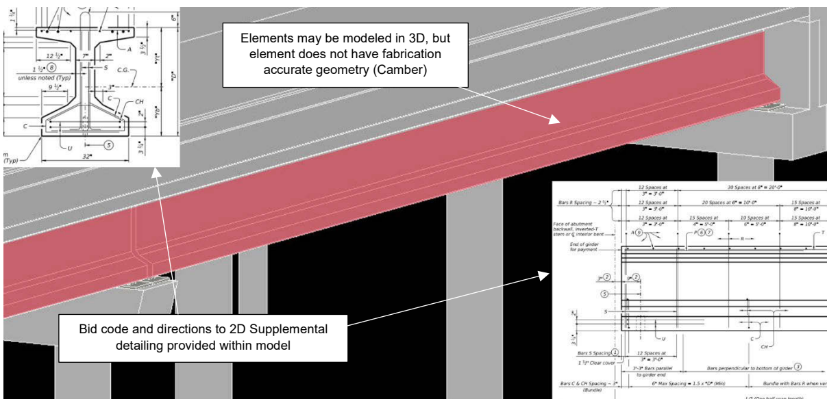
Figure 2.4 – Graphical Example for LOD 200 Design Element (Bridge Girder)
