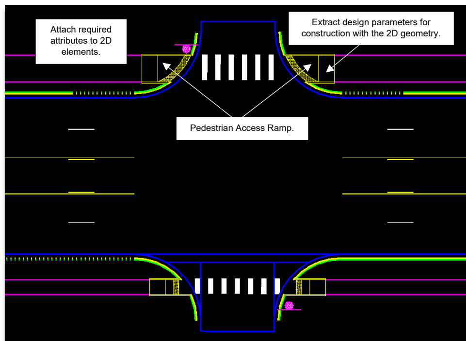
Figure 3.7 – Modeling Criteria for ADA Pedestrian Access Ramps
