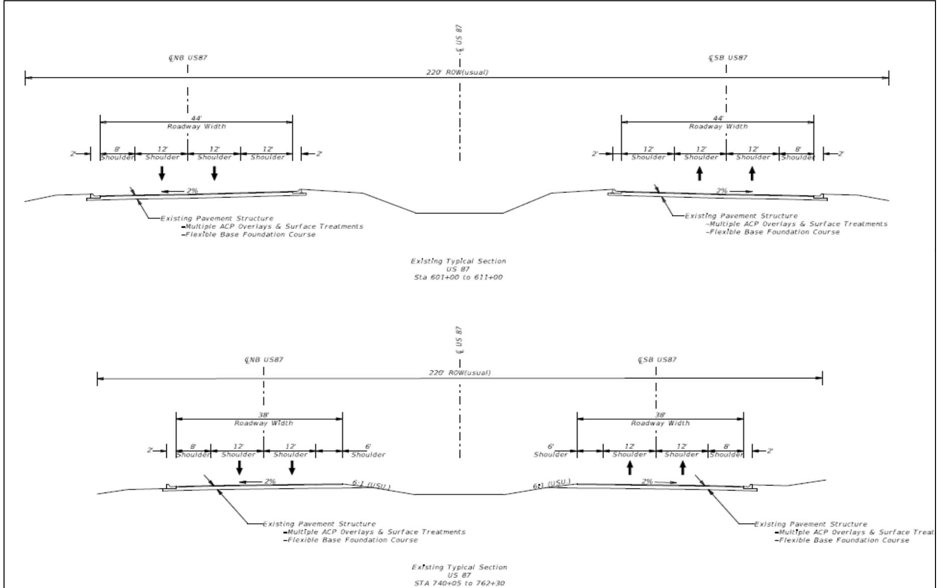
Figure 1.2. Existing Typical Sections (US 87, Tom Green County)
