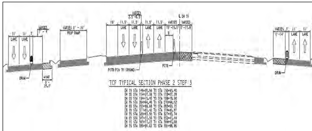
Figure 4.5. TCP Typical Section (I-35 Section 4B, McLennan County)
