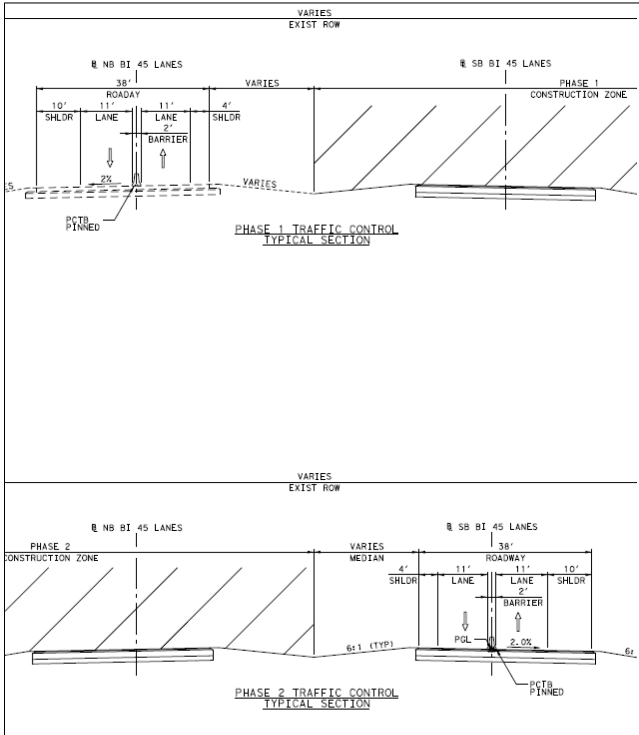
Figure 3.2. Phase 1 and Phase 2 Traffic Control Typical Sections (BI-45F, Navarro County)
