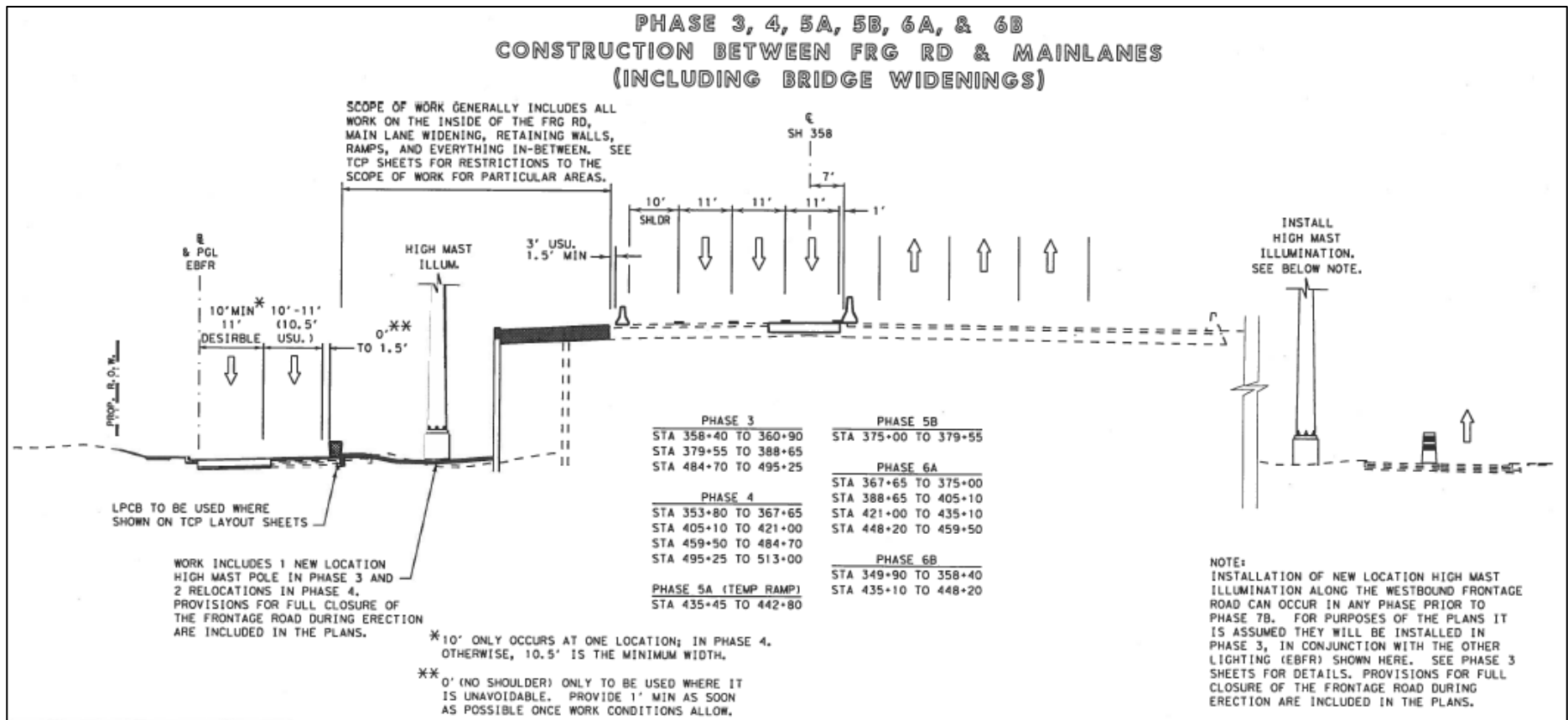
Figure 2.3. Phase Profile (SH 358, Nueces County)
