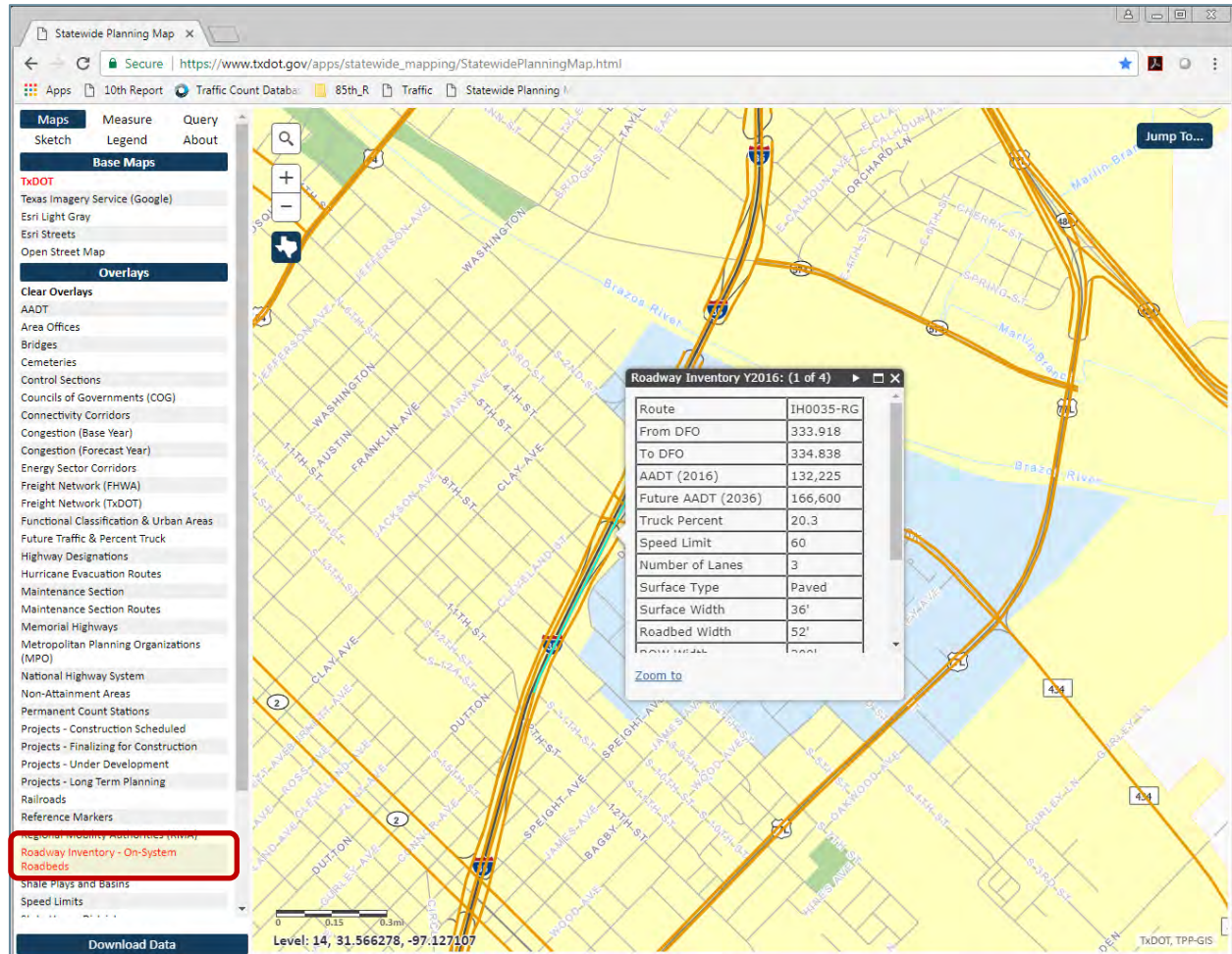
Figure 4.6. AADT from Statewide Planning Map (I-35 Section 4B, McLennan County)
