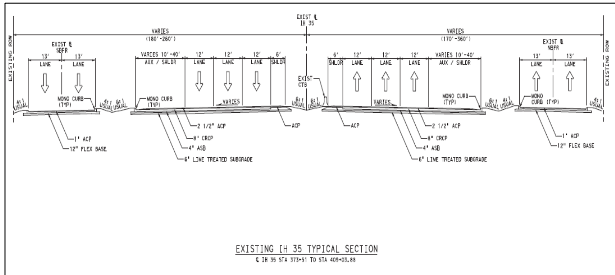
Figure 4.4. Existing Typical Section (I-35 Section 4B, McLennan County)
