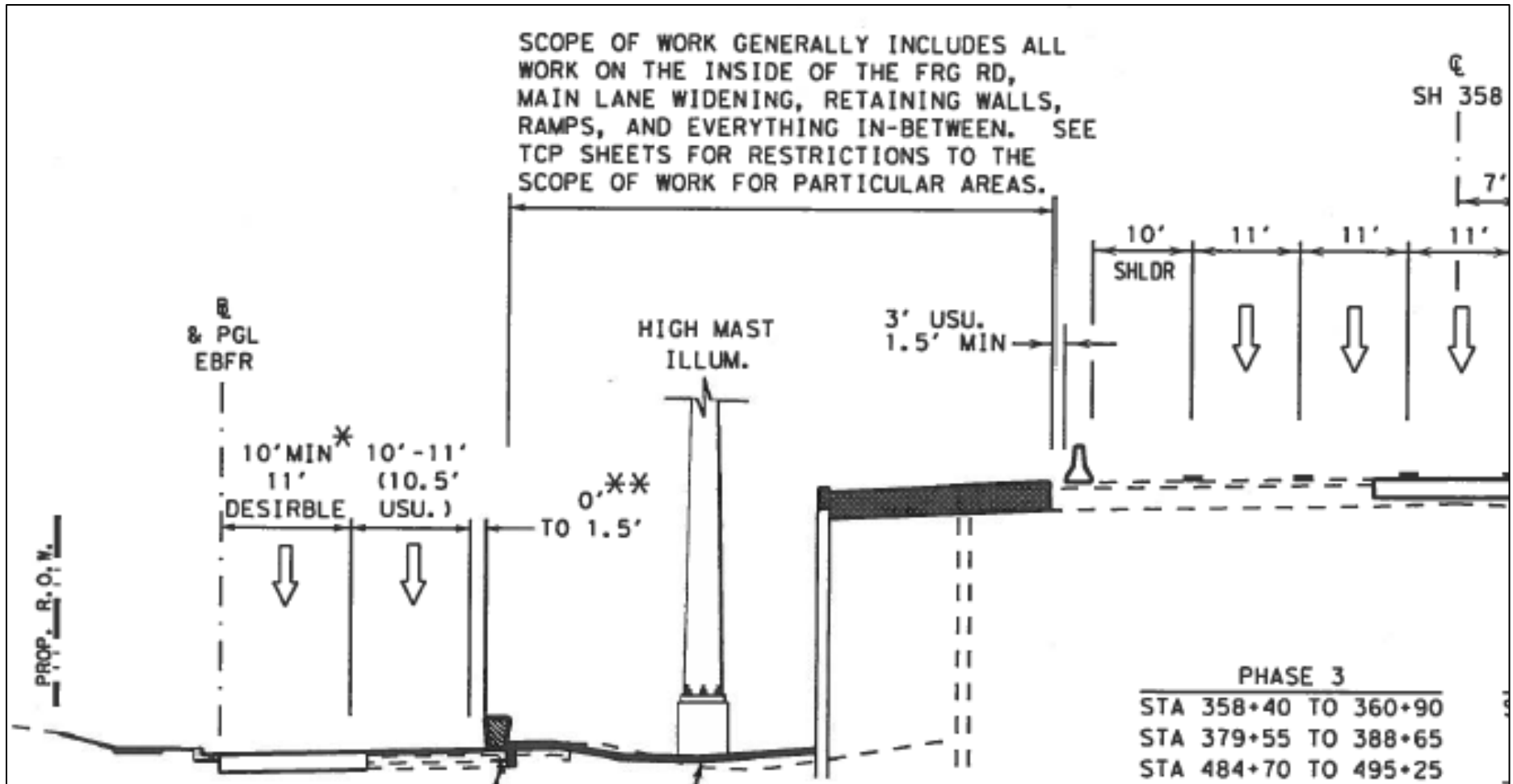
Figure 2.4. Phase 3 Profile (SH 358, Nueces County)
