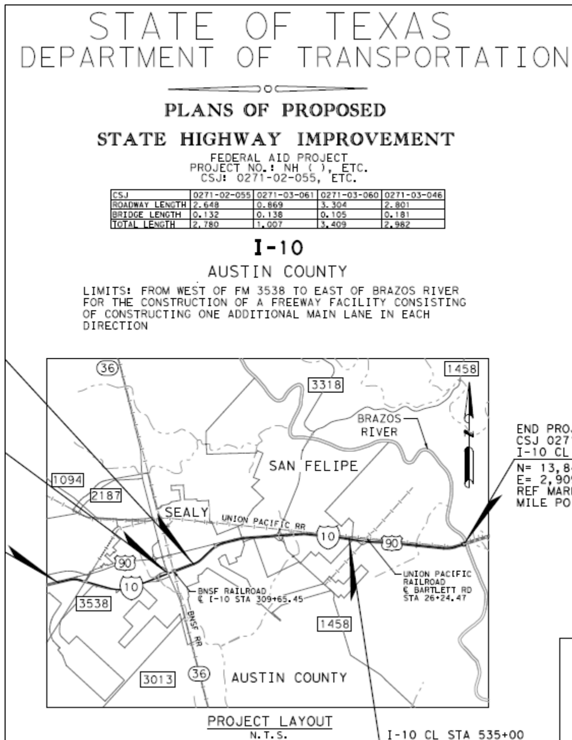
Figure 5.1. Project Title Sheet (I-10, Austin County)
