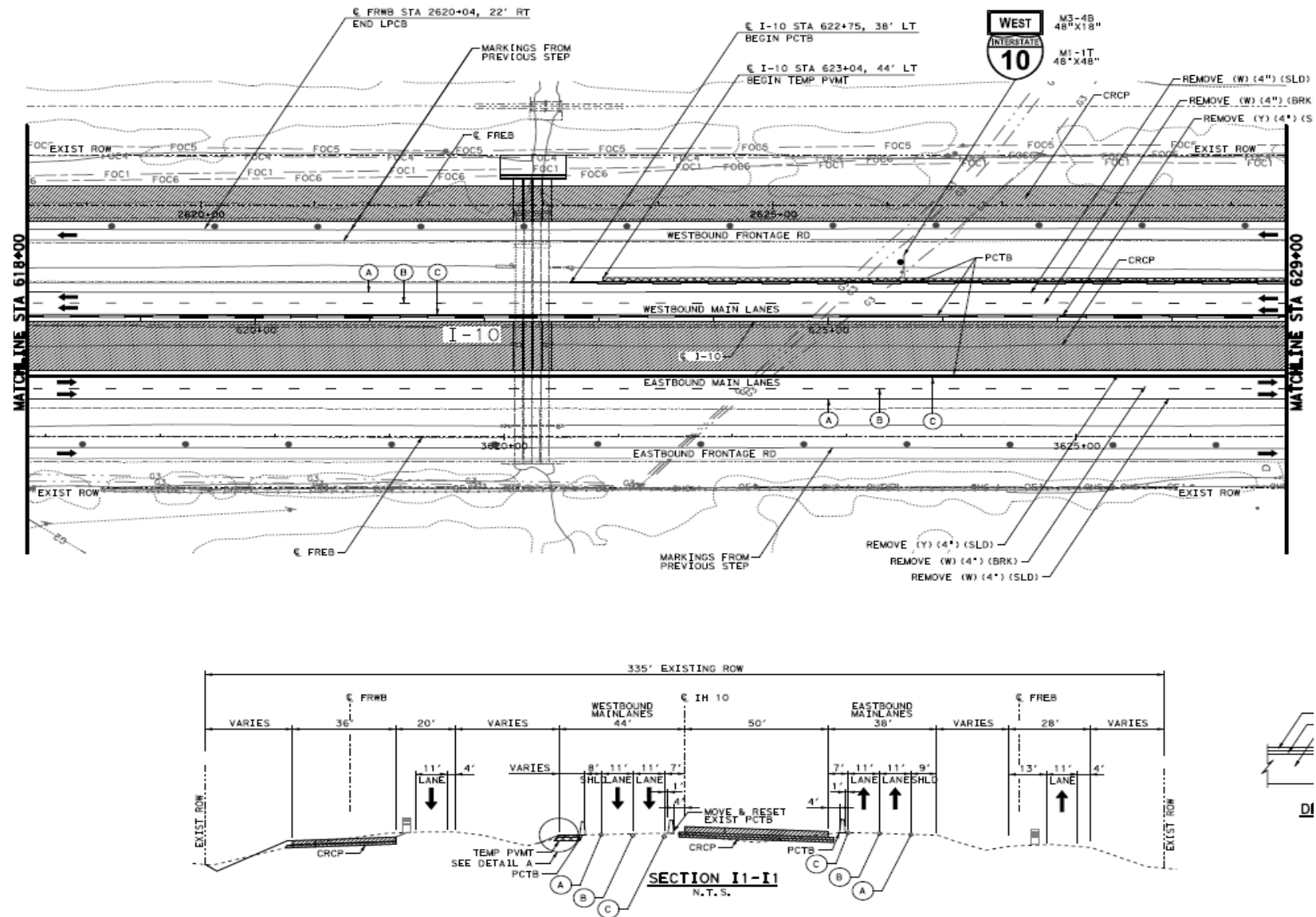
Figure 5.6. Traffic Control Plan – Phase 1
