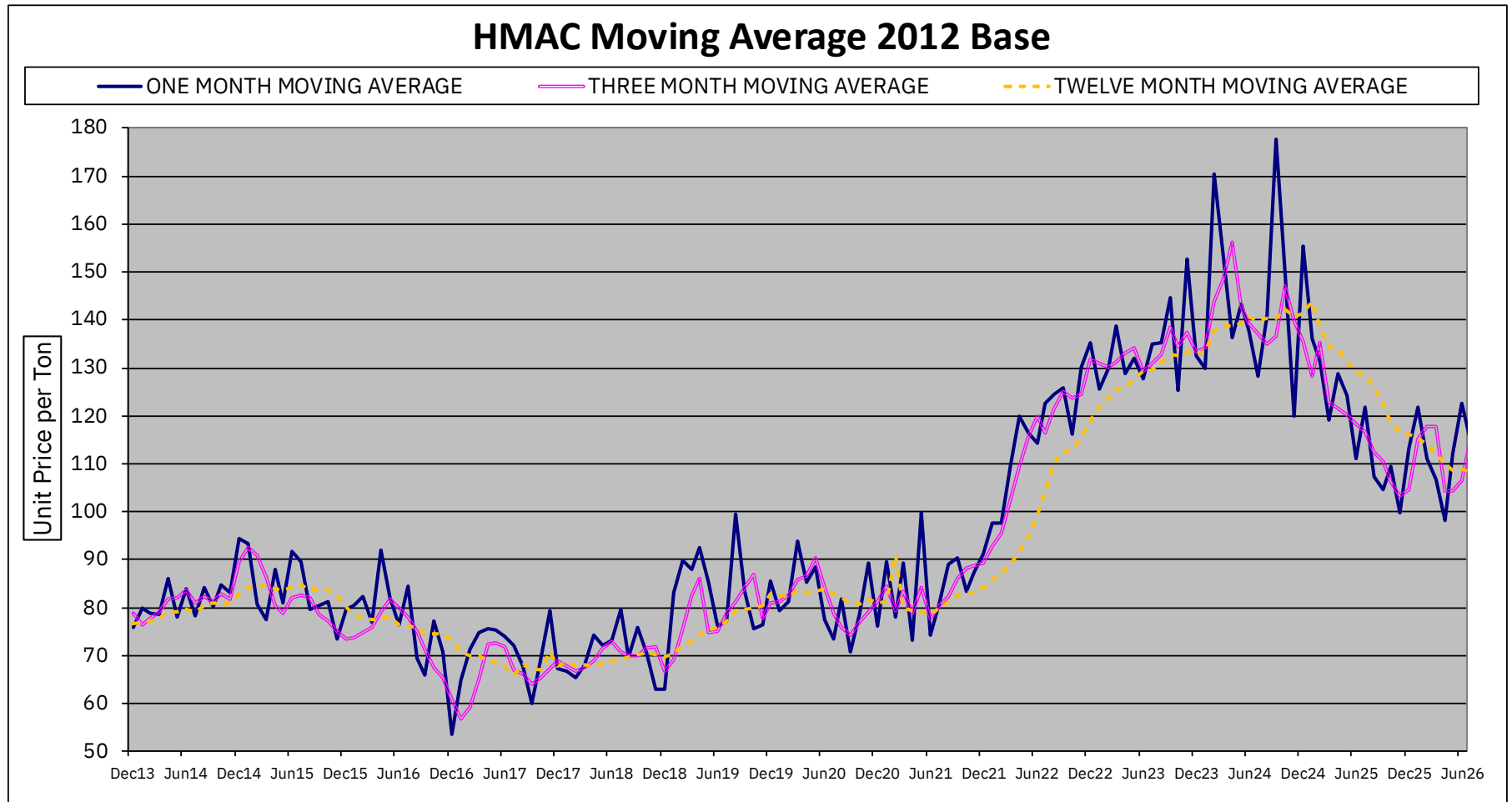
Graph 6 - Hot Mix Asphalt Concrete (HMAC) Moving Average 2012 Base
