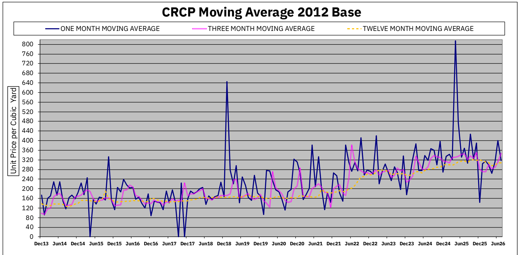
Graph 8 - Continuously Reinforced Concrete Pavement (CRCP) Moving Average (2012 Base)
