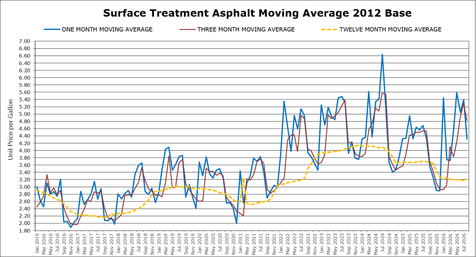
Graph 7 - Surface Treatment Asphalt Moving Average 2012 Base
