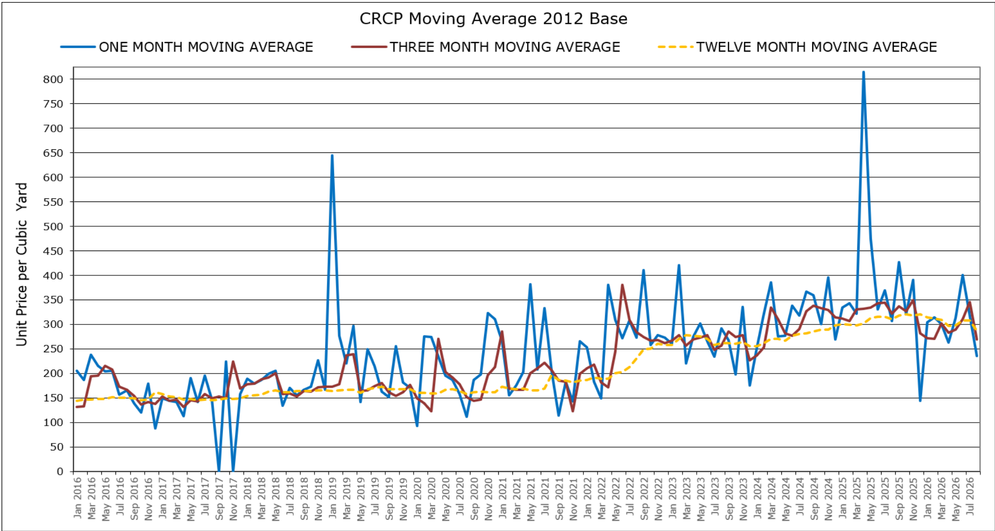
Graph 8 - Continuously Reinforced Concrete Pavement (CRCP) Moving Average (2012 Base)
