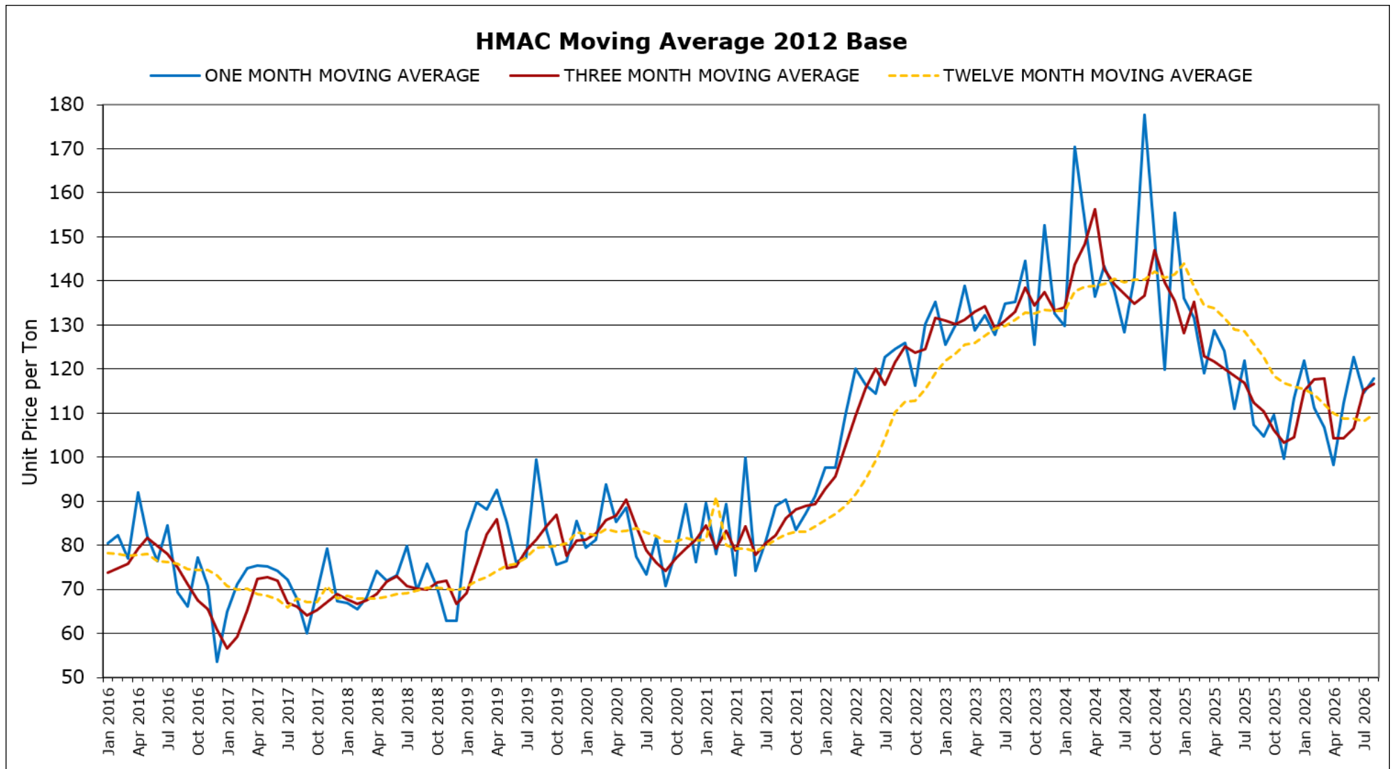
Graph 6 - Hot Mix Asphalt Concrete (HMAC) Moving Average 2012 Base
