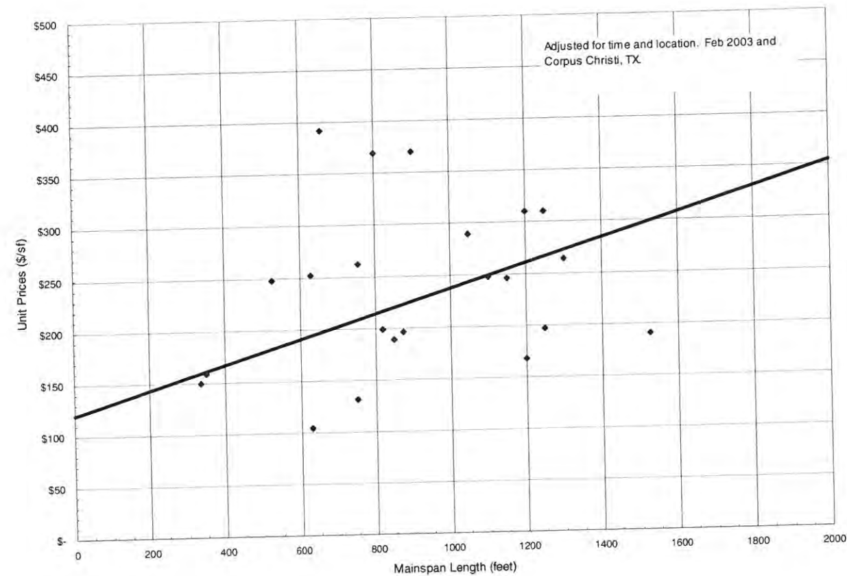
FIGURE 4.3-4 HISTORICAL PRICES FOR LONG SPAN BRIDGES IN NORTH AMERICA
