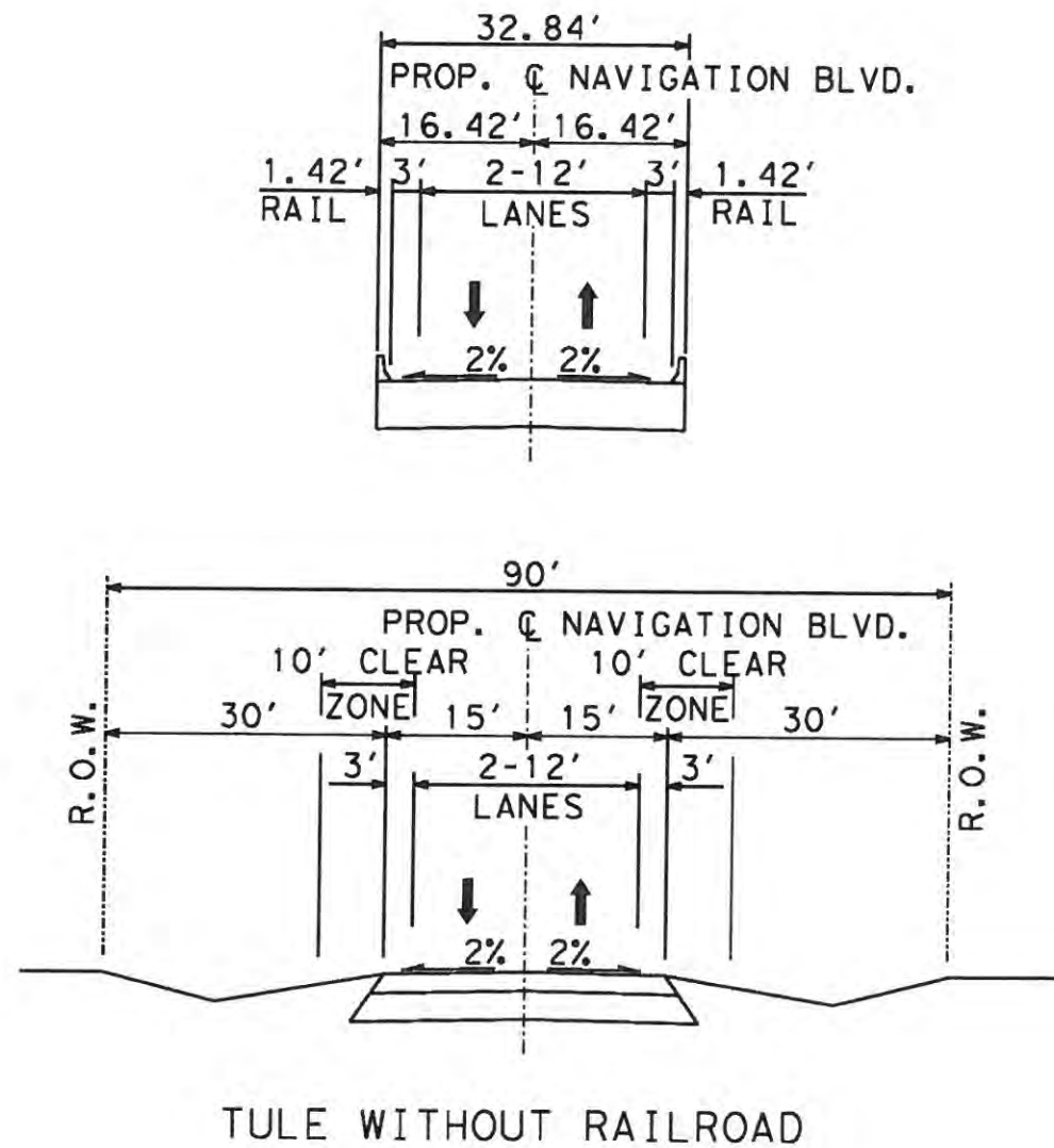
FIGURE 4.1-4 TULE LAKE LIFT BRIDGE WITHOUT RAIL TYPICAL CROSS SECTION
