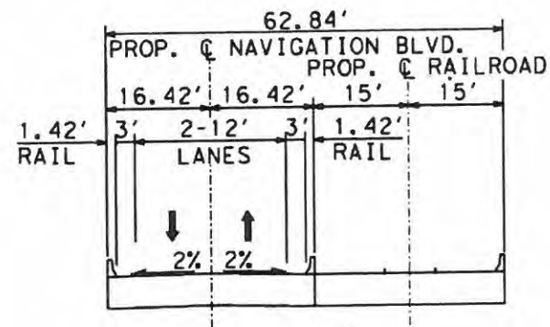
FIGURE 4.1-3 TULE LAKE LIFT BRIDGE WITH RAIL TYPICAL CROSS SECTION
