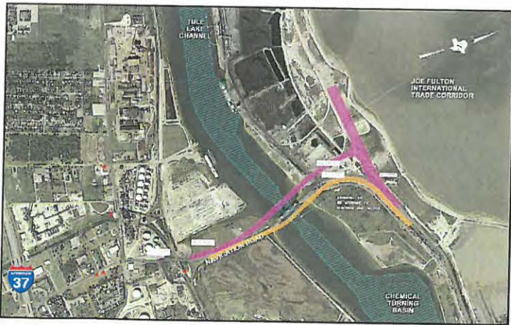
MID-LEVEL WITH RAIL
