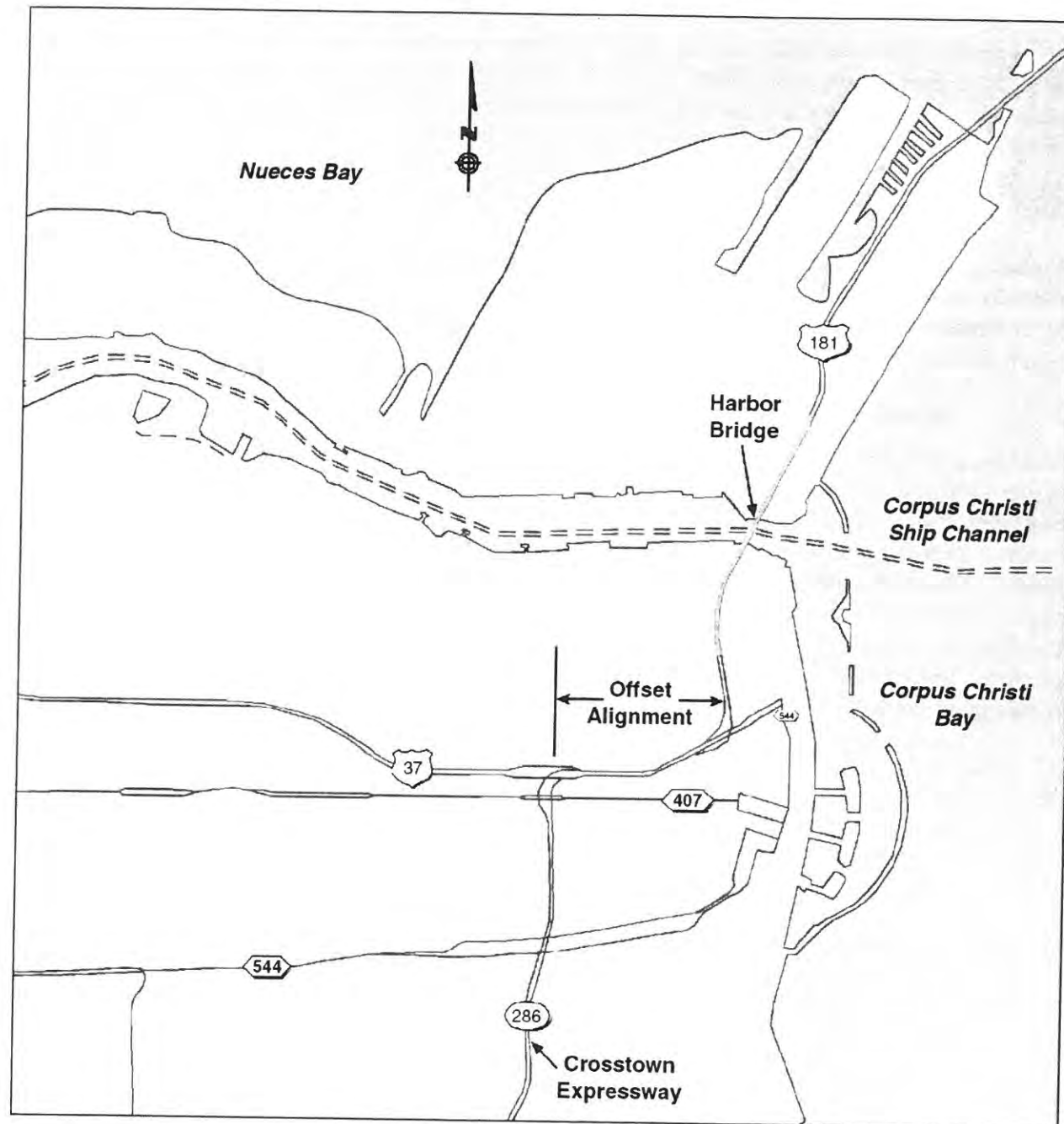
FIGURE 2.2-1 OFFSET BETWEEN SH 286 AND U.S. 181
