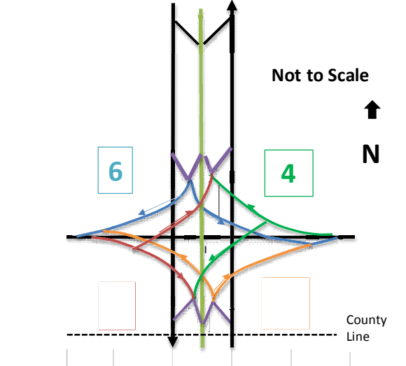
SH 288 Tolloed Lanes @ BW8 Stick Diagram
