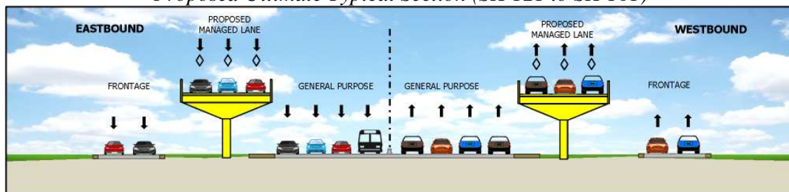
Proposed Ultimate Typical Section (SH 121 to SH 161)
