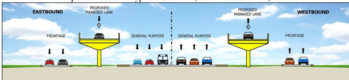
Proposed Phase 1 Typical Section (SH 121 to SH 161)
