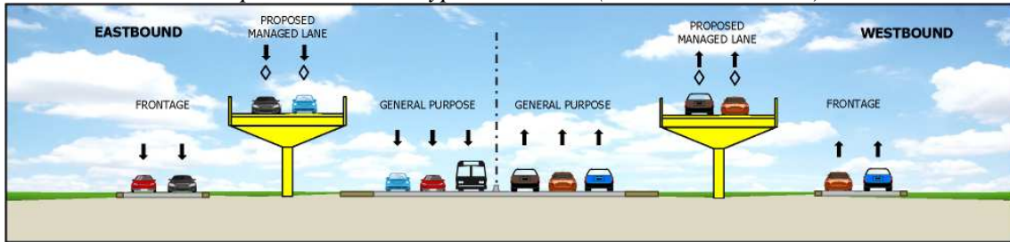
Proposed Phase 2 Typical Section (SH 121 to SH 161)
